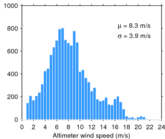
Figure 35. Histogram of science-valid wind over oceans and lakes for 05/07/2017. The mean ( \mu ) and standard deviation ( \sigma ) are also shown. Note that values larger than 24 m/s are excluded from the histogram for the sake of readability but not from the computation of \mu and \sigma .
