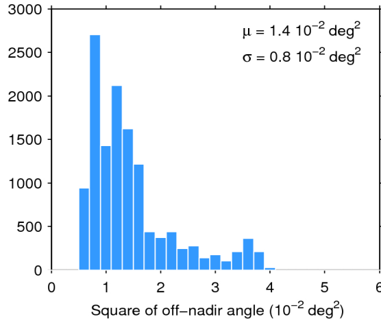
Figure 39. Histogram of flag-valid mispointing over oceans and lakes for 05/07/2017. The mean ( \mu ) and standard deviation ( \sigma ) are also shown. Note that values larger than 6 \cdot 10^{-2} \text{ deg}^2 are excluded from the histogram for the sake of readability but not from the computation of \mu and \sigma .
