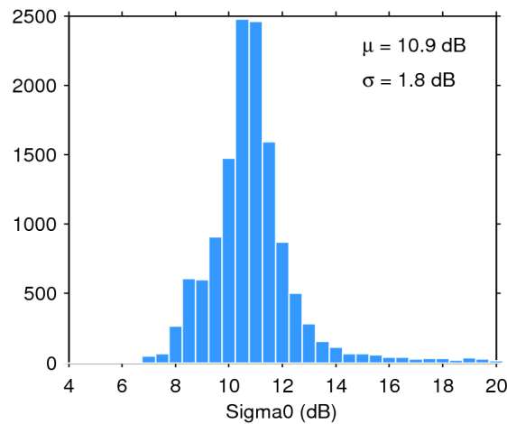
Figure 25. Histogram of flag-valid sigma0 over oceans and lakes for 05/07/2017. The mean ( \mu ) and standard deviation ( \sigma ) are also shown. Note that values outside [4 20] dB are excluded from the histogram for the sake of readability but not from the computation of \mu and \sigma .
