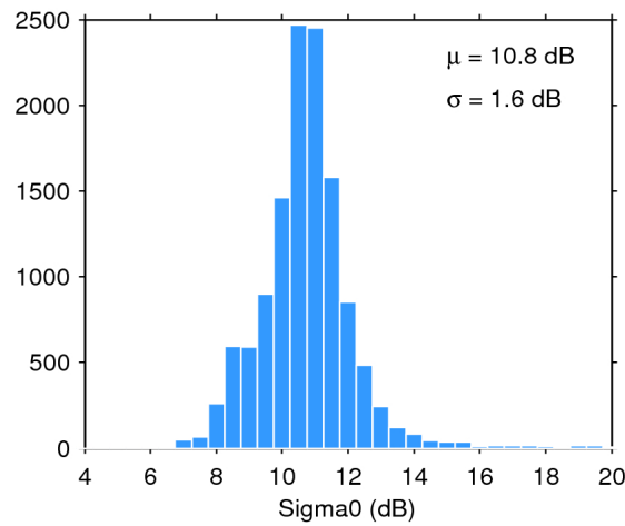
Figure 28. Histogram of science-valid sigma0 over oceans and lakes for 05/07/2017. The mean ( \mu ) and standard deviation ( \sigma ) are also shown. Note that values outside [4 20] dB are excluded from the histogram for the sake of readability but not from the computation of \mu and \sigma .
