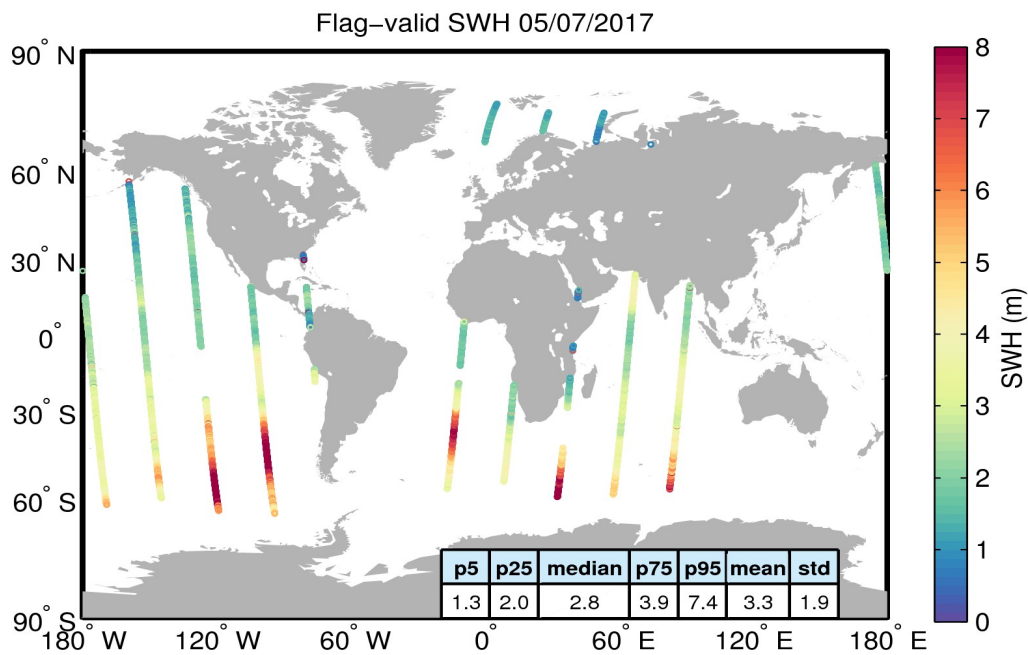
Figure 15. Geographical distribution of flag-valid SWH data over oceans and lakes for 05/07/2017. The statistical values shown in the table refer to the SWH in m and are calculated over all measurements shown in the figure.
