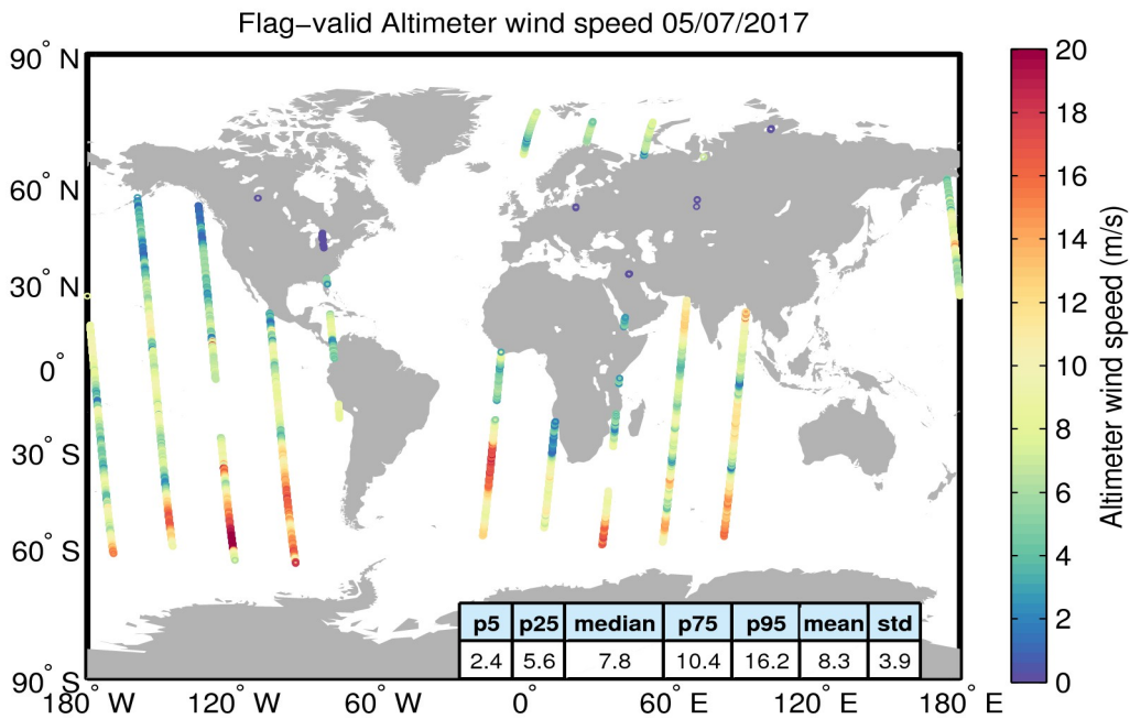
Figure 31. Geographical distribution of flag-valid wind data over oceans and lakes for 05/07/2017. The statistical values shown in the table refer to the wind in m/s and are calculated over all measurements shown in the figure.
