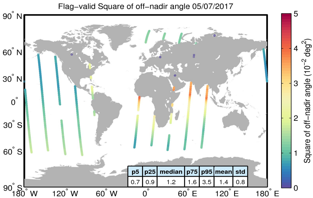
Figure 37. Geographical distribution of flag-valid mispointing data over oceans and lakes for 05/07/2017. The statistical values shown in the table refer to the mispointing in 10^{-2} deg 2 and are calculated over all measurements shown in the figure.
