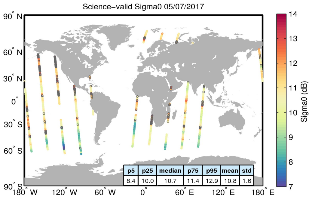
Figure 27. Geographical distribution of science-valid sigma0 data over oceans and lakes for 05/07/2017. The statistical values shown in the table refer to the sigma0 in dB and are calculated over all measurements shown in the figure. Gray circles denote records that have been rejected based on the editing criteria described in Table 4.
