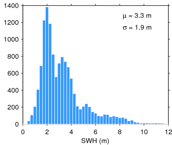
Figure 17. Histogram of flag-valid SWH over oceans and lakes for 05/07/2017. The mean ( \mu ) and standard deviation ( \sigma ) are also shown. Note that values larger than 12 m are excluded from the histogram for the sake of readability but not from the computation of \mu and \sigma .
