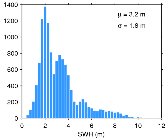
Figure 20. Histogram of science-valid SWH over oceans and lakes for 05/07/2017. The mean ( \mu ) and standard deviation ( \sigma ) are also shown. Note that values larger than 12 m are excluded from the histogram for the sake of readability but not from the computation of \mu and \sigma .
