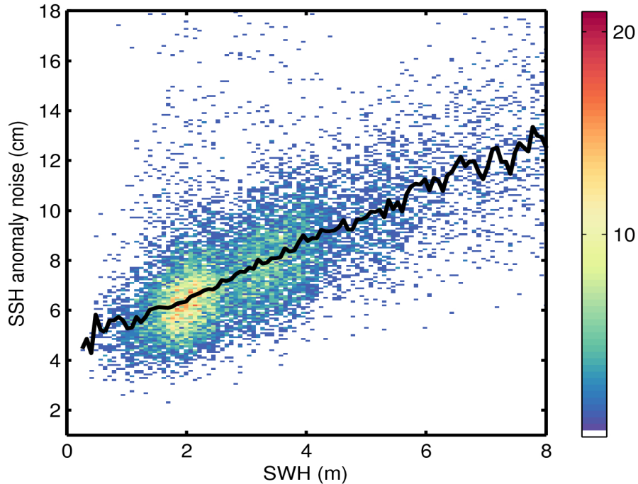
Figure 9. 2D histogram showing flag-valid SSH anomaly noise as a function of SWH for 05/07/2017. The black line denotes the median SSH anomaly noise as a function of SWH.
