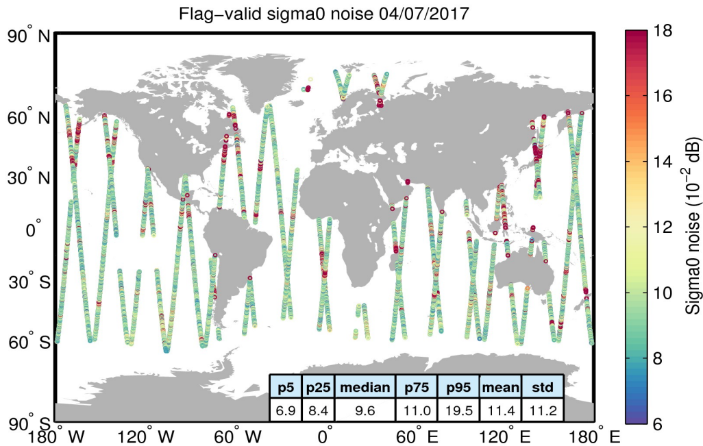
Figure 26. Geographical distribution of flag-valid 20-Hz sigma0 measurement noise over oceans and lakes for 04/07/2017. The statistical values shown in the table refer to the sigma0 noise and are calculated over all measurements shown in the figure.
