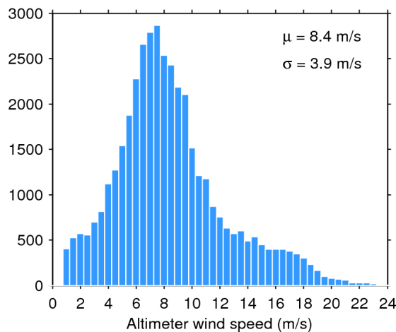
Figure 35. Histogram of science-valid wind over oceans and lakes for 04/07/2017. The mean ( \mu ) and standard deviation ( \sigma ) are also shown. Note that values larger than 24 m/s are excluded from the histogram for the sake of readability but not from the computation of \mu and \sigma .
