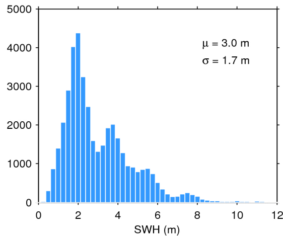
Figure 17. Histogram of flag-valid SWH over oceans and lakes for 04/07/2017. The mean ( \mu ) and standard deviation ( \sigma ) are also shown. Note that values larger than 12 m are excluded from the histogram for the sake of readability but not from the computation of \mu and \sigma .
