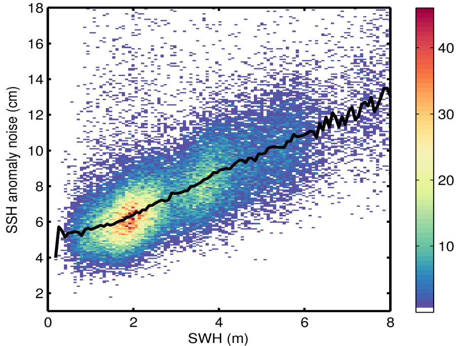
Figure 9. 2D histogram showing flag-valid SSH anomaly noise as a function of SWH for 04/07/2017. The black line denotes the median SSH anomaly noise as a function of SWH.
