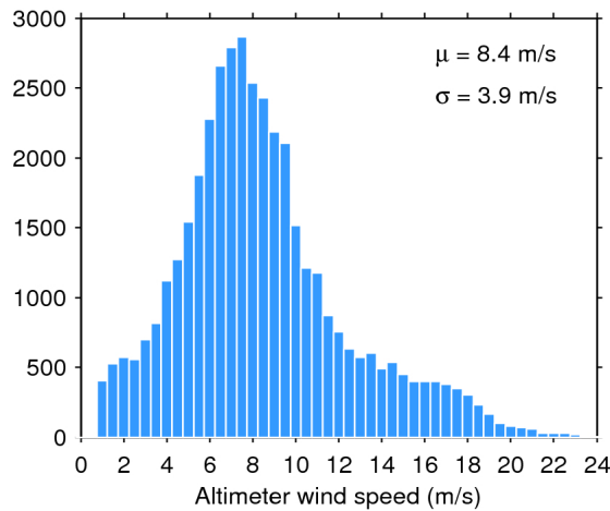
Figure 33. Histogram of flag-valid wind over oceans and lakes for 04/07/2017. The mean ( \mu ) and standard deviation ( \sigma ) are also shown. Note that values larger than 24 m/s are excluded from the histogram for the sake of readability but not from the computation of \mu and \sigma .
