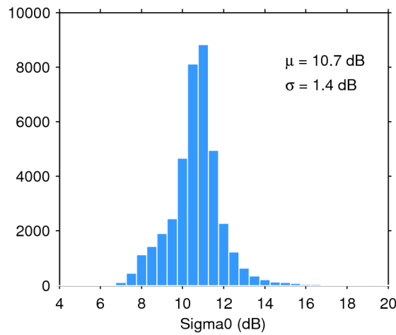
Figure 28. Histogram of science-valid sigma0 over oceans and lakes for 04/07/2017. The mean ( \mu ) and standard deviation ( \sigma ) are also shown. Note that values outside [4 20] dB are excluded from the histogram for the sake of readability but not from the computation of \mu and \sigma .
