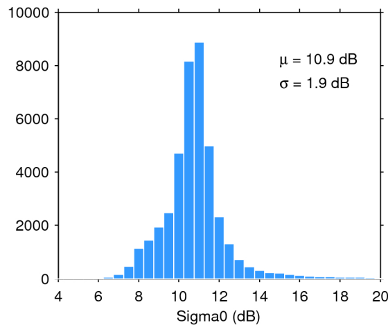
Figure 25. Histogram of flag-valid sigma0 over oceans and lakes for 04/07/2017. The mean ( \mu ) and standard deviation ( \sigma ) are also shown. Note that values outside [4 20] dB are excluded from the histogram for the sake of readability but not from the computation of \mu and \sigma .
