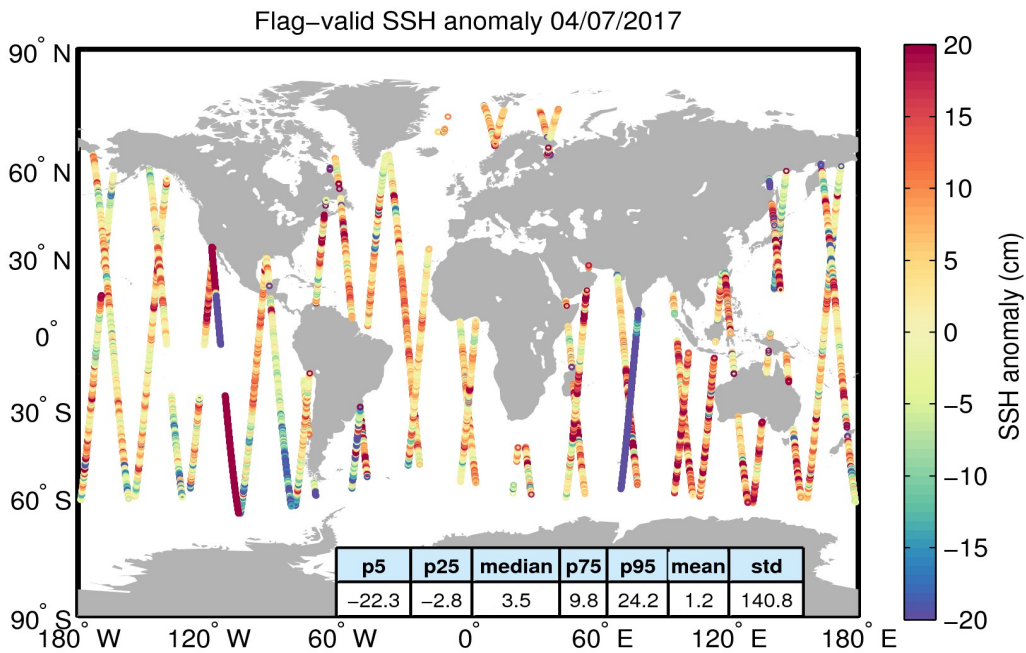
Figure 5. Geographical distribution of flag-valid 1-Hz SSH anomaly data over oceans and lakes for 04/07/2017. The statistical values shown in the table refer to the SSH anomaly in cm and are calculated over all measurements shown in the figure.
