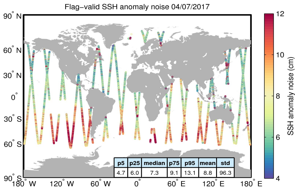
Figure 8. Geographical distribution of flag-valid 20-Hz SSH anomaly measurement noise over oceans and lakes for 04/07/2017. The statistical values shown in the table refer to the SSH anomaly noise and are calculated over all measurements shown in the figure.
