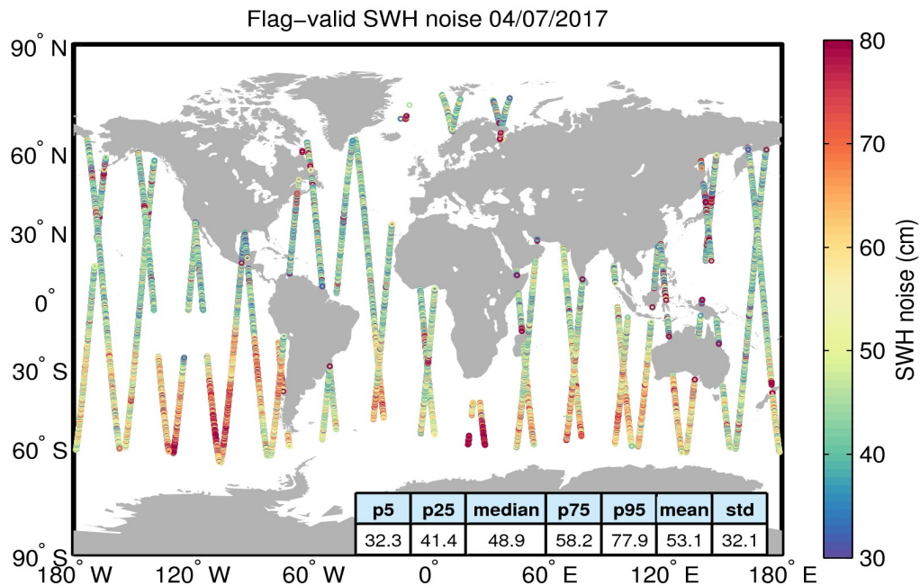
Figure 18. Geographical distribution of flag-valid 20-Hz SWH measurement noise over oceans and lakes for 04/07/2017. The statistical values shown in the table refer to the SWH noise and are calculated over all measurements shown in the figure.
