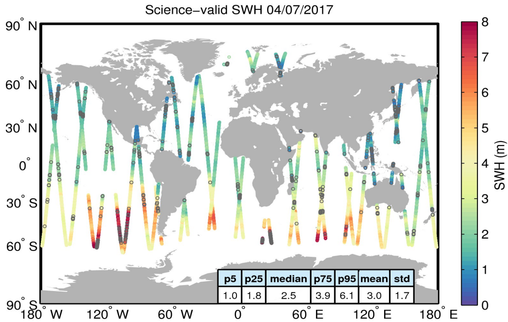
Figure 19. Geographical distribution of science-valid SWH data over oceans and lakes for 04/07/2017. The statistical values shown in the table refer to the SWH in m and are calculated over all measurements shown in the figure. Gray circles denote records that have been rejected based on the editing criteria described in Table 3.
