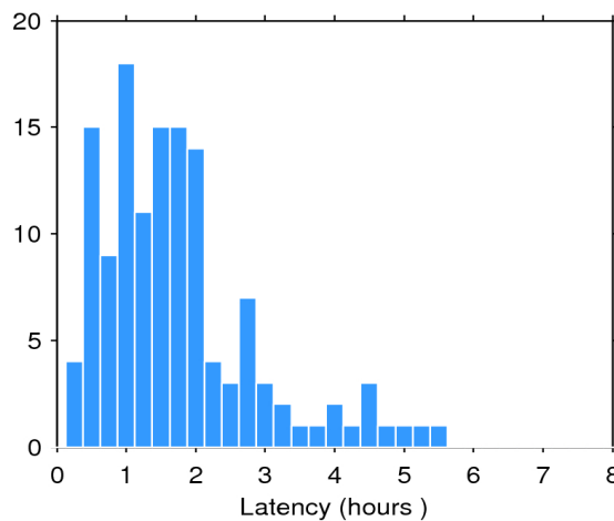
Figure 2. Histogram of the data latency for 04/07/2017. The y-axis denotes the number of files that are made available with a delay of x-hours with respect to the mean time of the records stored in the file.
