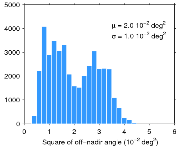
Figure 39. Histogram of flag-valid mispointing over oceans and lakes for 04/07/2017. The mean ( \mu ) and standard deviation ( \sigma ) are also shown. Note that values larger than 6 \cdot 10^{-2} \text{ deg}^2 are excluded from the histogram for the sake of readability but not from the computation of \mu and \sigma .
