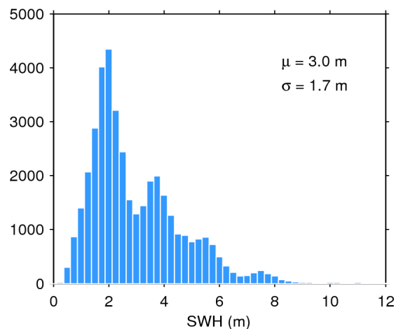
Figure 20. Histogram of science-valid SWH over oceans and lakes for 04/07/2017. The mean ( \mu ) and standard deviation ( \sigma ) are also shown. Note that values larger than 12 m are excluded from the histogram for the sake of readability but not from the computation of \mu and \sigma .
