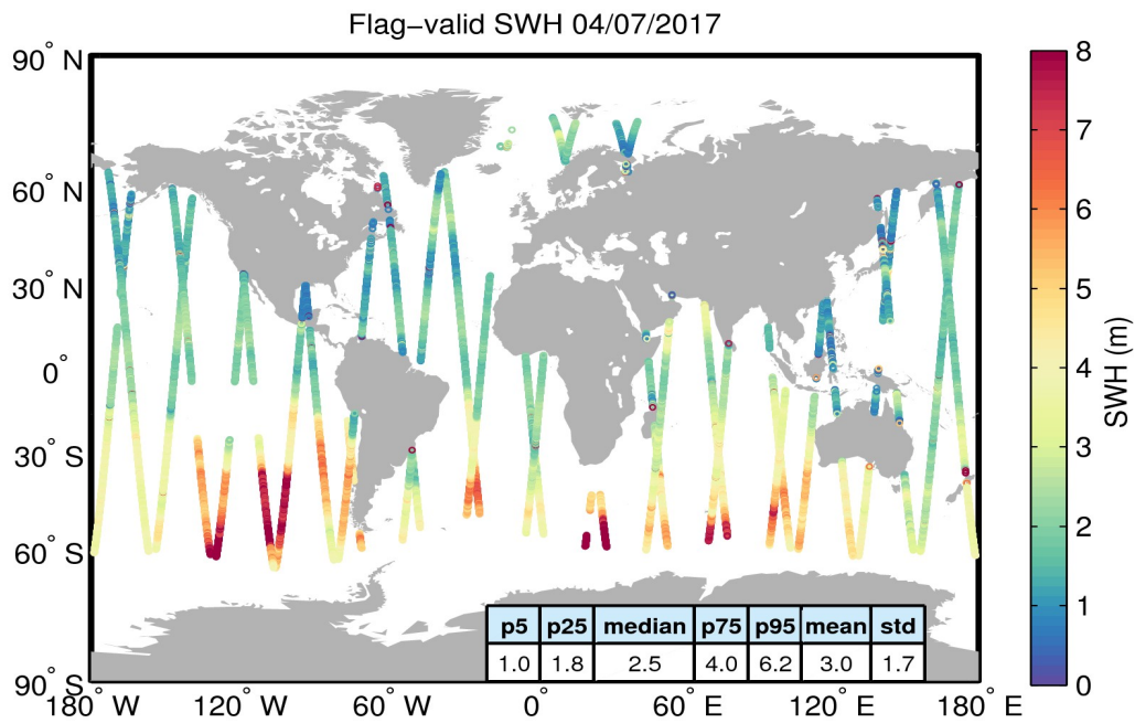
Figure 15. Geographical distribution of flag-valid SWH data over oceans and lakes for 04/07/2017. The statistical values shown in the table refer to the SWH in m and are calculated over all measurements shown in the figure.
