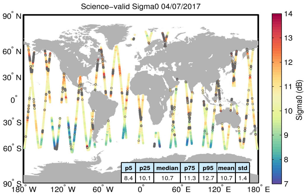
Figure 27. Geographical distribution of science-valid sigma0 data over oceans and lakes for 04/07/2017. The statistical values shown in the table refer to the sigma0 in dB and are calculated over all measurements shown in the figure. Gray circles denote records that have been rejected based on the editing criteria described in Table 4.
