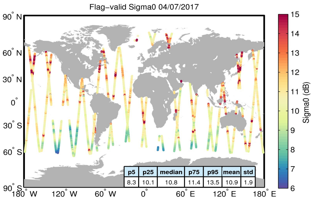
Figure 23. Geographical distribution of flag-valid sigma0 data over oceans and lakes for 04/07/2017. The statistical values shown in the table refer to the sigma0 in dB and are calculated over all measurements shown in the figure.
