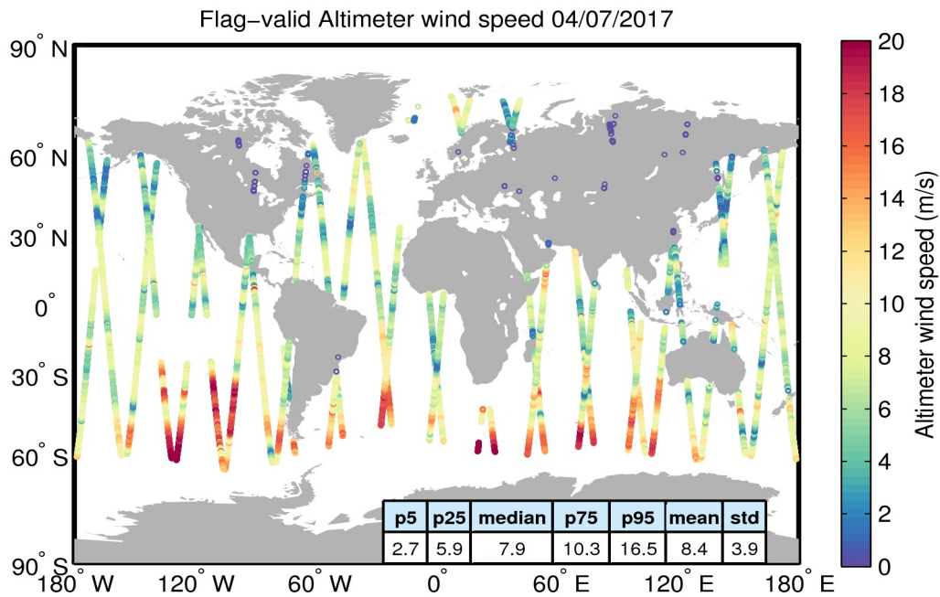
Figure 31. Geographical distribution of flag-valid wind data over oceans and lakes for 04/07/2017. The statistical values shown in the table refer to the wind in m/s and are calculated over all measurements shown in the figure.
