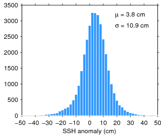
Figure 11. Histogram of science-valid SSH anomaly over oceans and lakes for 04/07/2017. The mean ( \mu ) and standard deviation ( \sigma ) are also shown. Note that values outside [-50 50] cm are excluded from the histogram for the sake of readability but not from the computation of \mu and \sigma .
