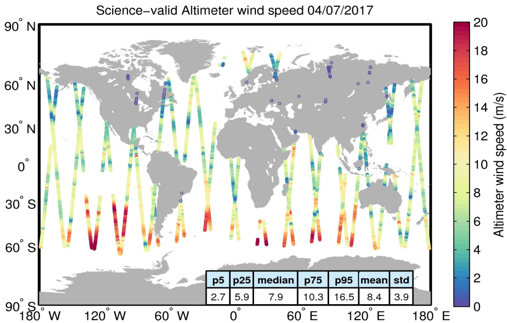
Figure 34. Geographical distribution of science-valid wind data over oceans and lakes for 04/07/2017. The statistical values shown in the table refer to the wind in m/s and are calculated over all measurements shown in the figure. Gray circles denote records that have been rejected based on the editing criteria described in Table 5.
