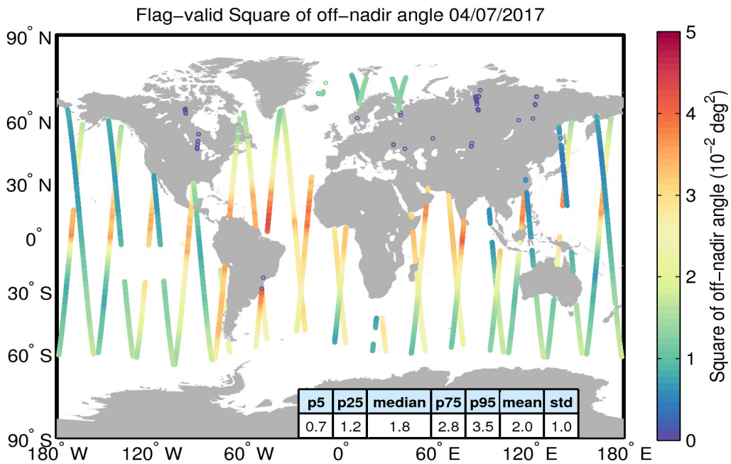
Figure 37. Geographical distribution of flag-valid mispointing data over oceans and lakes for 04/07/2017. The statistical values shown in the table refer to the mispointing in 10^{-2} deg 2 and are calculated over all measurements shown in the figure.
