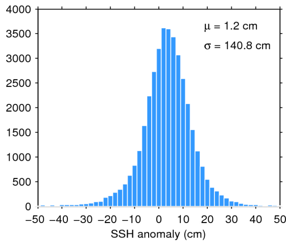
Figure 7. Histogram of flag-valid SSH anomaly over oceans and lakes for 04/07/2017. The mean ( \mu ) and standard deviation ( \sigma ) are also shown. Note that values outside [-50 50] cm are excluded from the histogram for the sake of readability but not from the computation of \mu and \sigma .
