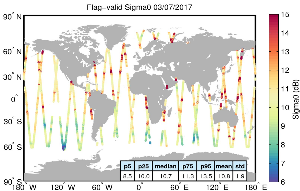
Figure 23. Geographical distribution of flag-valid sigma0 data over oceans and lakes for 03/07/2017. The statistical values shown in the table refer to the sigma0 in dB and are calculated over all measurements shown in the figure.
