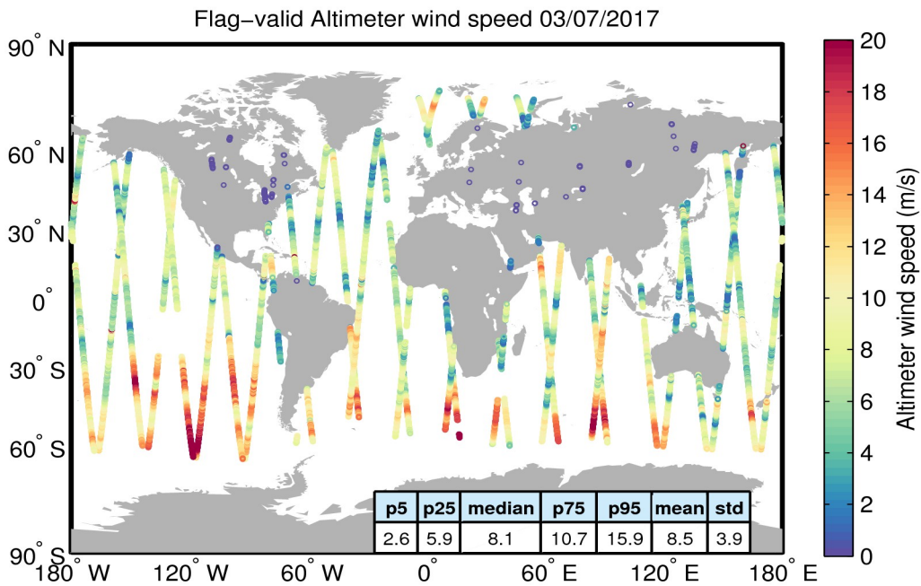
Figure 31. Geographical distribution of flag-valid wind data over oceans and lakes for 03/07/2017. The statistical values shown in the table refer to the wind in m/s and are calculated over all measurements shown in the figure.
