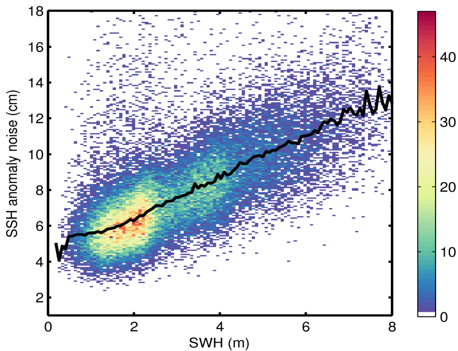
Figure 9. 2D histogram showing flag-valid SSH anomaly noise as a function of SWH for 03/07/2017. The black line denotes the median SSH anomaly noise as a function of SWH.
