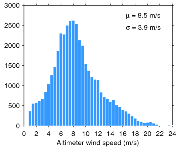
Figure 33. Histogram of flag-valid wind over oceans and lakes for 03/07/2017. The mean ( \mu ) and standard deviation ( \sigma ) are also shown. Note that values larger than 24 m/s are excluded from the histogram for the sake of readability but not from the computation of \mu and \sigma .
