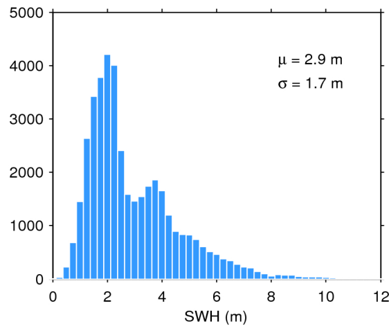
Figure 17. Histogram of flag-valid SWH over oceans and lakes for 03/07/2017. The mean ( \mu ) and standard deviation ( \sigma ) are also shown. Note that values larger than 12 m are excluded from the histogram for the sake of readability but not from the computation of \mu and \sigma .
