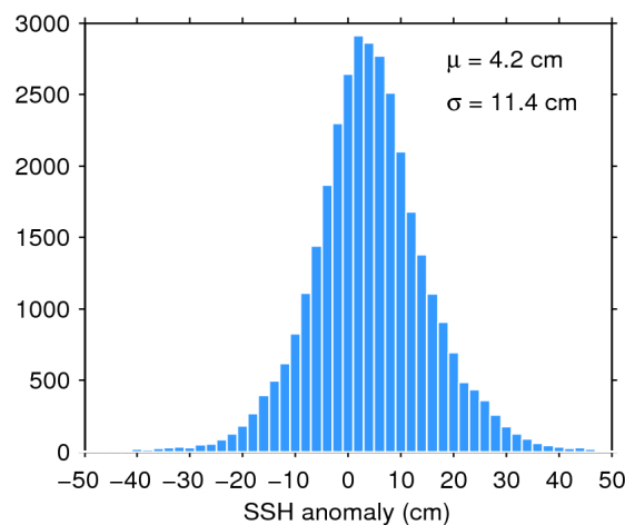
Figure 11. Histogram of science-valid SSH anomaly over oceans and lakes for 03/07/2017. The mean ( \mu ) and standard deviation ( \sigma ) are also shown. Note that values outside [-50 50] cm are excluded from the histogram for the sake of readability but not from the computation of \mu and \sigma .
