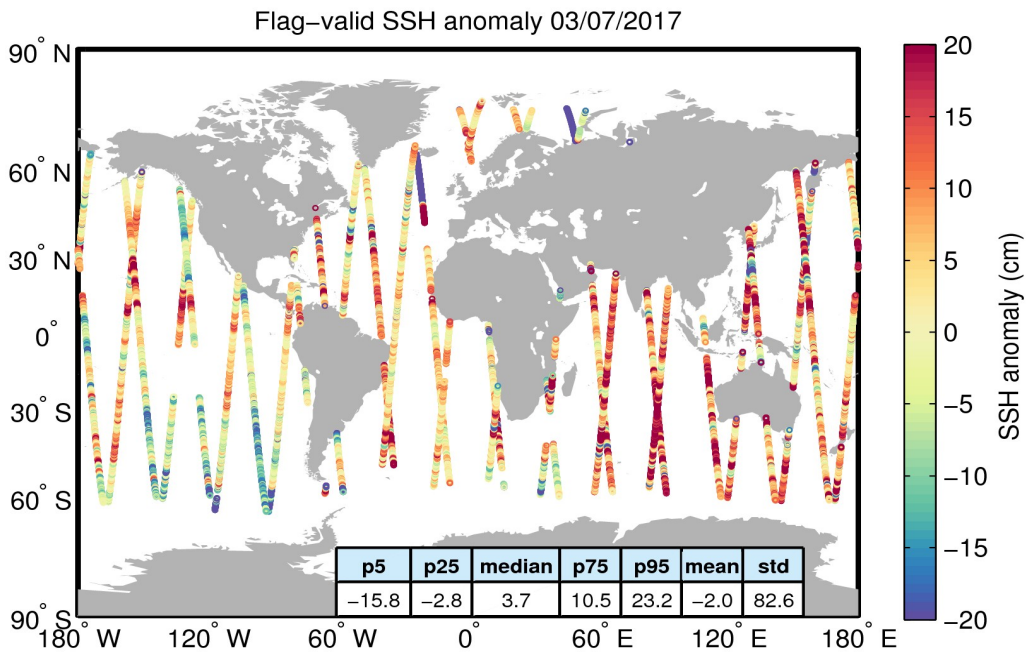
Figure 5. Geographical distribution of flag-valid 1-Hz SSH anomaly data over oceans and lakes for 03/07/2017. The statistical values shown in the table refer to the SSH anomaly in cm and are calculated over all measurements shown in the figure.
