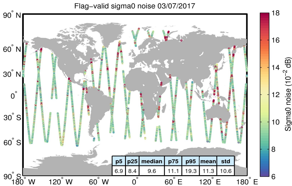
Figure 26. Geographical distribution of flag-valid 20-Hz sigma0 measurement noise over oceans and lakes for 03/07/2017. The statistical values shown in the table refer to the sigma0 noise and are calculated over all measurements shown in the figure.
