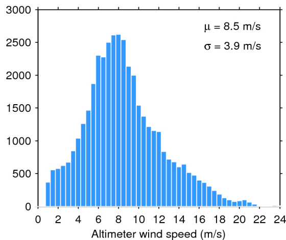
Figure 35. Histogram of science-valid wind over oceans and lakes for 03/07/2017. The mean ( \mu ) and standard deviation ( \sigma ) are also shown. Note that values larger than 24 m/s are excluded from the histogram for the sake of readability but not from the computation of \mu and \sigma .
