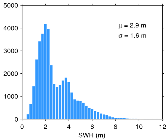
Figure 20. Histogram of science-valid SWH over oceans and lakes for 03/07/2017. The mean ( \mu ) and standard deviation ( \sigma ) are also shown. Note that values larger than 12 m are excluded from the histogram for the sake of readability but not from the computation of \mu and \sigma .
