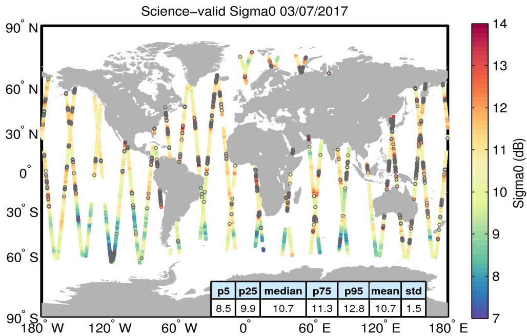
Figure 27. Geographical distribution of science-valid sigma0 data over oceans and lakes for 03/07/2017. The statistical values shown in the table refer to the sigma0 in dB and are calculated over all measurements shown in the figure. Gray circles denote records that have been rejected based on the editing criteria described in Table 4.
