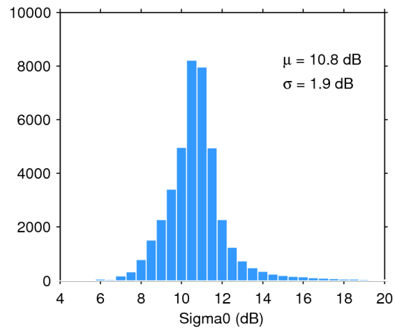
Figure 25. Histogram of flag-valid sigma0 over oceans and lakes for 03/07/2017. The mean ( \mu ) and standard deviation ( \sigma ) are also shown. Note that values outside [4 20] dB are excluded from the histogram for the sake of readability but not from the computation of \mu and \sigma .
