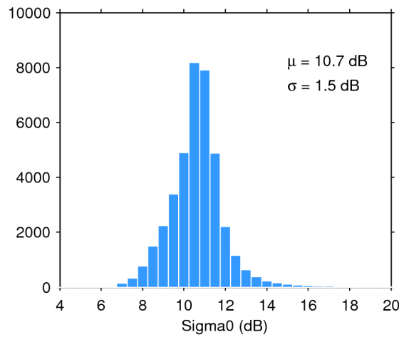
Figure 28. Histogram of science-valid sigma0 over oceans and lakes for 03/07/2017. The mean ( \mu ) and standard deviation ( \sigma ) are also shown. Note that values outside [4 20] dB are excluded from the histogram for the sake of readability but not from the computation of \mu and \sigma .
