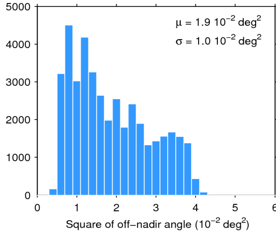
Figure 39. Histogram of flag-valid mispointing over oceans and lakes for 03/07/2017. The mean ( \mu ) and standard deviation ( \sigma ) are also shown. Note that values larger than 6 \cdot 10^{-2} \text{ deg}^2 are excluded from the histogram for the sake of readability but not from the computation of \mu and \sigma .
