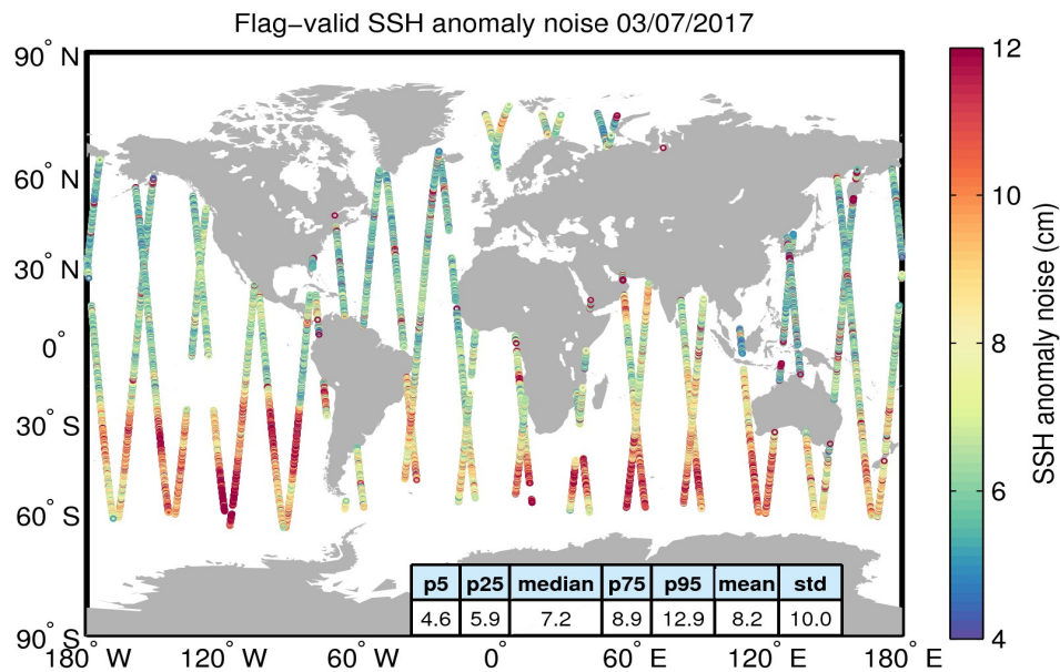
Figure 8. Geographical distribution of flag-valid 20-Hz SSH anomaly measurement noise over oceans and lakes for 03/07/2017. The statistical values shown in the table refer to the SSH anomaly noise and are calculated over all measurements shown in the figure.
