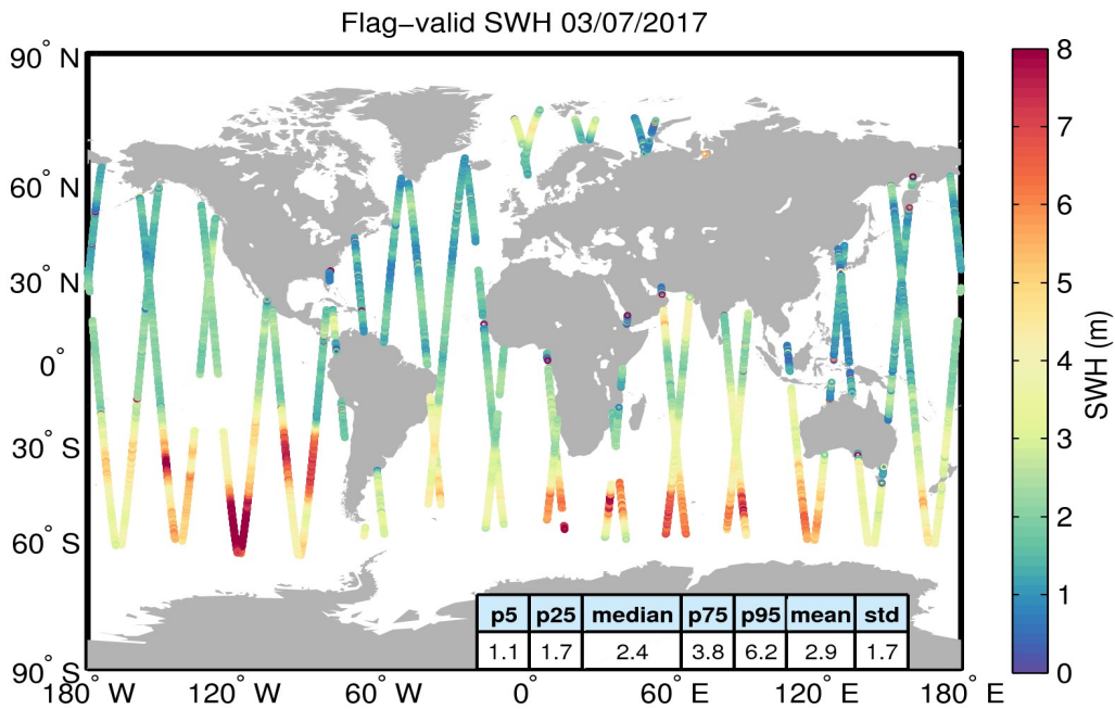
Figure 15. Geographical distribution of flag-valid SWH data over oceans and lakes for 03/07/2017. The statistical values shown in the table refer to the SWH in m and are calculated over all measurements shown in the figure.
