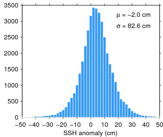
Figure 7. Histogram of flag-valid SSH anomaly over oceans and lakes for 03/07/2017. The mean ( \mu ) and standard deviation ( \sigma ) are also shown. Note that values outside [-50 50] cm are excluded from the histogram for the sake of readability but not from the computation of \mu and \sigma .
