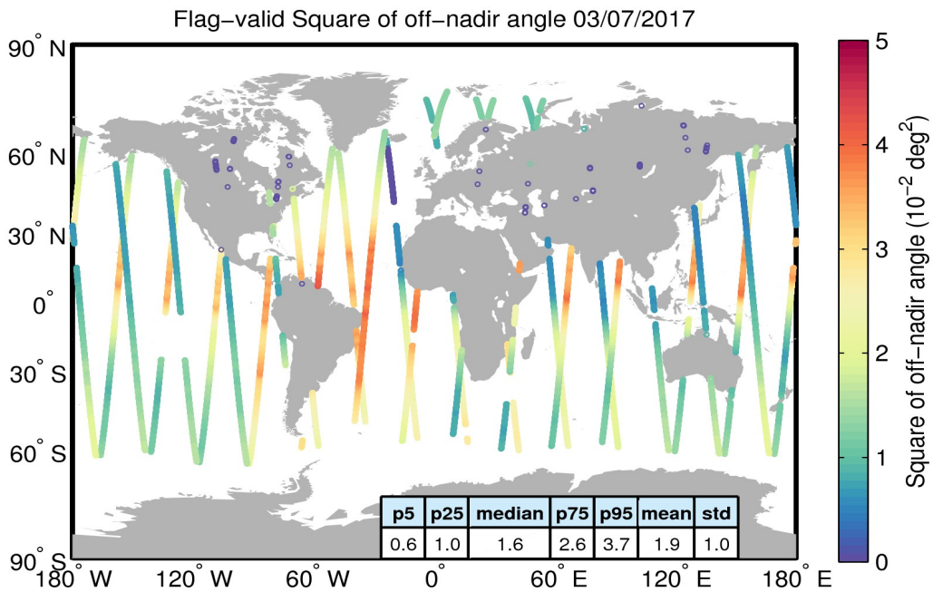
Figure 37. Geographical distribution of flag-valid mispointing data over oceans and lakes for 03/07/2017. The statistical values shown in the table refer to the mispointing in 10^{-2} deg 2 and are calculated over all measurements shown in the figure.
