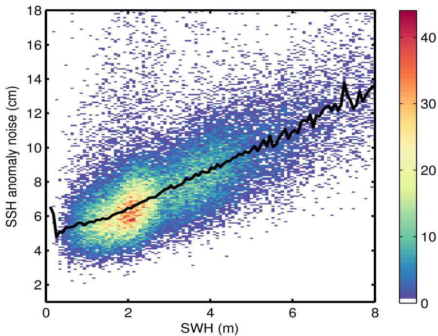
Figure 9. 2D histogram showing flag-valid SSH anomaly noise as a function of SWH for 02/07/2017. The black line denotes the median SSH anomaly noise as a function of SWH.
