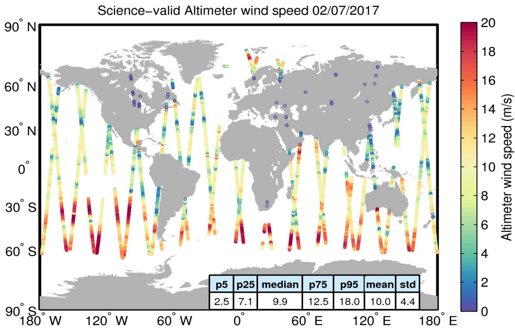
Figure 34. Geographical distribution of science-valid wind data over oceans and lakes for 02/07/2017. The statistical values shown in the table refer to the wind in m/s and are calculated over all measurements shown in the figure. Gray circles denote records that have been rejected based on the editing criteria described in Table 5.
