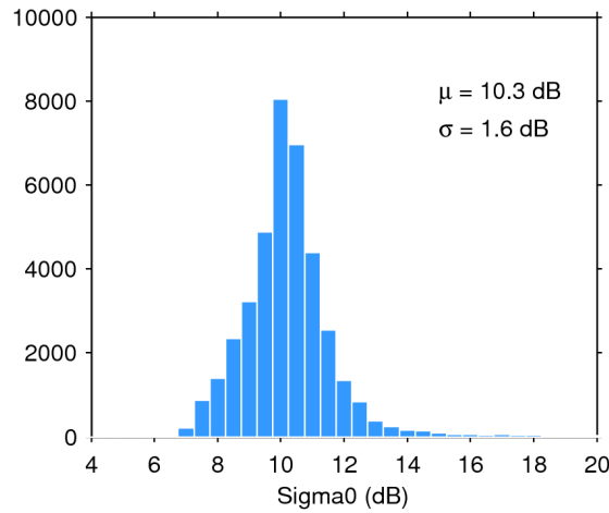
Figure 28. Histogram of science-valid sigma0 over oceans and lakes for 02/07/2017. The mean ( \mu ) and standard deviation ( \sigma ) are also shown. Note that values outside [4 20] dB are excluded from the histogram for the sake of readability but not from the computation of \mu and \sigma .
