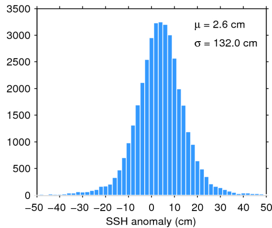
Figure 7. Histogram of flag-valid SSH anomaly over oceans and lakes for 02/07/2017. The mean ( \mu ) and standard deviation ( \sigma ) are also shown. Note that values outside [-50 50] cm are excluded from the histogram for the sake of readability but not from the computation of \mu and \sigma .
