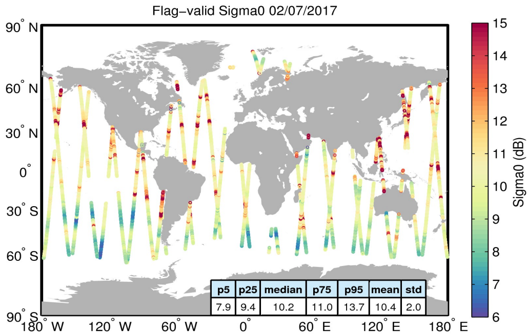
Figure 23. Geographical distribution of flag-valid sigma0 data over oceans and lakes for 02/07/2017. The statistical values shown in the table refer to the sigma0 in dB and are calculated over all measurements shown in the figure.
