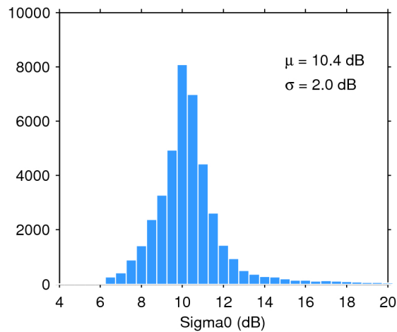
Figure 25. Histogram of flag-valid sigma0 over oceans and lakes for 02/07/2017. The mean ( \mu ) and standard deviation ( \sigma ) are also shown. Note that values outside [4 20] dB are excluded from the histogram for the sake of readability but not from the computation of \mu and \sigma .
