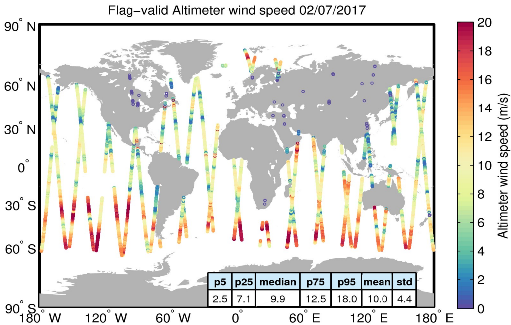
Figure 31. Geographical distribution of flag-valid wind data over oceans and lakes for 02/07/2017. The statistical values shown in the table refer to the wind in m/s and are calculated over all measurements shown in the figure.
