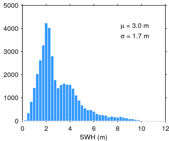
Figure 20. Histogram of science-valid SWH over oceans and lakes for 02/07/2017. The mean ( \mu ) and standard deviation ( \sigma ) are also shown. Note that values larger than 12 m are excluded from the histogram for the sake of readability but not from the computation of \mu and \sigma .
