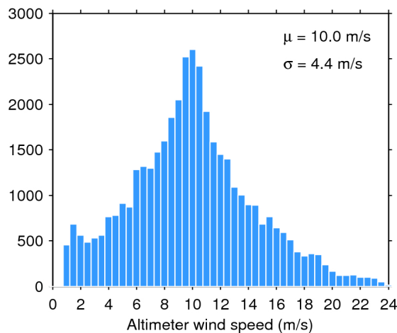
Figure 35. Histogram of science-valid wind over oceans and lakes for 02/07/2017. The mean ( \mu ) and standard deviation ( \sigma ) are also shown. Note that values larger than 24 m/s are excluded from the histogram for the sake of readability but not from the computation of \mu and \sigma .
