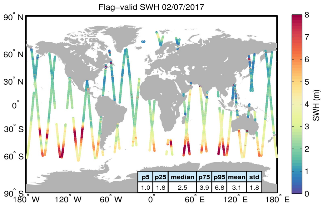
Figure 15. Geographical distribution of flag-valid SWH data over oceans and lakes for 02/07/2017. The statistical values shown in the table refer to the SWH in m and are calculated over all measurements shown in the figure.
