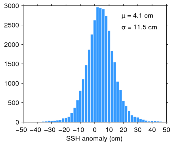
Figure 11. Histogram of science-valid SSH anomaly over oceans and lakes for 02/07/2017. The mean ( \mu ) and standard deviation ( \sigma ) are also shown. Note that values outside [-50 50] cm are excluded from the histogram for the sake of readability but not from the computation of \mu and \sigma .
