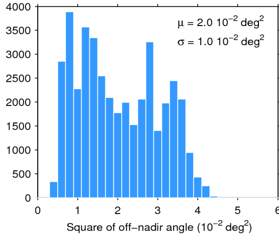
Figure 39. Histogram of flag-valid mispointing over oceans and lakes for 02/07/2017. The mean ( \mu ) and standard deviation ( \sigma ) are also shown. Note that values larger than 6 \cdot 10^{-2} \text{ deg}^2 are excluded from the histogram for the sake of readability but not from the computation of \mu and \sigma .
