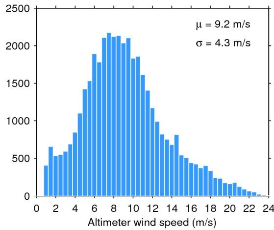
Figure 33. Histogram of flag-valid wind over oceans and lakes for 01/07/2017. The mean ( \mu ) and standard deviation ( \sigma ) are also shown. Note that values larger than 24 m/s are excluded from the histogram for the sake of readability but not from the computation of \mu and \sigma .
