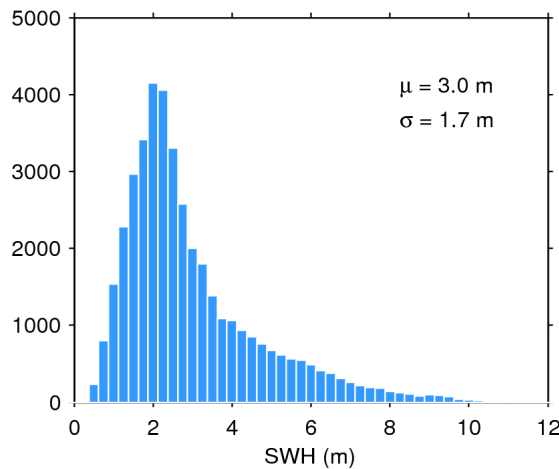
Figure 17. Histogram of flag-valid SWH over oceans and lakes for 01/07/2017. The mean ( \mu ) and standard deviation ( \sigma ) are also shown. Note that values larger than 12 m are excluded from the histogram for the sake of readability but not from the computation of \mu and \sigma .
