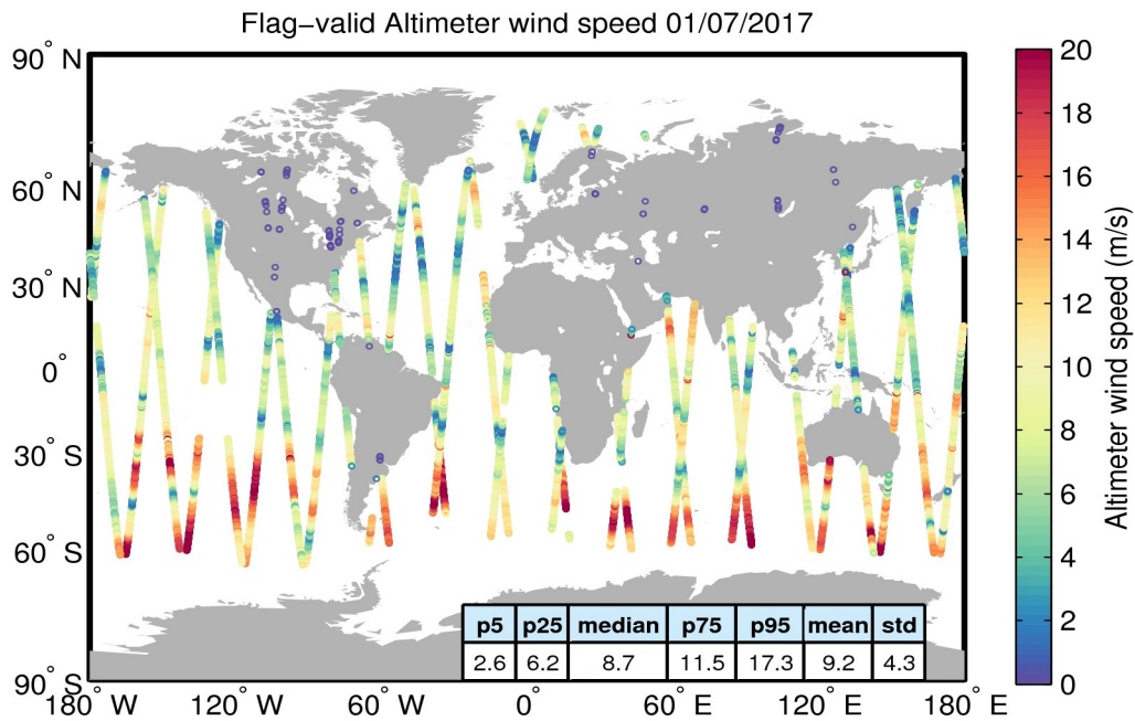
Figure 31. Geographical distribution of flag-valid wind data over oceans and lakes for 01/07/2017. The statistical values shown in the table refer to the wind in m/s and are calculated over all measurements shown in the figure.
