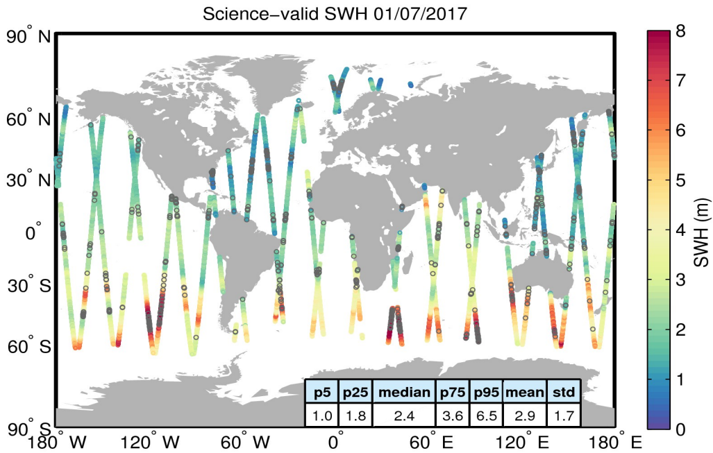
Figure 19. Geographical distribution of science-valid SWH data over oceans and lakes for 01/07/2017. The statistical values shown in the table refer to the SWH in m and are calculated over all measurements shown in the figure. Gray circles denote records that have been rejected based on the editing criteria described in Table 3.
