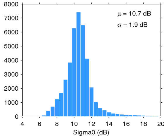
Figure 25. Histogram of flag-valid sigma0 over oceans and lakes for 01/07/2017. The mean ( \mu ) and standard deviation ( \sigma ) are also shown. Note that values outside [4 20] dB are excluded from the histogram for the sake of readability but not from the computation of \mu and \sigma .
