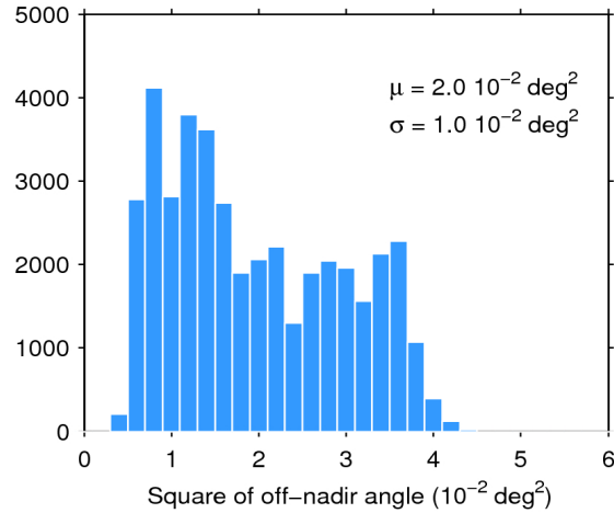
Figure 39. Histogram of flag-valid mispointing over oceans and lakes for 01/07/2017. The mean ( \mu ) and standard deviation ( \sigma ) are also shown. Note that values larger than 6 \cdot 10^{-2} \text{ deg}^2 are excluded from the histogram for the sake of readability but not from the computation of \mu and \sigma .
