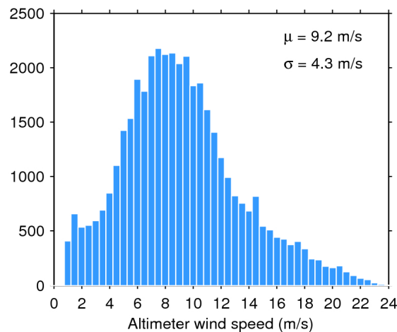
Figure 35. Histogram of science-valid wind over oceans and lakes for 01/07/2017. The mean ( \mu ) and standard deviation ( \sigma ) are also shown. Note that values larger than 24 m/s are excluded from the histogram for the sake of readability but not from the computation of \mu and \sigma .
