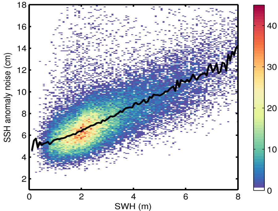
Figure 9. 2D histogram showing flag-valid SSH anomaly noise as a function of SWH for 01/07/2017. The black line denotes the median SSH anomaly noise as a function of SWH.
