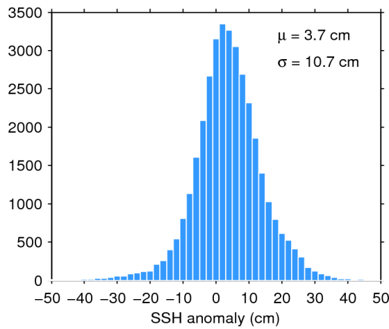
Figure 11. Histogram of science-valid SSH anomaly over oceans and lakes for 01/07/2017. The mean ( \mu ) and standard deviation ( \sigma ) are also shown. Note that values outside [-50 50] cm are excluded from the histogram for the sake of readability but not from the computation of \mu and \sigma .
