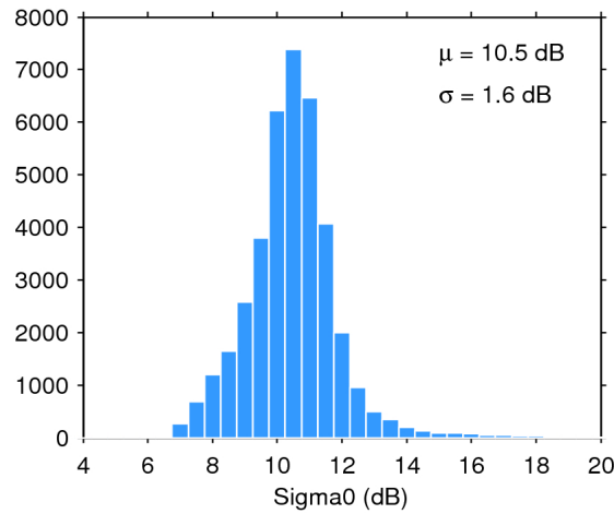
Figure 28. Histogram of science-valid sigma0 over oceans and lakes for 01/07/2017. The mean ( \mu ) and standard deviation ( \sigma ) are also shown. Note that values outside [4 20] dB are excluded from the histogram for the sake of readability but not from the computation of \mu and \sigma .
