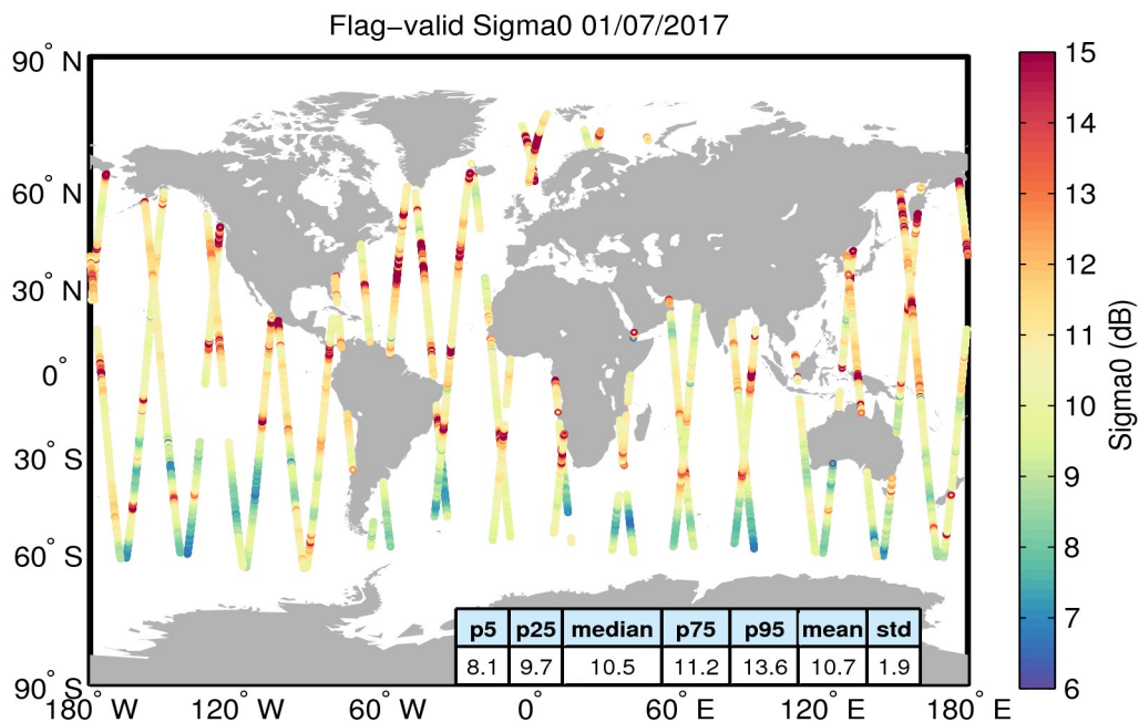
Figure 23. Geographical distribution of flag-valid sigma0 data over oceans and lakes for 01/07/2017. The statistical values shown in the table refer to the sigma0 in dB and are calculated over all measurements shown in the figure.
