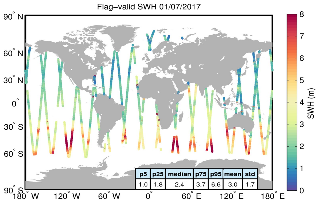
Figure 15. Geographical distribution of flag-valid SWH data over oceans and lakes for 01/07/2017. The statistical values shown in the table refer to the SWH in m and are calculated over all measurements shown in the figure.
