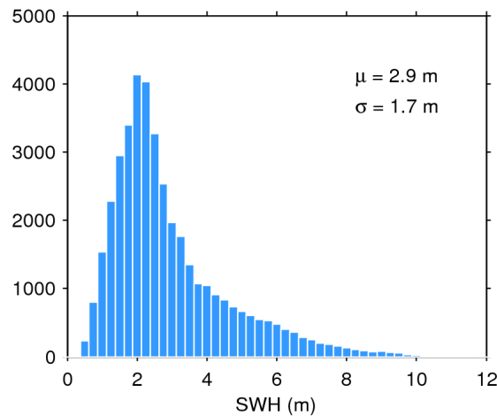
Figure 20. Histogram of science-valid SWH over oceans and lakes for 01/07/2017. The mean ( \mu ) and standard deviation ( \sigma ) are also shown. Note that values larger than 12 m are excluded from the histogram for the sake of readability but not from the computation of \mu and \sigma .
