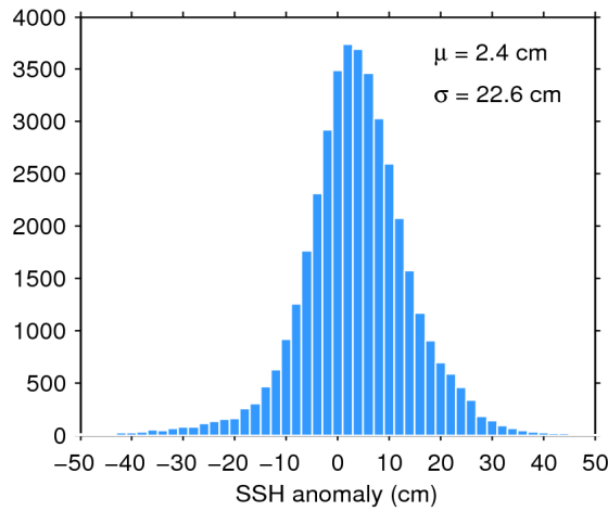
Figure 7. Histogram of flag-valid SSH anomaly over oceans and lakes for 01/07/2017. The mean ( \mu ) and standard deviation ( \sigma ) are also shown. Note that values outside [-50 50] cm are excluded from the histogram for the sake of readability but not from the computation of \mu and \sigma .
