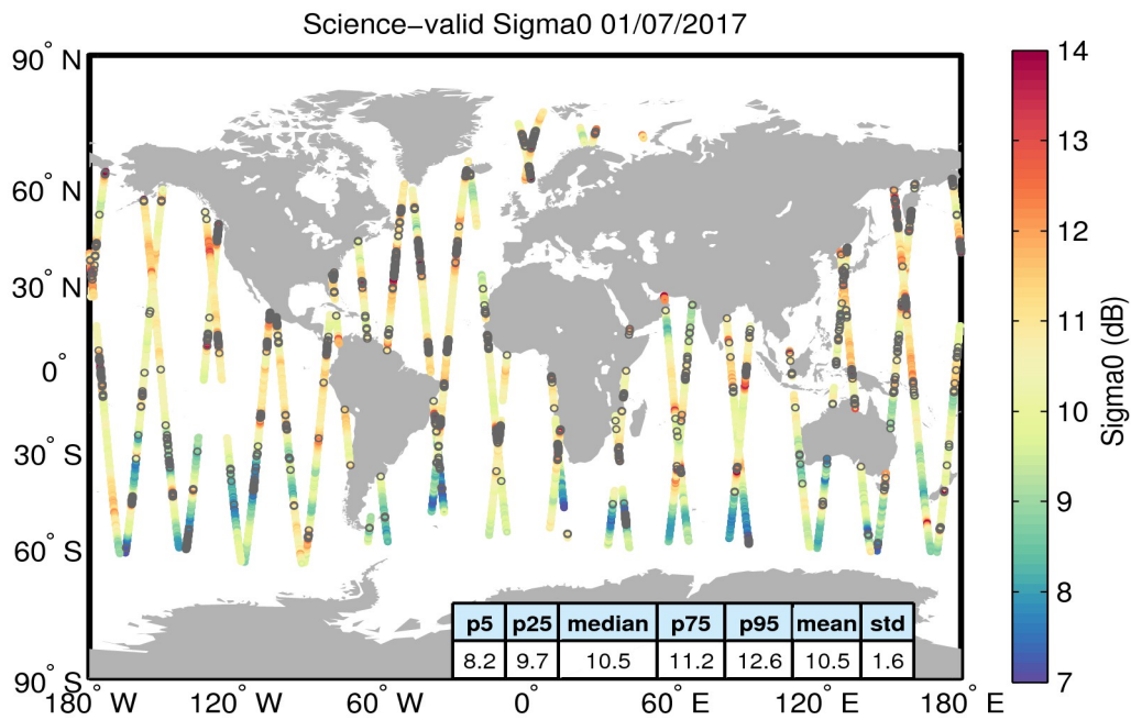
Figure 27. Geographical distribution of science-valid sigma0 data over oceans and lakes for 01/07/2017. The statistical values shown in the table refer to the sigma0 in dB and are calculated over all measurements shown in the figure. Gray circles denote records that have been rejected based on the editing criteria described in Table 4.
