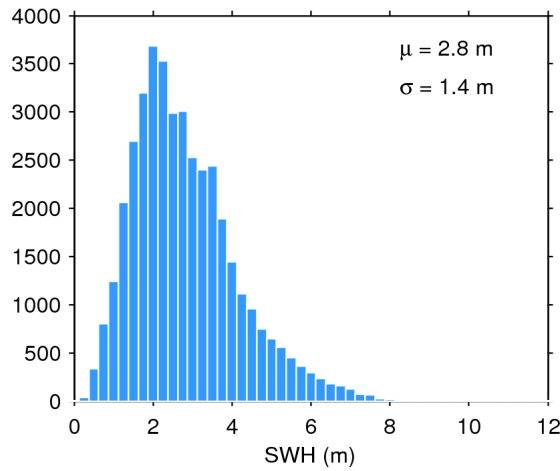
Figure 17. Histogram of flag-valid SWH over oceans and lakes for 28/06/2017. The mean ( \mu ) and standard deviation ( \sigma ) are also shown. Note that values larger than 12 m are excluded from the histogram for the sake of readability but not from the computation of \mu and \sigma .
