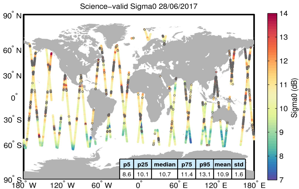
Figure 27. Geographical distribution of science-valid sigma0 data over oceans and lakes for 28/06/2017. The statistical values shown in the table refer to the sigma0 in dB and are calculated over all measurements shown in the figure. Gray circles denote records that have been rejected based on the editing criteria described in Table 4.
