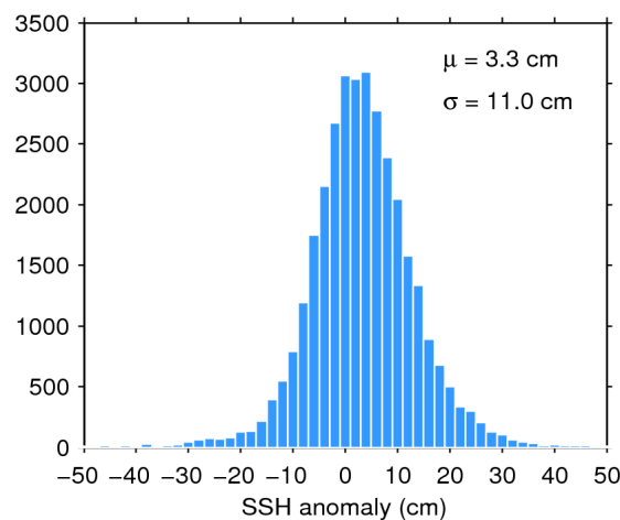
Figure 11. Histogram of science-valid SSH anomaly over oceans and lakes for 28/06/2017. The mean ( \mu ) and standard deviation ( \sigma ) are also shown. Note that values outside [-50 50] cm are excluded from the histogram for the sake of readability but not from the computation of \mu and \sigma .
