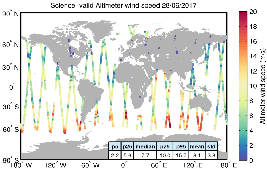
Figure 34. Geographical distribution of science-valid wind data over oceans and lakes for 28/06/2017. The statistical values shown in the table refer to the wind in m/s and are calculated over all measurements shown in the figure. Gray circles denote records that have been rejected based on the editing criteria described in Table 5.
