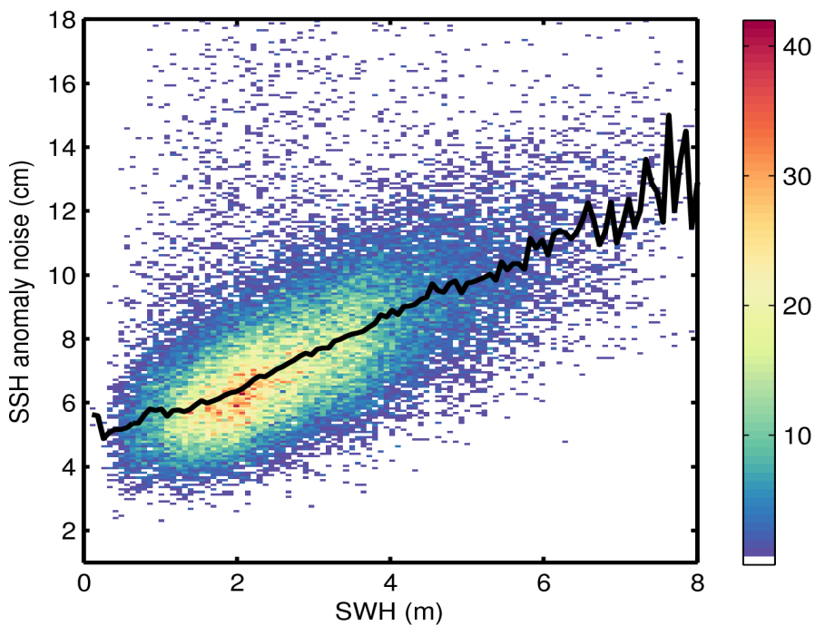
Figure 9. 2D histogram showing flag-valid SSH anomaly noise as a function of SWH for 28/06/2017. The black line denotes the median SSH anomaly noise as a function of SWH.
