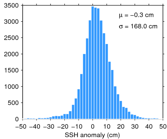
Figure 7. Histogram of flag-valid SSH anomaly over oceans and lakes for 28/06/2017. The mean ( \mu ) and standard deviation ( \sigma ) are also shown. Note that values outside [-50 50] cm are excluded from the histogram for the sake of readability but not from the computation of \mu and \sigma .
