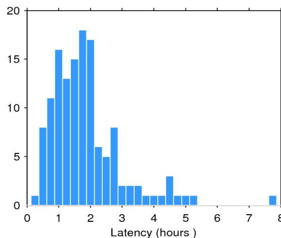
Figure 2. Histogram of the data latency for 28/06/2017. The y-axis denotes the number of files that are made available with a delay of x-hours with respect to the mean time of the records stored in the file.
