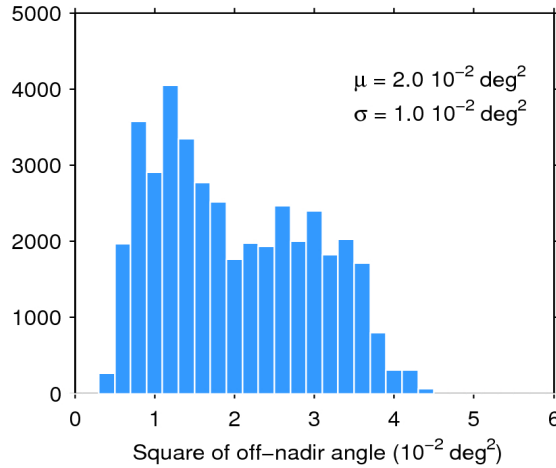
Figure 39. Histogram of flag-valid mispointing over oceans and lakes for 28/06/2017. The mean ( \mu ) and standard deviation ( \sigma ) are also shown. Note that values larger than 6 \cdot 10^{-2} \text{ deg}^2 are excluded from the histogram for the sake of readability but not from the computation of \mu and \sigma .
