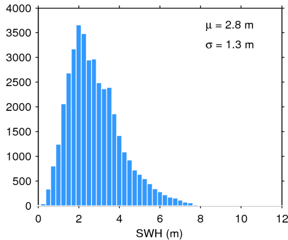
Figure 20. Histogram of science-valid SWH over oceans and lakes for 28/06/2017. The mean ( \mu ) and standard deviation ( \sigma ) are also shown. Note that values larger than 12 m are excluded from the histogram for the sake of readability but not from the computation of \mu and \sigma .
