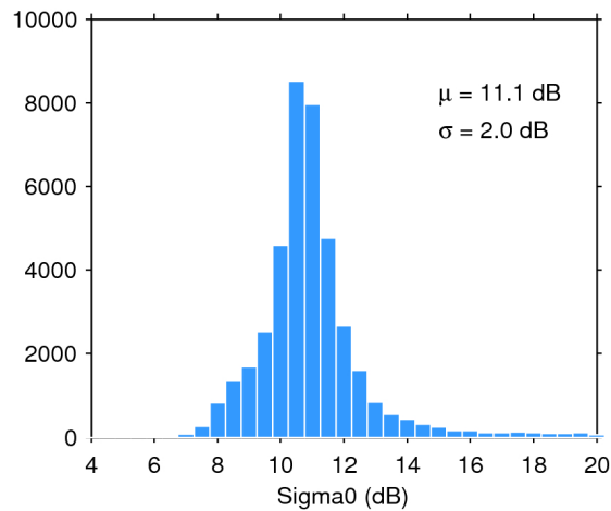
Figure 25. Histogram of flag-valid sigma0 over oceans and lakes for 28/06/2017. The mean ( \mu ) and standard deviation ( \sigma ) are also shown. Note that values outside [4 20] dB are excluded from the histogram for the sake of readability but not from the computation of \mu and \sigma .
