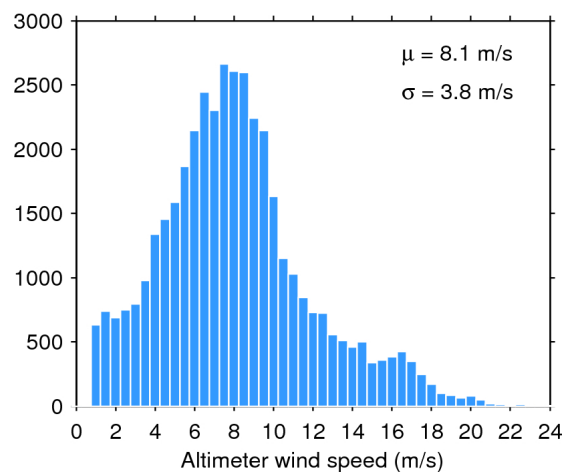
Figure 35. Histogram of science-valid wind over oceans and lakes for 28/06/2017. The mean ( \mu ) and standard deviation ( \sigma ) are also shown. Note that values larger than 24 m/s are excluded from the histogram for the sake of readability but not from the computation of \mu and \sigma .
