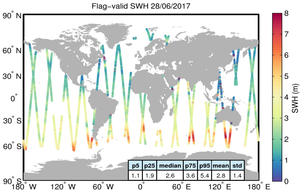
Figure 15. Geographical distribution of flag-valid SWH data over oceans and lakes for 28/06/2017. The statistical values shown in the table refer to the SWH in m and are calculated over all measurements shown in the figure.
