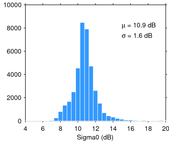
Figure 28. Histogram of science-valid sigma0 over oceans and lakes for 28/06/2017. The mean ( \mu ) and standard deviation ( \sigma ) are also shown. Note that values outside [4 20] dB are excluded from the histogram for the sake of readability but not from the computation of \mu and \sigma .
