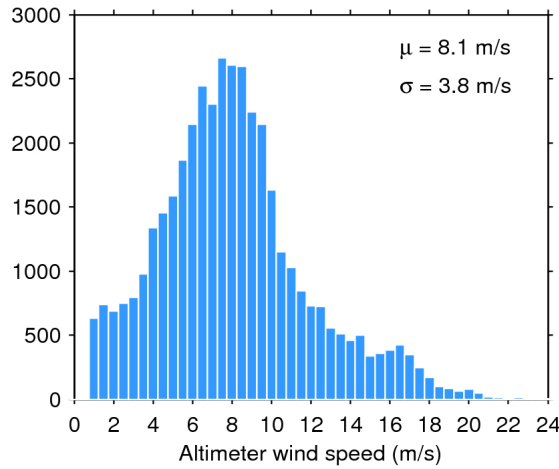
Figure 33. Histogram of flag-valid wind over oceans and lakes for 28/06/2017. The mean ( \mu ) and standard deviation ( \sigma ) are also shown. Note that values larger than 24 m/s are excluded from the histogram for the sake of readability but not from the computation of \mu and \sigma .
