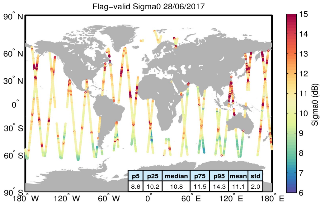
Figure 23. Geographical distribution of flag-valid sigma0 data over oceans and lakes for 28/06/2017. The statistical values shown in the table refer to the sigma0 in dB and are calculated over all measurements shown in the figure.
