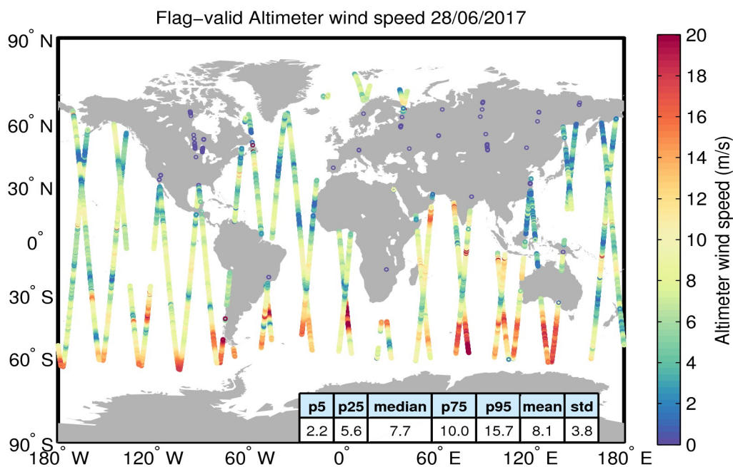
Figure 31. Geographical distribution of flag-valid wind data over oceans and lakes for 28/06/2017. The statistical values shown in the table refer to the wind in m/s and are calculated over all measurements shown in the figure.
