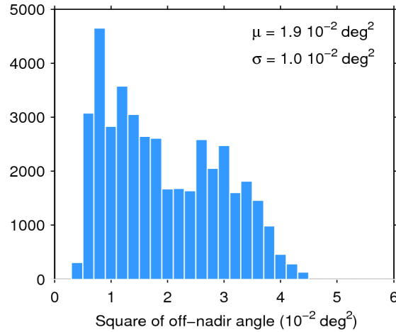
Figure 39. Histogram of flag-valid mispointing over oceans and lakes for 27/06/2017. The mean ( \mu ) and standard deviation ( \sigma ) are also shown. Note that values larger than 6 \cdot 10^{-2} \text{ deg}^2 are excluded from the histogram for the sake of readability but not from the computation of \mu and \sigma .
