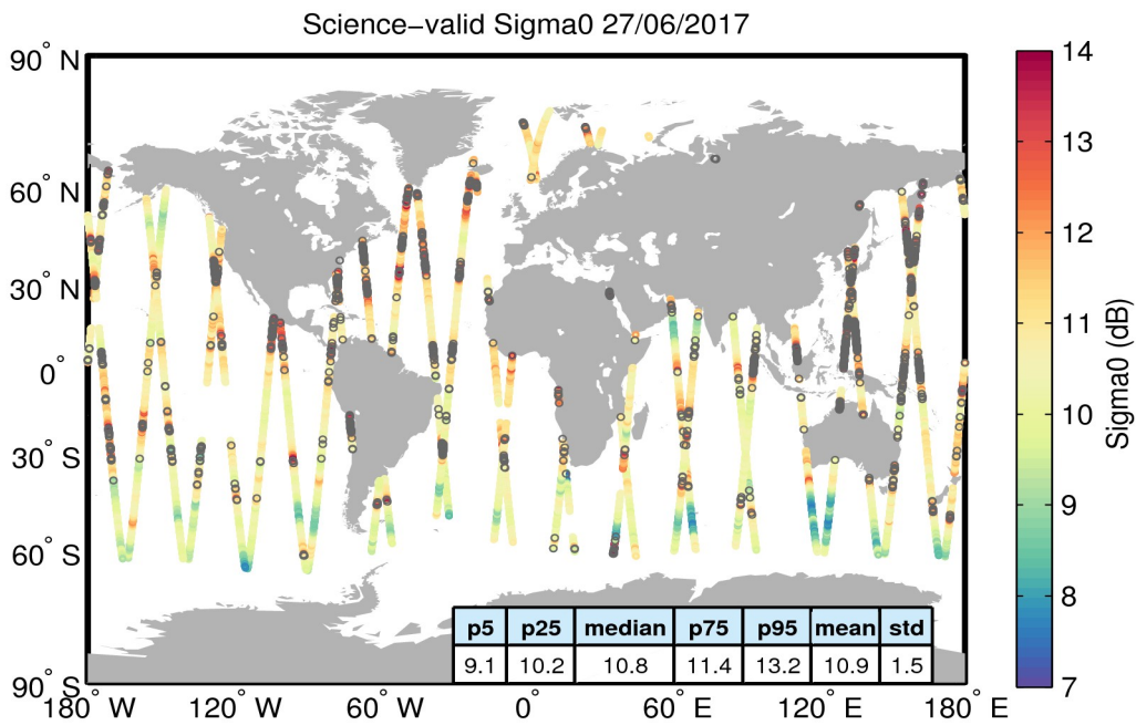
Figure 27. Geographical distribution of science-valid sigma0 data over oceans and lakes for 27/06/2017. The statistical values shown in the table refer to the sigma0 in dB and are calculated over all measurements shown in the figure. Gray circles denote records that have been rejected based on the editing criteria described in Table 4.
