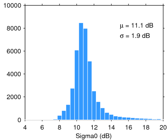
Figure 25. Histogram of flag-valid sigma0 over oceans and lakes for 27/06/2017. The mean ( \mu ) and standard deviation ( \sigma ) are also shown. Note that values outside [4 20] dB are excluded from the histogram for the sake of readability but not from the computation of \mu and \sigma .
