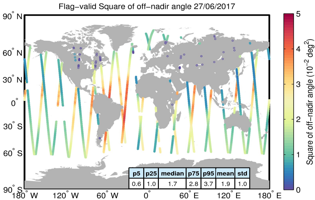
Figure 37. Geographical distribution of flag-valid mispointing data over oceans and lakes for 27/06/2017. The statistical values shown in the table refer to the mispointing in 10^{-2} deg 2 and are calculated over all measurements shown in the figure.
