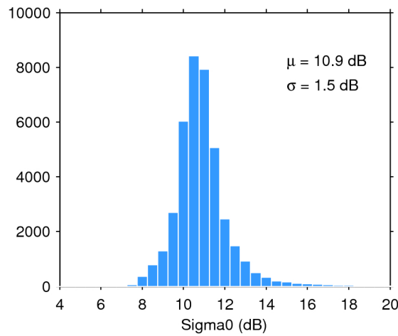
Figure 28. Histogram of science-valid sigma0 over oceans and lakes for 27/06/2017. The mean ( \mu ) and standard deviation ( \sigma ) are also shown. Note that values outside [4 20] dB are excluded from the histogram for the sake of readability but not from the computation of \mu and \sigma .
