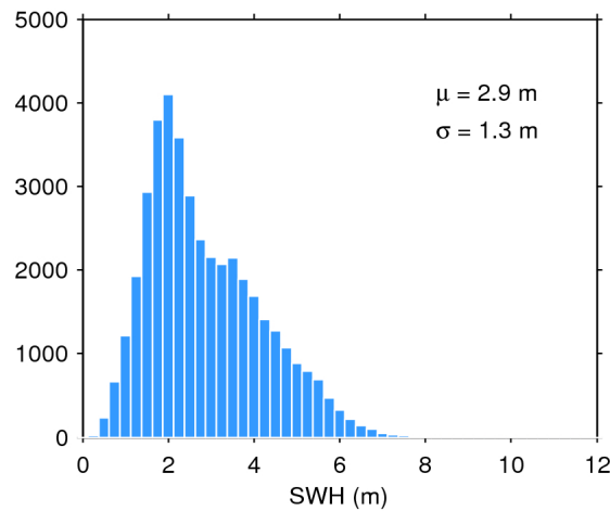
Figure 17. Histogram of flag-valid SWH over oceans and lakes for 27/06/2017. The mean ( \mu ) and standard deviation ( \sigma ) are also shown. Note that values larger than 12 m are excluded from the histogram for the sake of readability but not from the computation of \mu and \sigma .
