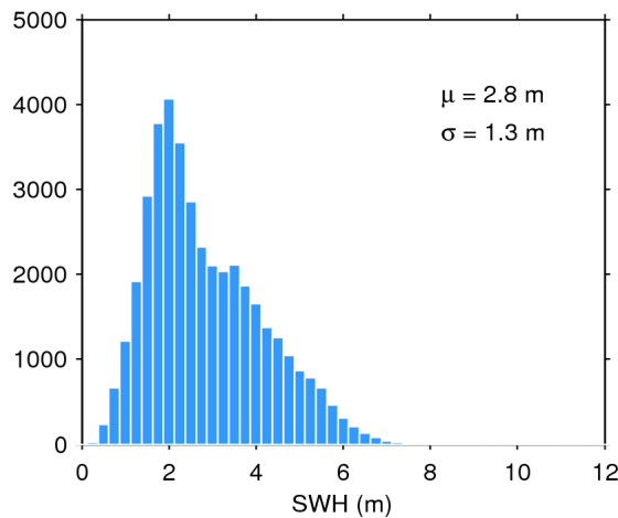
Figure 20. Histogram of science-valid SWH over oceans and lakes for 27/06/2017. The mean ( \mu ) and standard deviation ( \sigma ) are also shown. Note that values larger than 12 m are excluded from the histogram for the sake of readability but not from the computation of \mu and \sigma .
