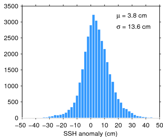
Figure 11. Histogram of science-valid SSH anomaly over oceans and lakes for 27/06/2017. The mean ( \mu ) and standard deviation ( \sigma ) are also shown. Note that values outside [-50 50] cm are excluded from the histogram for the sake of readability but not from the computation of \mu and \sigma .
