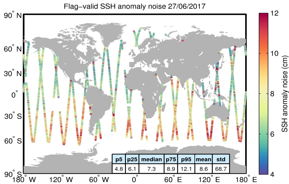
Figure 8. Geographical distribution of flag-valid 20-Hz SSH anomaly measurement noise over oceans and lakes for 27/06/2017. The statistical values shown in the table refer to the SSH anomaly noise and are calculated over all measurements shown in the figure.
