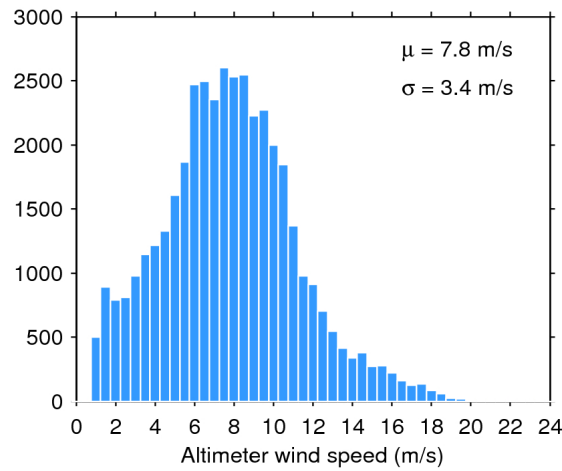
Figure 33. Histogram of flag-valid wind over oceans and lakes for 27/06/2017. The mean ( \mu ) and standard deviation ( \sigma ) are also shown. Note that values larger than 24 m/s are excluded from the histogram for the sake of readability but not from the computation of \mu and \sigma .
