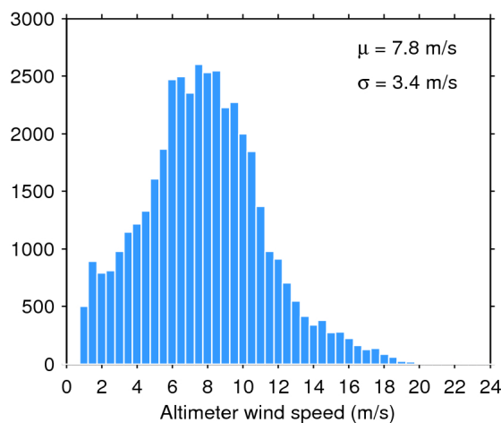
Figure 35. Histogram of science-valid wind over oceans and lakes for 27/06/2017. The mean ( \mu ) and standard deviation ( \sigma ) are also shown. Note that values larger than 24 m/s are excluded from the histogram for the sake of readability but not from the computation of \mu and \sigma .
