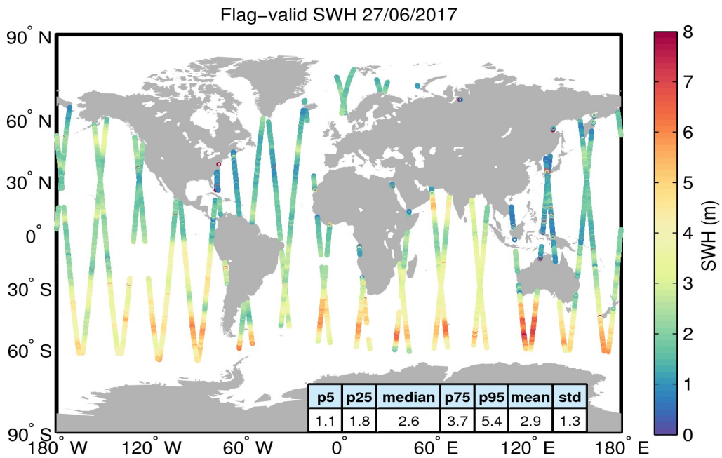
Figure 15. Geographical distribution of flag-valid SWH data over oceans and lakes for 27/06/2017. The statistical values shown in the table refer to the SWH in m and are calculated over all measurements shown in the figure.
