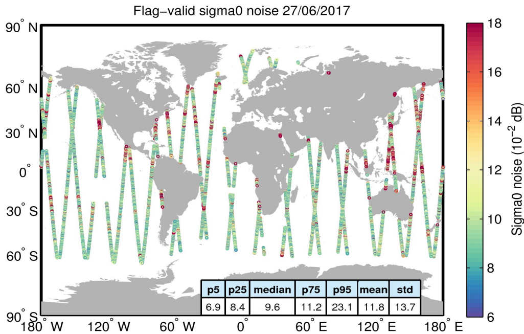
Figure 26. Geographical distribution of flag-valid 20-Hz sigma0 measurement noise over oceans and lakes for 27/06/2017. The statistical values shown in the table refer to the sigma0 noise and are calculated over all measurements shown in the figure.
