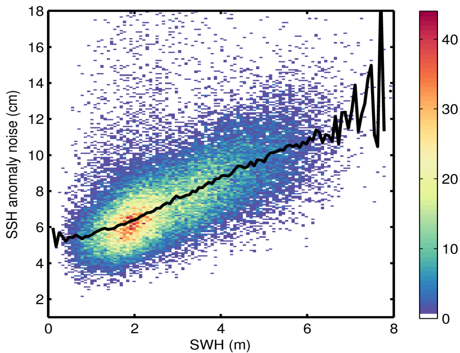
Figure 9. 2D histogram showing flag-valid SSH anomaly noise as a function of SWH for 27/06/2017. The black line denotes the median SSH anomaly noise as a function of SWH.
