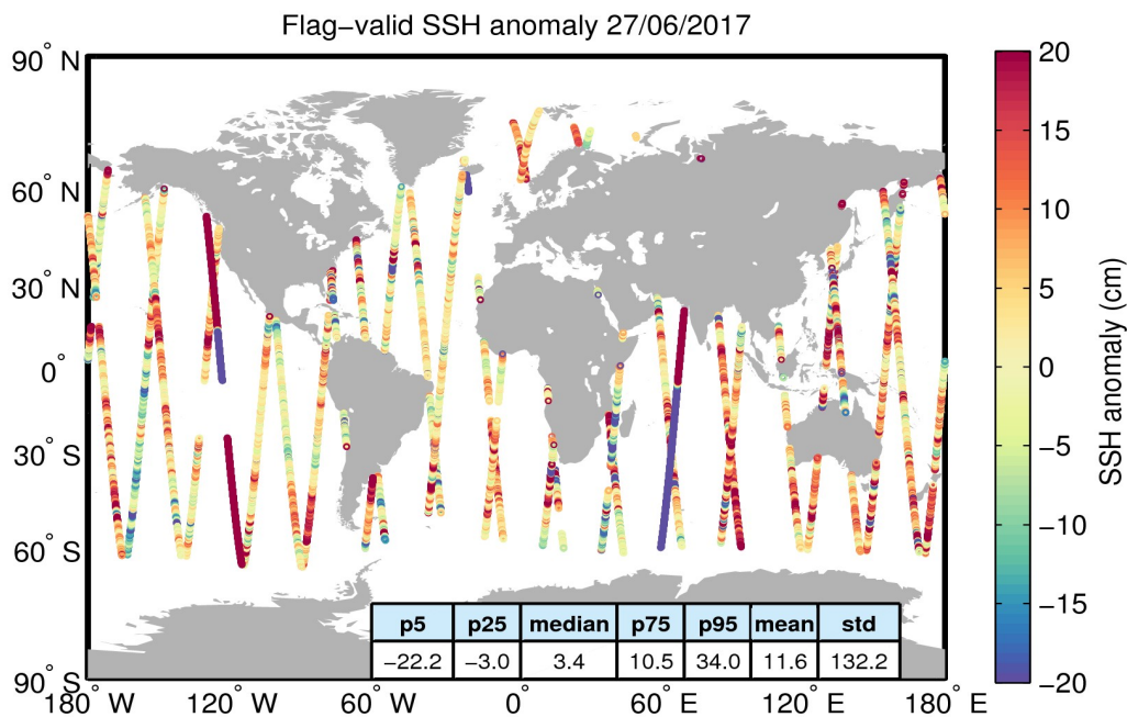
Figure 5. Geographical distribution of flag-valid 1-Hz SSH anomaly data over oceans and lakes for 27/06/2017. The statistical values shown in the table refer to the SSH anomaly in cm and are calculated over all measurements shown in the figure.
