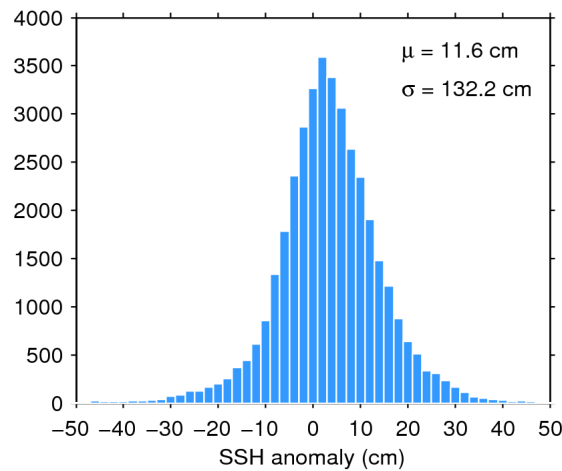
Figure 7. Histogram of flag-valid SSH anomaly over oceans and lakes for 27/06/2017. The mean ( \mu ) and standard deviation ( \sigma ) are also shown. Note that values outside [-50 50] cm are excluded from the histogram for the sake of readability but not from the computation of \mu and \sigma .
