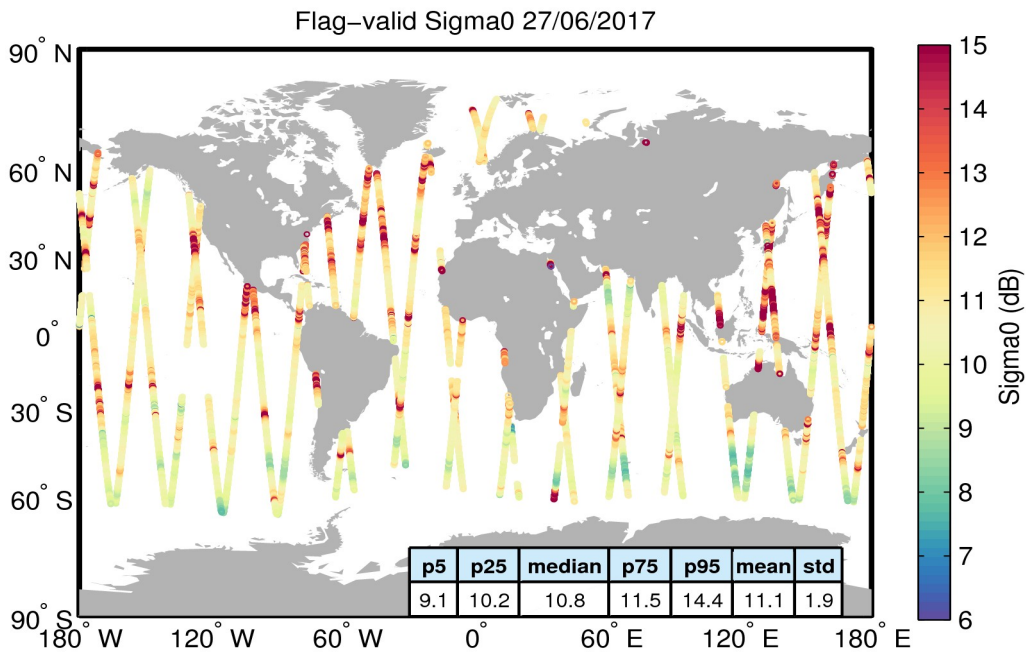
Figure 23. Geographical distribution of flag-valid sigma0 data over oceans and lakes for 27/06/2017. The statistical values shown in the table refer to the sigma0 in dB and are calculated over all measurements shown in the figure.
