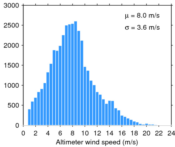
Figure 33. Histogram of flag-valid wind over oceans and lakes for 26/06/2017. The mean ( \mu ) and standard deviation ( \sigma ) are also shown. Note that values larger than 24 m/s are excluded from the histogram for the sake of readability but not from the computation of \mu and \sigma .
