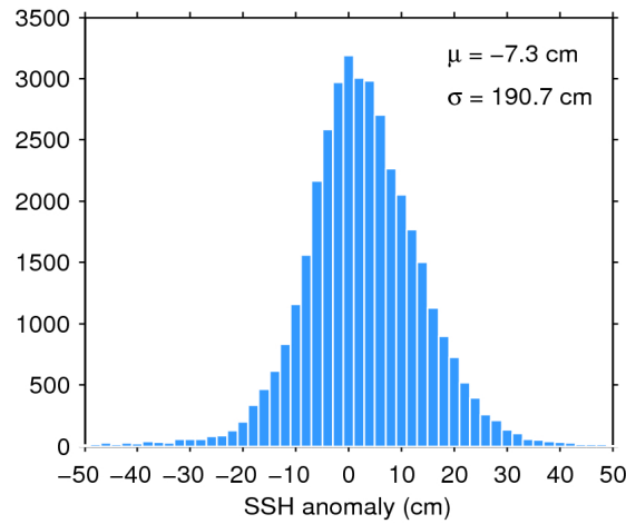
Figure 7. Histogram of flag-valid SSH anomaly over oceans and lakes for 26/06/2017. The mean ( \mu ) and standard deviation ( \sigma ) are also shown. Note that values outside [-50 50] cm are excluded from the histogram for the sake of readability but not from the computation of \mu and \sigma .
