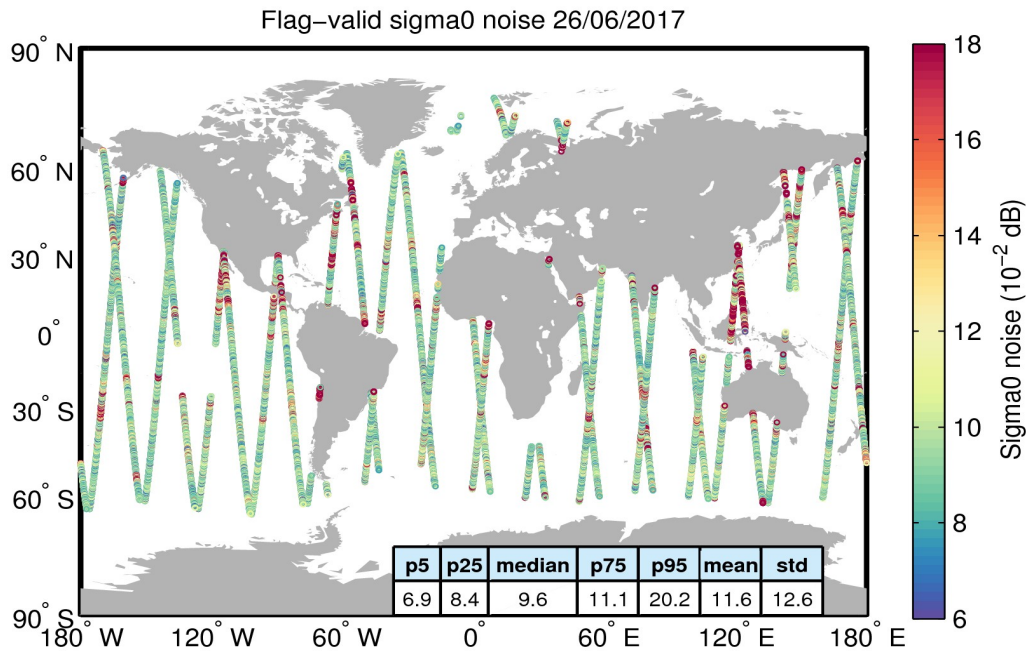
Figure 26. Geographical distribution of flag-valid 20-Hz sigma0 measurement noise over oceans and lakes for 26/06/2017. The statistical values shown in the table refer to the sigma0 noise and are calculated over all measurements shown in the figure.
