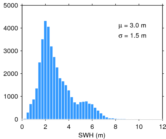
Figure 20. Histogram of science-valid SWH over oceans and lakes for 26/06/2017. The mean ( \mu ) and standard deviation ( \sigma ) are also shown. Note that values larger than 12 m are excluded from the histogram for the sake of readability but not from the computation of \mu and \sigma .
