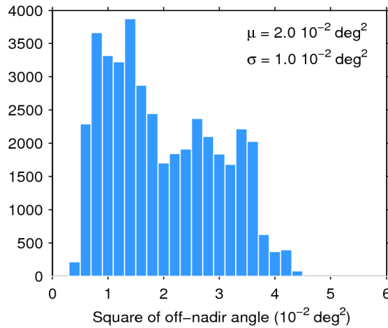
Figure 39. Histogram of flag-valid mispointing over oceans and lakes for 26/06/2017. The mean ( \mu ) and standard deviation ( \sigma ) are also shown. Note that values larger than 6 \cdot 10^{-2} \text{ deg}^2 are excluded from the histogram for the sake of readability but not from the computation of \mu and \sigma .
