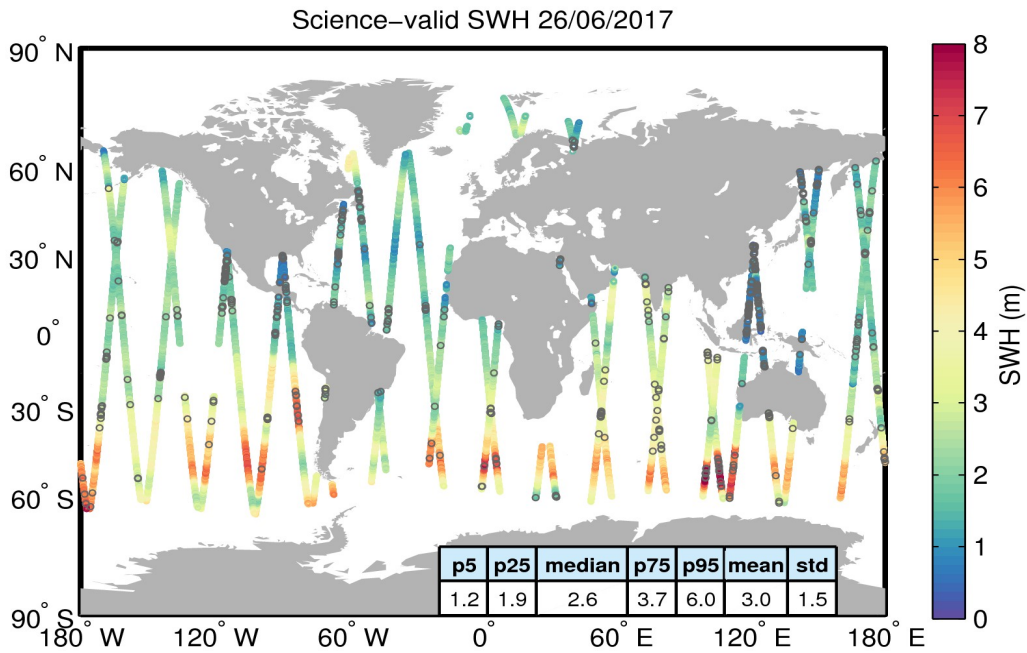
Figure 19. Geographical distribution of science-valid SWH data over oceans and lakes for 26/06/2017. The statistical values shown in the table refer to the SWH in m and are calculated over all measurements shown in the figure. Gray circles denote records that have been rejected based on the editing criteria described in Table 3.
