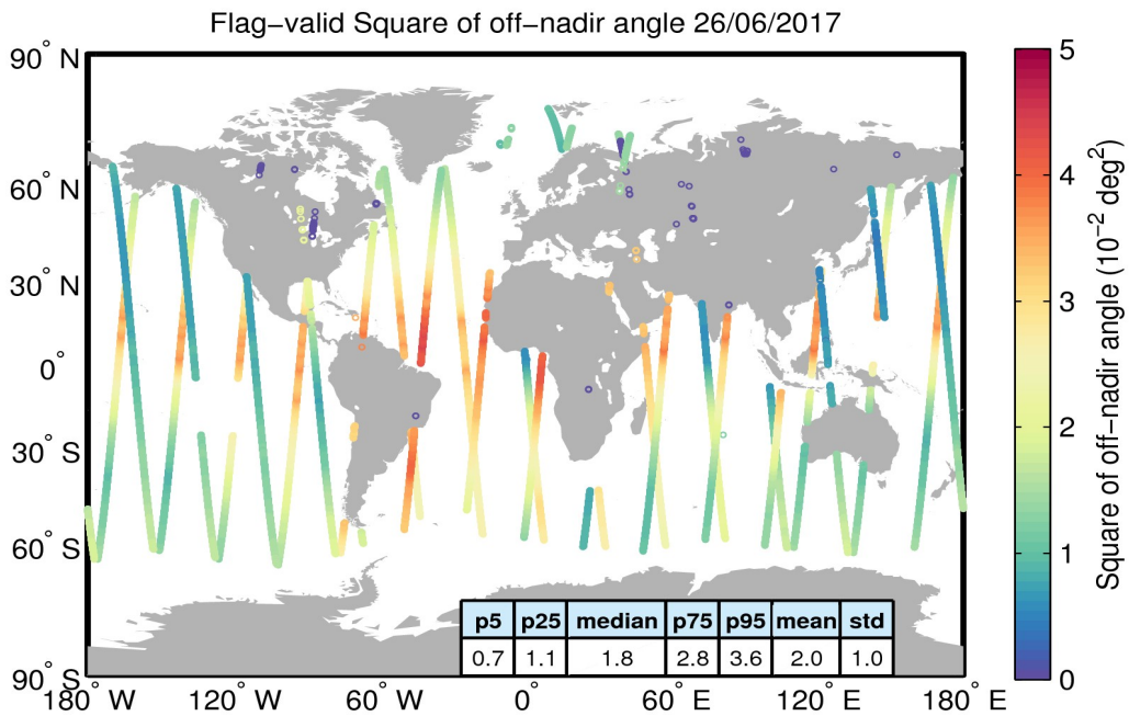
Figure 37. Geographical distribution of flag-valid mispointing data over oceans and lakes for 26/06/2017. The statistical values shown in the table refer to the mispointing in 10^{-2} deg 2 and are calculated over all measurements shown in the figure.
