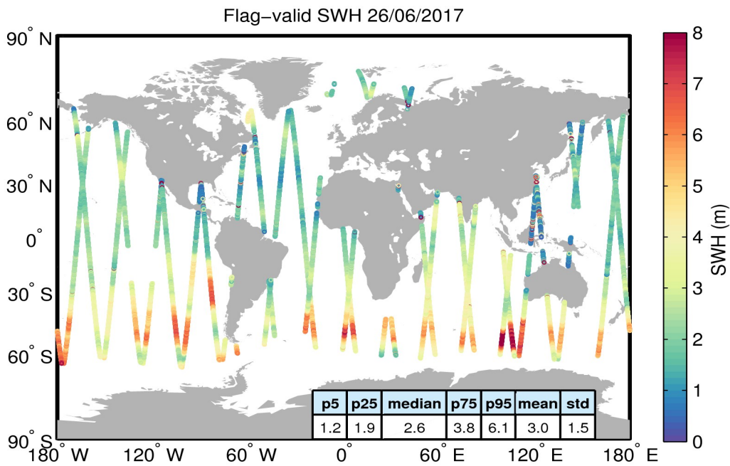
Figure 15. Geographical distribution of flag-valid SWH data over oceans and lakes for 26/06/2017. The statistical values shown in the table refer to the SWH in m and are calculated over all measurements shown in the figure.
