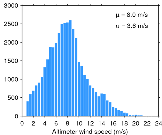
Figure 35. Histogram of science-valid wind over oceans and lakes for 26/06/2017. The mean ( \mu ) and standard deviation ( \sigma ) are also shown. Note that values larger than 24 m/s are excluded from the histogram for the sake of readability but not from the computation of \mu and \sigma .
