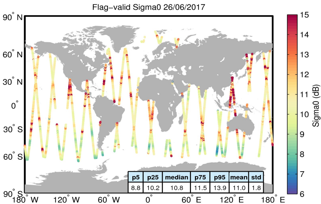
Figure 23. Geographical distribution of flag-valid sigma0 data over oceans and lakes for 26/06/2017. The statistical values shown in the table refer to the sigma0 in dB and are calculated over all measurements shown in the figure.
