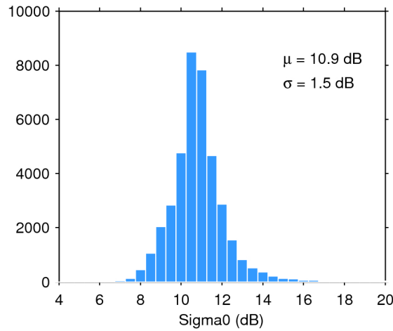
Figure 28. Histogram of science-valid sigma0 over oceans and lakes for 26/06/2017. The mean ( \mu ) and standard deviation ( \sigma ) are also shown. Note that values outside [4 20] dB are excluded from the histogram for the sake of readability but not from the computation of \mu and \sigma .
