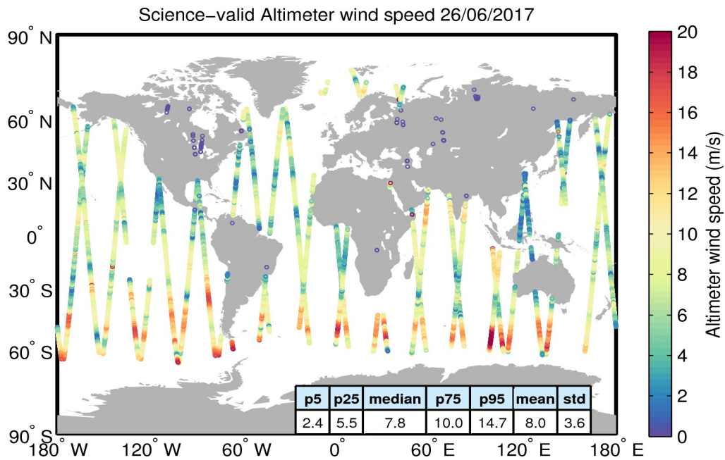
Figure 34. Geographical distribution of science-valid wind data over oceans and lakes for 26/06/2017. The statistical values shown in the table refer to the wind in m/s and are calculated over all measurements shown in the figure. Gray circles denote records that have been rejected based on the editing criteria described in Table 5.
