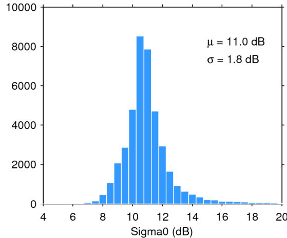
Figure 25. Histogram of flag-valid sigma0 over oceans and lakes for 26/06/2017. The mean ( \mu ) and standard deviation ( \sigma ) are also shown. Note that values outside [4 20] dB are excluded from the histogram for the sake of readability but not from the computation of \mu and \sigma .
