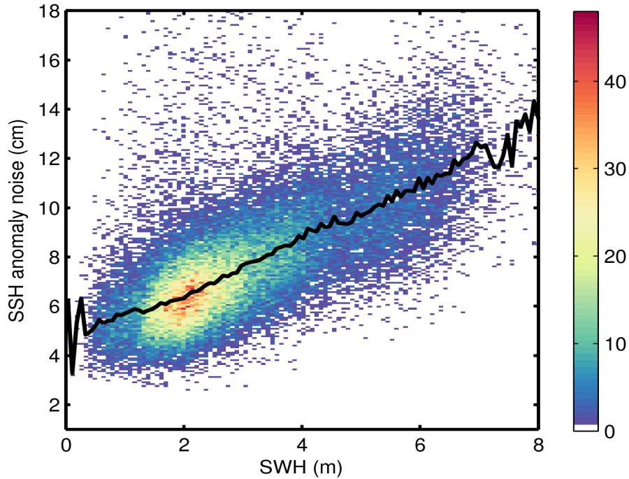
Figure 9. 2D histogram showing flag-valid SSH anomaly noise as a function of SWH for 26/06/2017. The black line denotes the median SSH anomaly noise as a function of SWH.
