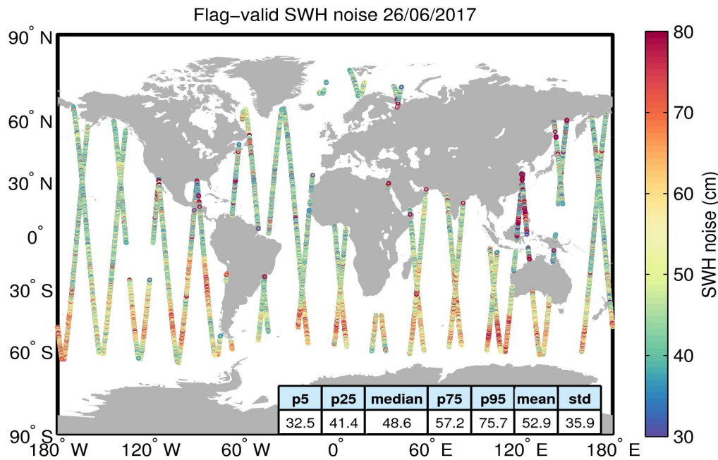
Figure 18. Geographical distribution of flag-valid 20-Hz SWH measurement noise over oceans and lakes for 26/06/2017. The statistical values shown in the table refer to the SWH noise and are calculated over all measurements shown in the figure.
