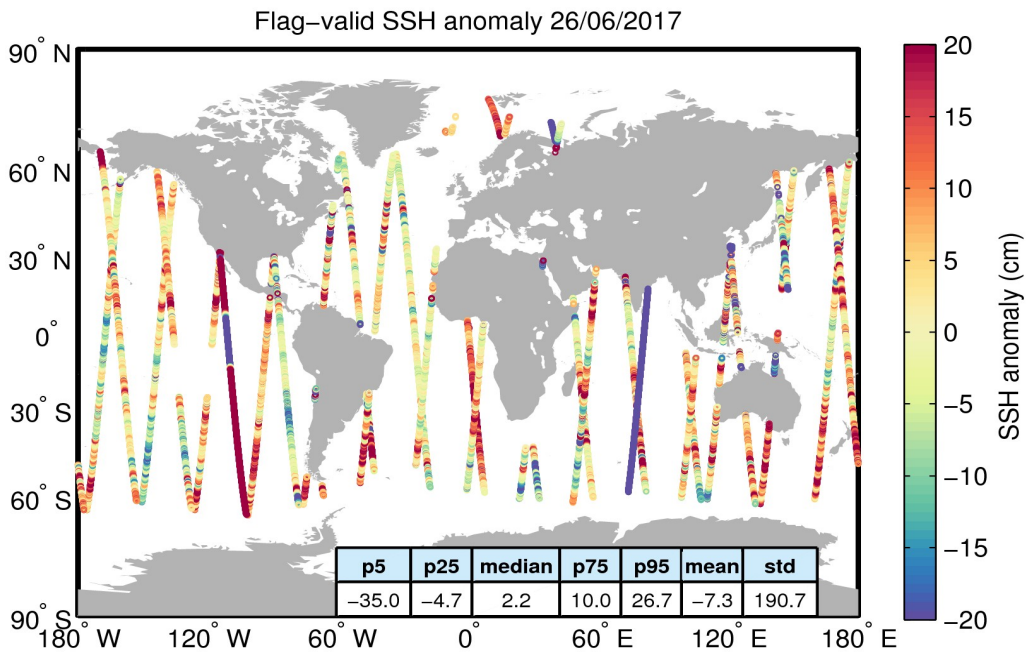
Figure 5. Geographical distribution of flag-valid 1-Hz SSH anomaly data over oceans and lakes for 26/06/2017. The statistical values shown in the table refer to the SSH anomaly in cm and are calculated over all measurements shown in the figure.
