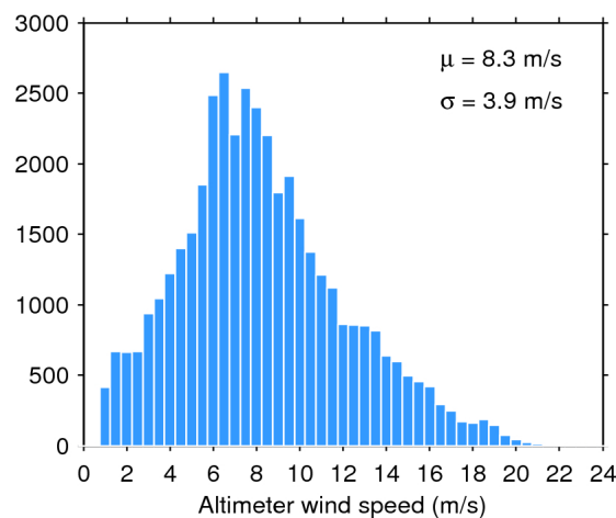
Figure 35. Histogram of science-valid wind over oceans and lakes for 25/06/2017. The mean ( \mu ) and standard deviation ( \sigma ) are also shown. Note that values larger than 24 m/s are excluded from the histogram for the sake of readability but not from the computation of \mu and \sigma .
