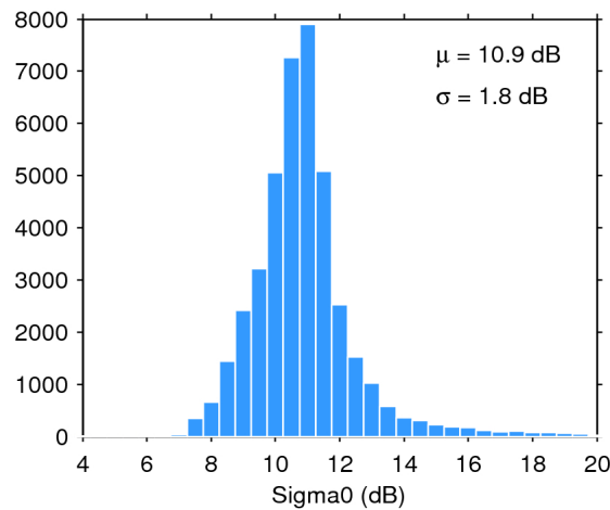
Figure 25. Histogram of flag-valid sigma0 over oceans and lakes for 25/06/2017. The mean ( \mu ) and standard deviation ( \sigma ) are also shown. Note that values outside [4 20] dB are excluded from the histogram for the sake of readability but not from the computation of \mu and \sigma .
