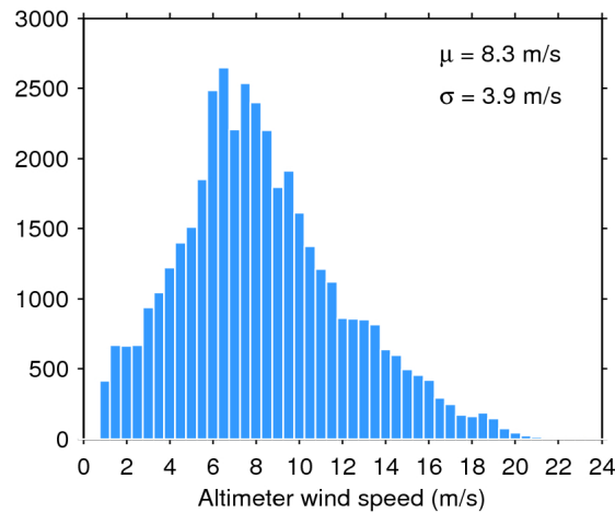
Figure 33. Histogram of flag-valid wind over oceans and lakes for 25/06/2017. The mean ( \mu ) and standard deviation ( \sigma ) are also shown. Note that values larger than 24 m/s are excluded from the histogram for the sake of readability but not from the computation of \mu and \sigma .
