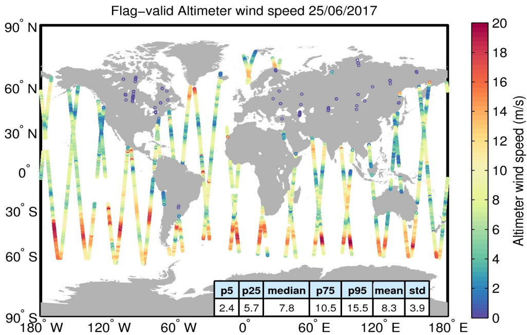
Figure 31. Geographical distribution of flag-valid wind data over oceans and lakes for 25/06/2017. The statistical values shown in the table refer to the wind in m/s and are calculated over all measurements shown in the figure.
