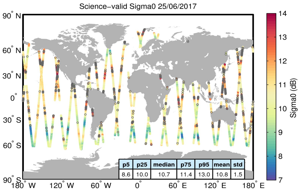
Figure 27. Geographical distribution of science-valid sigma0 data over oceans and lakes for 25/06/2017. The statistical values shown in the table refer to the sigma0 in dB and are calculated over all measurements shown in the figure. Gray circles denote records that have been rejected based on the editing criteria described in Table 4.
