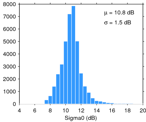
Figure 28. Histogram of science-valid sigma0 over oceans and lakes for 25/06/2017. The mean ( \mu ) and standard deviation ( \sigma ) are also shown. Note that values outside [4 20] dB are excluded from the histogram for the sake of readability but not from the computation of \mu and \sigma .
