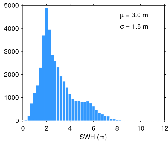
Figure 17. Histogram of flag-valid SWH over oceans and lakes for 25/06/2017. The mean ( \mu ) and standard deviation ( \sigma ) are also shown. Note that values larger than 12 m are excluded from the histogram for the sake of readability but not from the computation of \mu and \sigma .
