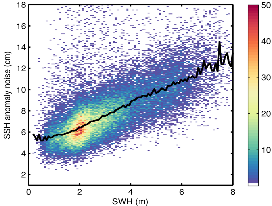
Figure 9. 2D histogram showing flag-valid SSH anomaly noise as a function of SWH for 25/06/2017. The black line denotes the median SSH anomaly noise as a function of SWH.
