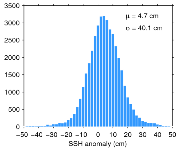
Figure 7. Histogram of flag-valid SSH anomaly over oceans and lakes for 25/06/2017. The mean ( \mu ) and standard deviation ( \sigma ) are also shown. Note that values outside [-50 50] cm are excluded from the histogram for the sake of readability but not from the computation of \mu and \sigma .
