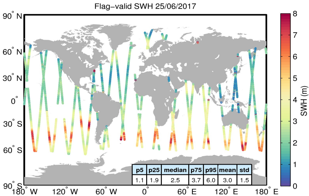
Figure 15. Geographical distribution of flag-valid SWH data over oceans and lakes for 25/06/2017. The statistical values shown in the table refer to the SWH in m and are calculated over all measurements shown in the figure.
