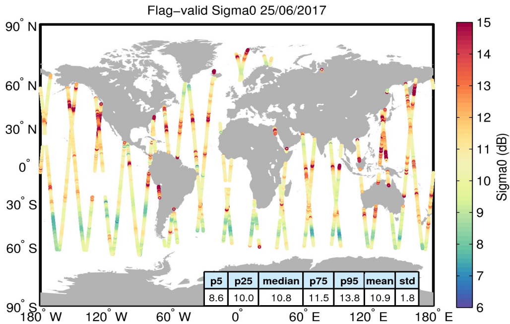
Figure 23. Geographical distribution of flag-valid sigma0 data over oceans and lakes for 25/06/2017. The statistical values shown in the table refer to the sigma0 in dB and are calculated over all measurements shown in the figure.
