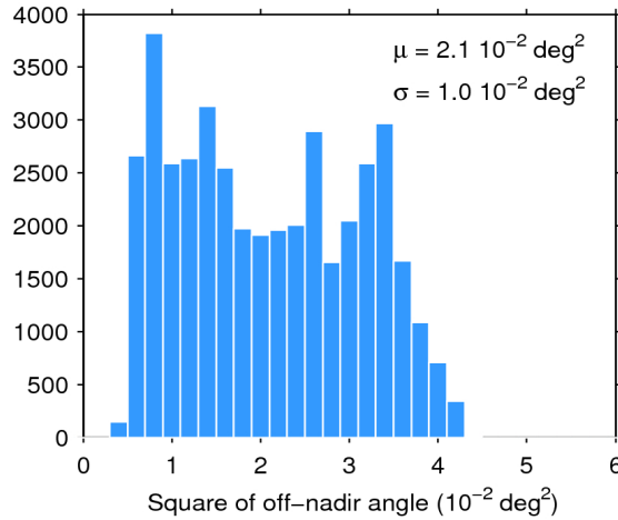
Figure 39. Histogram of flag-valid mispointing over oceans and lakes for 25/06/2017. The mean ( \mu ) and standard deviation ( \sigma ) are also shown. Note that values larger than 6 \cdot 10^{-2} \text{ deg}^2 are excluded from the histogram for the sake of readability but not from the computation of \mu and \sigma .
