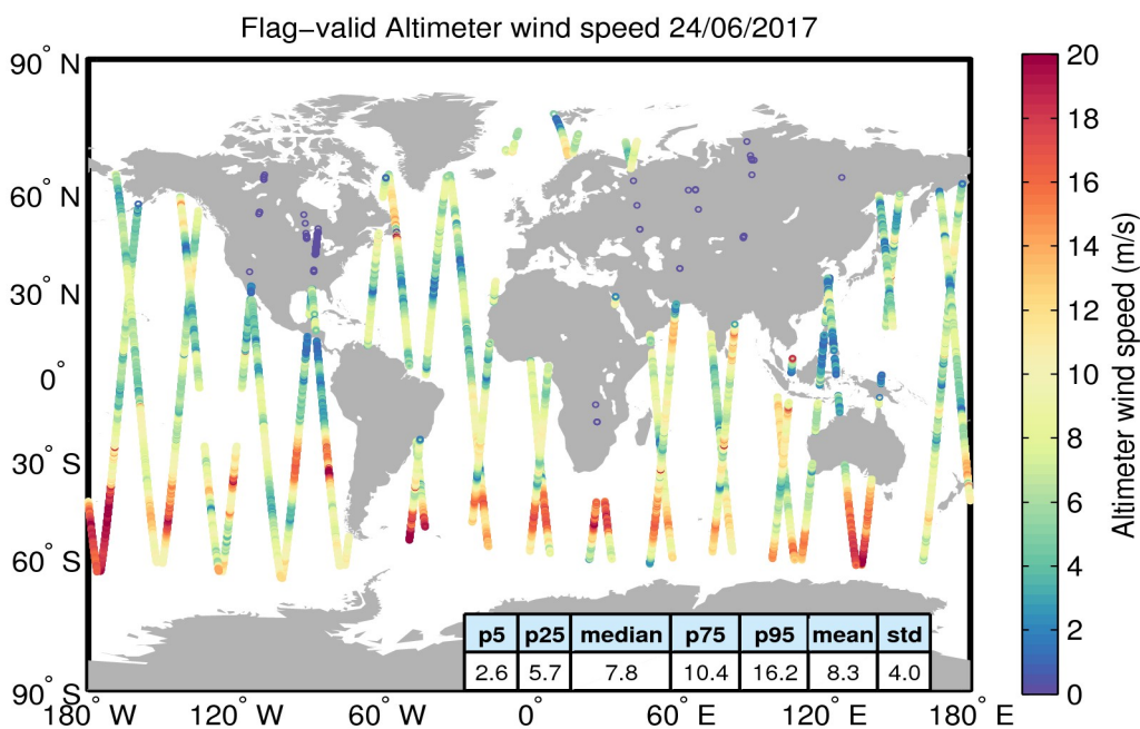
Figure 31. Geographical distribution of flag-valid wind data over oceans and lakes for 24/06/2017. The statistical values shown in the table refer to the wind in m/s and are calculated over all measurements shown in the figure.
