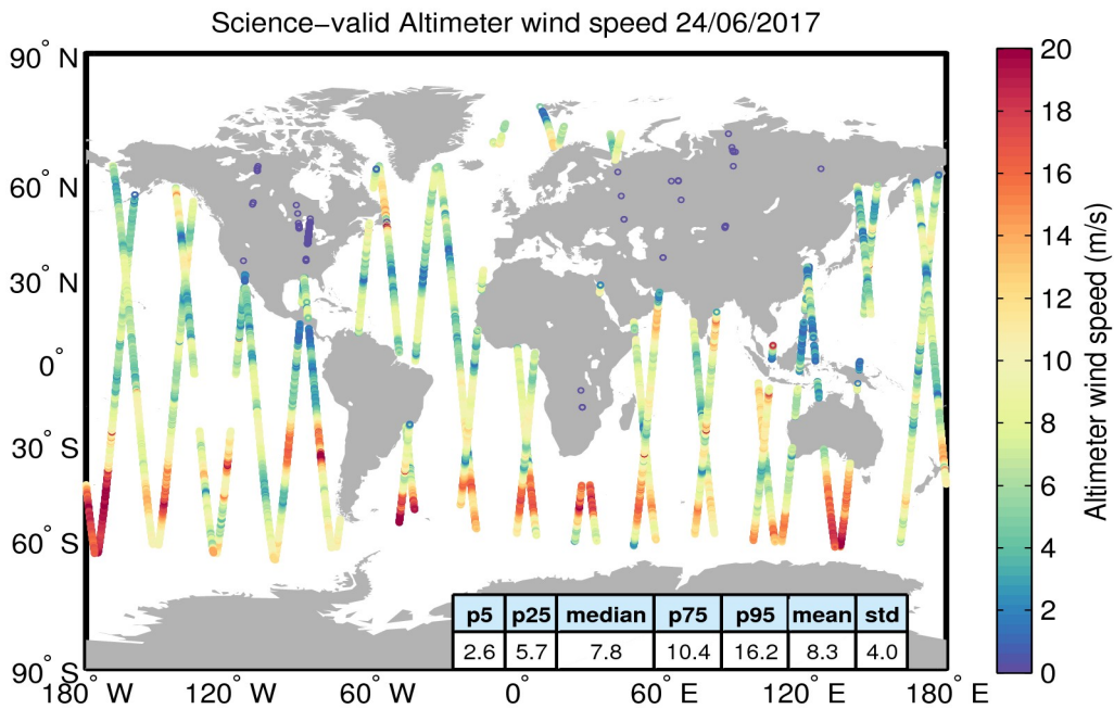
Figure 34. Geographical distribution of science-valid wind data over oceans and lakes for 24/06/2017. The statistical values shown in the table refer to the wind in m/s and are calculated over all measurements shown in the figure. Gray circles denote records that have been rejected based on the editing criteria described in Table 5.
