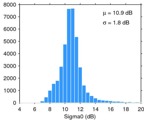
Figure 25. Histogram of flag-valid sigma0 over oceans and lakes for 24/06/2017. The mean ( \mu ) and standard deviation ( \sigma ) are also shown. Note that values outside [4 20] dB are excluded from the histogram for the sake of readability but not from the computation of \mu and \sigma .
