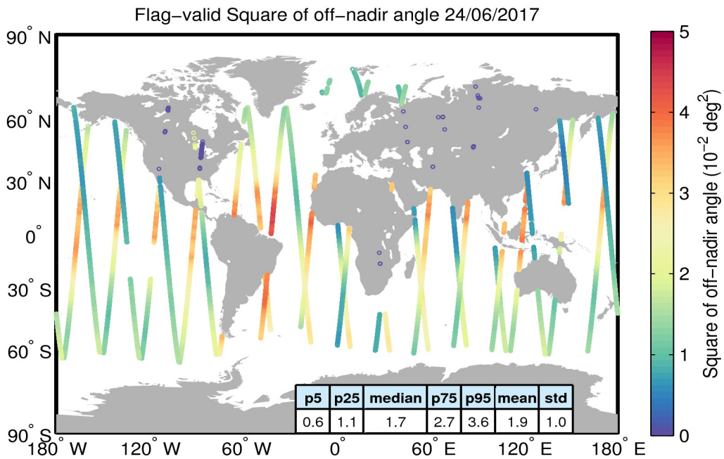
Figure 37. Geographical distribution of flag-valid mispointing data over oceans and lakes for 24/06/2017. The statistical values shown in the table refer to the mispointing in 10^{-2} deg 2 and are calculated over all measurements shown in the figure.
