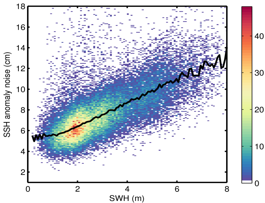
Figure 9. 2D histogram showing flag-valid SSH anomaly noise as a function of SWH for 24/06/2017. The black line denotes the median SSH anomaly noise as a function of SWH.
