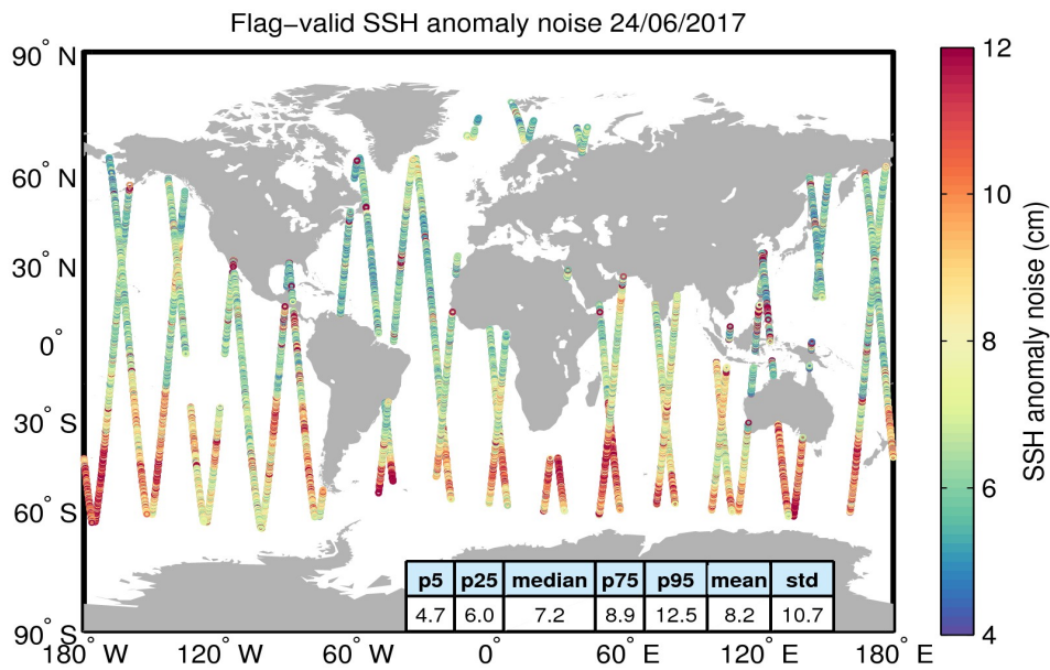
Figure 8. Geographical distribution of flag-valid 20-Hz SSH anomaly measurement noise over oceans and lakes for 24/06/2017. The statistical values shown in the table refer to the SSH anomaly noise and are calculated over all measurements shown in the figure.
