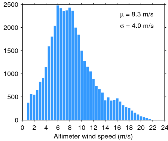
Figure 33. Histogram of flag-valid wind over oceans and lakes for 24/06/2017. The mean ( \mu ) and standard deviation ( \sigma ) are also shown. Note that values larger than 24 m/s are excluded from the histogram for the sake of readability but not from the computation of \mu and \sigma .
