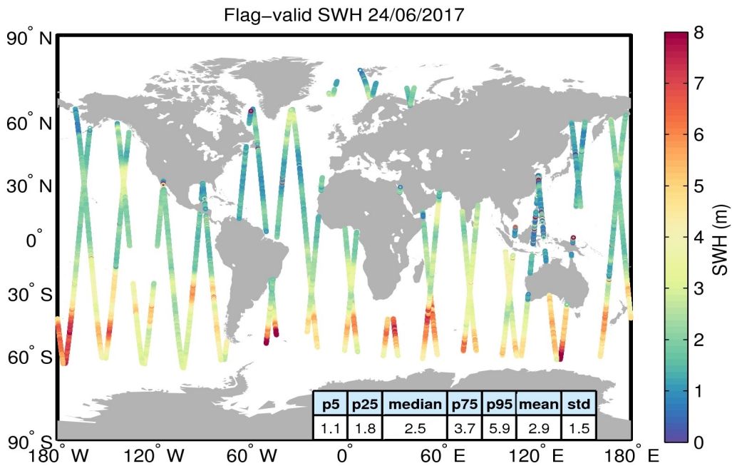
Figure 15. Geographical distribution of flag-valid SWH data over oceans and lakes for 24/06/2017. The statistical values shown in the table refer to the SWH in m and are calculated over all measurements shown in the figure.
