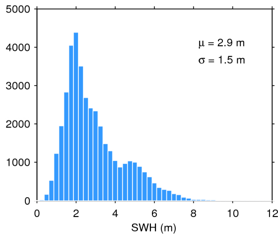
Figure 20. Histogram of science-valid SWH over oceans and lakes for 24/06/2017. The mean ( \mu ) and standard deviation ( \sigma ) are also shown. Note that values larger than 12 m are excluded from the histogram for the sake of readability but not from the computation of \mu and \sigma .
