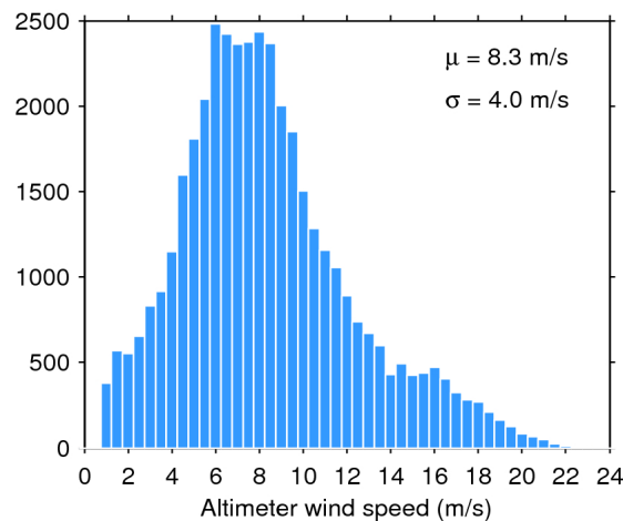
Figure 35. Histogram of science-valid wind over oceans and lakes for 24/06/2017. The mean ( \mu ) and standard deviation ( \sigma ) are also shown. Note that values larger than 24 m/s are excluded from the histogram for the sake of readability but not from the computation of \mu and \sigma .
