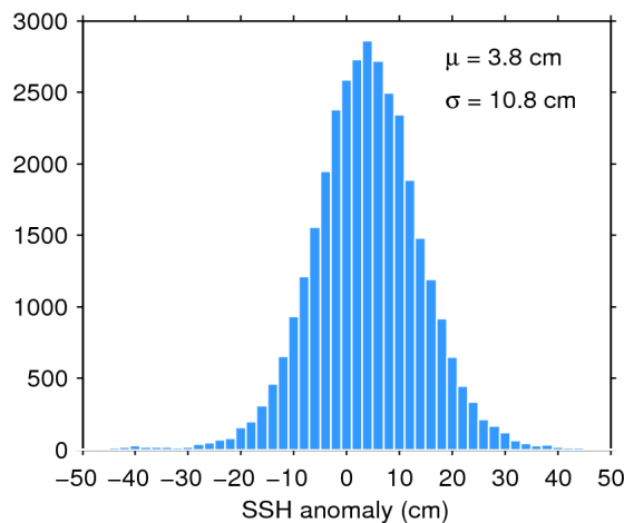
Figure 11. Histogram of science-valid SSH anomaly over oceans and lakes for 24/06/2017. The mean ( \mu ) and standard deviation ( \sigma ) are also shown. Note that values outside [-50 50] cm are excluded from the histogram for the sake of readability but not from the computation of \mu and \sigma .
