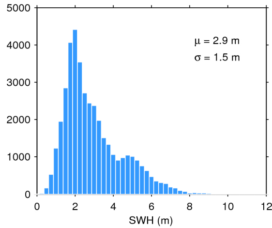
Figure 17. Histogram of flag-valid SWH over oceans and lakes for 24/06/2017. The mean ( \mu ) and standard deviation ( \sigma ) are also shown. Note that values larger than 12 m are excluded from the histogram for the sake of readability but not from the computation of \mu and \sigma .
