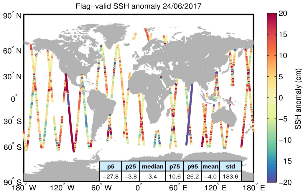
Figure 5. Geographical distribution of flag-valid 1-Hz SSH anomaly data over oceans and lakes for 24/06/2017. The statistical values shown in the table refer to the SSH anomaly in cm and are calculated over all measurements shown in the figure.
