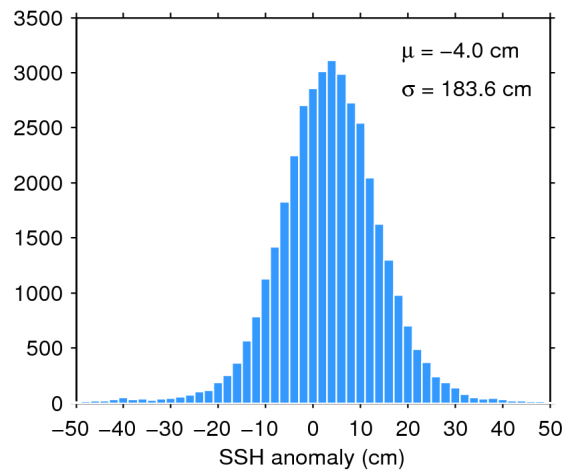
Figure 7. Histogram of flag-valid SSH anomaly over oceans and lakes for 24/06/2017. The mean ( \mu ) and standard deviation ( \sigma ) are also shown. Note that values outside [-50 50] cm are excluded from the histogram for the sake of readability but not from the computation of \mu and \sigma .
