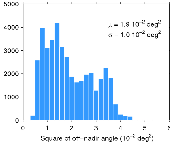
Figure 39. Histogram of flag-valid mispointing over oceans and lakes for 24/06/2017. The mean ( \mu ) and standard deviation ( \sigma ) are also shown. Note that values larger than 6 \cdot 10^{-2} \text{ deg}^2 are excluded from the histogram for the sake of readability but not from the computation of \mu and \sigma .
