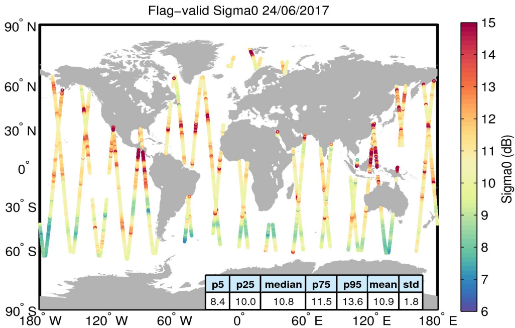
Figure 23. Geographical distribution of flag-valid sigma0 data over oceans and lakes for 24/06/2017. The statistical values shown in the table refer to the sigma0 in dB and are calculated over all measurements shown in the figure.
