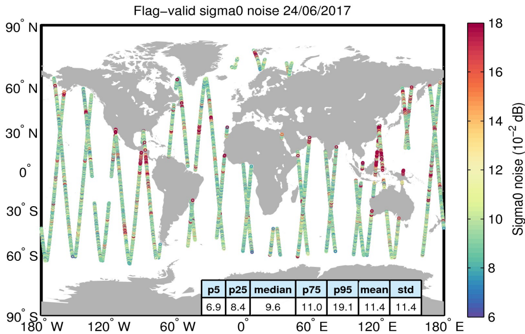
Figure 26. Geographical distribution of flag-valid 20-Hz sigma0 measurement noise over oceans and lakes for 24/06/2017. The statistical values shown in the table refer to the sigma0 noise and are calculated over all measurements shown in the figure.
