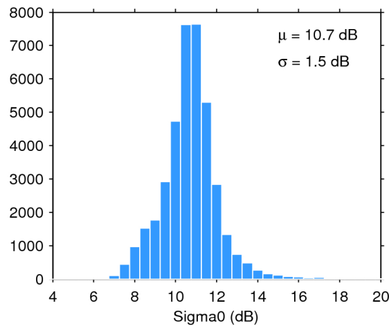
Figure 28. Histogram of science-valid sigma0 over oceans and lakes for 24/06/2017. The mean ( \mu ) and standard deviation ( \sigma ) are also shown. Note that values outside [4 20] dB are excluded from the histogram for the sake of readability but not from the computation of \mu and \sigma .
