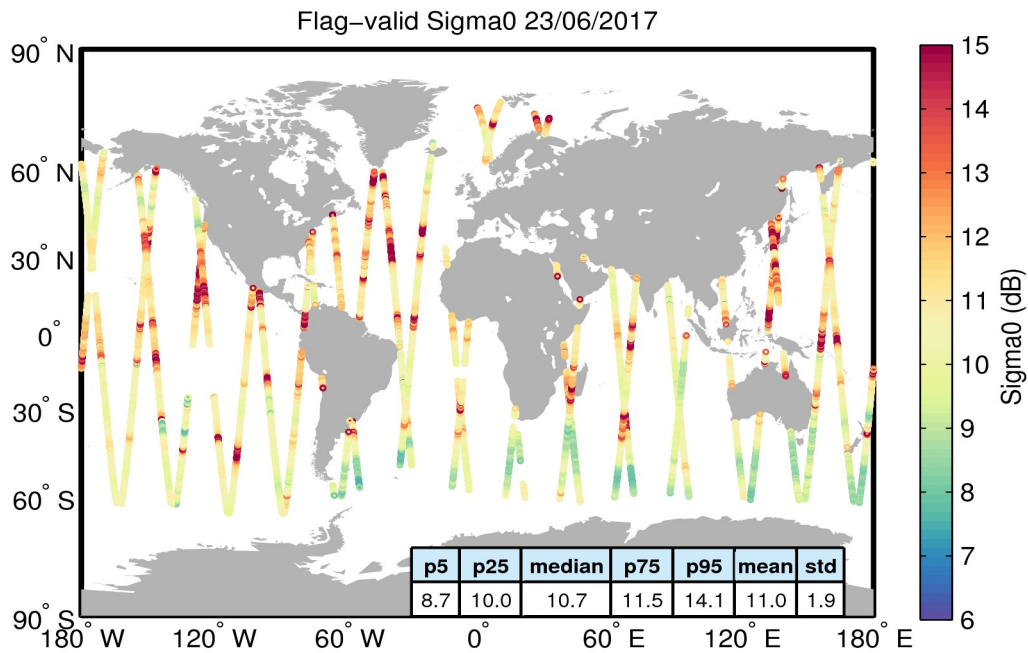
Figure 23. Geographical distribution of flag-valid sigma0 data over oceans and lakes for 23/06/2017. The statistical values shown in the table refer to the sigma0 in dB and are calculated over all measurements shown in the figure.
