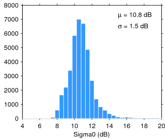
Figure 28. Histogram of science-valid sigma0 over oceans and lakes for 23/06/2017. The mean ( \mu ) and standard deviation ( \sigma ) are also shown. Note that values outside [4 20] dB are excluded from the histogram for the sake of readability but not from the computation of \mu and \sigma .
