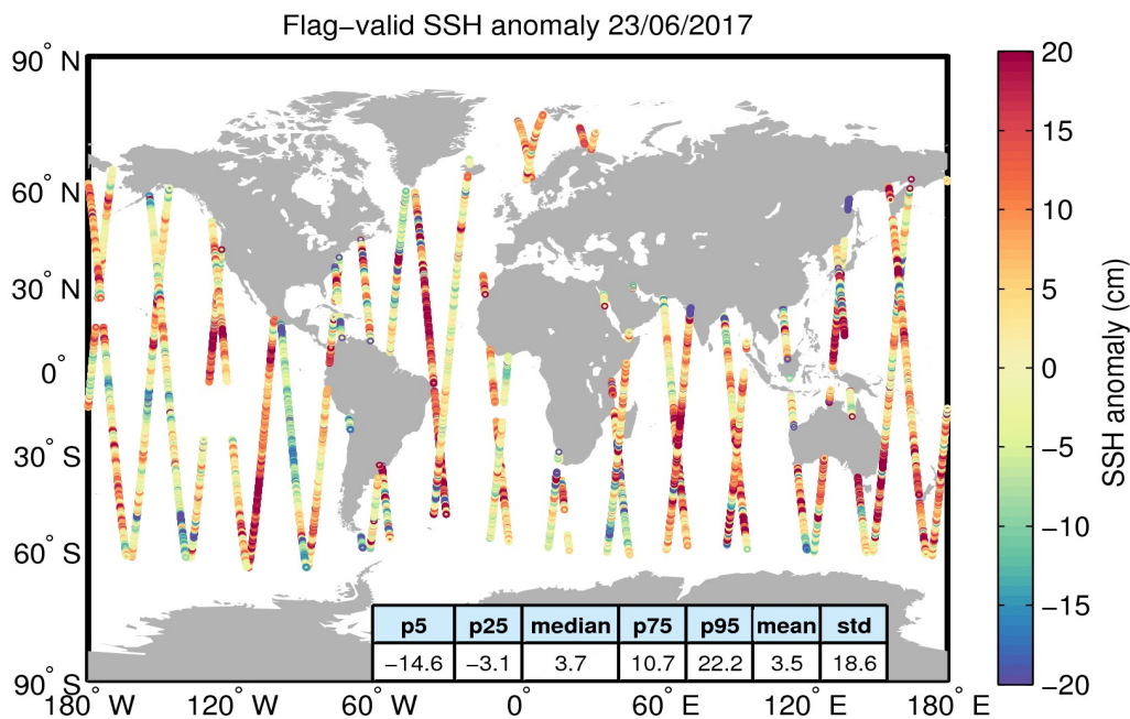
Figure 5. Geographical distribution of flag-valid 1-Hz SSH anomaly data over oceans and lakes for 23/06/2017. The statistical values shown in the table refer to the SSH anomaly in cm and are calculated over all measurements shown in the figure.
