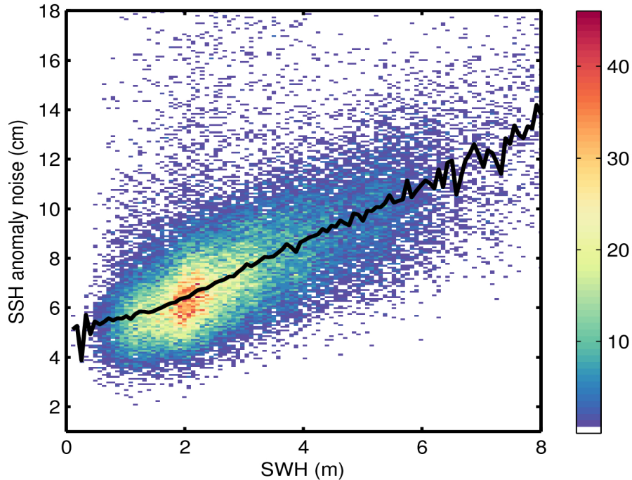
Figure 9. 2D histogram showing flag-valid SSH anomaly noise as a function of SWH for 23/06/2017. The black line denotes the median SSH anomaly noise as a function of SWH.
