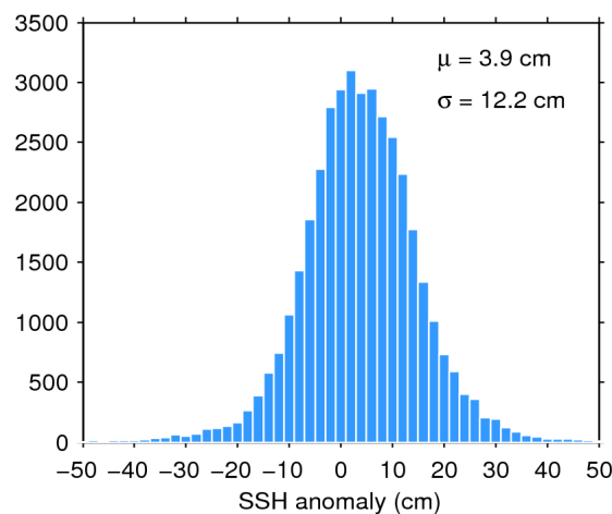
Figure 11. Histogram of science-valid SSH anomaly over oceans and lakes for 23/06/2017. The mean ( \mu ) and standard deviation ( \sigma ) are also shown. Note that values outside [-50 50] cm are excluded from the histogram for the sake of readability but not from the computation of \mu and \sigma .
