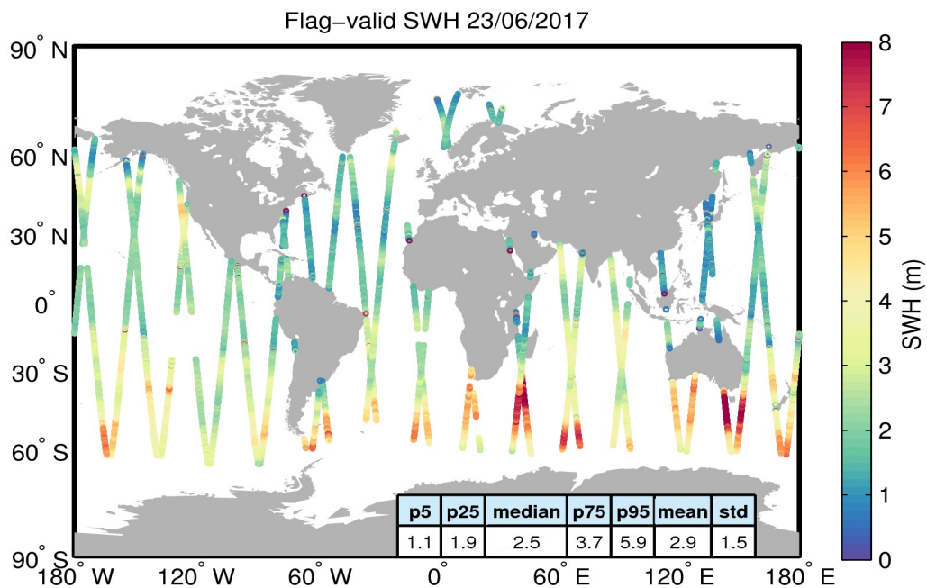
Figure 15. Geographical distribution of flag-valid SWH data over oceans and lakes for 23/06/2017. The statistical values shown in the table refer to the SWH in m and are calculated over all measurements shown in the figure.
