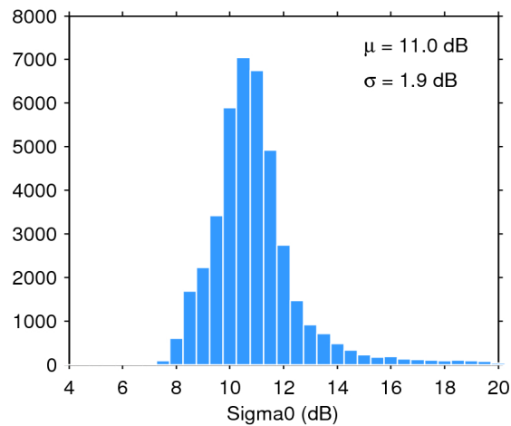
Figure 25. Histogram of flag-valid sigma0 over oceans and lakes for 23/06/2017. The mean ( \mu ) and standard deviation ( \sigma ) are also shown. Note that values outside [4 20] dB are excluded from the histogram for the sake of readability but not from the computation of \mu and \sigma .
