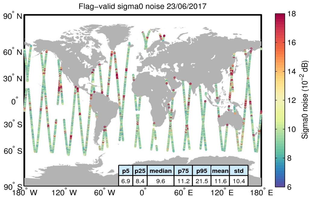
Figure 26. Geographical distribution of flag-valid 20-Hz sigma0 measurement noise over oceans and lakes for 23/06/2017. The statistical values shown in the table refer to the sigma0 noise and are calculated over all measurements shown in the figure.
