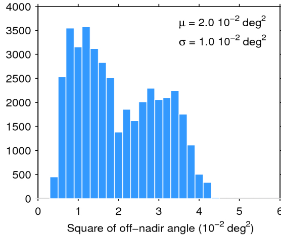
Figure 39. Histogram of flag-valid mispointing over oceans and lakes for 23/06/2017. The mean ( \mu ) and standard deviation ( \sigma ) are also shown. Note that values larger than 6 \cdot 10^{-2} \text{ deg}^2 are excluded from the histogram for the sake of readability but not from the computation of \mu and \sigma .
