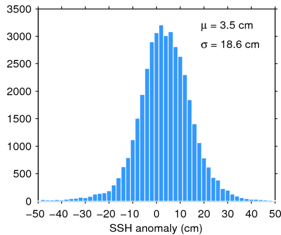
Figure 7. Histogram of flag-valid SSH anomaly over oceans and lakes for 23/06/2017. The mean ( \mu ) and standard deviation ( \sigma ) are also shown. Note that values outside [-50 50] cm are excluded from the histogram for the sake of readability but not from the computation of \mu and \sigma .
