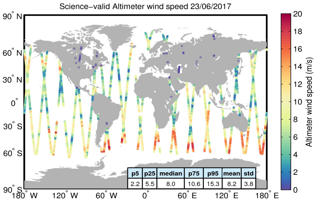
Figure 34. Geographical distribution of science-valid wind data over oceans and lakes for 23/06/2017. The statistical values shown in the table refer to the wind in m/s and are calculated over all measurements shown in the figure. Gray circles denote records that have been rejected based on the editing criteria described in Table 5.
