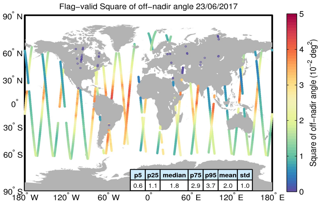
Figure 37. Geographical distribution of flag-valid mispointing data over oceans and lakes for 23/06/2017. The statistical values shown in the table refer to the mispointing in 10^{-2} deg 2 and are calculated over all measurements shown in the figure.
