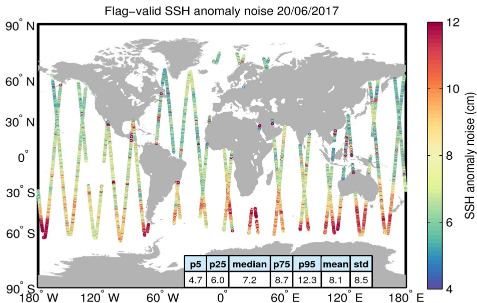
Figure 8. Geographical distribution of flag-valid 20-Hz SSH anomaly measurement noise over oceans and lakes for 20/06/2017. The statistical values shown in the table refer to the SSH anomaly noise and are calculated over all measurements shown in the figure.
