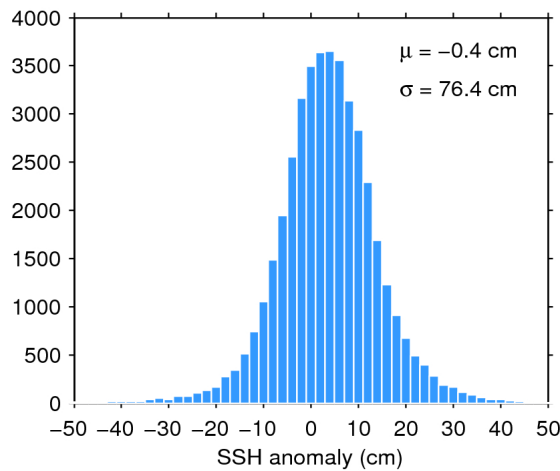
Figure 7. Histogram of flag-valid SSH anomaly over oceans and lakes for 20/06/2017. The mean ( \mu ) and standard deviation ( \sigma ) are also shown. Note that values outside [-50 50] cm are excluded from the histogram for the sake of readability but not from the computation of \mu and \sigma .
