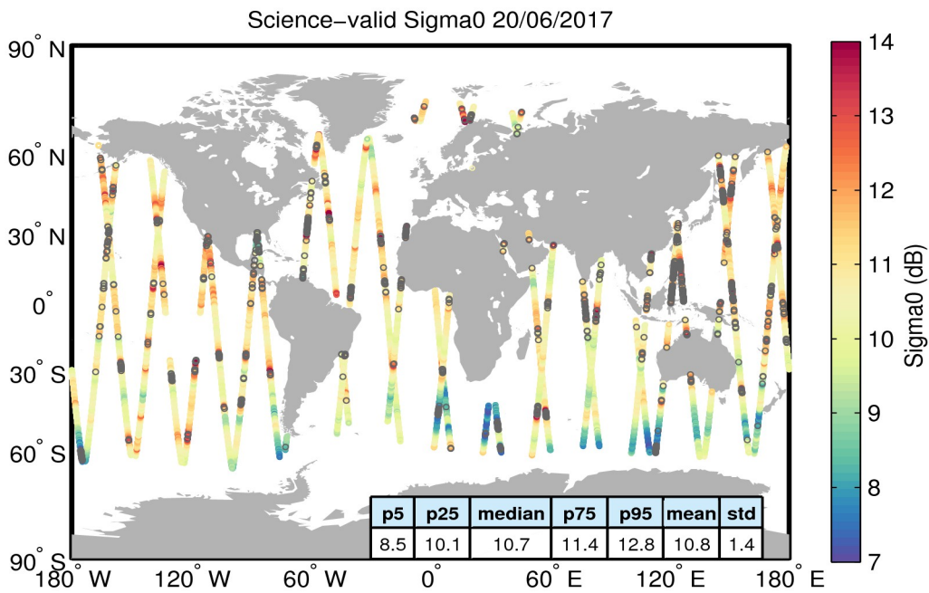
Figure 27. Geographical distribution of science-valid sigma0 data over oceans and lakes for 20/06/2017. The statistical values shown in the table refer to the sigma0 in dB and are calculated over all measurements shown in the figure. Gray circles denote records that have been rejected based on the editing criteria described in Table 4.
