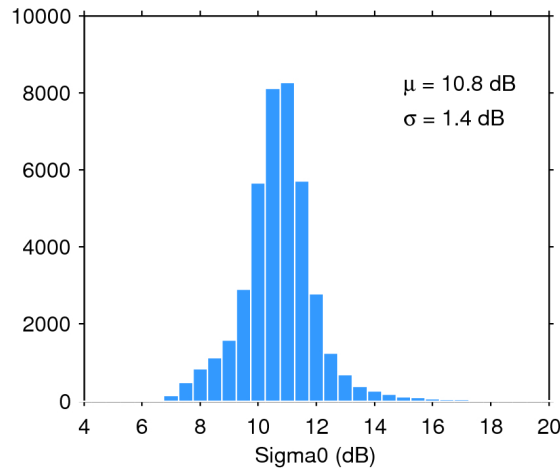
Figure 28. Histogram of science-valid sigma0 over oceans and lakes for 20/06/2017. The mean ( \mu ) and standard deviation ( \sigma ) are also shown. Note that values outside [4 20] dB are excluded from the histogram for the sake of readability but not from the computation of \mu and \sigma .
