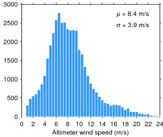
Figure 33. Histogram of flag-valid wind over oceans and lakes for 20/06/2017. The mean ( \mu ) and standard deviation ( \sigma ) are also shown. Note that values larger than 24 m/s are excluded from the histogram for the sake of readability but not from the computation of \mu and \sigma .
