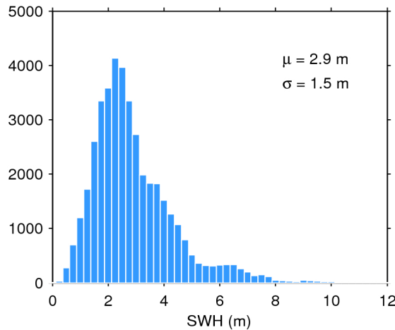
Figure 20. Histogram of science-valid SWH over oceans and lakes for 20/06/2017. The mean ( \mu ) and standard deviation ( \sigma ) are also shown. Note that values larger than 12 m are excluded from the histogram for the sake of readability but not from the computation of \mu and \sigma .
