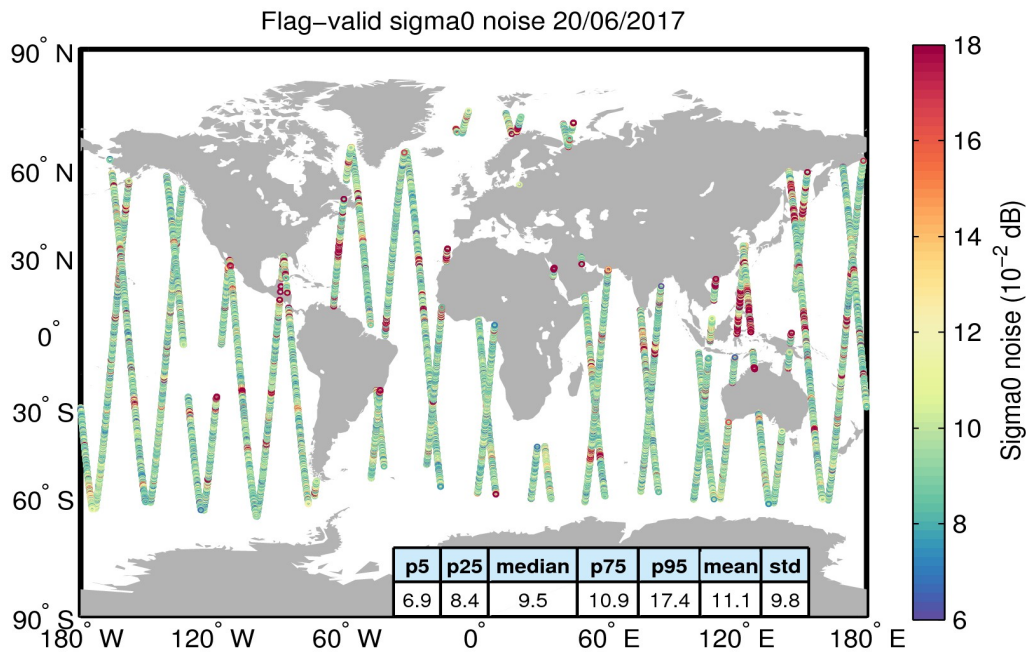
Figure 26. Geographical distribution of flag-valid 20-Hz sigma0 measurement noise over oceans and lakes for 20/06/2017. The statistical values shown in the table refer to the sigma0 noise and are calculated over all measurements shown in the figure.
