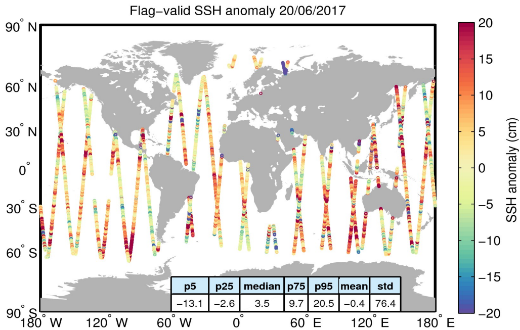
Figure 5. Geographical distribution of flag-valid 1-Hz SSH anomaly data over oceans and lakes for 20/06/2017. The statistical values shown in the table refer to the SSH anomaly in cm and are calculated over all measurements shown in the figure.
