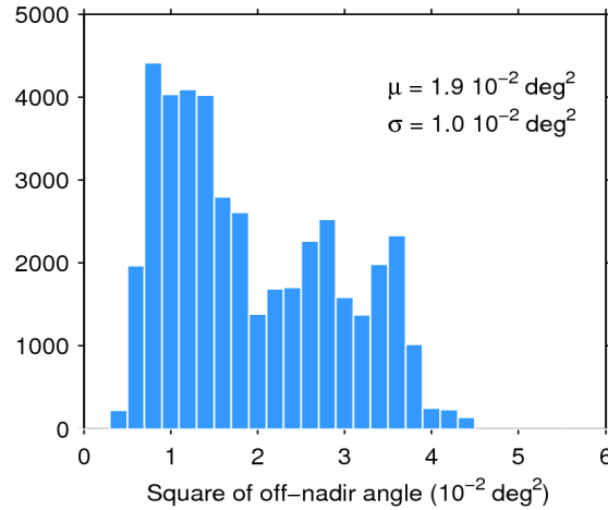
Figure 39. Histogram of flag-valid mispointing over oceans and lakes for 20/06/2017. The mean ( \mu ) and standard deviation ( \sigma ) are also shown. Note that values larger than 6 \cdot 10^{-2} \text{ deg}^2 are excluded from the histogram for the sake of readability but not from the computation of \mu and \sigma .
