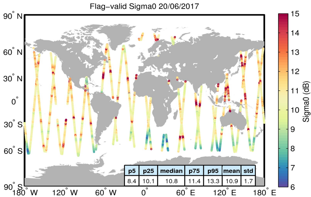
Figure 23. Geographical distribution of flag-valid sigma0 data over oceans and lakes for 20/06/2017. The statistical values shown in the table refer to the sigma0 in dB and are calculated over all measurements shown in the figure.
