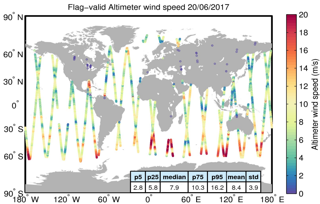
Figure 31. Geographical distribution of flag-valid wind data over oceans and lakes for 20/06/2017. The statistical values shown in the table refer to the wind in m/s and are calculated over all measurements shown in the figure.
