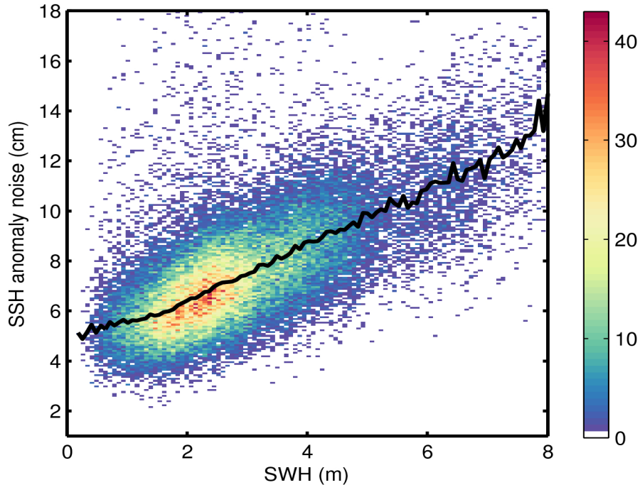
Figure 9. 2D histogram showing flag-valid SSH anomaly noise as a function of SWH for 20/06/2017. The black line denotes the median SSH anomaly noise as a function of SWH.
