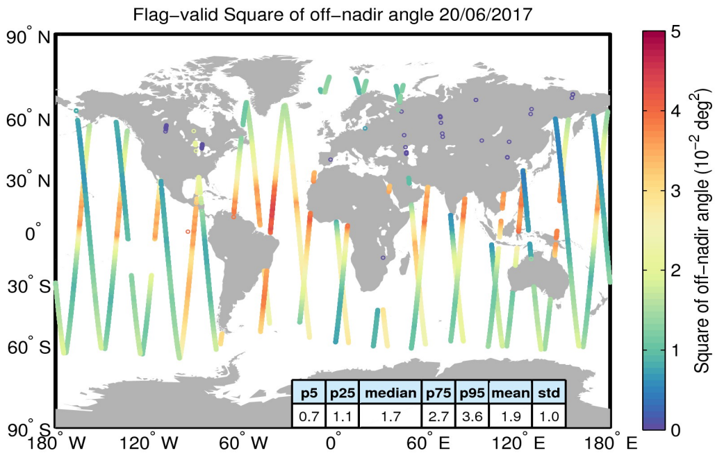
Figure 37. Geographical distribution of flag-valid mispointing data over oceans and lakes for 20/06/2017. The statistical values shown in the table refer to the mispointing in 10^{-2} deg 2 and are calculated over all measurements shown in the figure.
