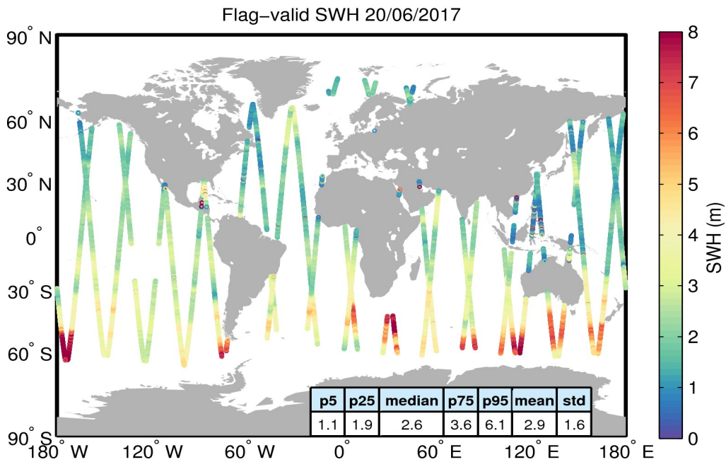
Figure 15. Geographical distribution of flag-valid SWH data over oceans and lakes for 20/06/2017. The statistical values shown in the table refer to the SWH in m and are calculated over all measurements shown in the figure.
