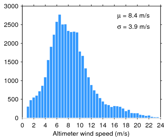
Figure 35. Histogram of science-valid wind over oceans and lakes for 20/06/2017. The mean ( \mu ) and standard deviation ( \sigma ) are also shown. Note that values larger than 24 m/s are excluded from the histogram for the sake of readability but not from the computation of \mu and \sigma .
