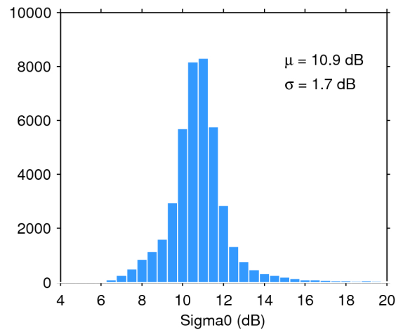
Figure 25. Histogram of flag-valid sigma0 over oceans and lakes for 20/06/2017. The mean ( \mu ) and standard deviation ( \sigma ) are also shown. Note that values outside [4 20] dB are excluded from the histogram for the sake of readability but not from the computation of \mu and \sigma .
