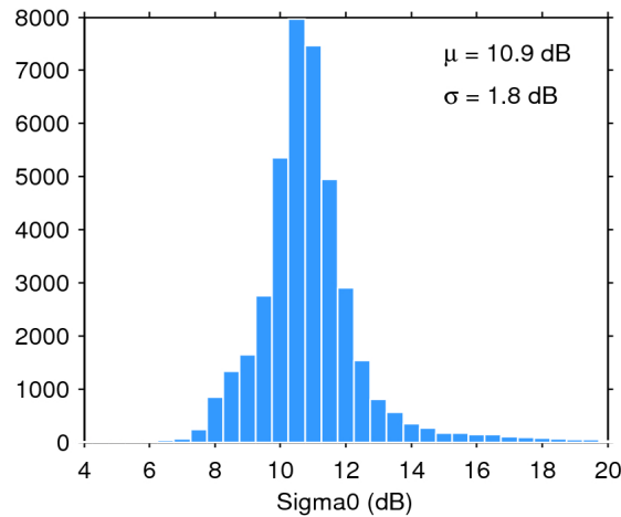
Figure 25. Histogram of flag-valid sigma0 over oceans and lakes for 19/06/2017. The mean ( \mu ) and standard deviation ( \sigma ) are also shown. Note that values outside [4 20] dB are excluded from the histogram for the sake of readability but not from the computation of \mu and \sigma .
