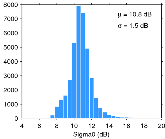
Figure 28. Histogram of science-valid sigma0 over oceans and lakes for 19/06/2017. The mean ( \mu ) and standard deviation ( \sigma ) are also shown. Note that values outside [4 20] dB are excluded from the histogram for the sake of readability but not from the computation of \mu and \sigma .
