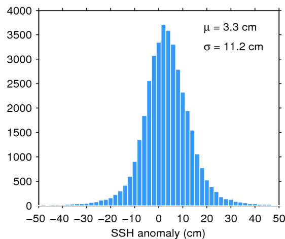
Figure 11. Histogram of science-valid SSH anomaly over oceans and lakes for 19/06/2017. The mean ( \mu ) and standard deviation ( \sigma ) are also shown. Note that values outside [-50 50] cm are excluded from the histogram for the sake of readability but not from the computation of \mu and \sigma .
