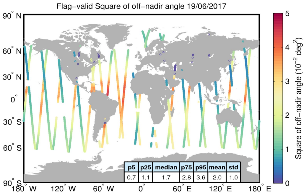
Figure 37. Geographical distribution of flag-valid mispointing data over oceans and lakes for 19/06/2017. The statistical values shown in the table refer to the mispointing in 10^{-2} deg 2 and are calculated over all measurements shown in the figure.
