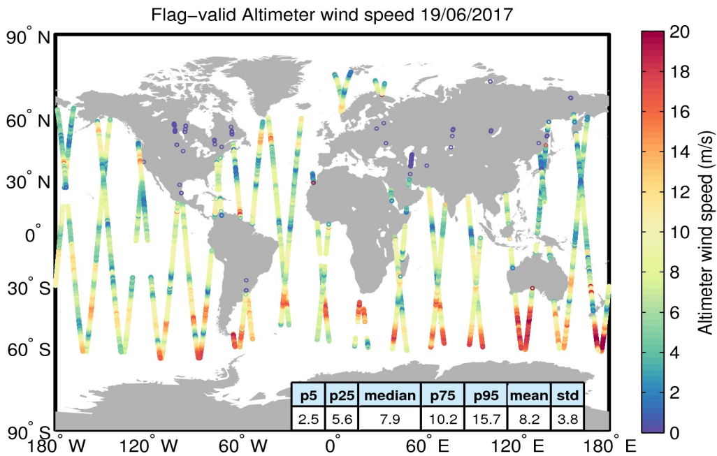
Figure 31. Geographical distribution of flag-valid wind data over oceans and lakes for 19/06/2017. The statistical values shown in the table refer to the wind in m/s and are calculated over all measurements shown in the figure.
