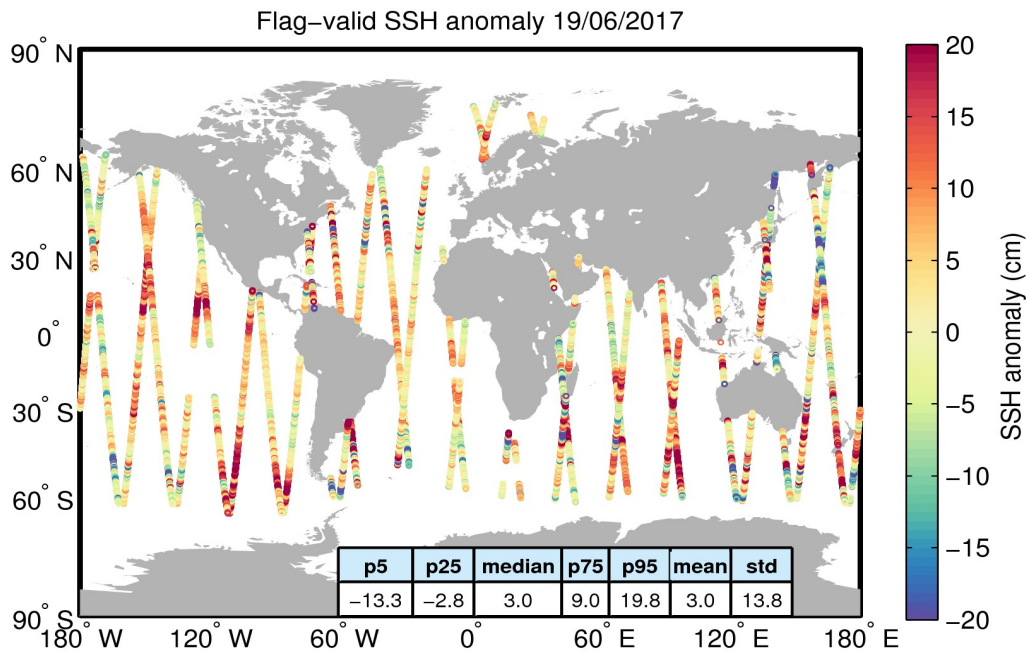
Figure 5. Geographical distribution of flag-valid 1-Hz SSH anomaly data over oceans and lakes for 19/06/2017. The statistical values shown in the table refer to the SSH anomaly in cm and are calculated over all measurements shown in the figure.
