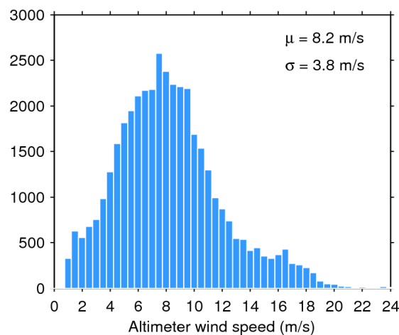
Figure 35. Histogram of science-valid wind over oceans and lakes for 19/06/2017. The mean ( \mu ) and standard deviation ( \sigma ) are also shown. Note that values larger than 24 m/s are excluded from the histogram for the sake of readability but not from the computation of \mu and \sigma .
