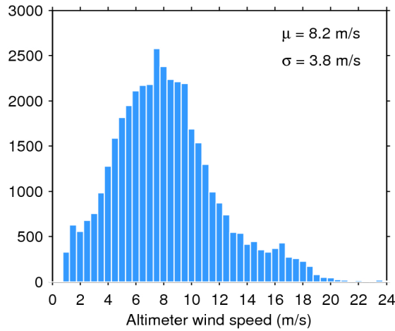
Figure 33. Histogram of flag-valid wind over oceans and lakes for 19/06/2017. The mean ( \mu ) and standard deviation ( \sigma ) are also shown. Note that values larger than 24 m/s are excluded from the histogram for the sake of readability but not from the computation of \mu and \sigma .
