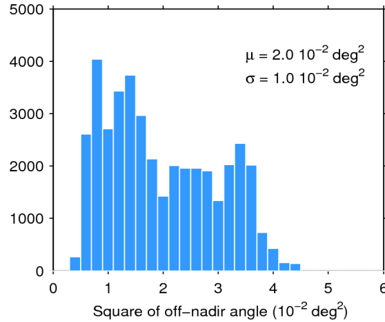
Figure 39. Histogram of flag-valid mispointing over oceans and lakes for 19/06/2017. The mean ( \mu ) and standard deviation ( \sigma ) are also shown. Note that values larger than 6 \cdot 10^{-2} \text{ deg}^2 are excluded from the histogram for the sake of readability but not from the computation of \mu and \sigma .
