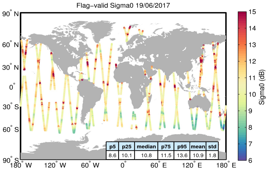
Figure 23. Geographical distribution of flag-valid sigma0 data over oceans and lakes for 19/06/2017. The statistical values shown in the table refer to the sigma0 in dB and are calculated over all measurements shown in the figure.
