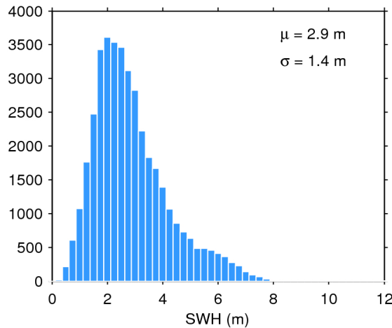
Figure 20. Histogram of science-valid SWH over oceans and lakes for 19/06/2017. The mean ( \mu ) and standard deviation ( \sigma ) are also shown. Note that values larger than 12 m are excluded from the histogram for the sake of readability but not from the computation of \mu and \sigma .
