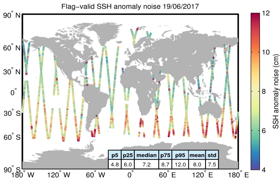
Figure 8. Geographical distribution of flag-valid 20-Hz SSH anomaly measurement noise over oceans and lakes for 19/06/2017. The statistical values shown in the table refer to the SSH anomaly noise and are calculated over all measurements shown in the figure.
