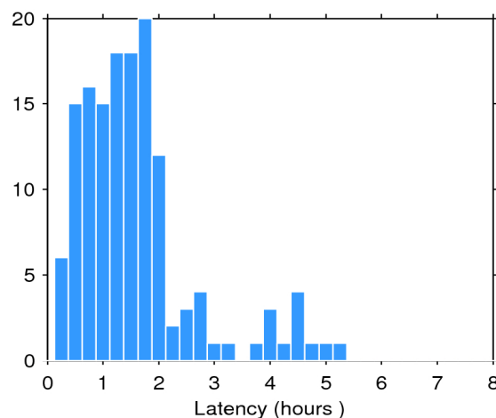
Figure 2. Histogram of the data latency for 19/06/2017. The y-axis denotes the number of files that are made available with a delay of x-hours with respect to the mean time of the records stored in the file.
