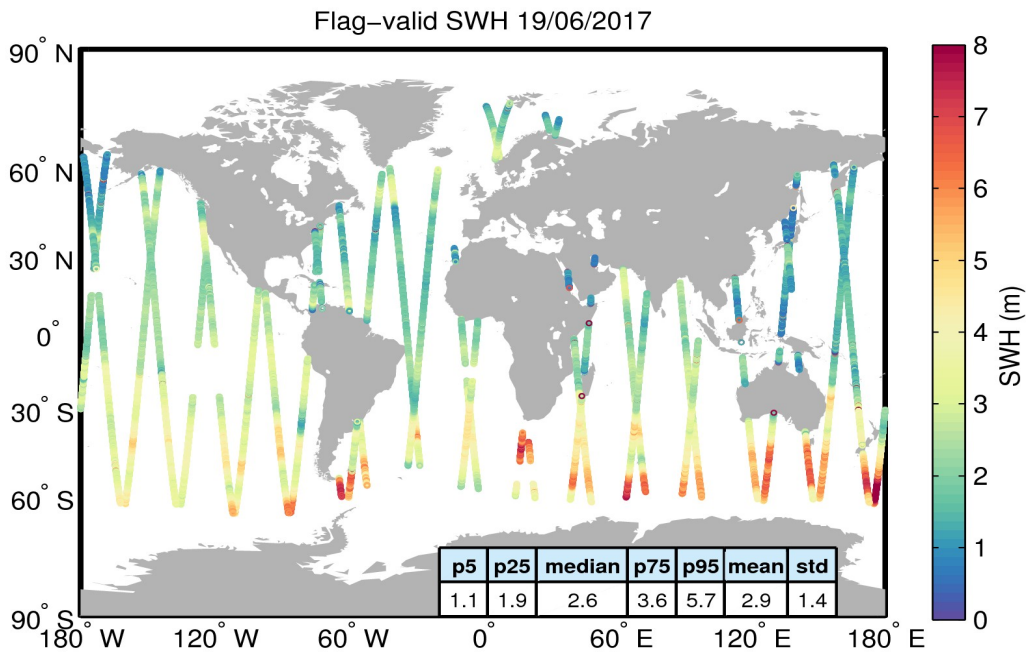
Figure 15. Geographical distribution of flag-valid SWH data over oceans and lakes for 19/06/2017. The statistical values shown in the table refer to the SWH in m and are calculated over all measurements shown in the figure.
