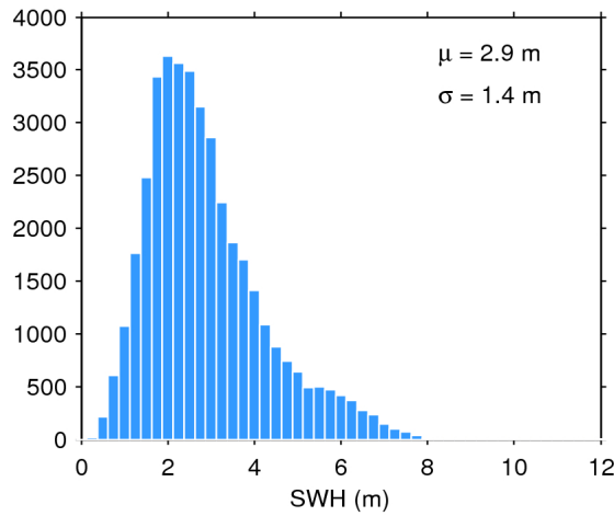
Figure 17. Histogram of flag-valid SWH over oceans and lakes for 19/06/2017. The mean ( \mu ) and standard deviation ( \sigma ) are also shown. Note that values larger than 12 m are excluded from the histogram for the sake of readability but not from the computation of \mu and \sigma .
