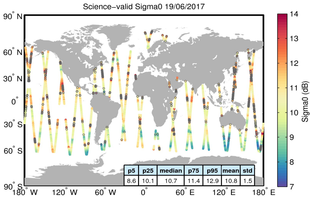
Figure 27. Geographical distribution of science-valid sigma0 data over oceans and lakes for 19/06/2017. The statistical values shown in the table refer to the sigma0 in dB and are calculated over all measurements shown in the figure. Gray circles denote records that have been rejected based on the editing criteria described in Table 4.
