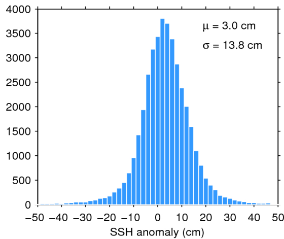
Figure 7. Histogram of flag-valid SSH anomaly over oceans and lakes for 19/06/2017. The mean ( \mu ) and standard deviation ( \sigma ) are also shown. Note that values outside [-50 50] cm are excluded from the histogram for the sake of readability but not from the computation of \mu and \sigma .
