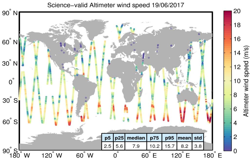
Figure 34. Geographical distribution of science-valid wind data over oceans and lakes for 19/06/2017. The statistical values shown in the table refer to the wind in m/s and are calculated over all measurements shown in the figure. Gray circles denote records that have been rejected based on the editing criteria described in Table 5.
