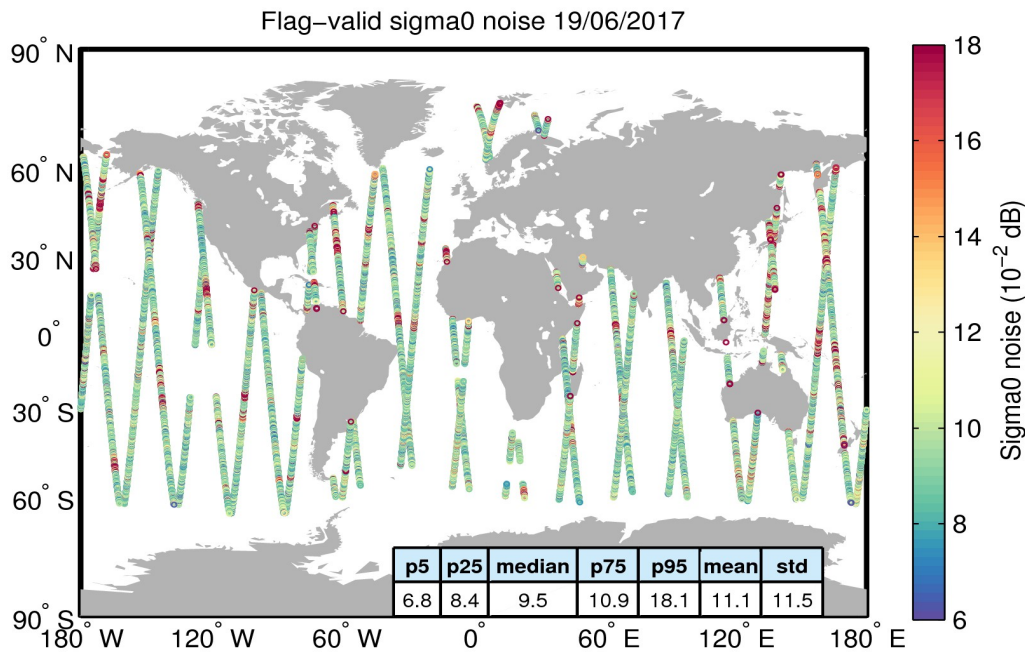
Figure 26. Geographical distribution of flag-valid 20-Hz sigma0 measurement noise over oceans and lakes for 19/06/2017. The statistical values shown in the table refer to the sigma0 noise and are calculated over all measurements shown in the figure.
