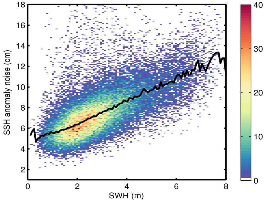
Figure 9. 2D histogram showing flag-valid SSH anomaly noise as a function of SWH for 19/06/2017. The black line denotes the median SSH anomaly noise as a function of SWH.
