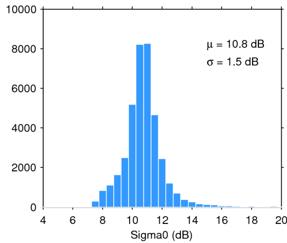
Figure 28. Histogram of science-valid sigma0 over oceans and lakes for 17/06/2017. The mean ( \mu ) and standard deviation ( \sigma ) are also shown. Note that values outside [4 20] dB are excluded from the histogram for the sake of readability but not from the computation of \mu and \sigma .
