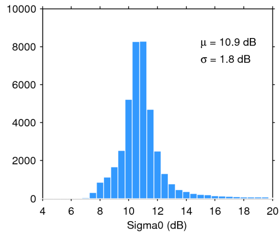
Figure 25. Histogram of flag-valid sigma0 over oceans and lakes for 17/06/2017. The mean ( \mu ) and standard deviation ( \sigma ) are also shown. Note that values outside [4 20] dB are excluded from the histogram for the sake of readability but not from the computation of \mu and \sigma .
