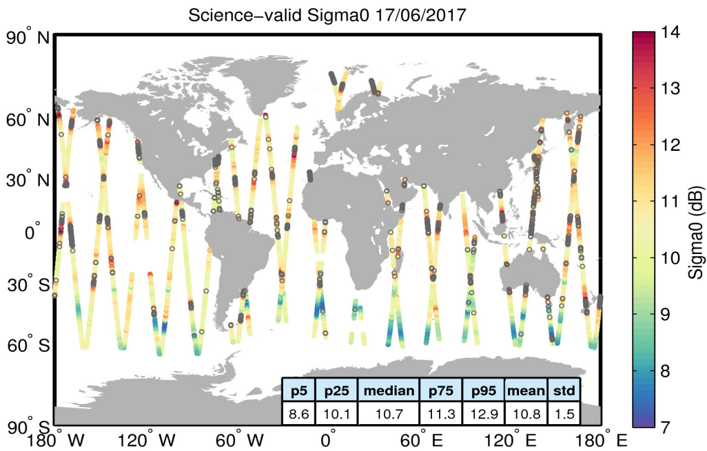
Figure 27. Geographical distribution of science-valid sigma0 data over oceans and lakes for 17/06/2017. The statistical values shown in the table refer to the sigma0 in dB and are calculated over all measurements shown in the figure. Gray circles denote records that have been rejected based on the editing criteria described in Table 4.
