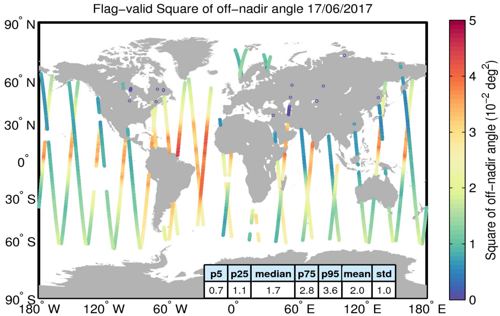
Figure 37. Geographical distribution of flag-valid mispointing data over oceans and lakes for 17/06/2017. The statistical values shown in the table refer to the mispointing in 10^{-2} deg 2 and are calculated over all measurements shown in the figure.
