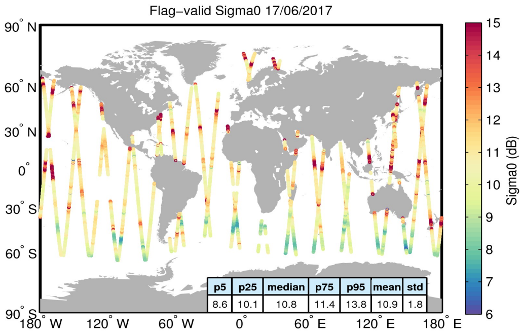
Figure 23. Geographical distribution of flag-valid sigma0 data over oceans and lakes for 17/06/2017. The statistical values shown in the table refer to the sigma0 in dB and are calculated over all measurements shown in the figure.
