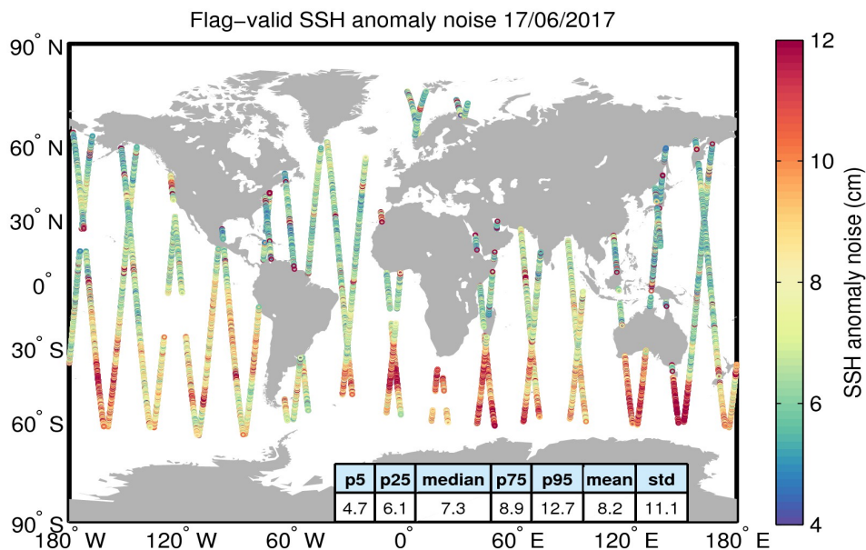
Figure 8. Geographical distribution of flag-valid 20-Hz SSH anomaly measurement noise over oceans and lakes for 17/06/2017. The statistical values shown in the table refer to the SSH anomaly noise and are calculated over all measurements shown in the figure.
