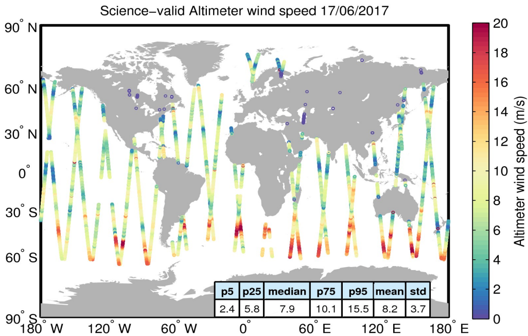
Figure 34. Geographical distribution of science-valid wind data over oceans and lakes for 17/06/2017. The statistical values shown in the table refer to the wind in m/s and are calculated over all measurements shown in the figure. Gray circles denote records that have been rejected based on the editing criteria described in Table 5.
