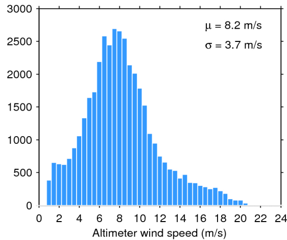
Figure 33. Histogram of flag-valid wind over oceans and lakes for 17/06/2017. The mean ( \mu ) and standard deviation ( \sigma ) are also shown. Note that values larger than 24 m/s are excluded from the histogram for the sake of readability but not from the computation of \mu and \sigma .
