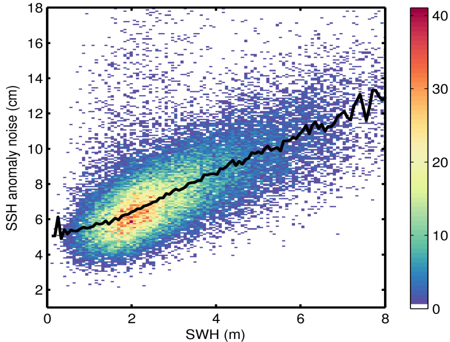
Figure 9. 2D histogram showing flag-valid SSH anomaly noise as a function of SWH for 17/06/2017. The black line denotes the median SSH anomaly noise as a function of SWH.
