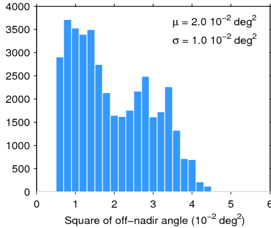
Figure 39. Histogram of flag-valid mispointing over oceans and lakes for 17/06/2017. The mean ( \mu ) and standard deviation ( \sigma ) are also shown. Note that values larger than 6 \cdot 10^{-2} \text{ deg}^2 are excluded from the histogram for the sake of readability but not from the computation of \mu and \sigma .
