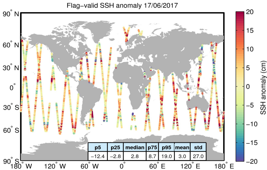
Figure 5. Geographical distribution of flag-valid 1-Hz SSH anomaly data over oceans and lakes for 17/06/2017. The statistical values shown in the table refer to the SSH anomaly in cm and are calculated over all measurements shown in the figure.
