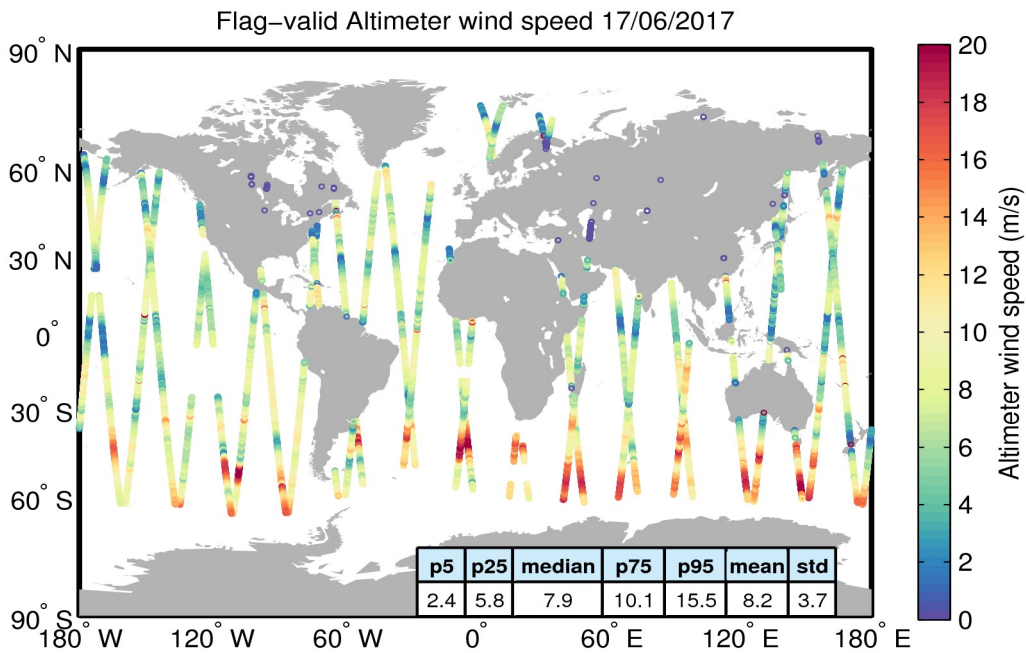
Figure 31. Geographical distribution of flag-valid wind data over oceans and lakes for 17/06/2017. The statistical values shown in the table refer to the wind in m/s and are calculated over all measurements shown in the figure.
