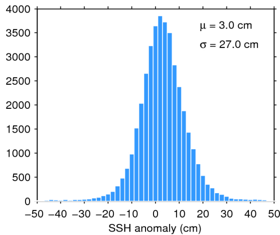
Figure 7. Histogram of flag-valid SSH anomaly over oceans and lakes for 17/06/2017. The mean ( \mu ) and standard deviation ( \sigma ) are also shown. Note that values outside [-50\ 50] cm are excluded from the histogram for the sake of readability but not from the computation of \mu and \sigma .
