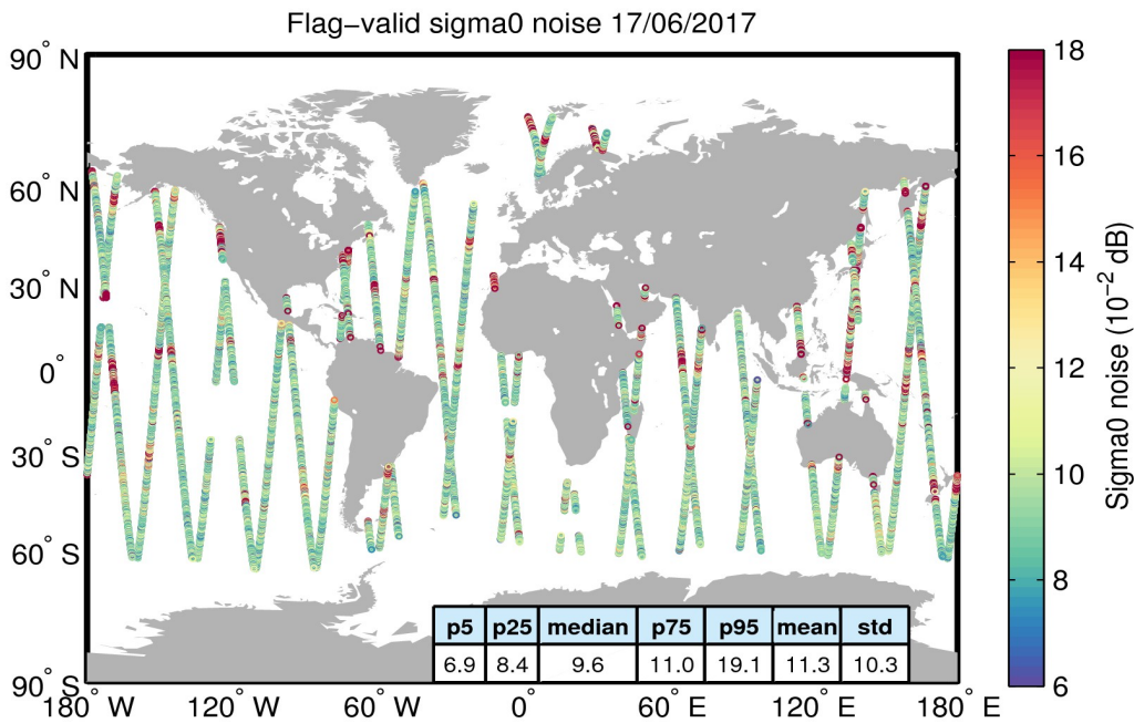
Figure 26. Geographical distribution of flag-valid 20-Hz sigma0 measurement noise over oceans and lakes for 17/06/2017. The statistical values shown in the table refer to the sigma0 noise and are calculated over all measurements shown in the figure.
