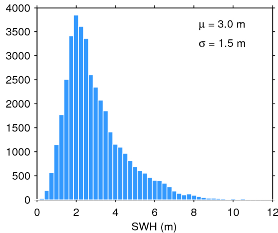
Figure 20. Histogram of science-valid SWH over oceans and lakes for 17/06/2017. The mean ( \mu ) and standard deviation ( \sigma ) are also shown. Note that values larger than 12 m are excluded from the histogram for the sake of readability but not from the computation of \mu and \sigma .
