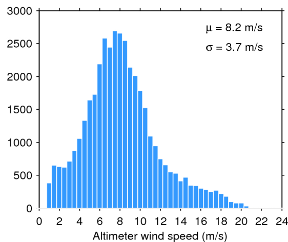
Figure 35. Histogram of science-valid wind over oceans and lakes for 17/06/2017. The mean ( \mu ) and standard deviation ( \sigma ) are also shown. Note that values larger than 24 m/s are excluded from the histogram for the sake of readability but not from the computation of \mu and \sigma .
