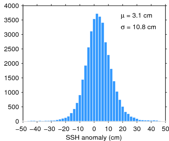
Figure 11. Histogram of science-valid SSH anomaly over oceans and lakes for 17/06/2017. The mean ( \mu ) and standard deviation ( \sigma ) are also shown. Note that values outside [-50 50] cm are excluded from the histogram for the sake of readability but not from the computation of \mu and \sigma .
