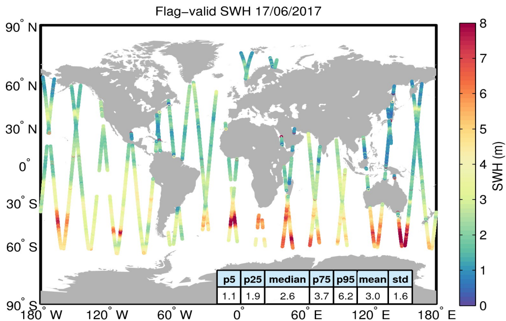
Figure 15. Geographical distribution of flag-valid SWH data over oceans and lakes for 17/06/2017. The statistical values shown in the table refer to the SWH in m and are calculated over all measurements shown in the figure.
