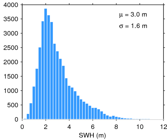
Figure 17. Histogram of flag-valid SWH over oceans and lakes for 17/06/2017. The mean ( \mu ) and standard deviation ( \sigma ) are also shown. Note that values larger than 12 m are excluded from the histogram for the sake of readability but not from the computation of \mu and \sigma .
