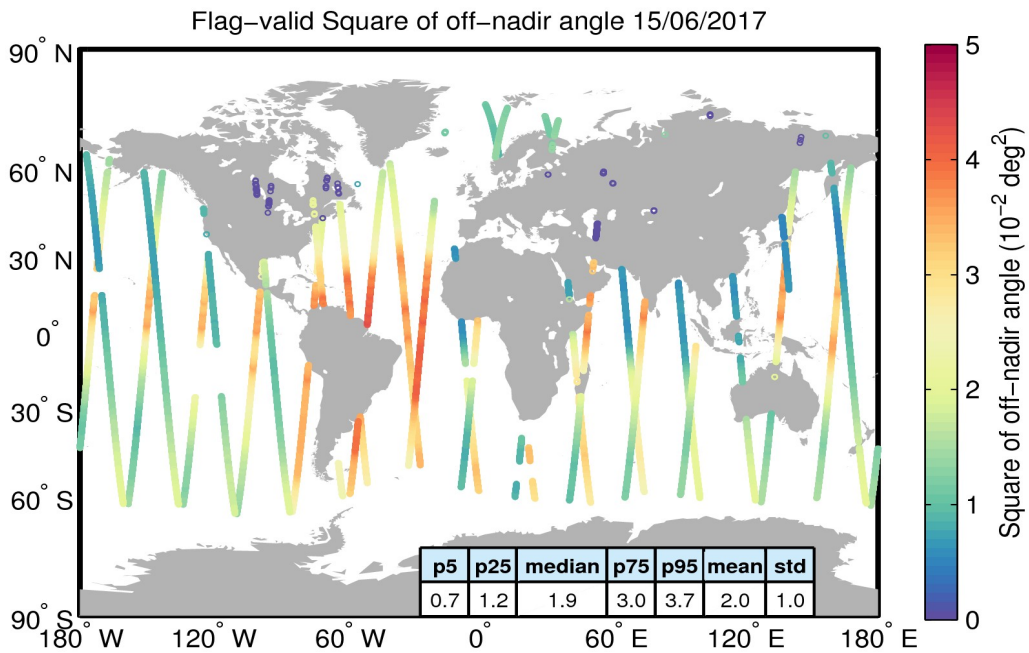
Figure 37. Geographical distribution of flag-valid mispointing data over oceans and lakes for 15/06/2017. The statistical values shown in the table refer to the mispointing in 10^{-2} \text{ deg}^2 and are calculated over all measurements shown in the figure.
