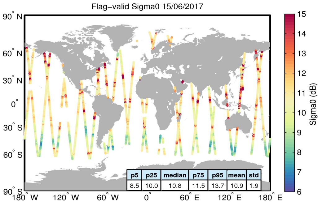
Figure 23. Geographical distribution of flag-valid sigma0 data over oceans and lakes for 15/06/2017. The statistical values shown in the table refer to the sigma0 in dB and are calculated over all measurements shown in the figure.
