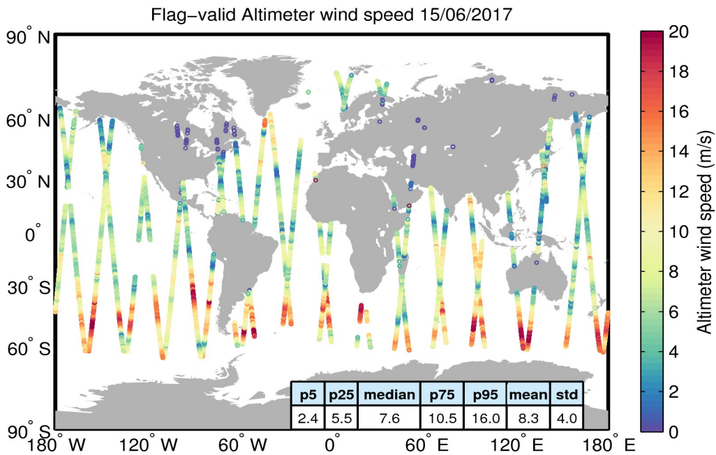
Figure 31. Geographical distribution of flag-valid wind data over oceans and lakes for 15/06/2017. The statistical values shown in the table refer to the wind in m/s and are calculated over all measurements shown in the figure.
