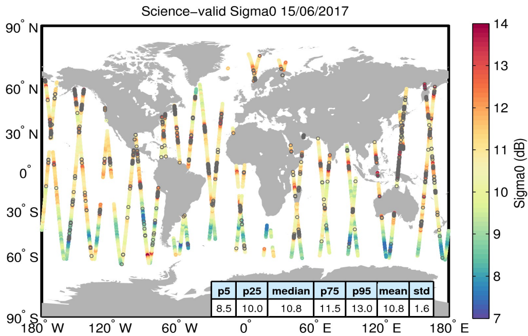
Figure 27. Geographical distribution of science-valid sigma0 data over oceans and lakes for 15/06/2017. The statistical values shown in the table refer to the sigma0 in dB and are calculated over all measurements shown in the figure. Gray circles denote records that have been rejected based on the editing criteria described in Table 4.
