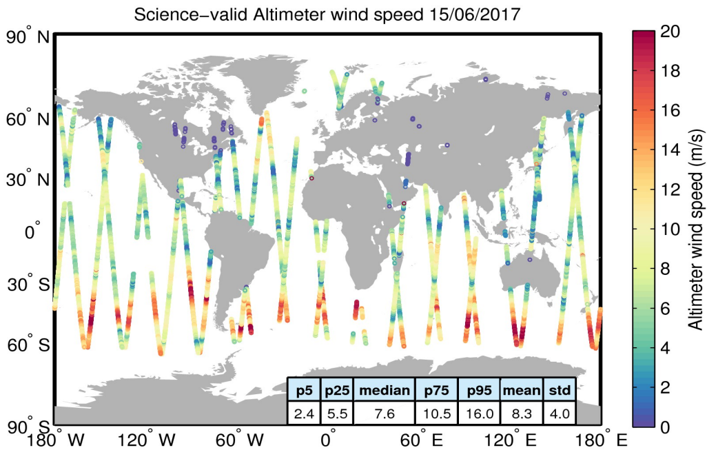
Figure 34. Geographical distribution of science-valid wind data over oceans and lakes for 15/06/2017. The statistical values shown in the table refer to the wind in m/s and are calculated over all measurements shown in the figure. Gray circles denote records that have been rejected based on the editing criteria described in Table 5.
