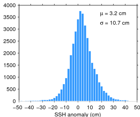
Figure 11. Histogram of science-valid SSH anomaly over oceans and lakes for 15/06/2017. The mean ( \mu ) and standard deviation ( \sigma ) are also shown. Note that values outside [-50 50] cm are excluded from the histogram for the sake of readability but not from the computation of \mu and \sigma .
