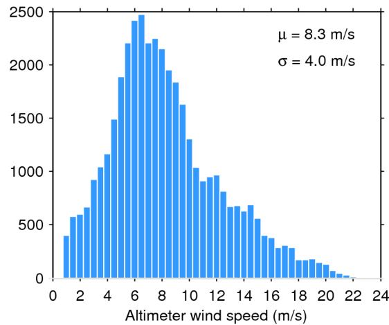
Figure 33. Histogram of flag-valid wind over oceans and lakes for 15/06/2017. The mean ( \mu ) and standard deviation ( \sigma ) are also shown. Note that values larger than 24 m/s are excluded from the histogram for the sake of readability but not from the computation of \mu and \sigma .
