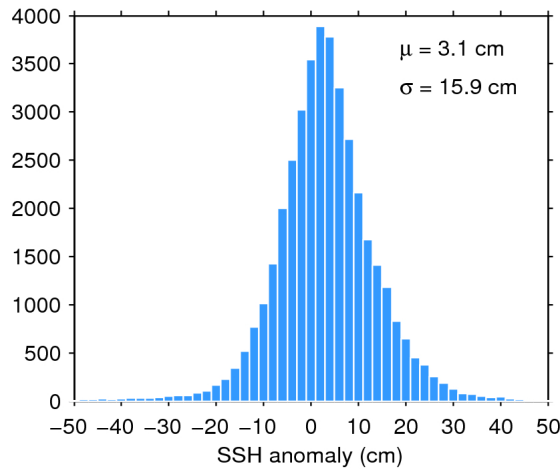
Figure 7. Histogram of flag-valid SSH anomaly over oceans and lakes for 15/06/2017. The mean ( \mu ) and standard deviation ( \sigma ) are also shown. Note that values outside [-50 50] cm are excluded from the histogram for the sake of readability but not from the computation of \mu and \sigma .
