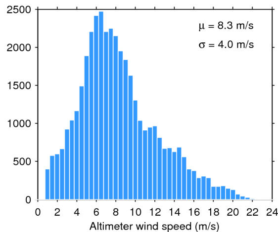
Figure 35. Histogram of science-valid wind over oceans and lakes for 15/06/2017. The mean ( \mu ) and standard deviation ( \sigma ) are also shown. Note that values larger than 24 m/s are excluded from the histogram for the sake of readability but not from the computation of \mu and \sigma .
