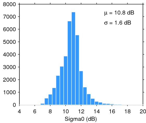
Figure 28. Histogram of science-valid sigma0 over oceans and lakes for 15/06/2017. The mean ( \mu ) and standard deviation ( \sigma ) are also shown. Note that values outside [4 20] dB are excluded from the histogram for the sake of readability but not from the computation of \mu and \sigma .
