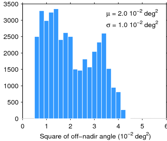
Figure 39. Histogram of flag-valid mispointing over oceans and lakes for 15/06/2017. The mean ( \mu ) and standard deviation ( \sigma ) are also shown. Note that values larger than 6 \cdot 10^{-2} \text{ deg}^2 are excluded from the histogram for the sake of readability but not from the computation of \mu and \sigma .
