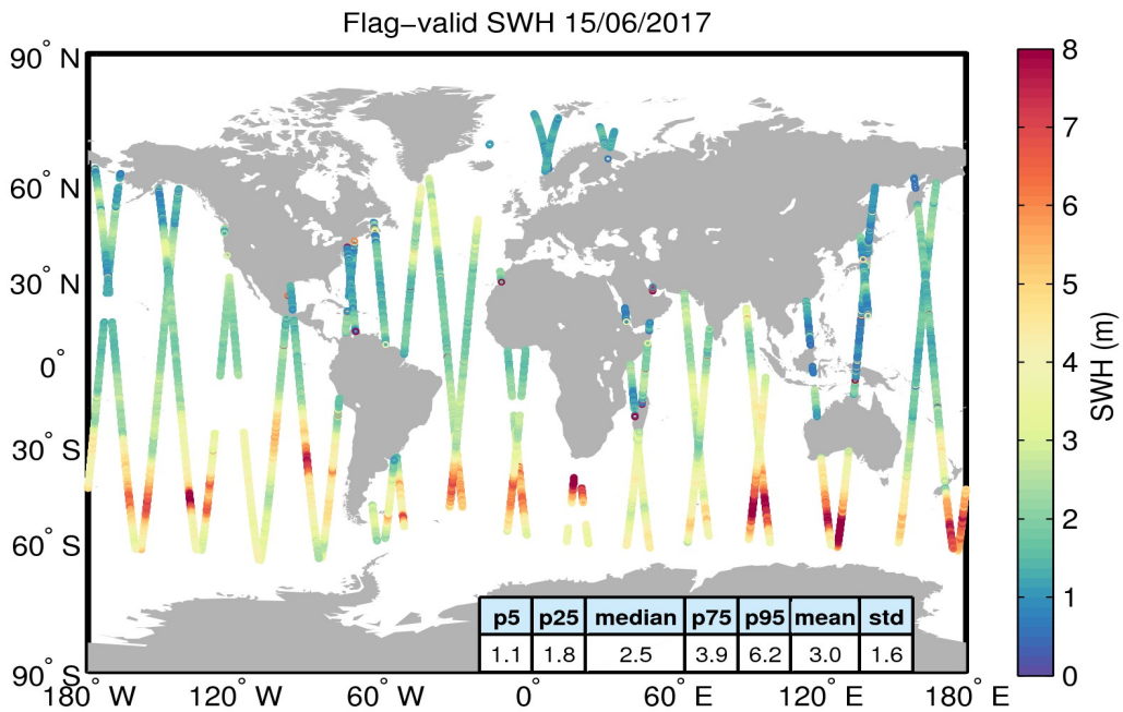
Figure 15. Geographical distribution of flag-valid SWH data over oceans and lakes for 15/06/2017. The statistical values shown in the table refer to the SWH in m and are calculated over all measurements shown in the figure.
