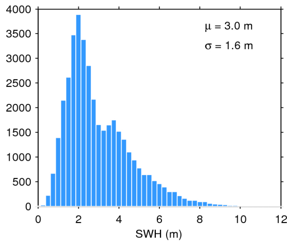
Figure 17. Histogram of flag-valid SWH over oceans and lakes for 15/06/2017. The mean ( \mu ) and standard deviation ( \sigma ) are also shown. Note that values larger than 12 m are excluded from the histogram for the sake of readability but not from the computation of \mu and \sigma .
