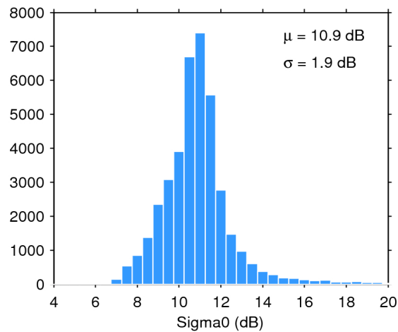
Figure 25. Histogram of flag-valid sigma0 over oceans and lakes for 15/06/2017. The mean ( \mu ) and standard deviation ( \sigma ) are also shown. Note that values outside [4 20] dB are excluded from the histogram for the sake of readability but not from the computation of \mu and \sigma .
