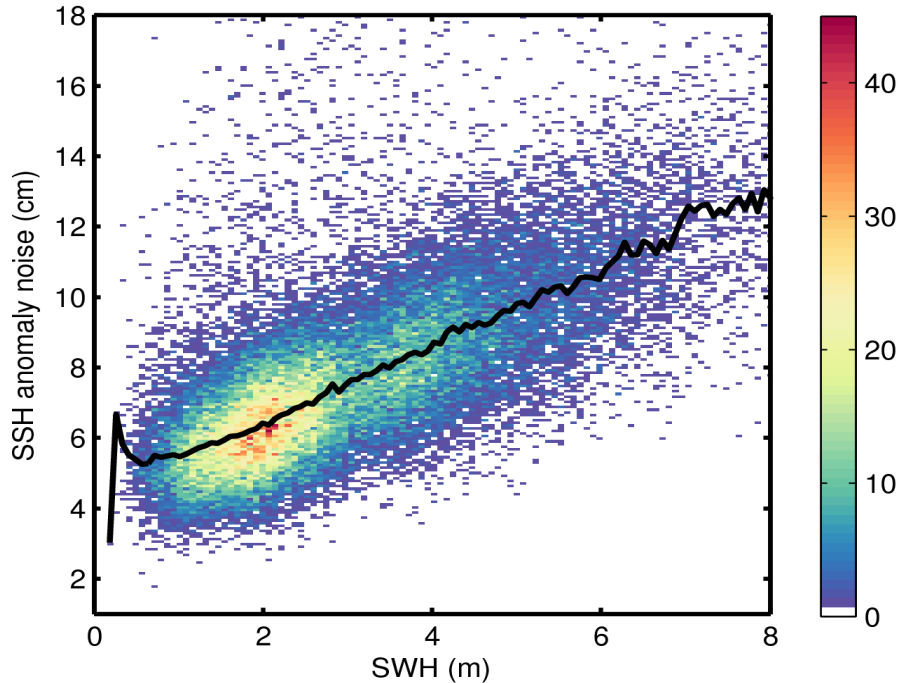
Figure 9. 2D histogram showing flag-valid SSH anomaly noise as a function of SWH for 15/06/2017. The black line denotes the median SSH anomaly noise as a function of SWH.
