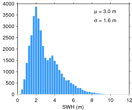
Figure 20. Histogram of science-valid SWH over oceans and lakes for 15/06/2017. The mean ( \mu ) and standard deviation ( \sigma ) are also shown. Note that values larger than 12 m are excluded from the histogram for the sake of readability but not from the computation of \mu and \sigma .
