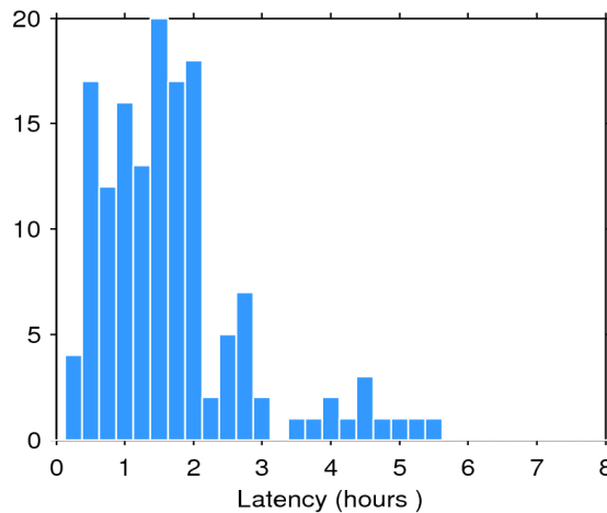
Figure 2. Histogram of the data latency for 15/06/2017. The y-axis denotes the number of files that are made available with a delay of x-hours with respect to the mean time of the records stored in the file.
