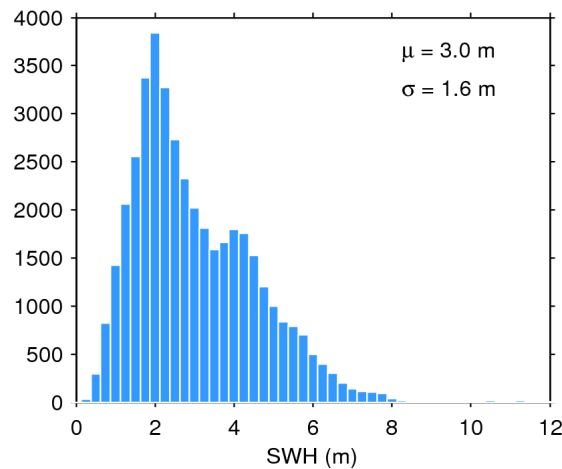
Figure 17. Histogram of flag-valid SWH over oceans and lakes for 14/06/2017. The mean ( \mu ) and standard deviation ( \sigma ) are also shown. Note that values larger than 12 m are excluded from the histogram for the sake of readability but not from the computation of \mu and \sigma .
