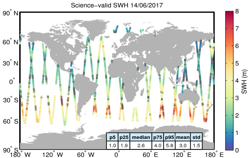
Figure 19. Geographical distribution of science-valid SWH data over oceans and lakes for 14/06/2017. The statistical values shown in the table refer to the SWH in m and are calculated over all measurements shown in the figure. Gray circles denote records that have been rejected based on the editing criteria described in Table 3.
