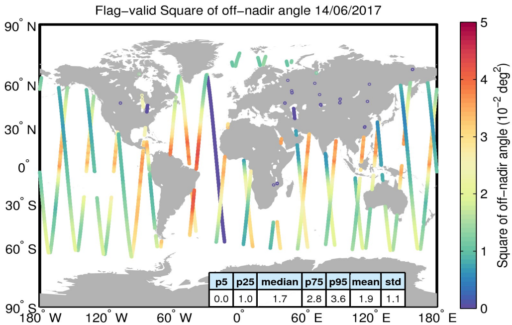
Figure 37. Geographical distribution of flag-valid mispointing data over oceans and lakes for 14/06/2017. The statistical values shown in the table refer to the mispointing in 10^{-2} \text{ deg}^2 and are calculated over all measurements shown in the figure.
