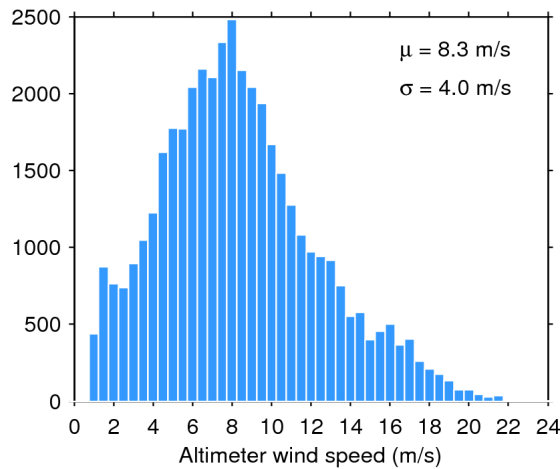
Figure 33. Histogram of flag-valid wind over oceans and lakes for 14/06/2017. The mean ( \mu ) and standard deviation ( \sigma ) are also shown. Note that values larger than 24 m/s are excluded from the histogram for the sake of readability but not from the computation of \mu and \sigma .
