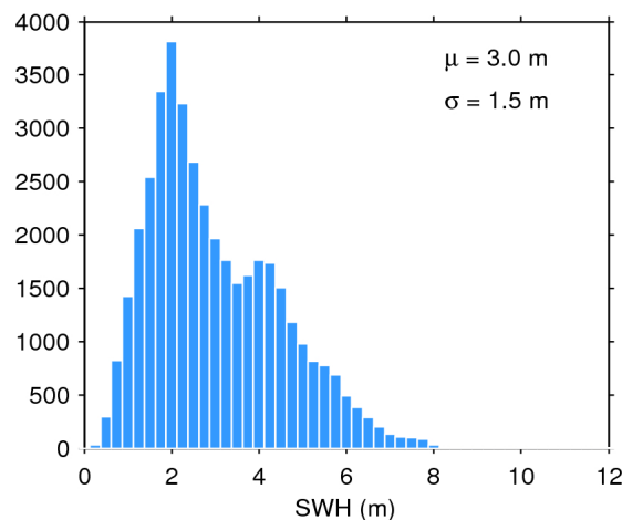
Figure 20. Histogram of science-valid SWH over oceans and lakes for 14/06/2017. The mean ( \mu ) and standard deviation ( \sigma ) are also shown. Note that values larger than 12 m are excluded from the histogram for the sake of readability but not from the computation of \mu and \sigma .
