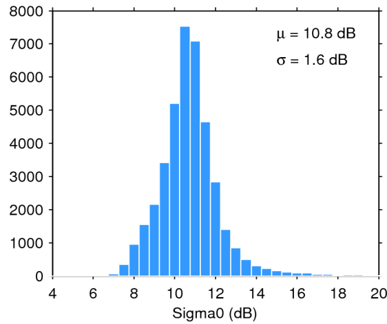
Figure 28. Histogram of science-valid sigma0 over oceans and lakes for 14/06/2017. The mean ( \mu ) and standard deviation ( \sigma ) are also shown. Note that values outside [4 20] dB are excluded from the histogram for the sake of readability but not from the computation of \mu and \sigma .
