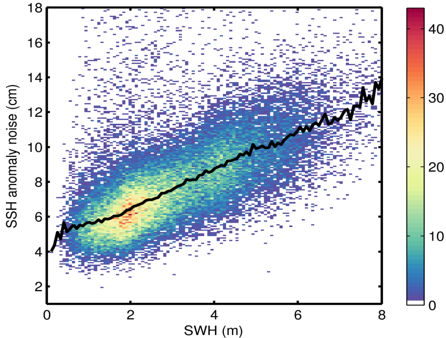
Figure 9. 2D histogram showing flag-valid SSH anomaly noise as a function of SWH for 14/06/2017. The black line denotes the median SSH anomaly noise as a function of SWH.
