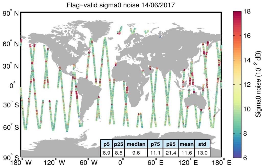
Figure 26. Geographical distribution of flag-valid 20-Hz sigma0 measurement noise over oceans and lakes for 14/06/2017. The statistical values shown in the table refer to the sigma0 noise and are calculated over all measurements shown in the figure.
