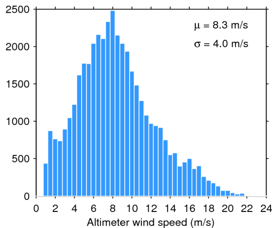
Figure 35. Histogram of science-valid wind over oceans and lakes for 14/06/2017. The mean ( \mu ) and standard deviation ( \sigma ) are also shown. Note that values larger than 24 m/s are excluded from the histogram for the sake of readability but not from the computation of \mu and \sigma .
