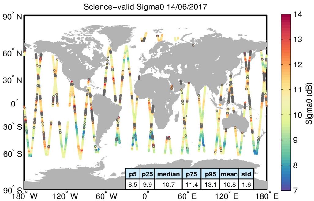
Figure 27. Geographical distribution of science-valid sigma0 data over oceans and lakes for 14/06/2017. The statistical values shown in the table refer to the sigma0 in dB and are calculated over all measurements shown in the figure. Gray circles denote records that have been rejected based on the editing criteria described in Table 4.
