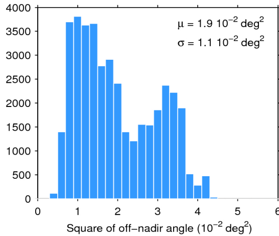
Figure 39. Histogram of flag-valid mispointing over oceans and lakes for 14/06/2017. The mean ( \mu ) and standard deviation ( \sigma ) are also shown. Note that values larger than 6 \cdot 10^{-2} \text{ deg}^2 are excluded from the histogram for the sake of readability but not from the computation of \mu and \sigma .
