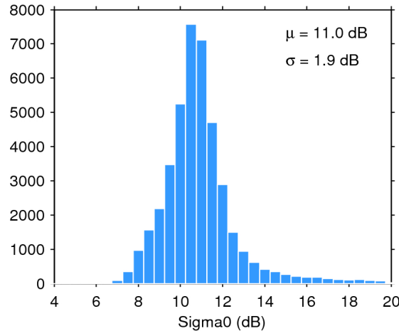
Figure 25. Histogram of flag-valid sigma0 over oceans and lakes for 14/06/2017. The mean ( \mu ) and standard deviation ( \sigma ) are also shown. Note that values outside [4 20] dB are excluded from the histogram for the sake of readability but not from the computation of \mu and \sigma .
