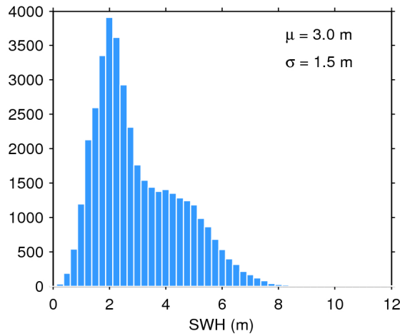
Figure 17. Histogram of flag-valid SWH over oceans and lakes for 13/06/2017. The mean ( \mu ) and standard deviation ( \sigma ) are also shown. Note that values larger than 12 m are excluded from the histogram for the sake of readability but not from the computation of \mu and \sigma .
