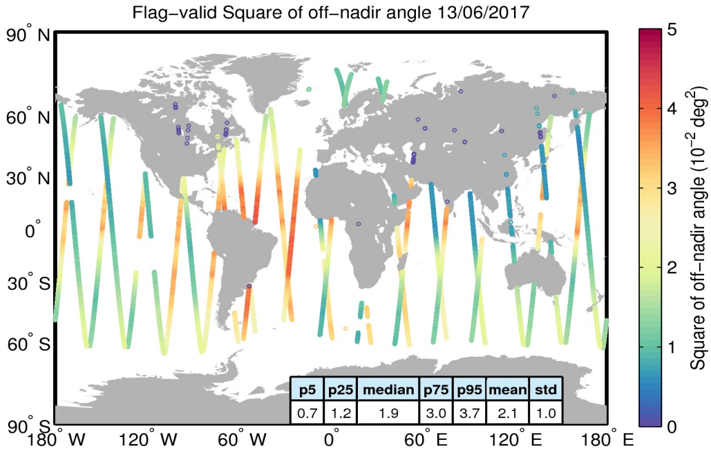
Figure 37. Geographical distribution of flag-valid mispointing data over oceans and lakes for 13/06/2017. The statistical values shown in the table refer to the mispointing in 10^{-2} deg 2 and are calculated over all measurements shown in the figure.
