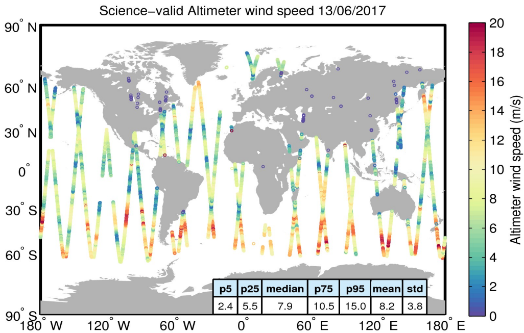
Figure 34. Geographical distribution of science-valid wind data over oceans and lakes for 13/06/2017. The statistical values shown in the table refer to the wind in m/s and are calculated over all measurements shown in the figure. Gray circles denote records that have been rejected based on the editing criteria described in Table 5.
