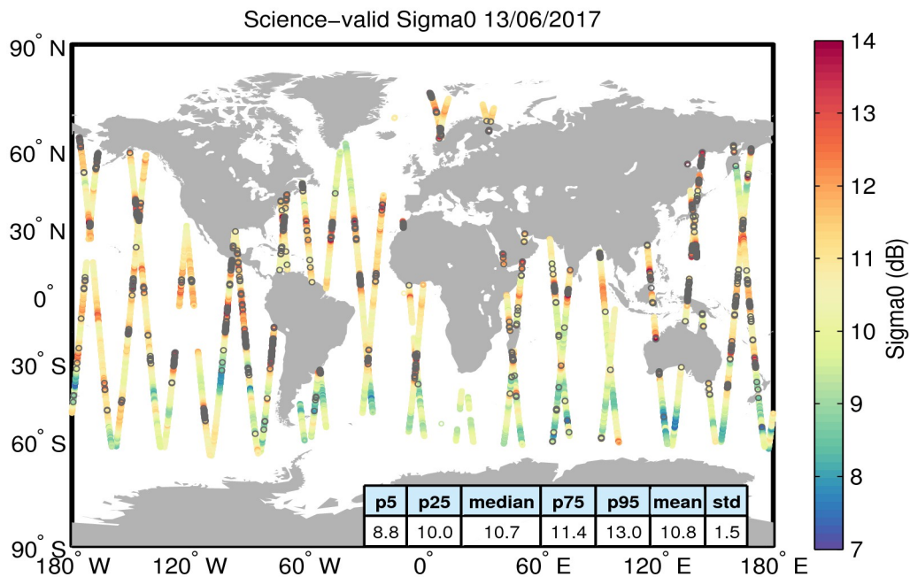
Figure 27. Geographical distribution of science-valid sigma0 data over oceans and lakes for 13/06/2017. The statistical values shown in the table refer to the sigma0 in dB and are calculated over all measurements shown in the figure. Gray circles denote records that have been rejected based on the editing criteria described in Table 4.
