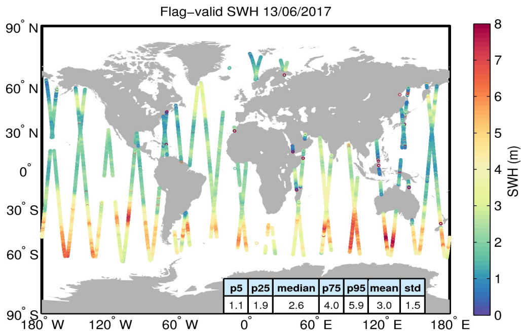
Figure 15. Geographical distribution of flag-valid SWH data over oceans and lakes for 13/06/2017. The statistical values shown in the table refer to the SWH in m and are calculated over all measurements shown in the figure.
