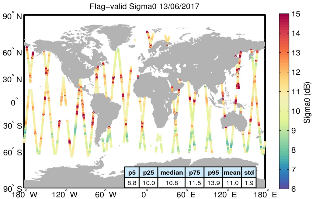
Figure 23. Geographical distribution of flag-valid sigma0 data over oceans and lakes for 13/06/2017. The statistical values shown in the table refer to the sigma0 in dB and are calculated over all measurements shown in the figure.
