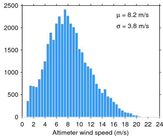
Figure 35. Histogram of science-valid wind over oceans and lakes for 13/06/2017. The mean ( \mu ) and standard deviation ( \sigma ) are also shown. Note that values larger than 24 m/s are excluded from the histogram for the sake of readability but not from the computation of \mu and \sigma .
