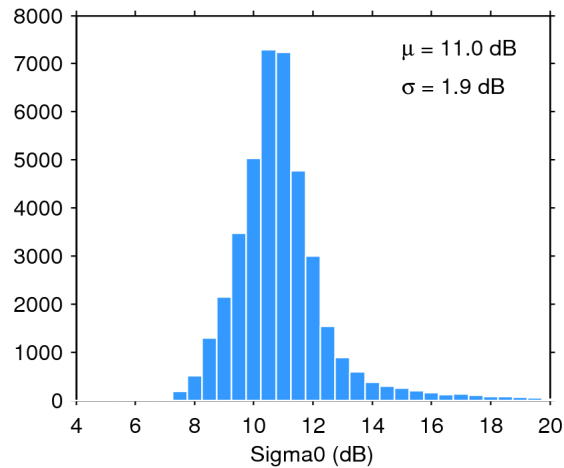
Figure 25. Histogram of flag-valid sigma0 over oceans and lakes for 13/06/2017. The mean ( \mu ) and standard deviation ( \sigma ) are also shown. Note that values outside [4 20] dB are excluded from the histogram for the sake of readability but not from the computation of \mu and \sigma .
