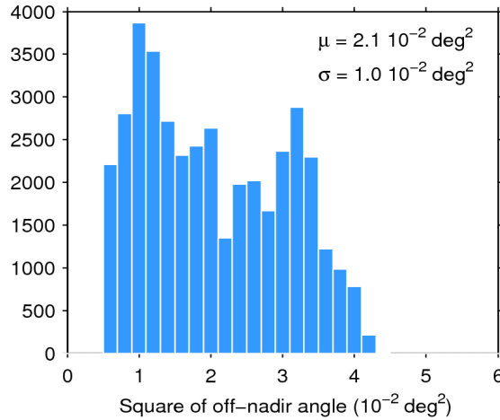
Figure 39. Histogram of flag-valid mispointing over oceans and lakes for 13/06/2017. The mean ( \mu ) and standard deviation ( \sigma ) are also shown. Note that values larger than 6 \cdot 10^{-2} \text{ deg}^2 are excluded from the histogram for the sake of readability but not from the computation of \mu and \sigma .
