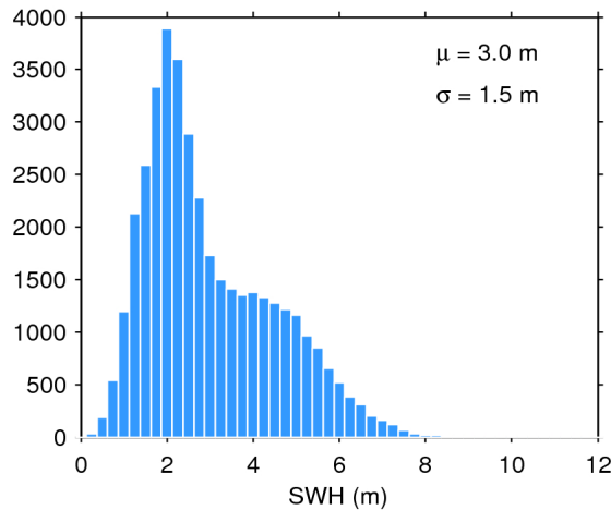
Figure 20. Histogram of science-valid SWH over oceans and lakes for 13/06/2017. The mean ( \mu ) and standard deviation ( \sigma ) are also shown. Note that values larger than 12 m are excluded from the histogram for the sake of readability but not from the computation of \mu and \sigma .
