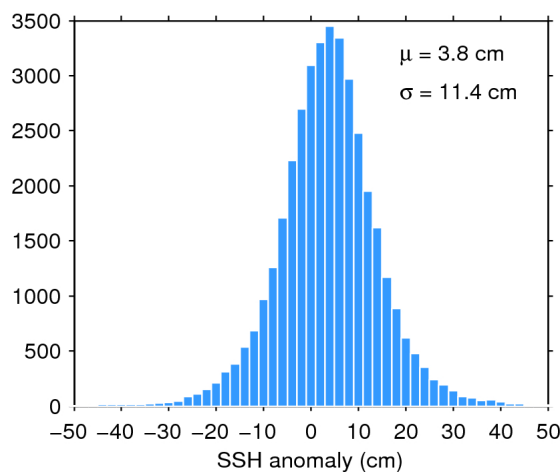
Figure 11. Histogram of science-valid SSH anomaly over oceans and lakes for 13/06/2017. The mean ( \mu ) and standard deviation ( \sigma ) are also shown. Note that values outside [-50 50] cm are excluded from the histogram for the sake of readability but not from the computation of \mu and \sigma .
