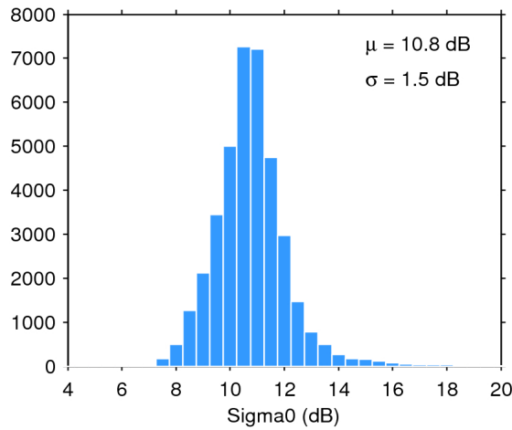
Figure 28. Histogram of science-valid sigma0 over oceans and lakes for 13/06/2017. The mean ( \mu ) and standard deviation ( \sigma ) are also shown. Note that values outside [4 20] dB are excluded from the histogram for the sake of readability but not from the computation of \mu and \sigma .
