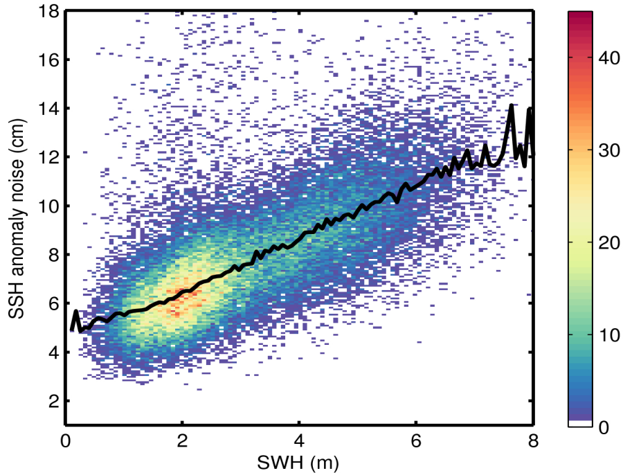
Figure 9. 2D histogram showing flag-valid SSH anomaly noise as a function of SWH for 13/06/2017. The black line denotes the median SSH anomaly noise as a function of SWH.
