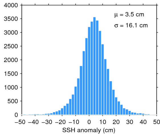
Figure 7. Histogram of flag-valid SSH anomaly over oceans and lakes for 13/06/2017. The mean ( \mu ) and standard deviation ( \sigma ) are also shown. Note that values outside [-50\ 50] cm are excluded from the histogram for the sake of readability but not from the computation of \mu and \sigma .
