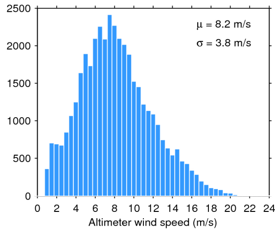
Figure 33. Histogram of flag-valid wind over oceans and lakes for 13/06/2017. The mean ( \mu ) and standard deviation ( \sigma ) are also shown. Note that values larger than 24 m/s are excluded from the histogram for the sake of readability but not from the computation of \mu and \sigma .
