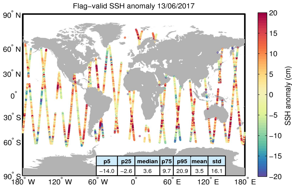
Figure 5. Geographical distribution of flag-valid 1-Hz SSH anomaly data over oceans and lakes for 13/06/2017. The statistical values shown in the table refer to the SSH anomaly in cm and are calculated over all measurements shown in the figure.
