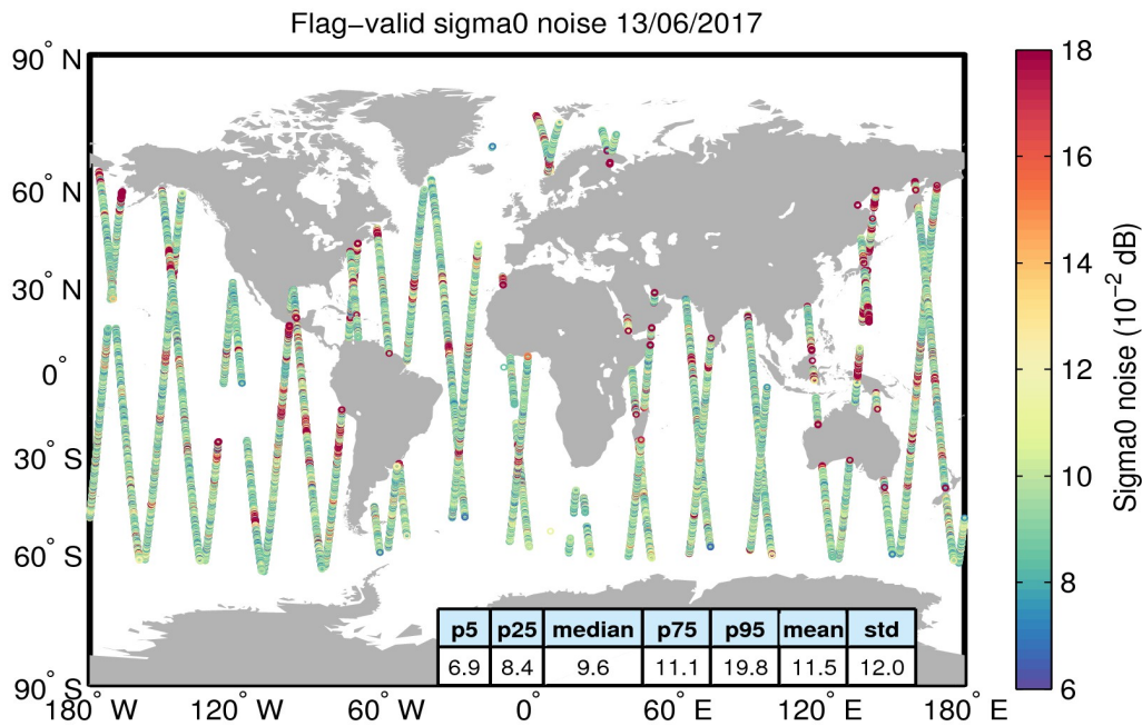
Figure 26. Geographical distribution of flag-valid 20-Hz sigma0 measurement noise over oceans and lakes for 13/06/2017. The statistical values shown in the table refer to the sigma0 noise and are calculated over all measurements shown in the figure.
