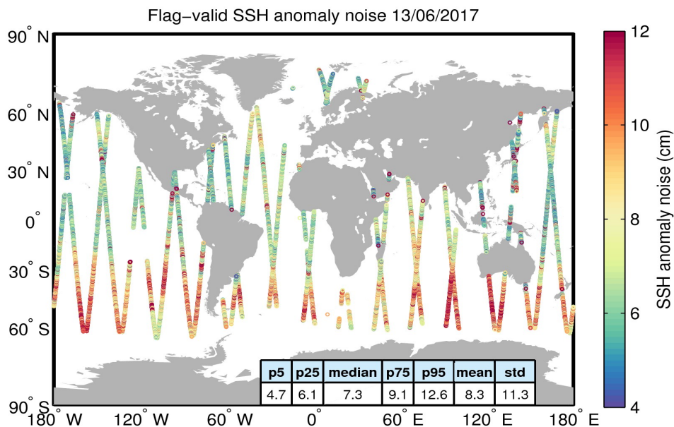
Figure 8. Geographical distribution of flag-valid 20-Hz SSH anomaly measurement noise over oceans and lakes for 13/06/2017. The statistical values shown in the table refer to the SSH anomaly noise and are calculated over all measurements shown in the figure.
