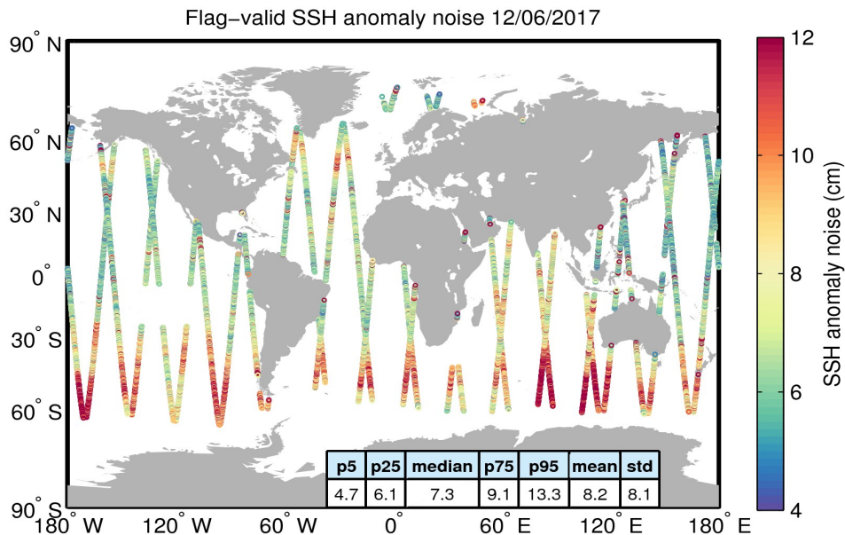
Figure 8. Geographical distribution of flag-valid 20-Hz SSH anomaly measurement noise over oceans and lakes for 12/06/2017. The statistical values shown in the table refer to the SSH anomaly noise and are calculated over all measurements shown in the figure.
