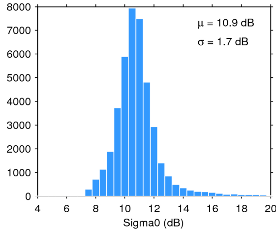
Figure 25. Histogram of flag-valid sigma0 over oceans and lakes for 12/06/2017. The mean ( \mu ) and standard deviation ( \sigma ) are also shown. Note that values outside [4 20] dB are excluded from the histogram for the sake of readability but not from the computation of \mu and \sigma .
