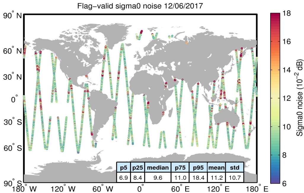
Figure 26. Geographical distribution of flag-valid 20-Hz sigma0 measurement noise over oceans and lakes for 12/06/2017. The statistical values shown in the table refer to the sigma0 noise and are calculated over all measurements shown in the figure.
