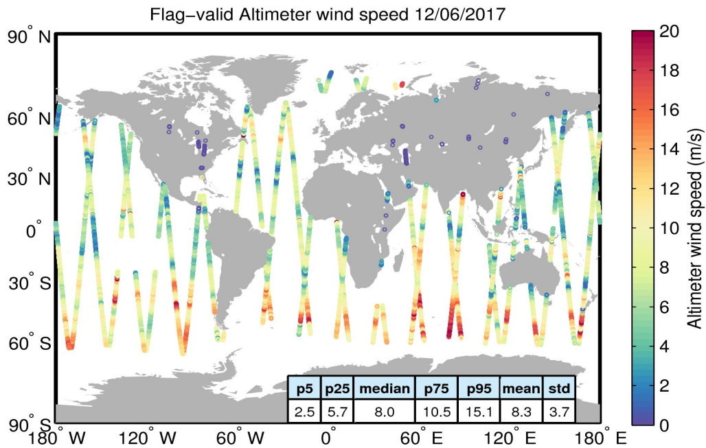
Figure 31. Geographical distribution of flag-valid wind data over oceans and lakes for 12/06/2017. The statistical values shown in the table refer to the wind in m/s and are calculated over all measurements shown in the figure.
