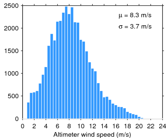
Figure 35. Histogram of science-valid wind over oceans and lakes for 12/06/2017. The mean ( \mu ) and standard deviation ( \sigma ) are also shown. Note that values larger than 24 m/s are excluded from the histogram for the sake of readability but not from the computation of \mu and \sigma .
