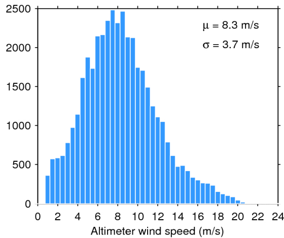
Figure 33. Histogram of flag-valid wind over oceans and lakes for 12/06/2017. The mean ( \mu ) and standard deviation ( \sigma ) are also shown. Note that values larger than 24 m/s are excluded from the histogram for the sake of readability but not from the computation of \mu and \sigma .
