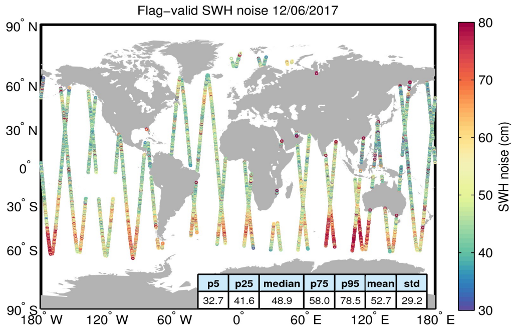
Figure 18. Geographical distribution of flag-valid 20-Hz SWH measurement noise over oceans and lakes for 12/06/2017. The statistical values shown in the table refer to the SWH noise and are calculated over all measurements shown in the figure.
