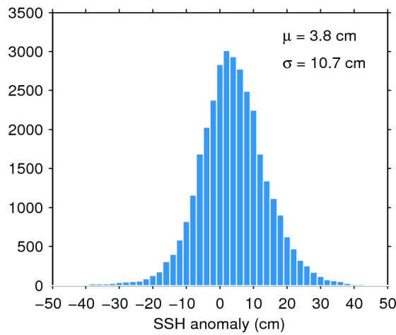
Figure 11. Histogram of science-valid SSH anomaly over oceans and lakes for 12/06/2017. The mean ( \mu ) and standard deviation ( \sigma ) are also shown. Note that values outside [-50 50] cm are excluded from the histogram for the sake of readability but not from the computation of \mu and \sigma .
