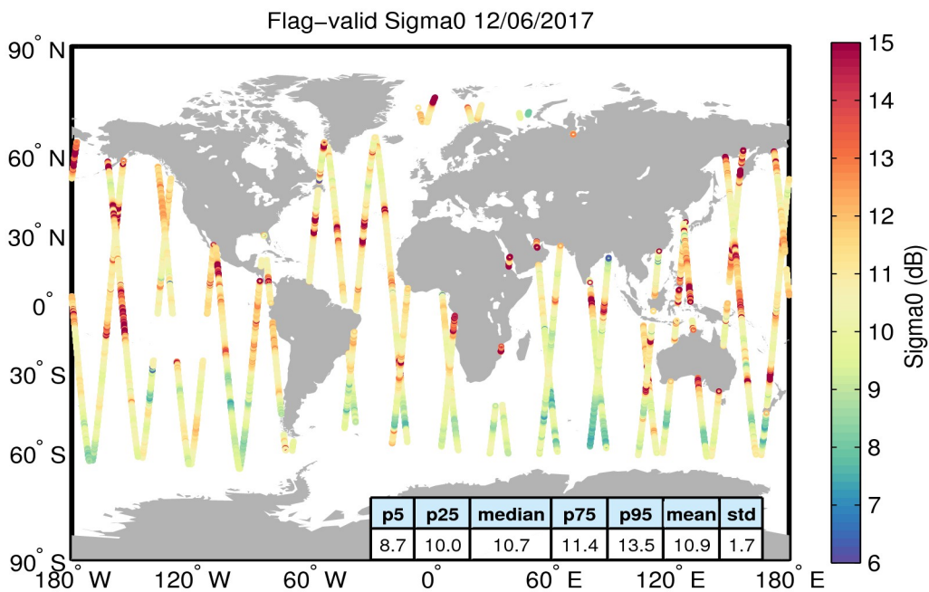
Figure 23. Geographical distribution of flag-valid sigma0 data over oceans and lakes for 12/06/2017. The statistical values shown in the table refer to the sigma0 in dB and are calculated over all measurements shown in the figure.
