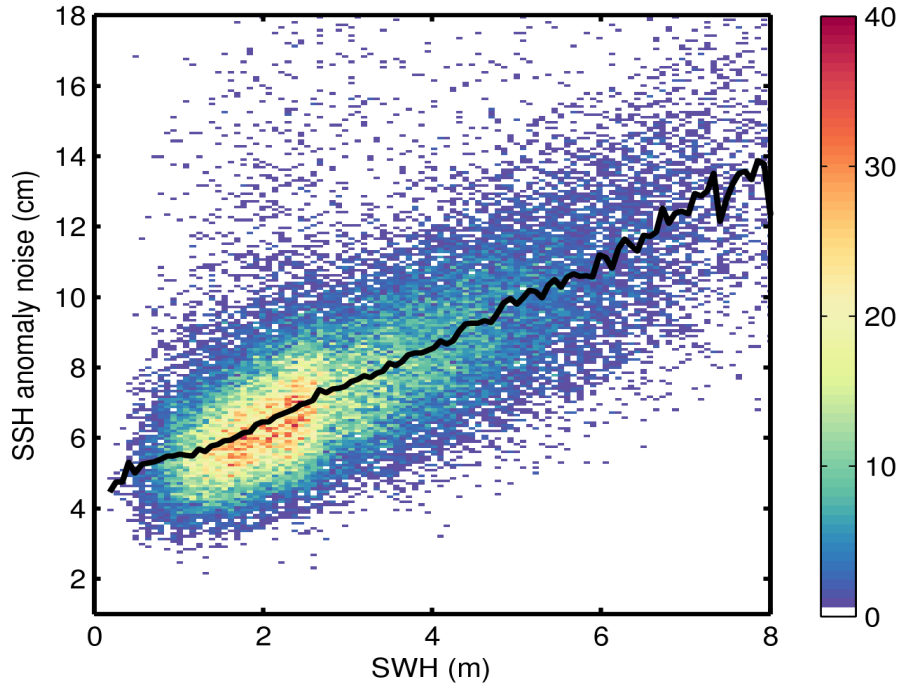
Figure 9. 2D histogram showing flag-valid SSH anomaly noise as a function of SWH for 12/06/2017. The black line denotes the median SSH anomaly noise as a function of SWH.
