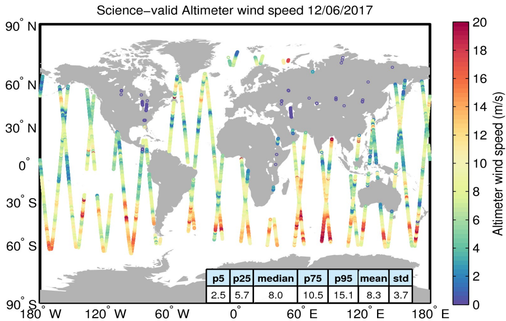
Figure 34. Geographical distribution of science-valid wind data over oceans and lakes for 12/06/2017. The statistical values shown in the table refer to the wind in m/s and are calculated over all measurements shown in the figure. Gray circles denote records that have been rejected based on the editing criteria described in Table 5.
