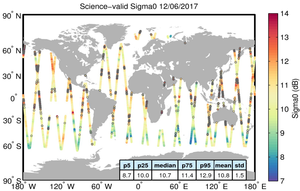
Figure 27. Geographical distribution of science-valid sigma0 data over oceans and lakes for 12/06/2017. The statistical values shown in the table refer to the sigma0 in dB and are calculated over all measurements shown in the figure. Gray circles denote records that have been rejected based on the editing criteria described in Table 4.
