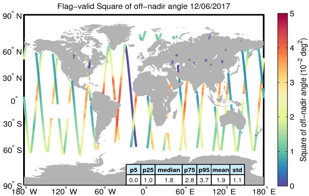
Figure 37. Geographical distribution of flag-valid mispointing data over oceans and lakes for 12/06/2017. The statistical values shown in the table refer to the mispointing in 10^{-2} deg 2 and are calculated over all measurements shown in the figure.
