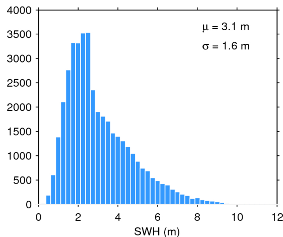
Figure 20. Histogram of science-valid SWH over oceans and lakes for 12/06/2017. The mean ( \mu ) and standard deviation ( \sigma ) are also shown. Note that values larger than 12 m are excluded from the histogram for the sake of readability but not from the computation of \mu and \sigma .
