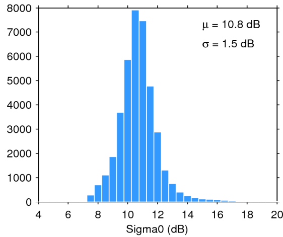
Figure 28. Histogram of science-valid sigma0 over oceans and lakes for 12/06/2017. The mean ( \mu ) and standard deviation ( \sigma ) are also shown. Note that values outside [4 20] dB are excluded from the histogram for the sake of readability but not from the computation of \mu and \sigma .
