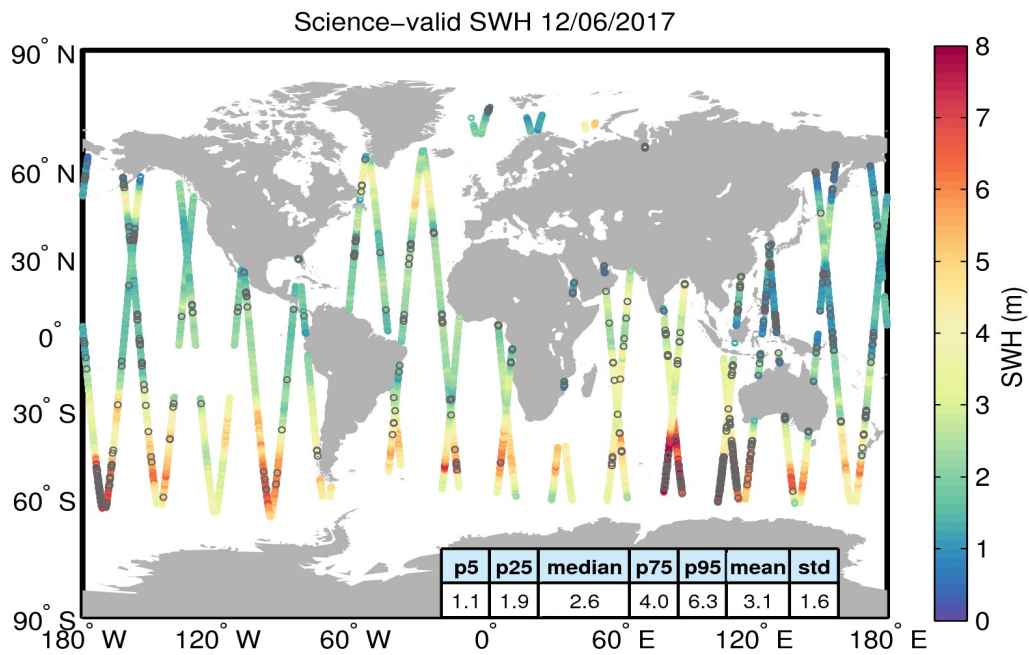
Figure 19. Geographical distribution of science-valid SWH data over oceans and lakes for 12/06/2017. The statistical values shown in the table refer to the SWH in m and are calculated over all measurements shown in the figure. Gray circles denote records that have been rejected based on the editing criteria described in Table 3.
