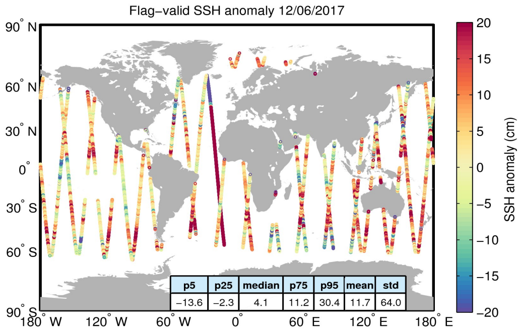
Figure 5. Geographical distribution of flag-valid 1-Hz SSH anomaly data over oceans and lakes for 12/06/2017. The statistical values shown in the table refer to the SSH anomaly in cm and are calculated over all measurements shown in the figure.
