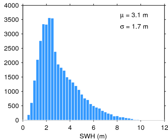
Figure 17. Histogram of flag-valid SWH over oceans and lakes for 12/06/2017. The mean ( \mu ) and standard deviation ( \sigma ) are also shown. Note that values larger than 12 m are excluded from the histogram for the sake of readability but not from the computation of \mu and \sigma .
