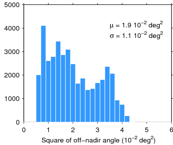
Figure 39. Histogram of flag-valid mispointing over oceans and lakes for 12/06/2017. The mean ( \mu ) and standard deviation ( \sigma ) are also shown. Note that values larger than 6 \cdot 10^{-2} \text{ deg}^2 are excluded from the histogram for the sake of readability but not from the computation of \mu and \sigma .
