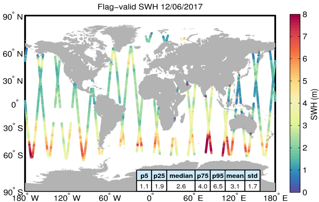
Figure 15. Geographical distribution of flag-valid SWH data over oceans and lakes for 12/06/2017. The statistical values shown in the table refer to the SWH in m and are calculated over all measurements shown in the figure.
