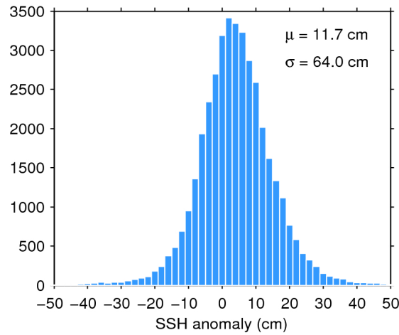
Figure 7. Histogram of flag-valid SSH anomaly over oceans and lakes for 12/06/2017. The mean ( \mu ) and standard deviation ( \sigma ) are also shown. Note that values outside [-50 50] cm are excluded from the histogram for the sake of readability but not from the computation of \mu and \sigma .
