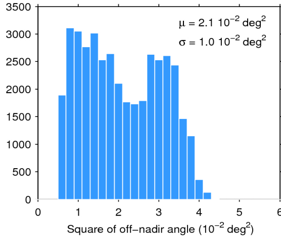
Figure 39. Histogram of flag-valid mispointing over oceans and lakes for 11/06/2017. The mean ( \mu ) and standard deviation ( \sigma ) are also shown. Note that values larger than 6 \cdot 10^{-2} \text{ deg}^2 are excluded from the histogram for the sake of readability but not from the computation of \mu and \sigma .
