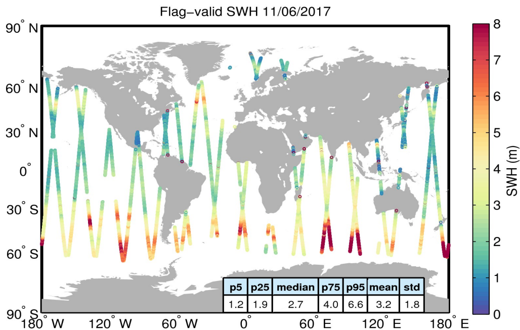
Figure 15. Geographical distribution of flag-valid SWH data over oceans and lakes for 11/06/2017. The statistical values shown in the table refer to the SWH in m and are calculated over all measurements shown in the figure.
