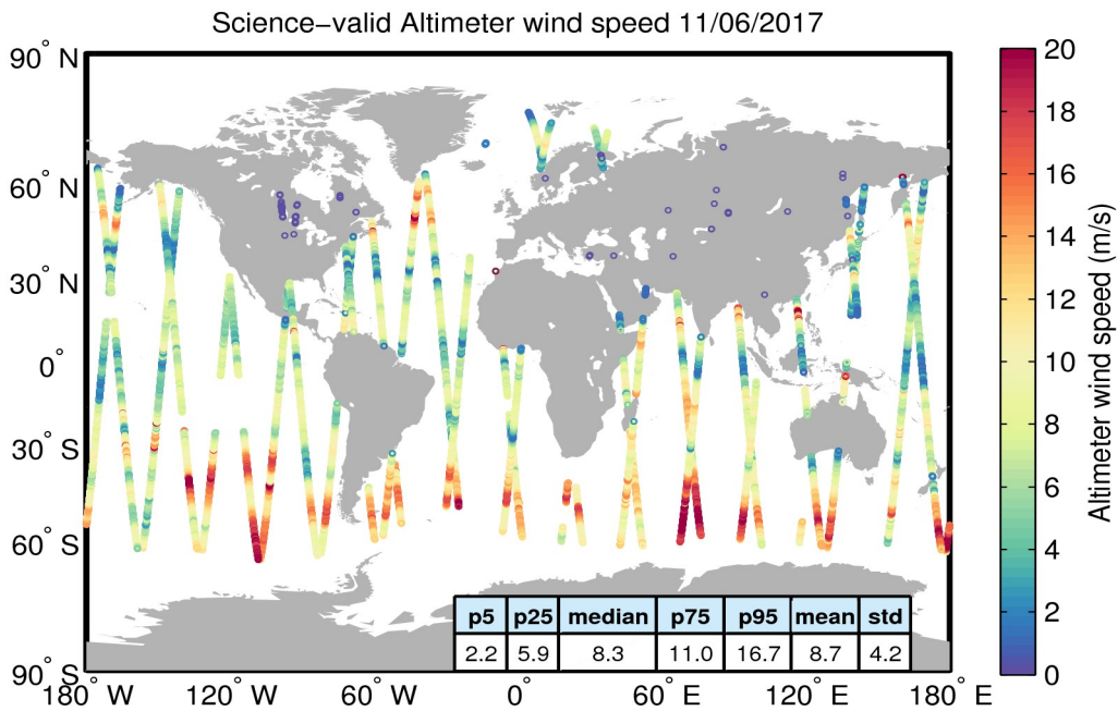
Figure 34. Geographical distribution of science-valid wind data over oceans and lakes for 11/06/2017. The statistical values shown in the table refer to the wind in m/s and are calculated over all measurements shown in the figure. Gray circles denote records that have been rejected based on the editing criteria described in Table 5.
