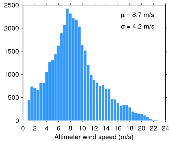
Figure 33. Histogram of flag-valid wind over oceans and lakes for 11/06/2017. The mean ( \mu ) and standard deviation ( \sigma ) are also shown. Note that values larger than 24 m/s are excluded from the histogram for the sake of readability but not from the computation of \mu and \sigma .
