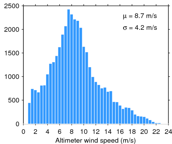
Figure 35. Histogram of science-valid wind over oceans and lakes for 11/06/2017. The mean ( \mu ) and standard deviation ( \sigma ) are also shown. Note that values larger than 24 m/s are excluded from the histogram for the sake of readability but not from the computation of \mu and \sigma .
