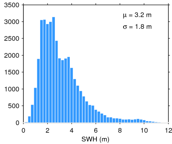
Figure 17. Histogram of flag-valid SWH over oceans and lakes for 11/06/2017. The mean ( \mu ) and standard deviation ( \sigma ) are also shown. Note that values larger than 12 m are excluded from the histogram for the sake of readability but not from the computation of \mu and \sigma .
