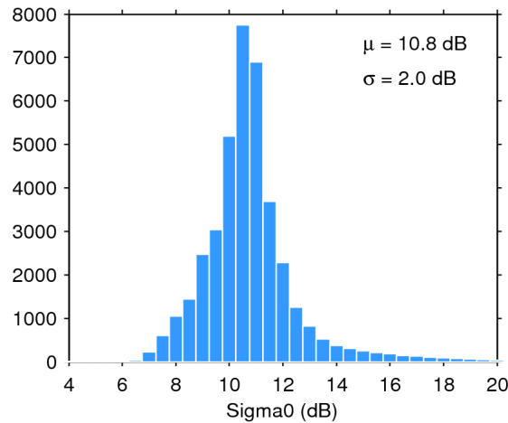
Figure 25. Histogram of flag-valid sigma0 over oceans and lakes for 11/06/2017. The mean ( \mu ) and standard deviation ( \sigma ) are also shown. Note that values outside [4 20] dB are excluded from the histogram for the sake of readability but not from the computation of \mu and \sigma .
