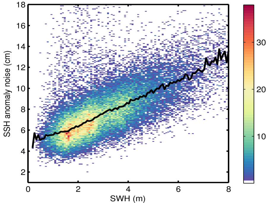
Figure 9. 2D histogram showing flag-valid SSH anomaly noise as a function of SWH for 11/06/2017. The black line denotes the median SSH anomaly noise as a function of SWH.
