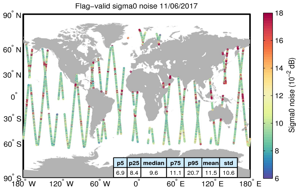
Figure 26. Geographical distribution of flag-valid 20-Hz sigma0 measurement noise over oceans and lakes for 11/06/2017. The statistical values shown in the table refer to the sigma0 noise and are calculated over all measurements shown in the figure.
