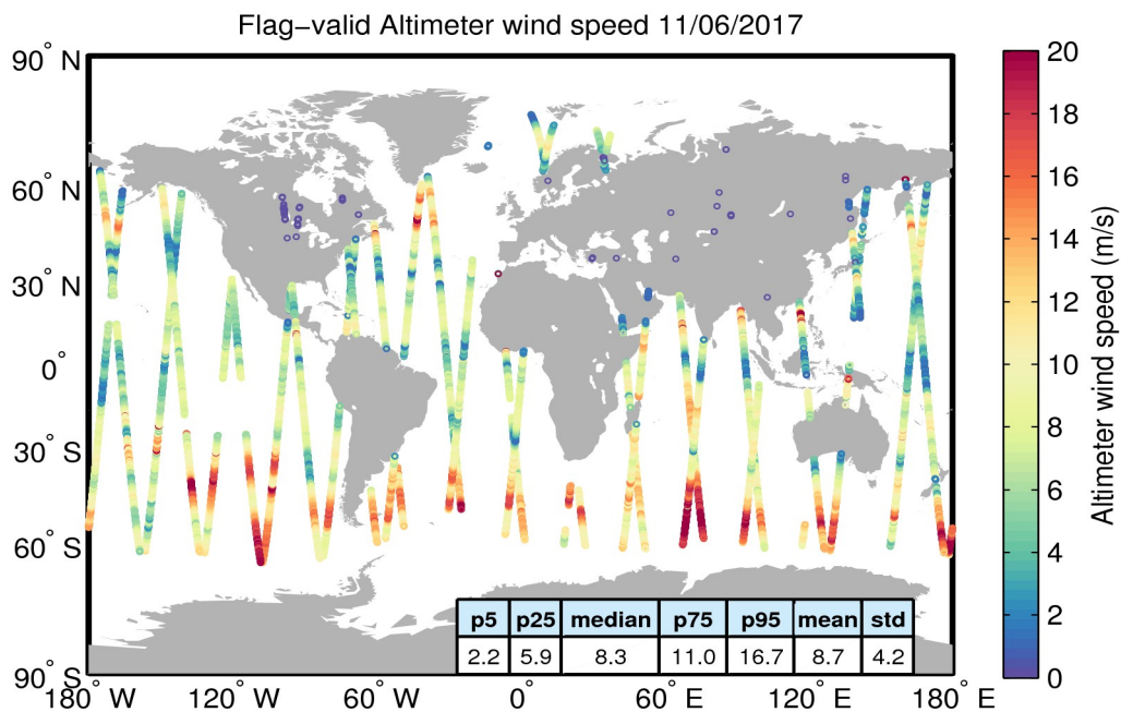
Figure 31. Geographical distribution of flag-valid wind data over oceans and lakes for 11/06/2017. The statistical values shown in the table refer to the wind in m/s and are calculated over all measurements shown in the figure.
