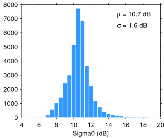
Figure 28. Histogram of science-valid sigma0 over oceans and lakes for 11/06/2017. The mean ( \mu ) and standard deviation ( \sigma ) are also shown. Note that values outside [4 20] dB are excluded from the histogram for the sake of readability but not from the computation of \mu and \sigma .
