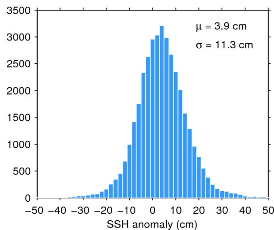
Figure 11. Histogram of science-valid SSH anomaly over oceans and lakes for 11/06/2017. The mean ( \mu ) and standard deviation ( \sigma ) are also shown. Note that values outside [-50 50] cm are excluded from the histogram for the sake of readability but not from the computation of \mu and \sigma .
