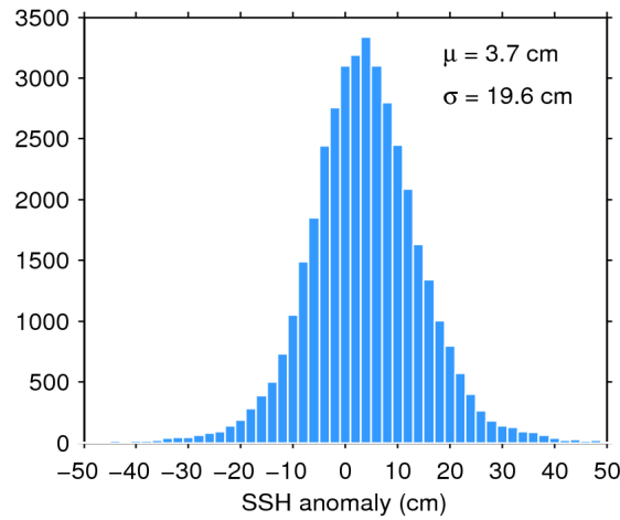
Figure 7. Histogram of flag-valid SSH anomaly over oceans and lakes for 11/06/2017. The mean ( \mu ) and standard deviation ( \sigma ) are also shown. Note that values outside [-50 50] cm are excluded from the histogram for the sake of readability but not from the computation of \mu and \sigma .
