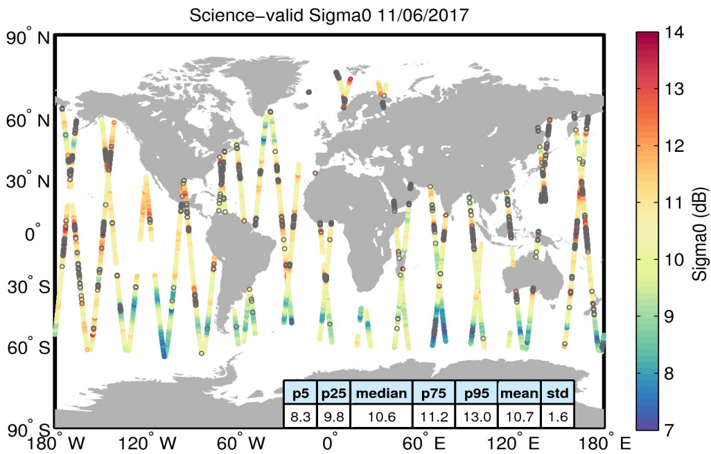
Figure 27. Geographical distribution of science-valid sigma0 data over oceans and lakes for 11/06/2017. The statistical values shown in the table refer to the sigma0 in dB and are calculated over all measurements shown in the figure. Gray circles denote records that have been rejected based on the editing criteria described in Table 4.
