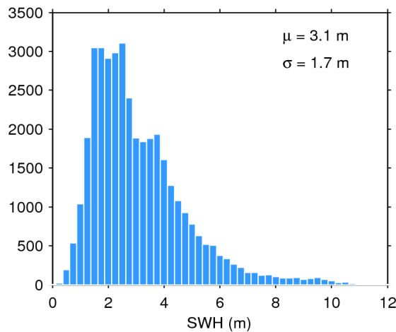
Figure 20. Histogram of science-valid SWH over oceans and lakes for 11/06/2017. The mean ( \mu ) and standard deviation ( \sigma ) are also shown. Note that values larger than 12 m are excluded from the histogram for the sake of readability but not from the computation of \mu and \sigma .
