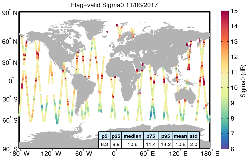
Figure 23. Geographical distribution of flag-valid sigma0 data over oceans and lakes for 11/06/2017. The statistical values shown in the table refer to the sigma0 in dB and are calculated over all measurements shown in the figure.
