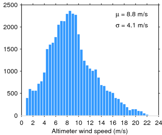
Figure 33. Histogram of flag-valid wind over oceans and lakes for 10/06/2017. The mean ( \mu ) and standard deviation ( \sigma ) are also shown. Note that values larger than 24 m/s are excluded from the histogram for the sake of readability but not from the computation of \mu and \sigma .
