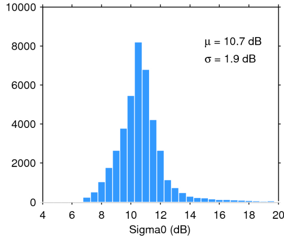
Figure 25. Histogram of flag-valid sigma0 over oceans and lakes for 10/06/2017. The mean ( \mu ) and standard deviation ( \sigma ) are also shown. Note that values outside [4 20] dB are excluded from the histogram for the sake of readability but not from the computation of \mu and \sigma .
