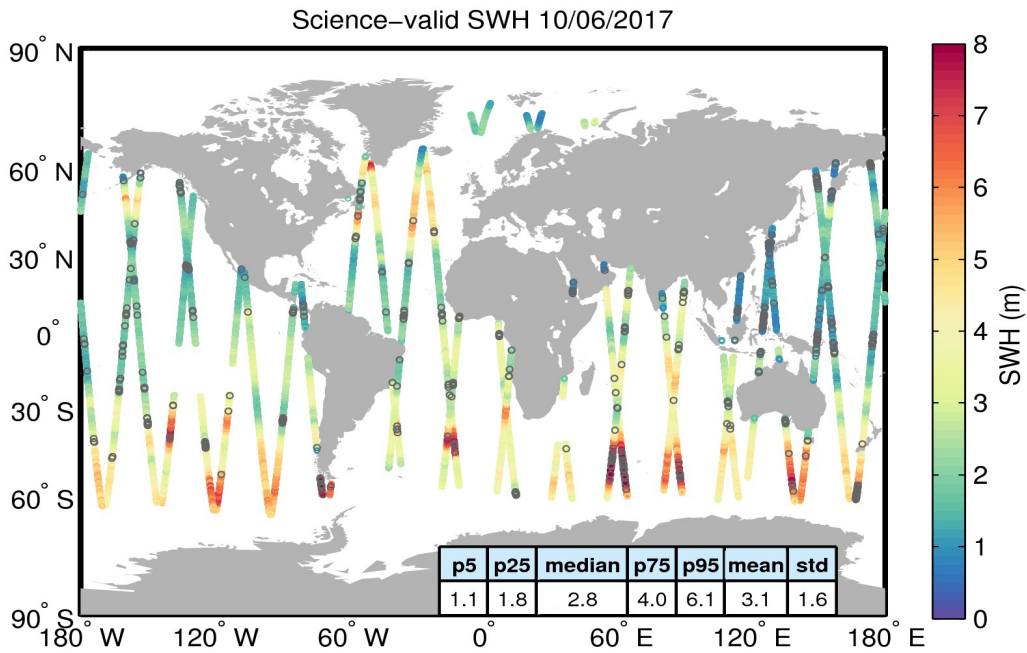
Figure 19. Geographical distribution of science-valid SWH data over oceans and lakes for 10/06/2017. The statistical values shown in the table refer to the SWH in m and are calculated over all measurements shown in the figure. Gray circles denote records that have been rejected based on the editing criteria described in Table 3.
