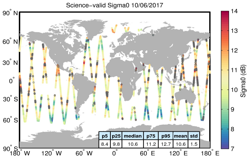
Figure 27. Geographical distribution of science-valid sigma0 data over oceans and lakes for 10/06/2017. The statistical values shown in the table refer to the sigma0 in dB and are calculated over all measurements shown in the figure. Gray circles denote records that have been rejected based on the editing criteria described in Table 4.
