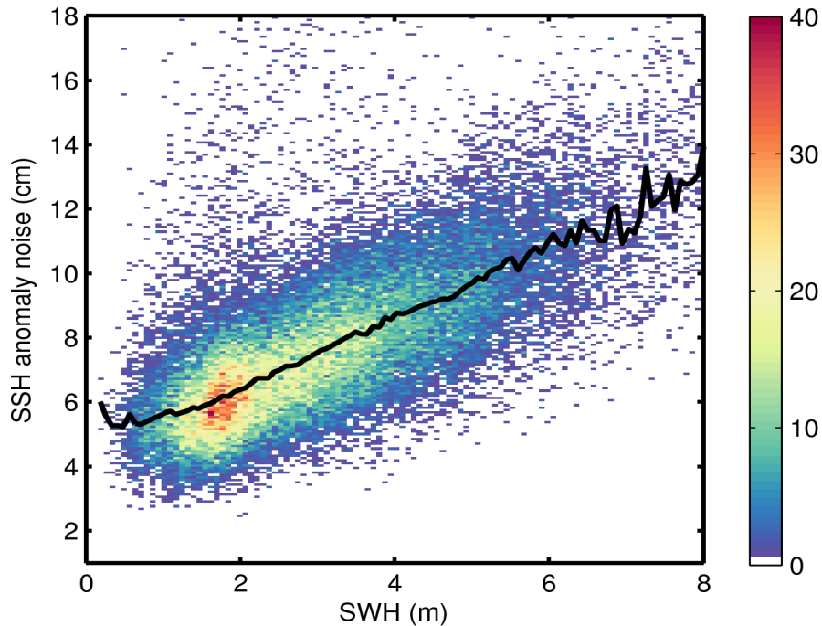
Figure 9. 2D histogram showing flag-valid SSH anomaly noise as a function of SWH for 10/06/2017. The black line denotes the median SSH anomaly noise as a function of SWH.
