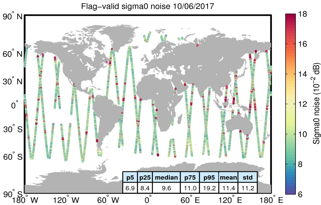
Figure 26. Geographical distribution of flag-valid 20-Hz sigma0 measurement noise over oceans and lakes for 10/06/2017. The statistical values shown in the table refer to the sigma0 noise and are calculated over all measurements shown in the figure.
