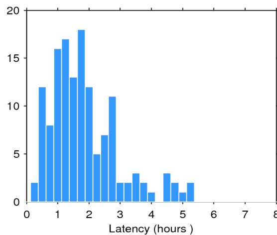
Figure 2. Histogram of the data latency for 10/06/2017. The y-axis denotes the number of files that are made available with a delay of x-hours with respect to the mean time of the records stored in the file.
