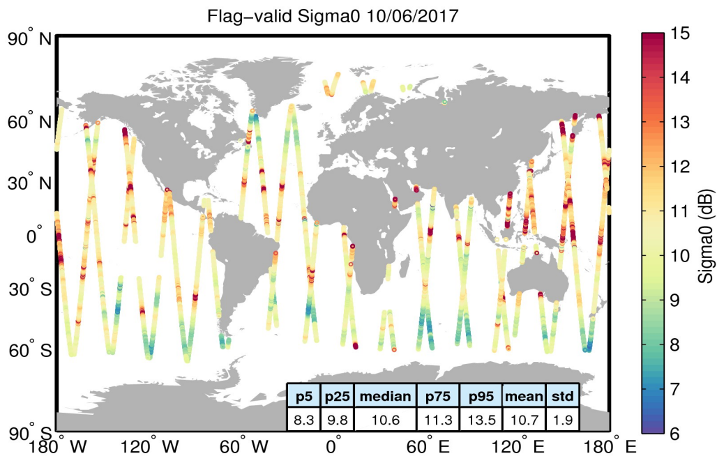
Figure 23. Geographical distribution of flag-valid sigma0 data over oceans and lakes for 10/06/2017. The statistical values shown in the table refer to the sigma0 in dB and are calculated over all measurements shown in the figure.
