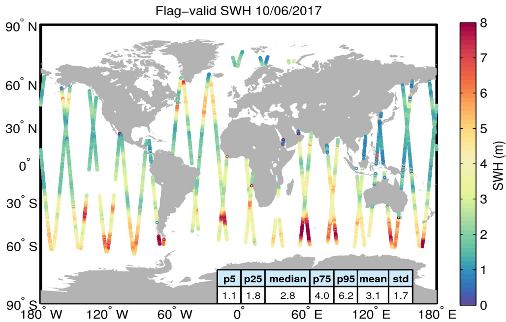
Figure 15. Geographical distribution of flag-valid SWH data over oceans and lakes for 10/06/2017. The statistical values shown in the table refer to the SWH in m and are calculated over all measurements shown in the figure.
