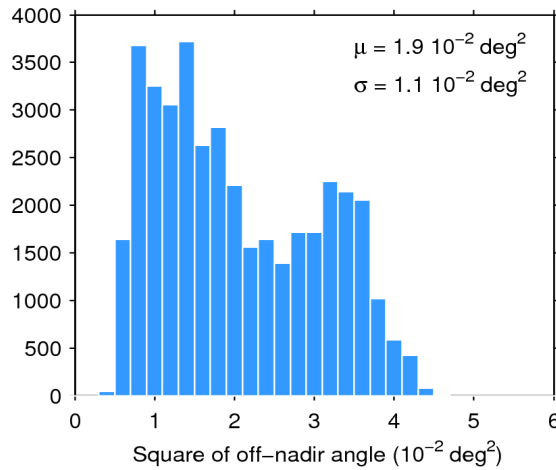
Figure 39. Histogram of flag-valid mispointing over oceans and lakes for 10/06/2017. The mean ( \mu ) and standard deviation ( \sigma ) are also shown. Note that values larger than 6 \cdot 10^{-2} \text{ deg}^2 are excluded from the histogram for the sake of readability but not from the computation of \mu and \sigma .
