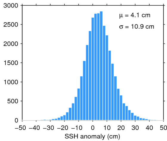
Figure 11. Histogram of science-valid SSH anomaly over oceans and lakes for 10/06/2017. The mean ( \mu ) and standard deviation ( \sigma ) are also shown. Note that values outside [-50 50] cm are excluded from the histogram for the sake of readability but not from the computation of \mu and \sigma .
