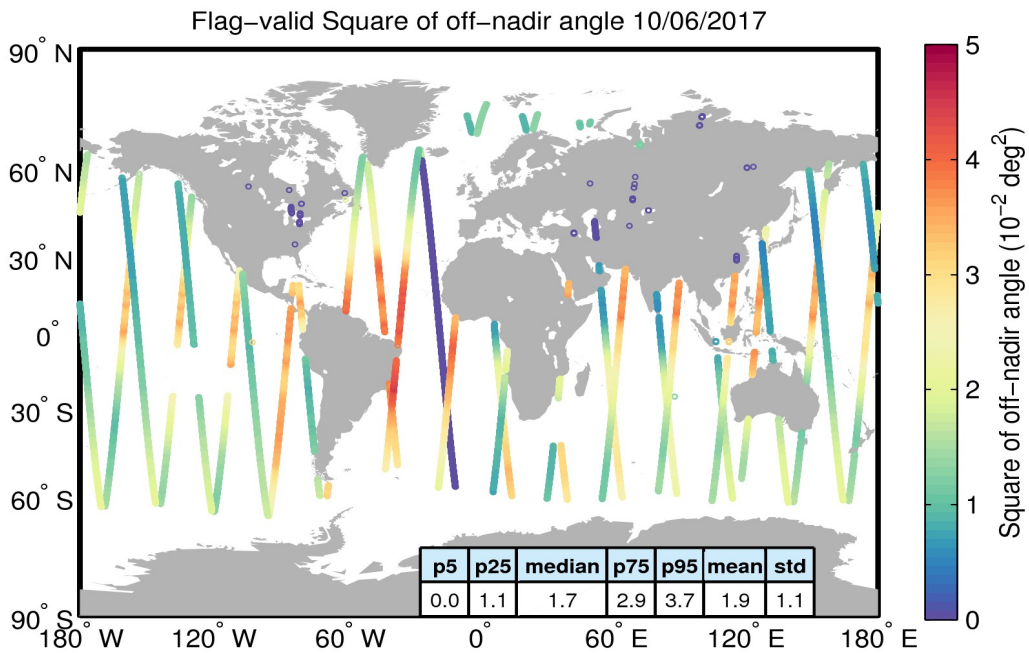
Figure 37. Geographical distribution of flag-valid mispointing data over oceans and lakes for 10/06/2017. The statistical values shown in the table refer to the mispointing in 10^{-2} deg 2 and are calculated over all measurements shown in the figure.
