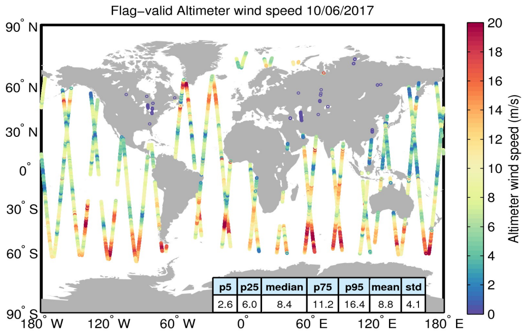
Figure 31. Geographical distribution of flag-valid wind data over oceans and lakes for 10/06/2017. The statistical values shown in the table refer to the wind in m/s and are calculated over all measurements shown in the figure.
