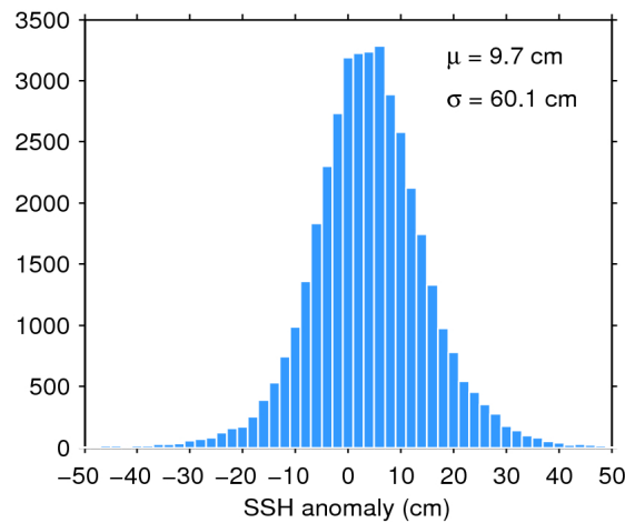
Figure 7. Histogram of flag-valid SSH anomaly over oceans and lakes for 10/06/2017. The mean ( \mu ) and standard deviation ( \sigma ) are also shown. Note that values outside [-50 50] cm are excluded from the histogram for the sake of readability but not from the computation of \mu and \sigma .
