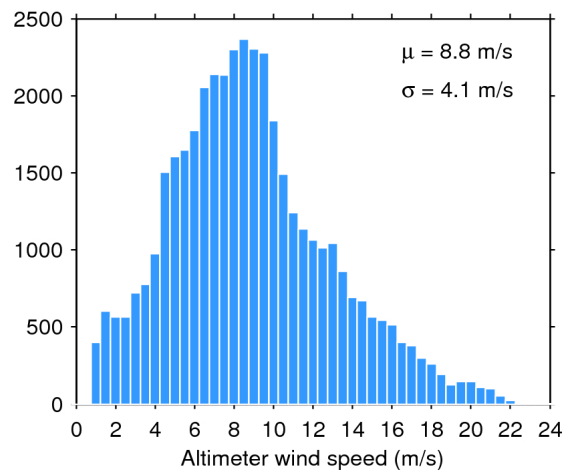
Figure 35. Histogram of science-valid wind over oceans and lakes for 10/06/2017. The mean ( \mu ) and standard deviation ( \sigma ) are also shown. Note that values larger than 24 m/s are excluded from the histogram for the sake of readability but not from the computation of \mu and \sigma .
