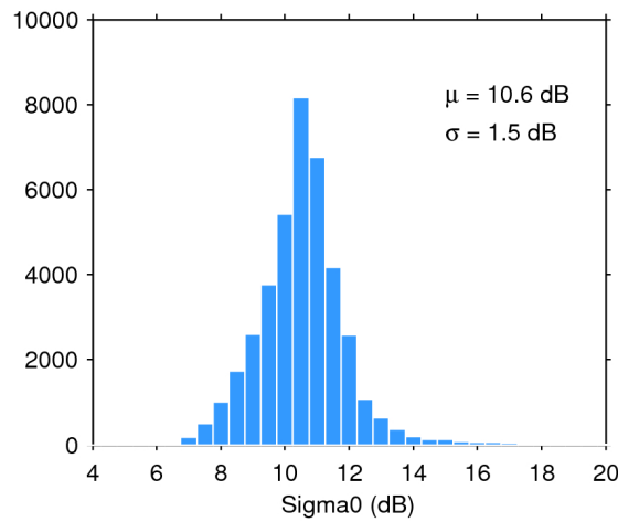
Figure 28. Histogram of science-valid sigma0 over oceans and lakes for 10/06/2017. The mean ( \mu ) and standard deviation ( \sigma ) are also shown. Note that values outside [4 20] dB are excluded from the histogram for the sake of readability but not from the computation of \mu and \sigma .
