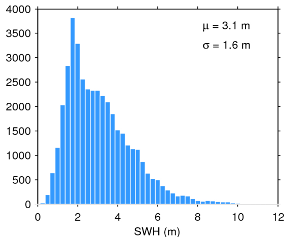
Figure 20. Histogram of science-valid SWH over oceans and lakes for 10/06/2017. The mean ( \mu ) and standard deviation ( \sigma ) are also shown. Note that values larger than 12 m are excluded from the histogram for the sake of readability but not from the computation of \mu and \sigma .
