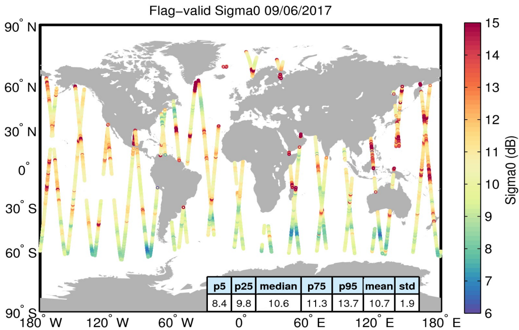
Figure 23. Geographical distribution of flag-valid sigma0 data over oceans and lakes for 09/06/2017. The statistical values shown in the table refer to the sigma0 in dB and are calculated over all measurements shown in the figure.
