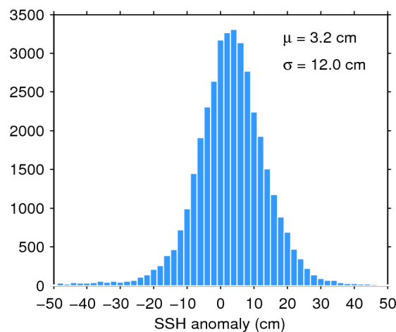
Figure 11. Histogram of science-valid SSH anomaly over oceans and lakes for 09/06/2017. The mean ( \mu ) and standard deviation ( \sigma ) are also shown. Note that values outside [-50 50] cm are excluded from the histogram for the sake of readability but not from the computation of \mu and \sigma .
