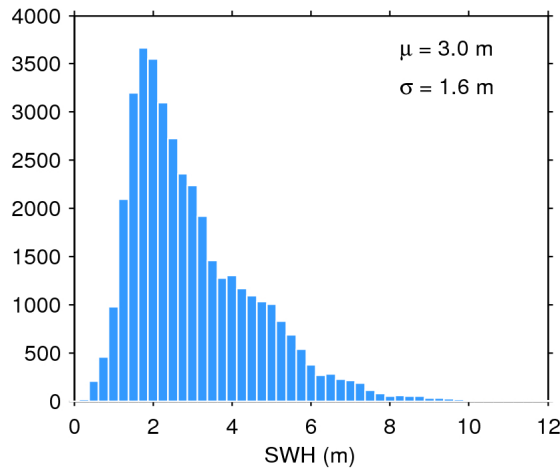
Figure 20. Histogram of science-valid SWH over oceans and lakes for 09/06/2017. The mean ( \mu ) and standard deviation ( \sigma ) are also shown. Note that values larger than 12 m are excluded from the histogram for the sake of readability but not from the computation of \mu and \sigma .
