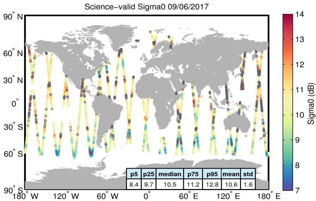
Figure 27. Geographical distribution of science-valid sigma0 data over oceans and lakes for 09/06/2017. The statistical values shown in the table refer to the sigma0 in dB and are calculated over all measurements shown in the figure. Gray circles denote records that have been rejected based on the editing criteria described in Table 4.
