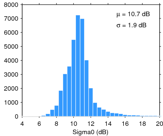
Figure 25. Histogram of flag-valid sigma0 over oceans and lakes for 09/06/2017. The mean ( \mu ) and standard deviation ( \sigma ) are also shown. Note that values outside [4 20] dB are excluded from the histogram for the sake of readability but not from the computation of \mu and \sigma .
