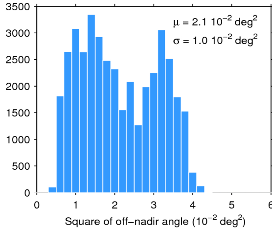
Figure 39. Histogram of flag-valid mispointing over oceans and lakes for 09/06/2017. The mean ( \mu ) and standard deviation ( \sigma ) are also shown. Note that values larger than 6 \cdot 10^{-2} \text{ deg}^2 are excluded from the histogram for the sake of readability but not from the computation of \mu and \sigma .
