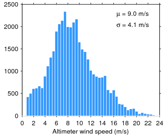
Figure 33. Histogram of flag-valid wind over oceans and lakes for 09/06/2017. The mean ( \mu ) and standard deviation ( \sigma ) are also shown. Note that values larger than 24 m/s are excluded from the histogram for the sake of readability but not from the computation of \mu and \sigma .
