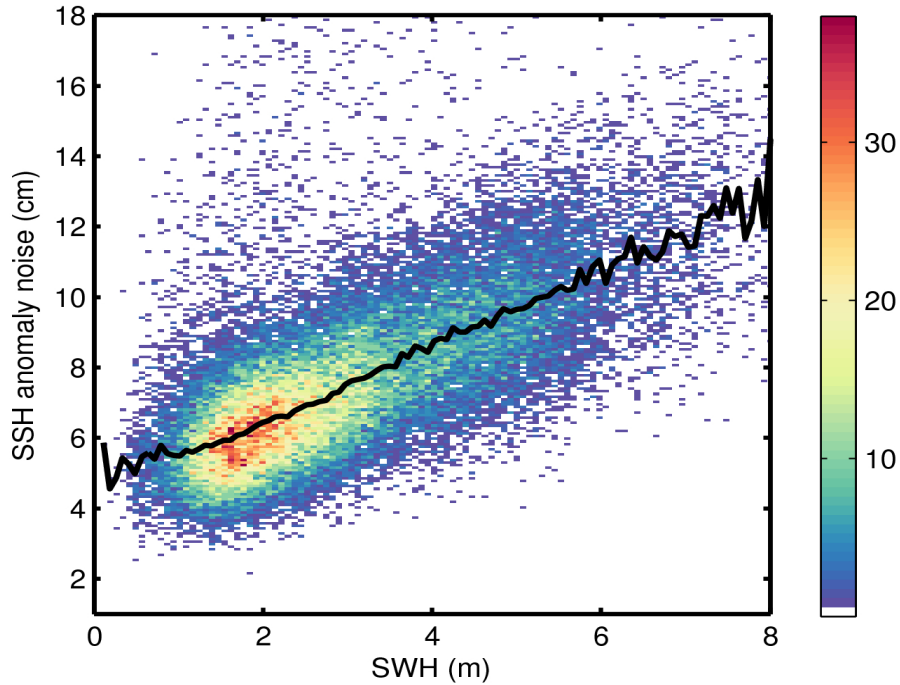
Figure 9. 2D histogram showing flag-valid SSH anomaly noise as a function of SWH for 09/06/2017. The black line denotes the median SSH anomaly noise as a function of SWH.
