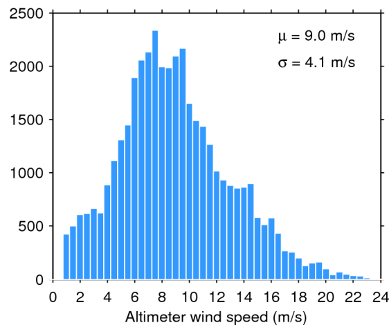
Figure 35. Histogram of science-valid wind over oceans and lakes for 09/06/2017. The mean ( \mu ) and standard deviation ( \sigma ) are also shown. Note that values larger than 24 m/s are excluded from the histogram for the sake of readability but not from the computation of \mu and \sigma .
