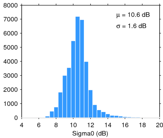
Figure 28. Histogram of science-valid sigma0 over oceans and lakes for 09/06/2017. The mean ( \mu ) and standard deviation ( \sigma ) are also shown. Note that values outside [4 20] dB are excluded from the histogram for the sake of readability but not from the computation of \mu and \sigma .
