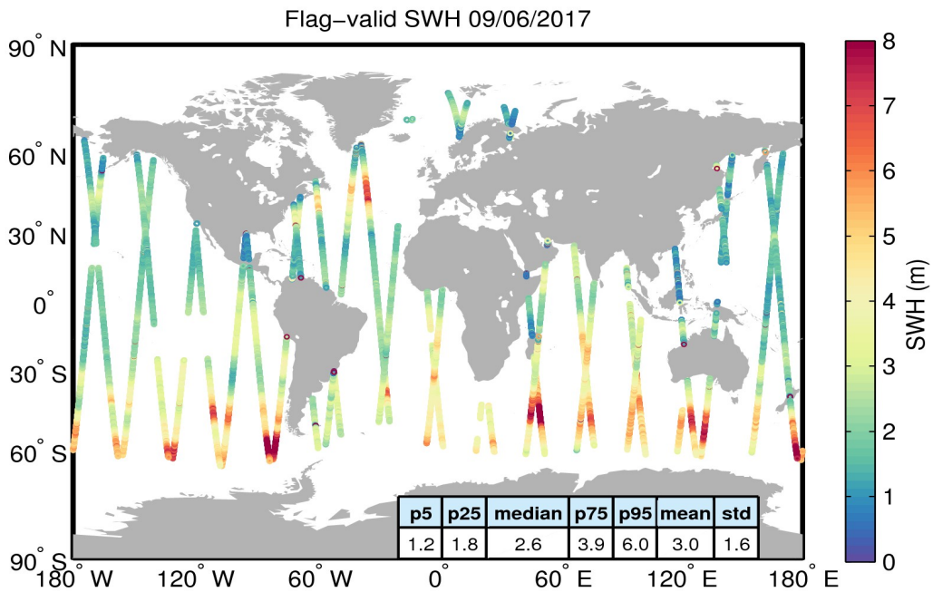
Figure 15. Geographical distribution of flag-valid SWH data over oceans and lakes for 09/06/2017. The statistical values shown in the table refer to the SWH in m and are calculated over all measurements shown in the figure.
