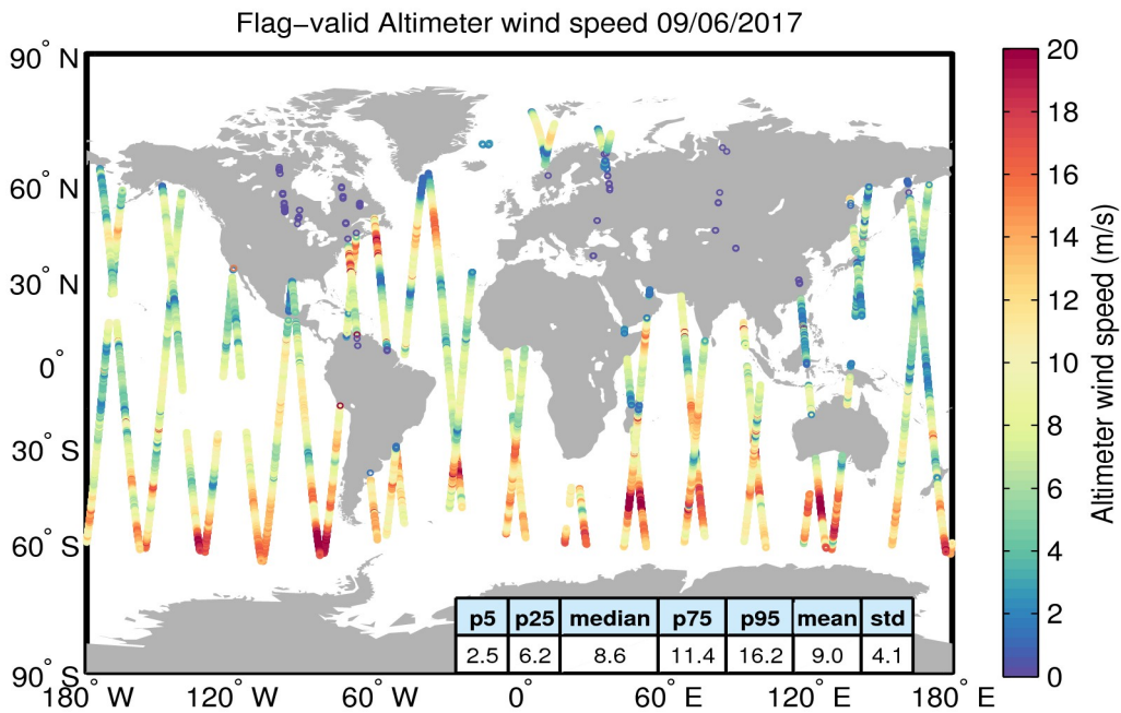
Figure 31. Geographical distribution of flag-valid wind data over oceans and lakes for 09/06/2017. The statistical values shown in the table refer to the wind in m/s and are calculated over all measurements shown in the figure.
