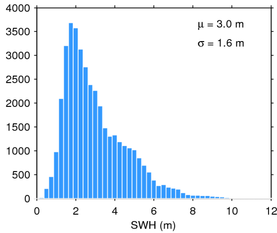
Figure 17. Histogram of flag-valid SWH over oceans and lakes for 09/06/2017. The mean ( \mu ) and standard deviation ( \sigma ) are also shown. Note that values larger than 12 m are excluded from the histogram for the sake of readability but not from the computation of \mu and \sigma .
