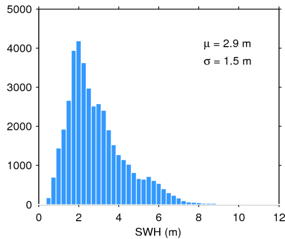
Figure 17. Histogram of flag-valid SWH over oceans and lakes for 08/06/2017. The mean ( \mu ) and standard deviation ( \sigma ) are also shown. Note that values larger than 12 m are excluded from the histogram for the sake of readability but not from the computation of \mu and \sigma .
