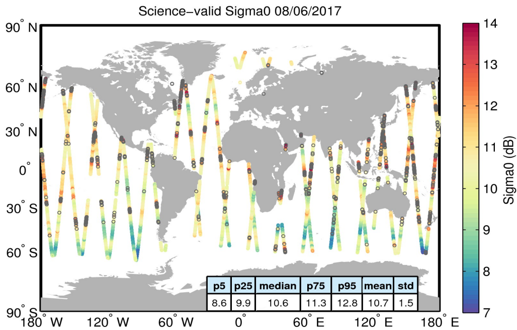
Figure 27. Geographical distribution of science-valid sigma0 data over oceans and lakes for 08/06/2017. The statistical values shown in the table refer to the sigma0 in dB and are calculated over all measurements shown in the figure. Gray circles denote records that have been rejected based on the editing criteria described in Table 4.
