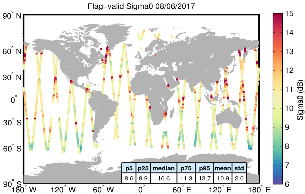
Figure 23. Geographical distribution of flag-valid sigma0 data over oceans and lakes for 08/06/2017. The statistical values shown in the table refer to the sigma0 in dB and are calculated over all measurements shown in the figure.
