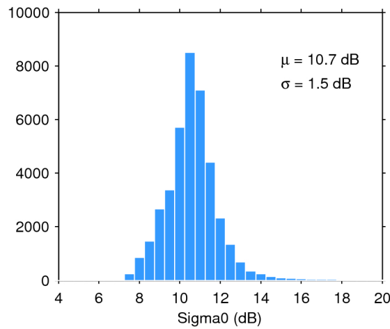
Figure 28. Histogram of science-valid sigma0 over oceans and lakes for 08/06/2017. The mean ( \mu ) and standard deviation ( \sigma ) are also shown. Note that values outside [4 20] dB are excluded from the histogram for the sake of readability but not from the computation of \mu and \sigma .
