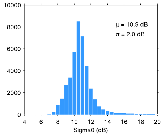
Figure 25. Histogram of flag-valid sigma0 over oceans and lakes for 08/06/2017. The mean ( \mu ) and standard deviation ( \sigma ) are also shown. Note that values outside [4 20] dB are excluded from the histogram for the sake of readability but not from the computation of \mu and \sigma .
