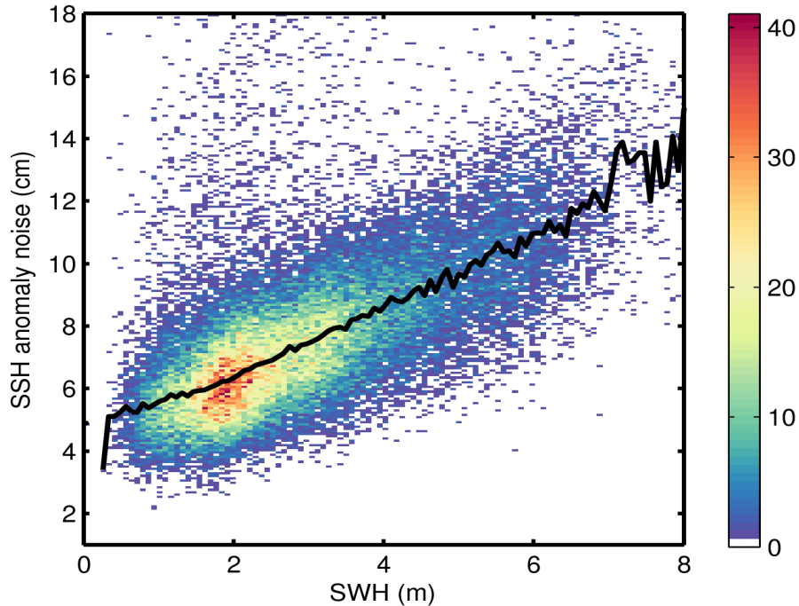
Figure 9. 2D histogram showing flag-valid SSH anomaly noise as a function of SWH for 08/06/2017. The black line denotes the median SSH anomaly noise as a function of SWH.
