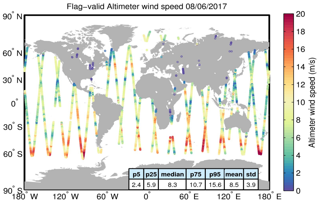
Figure 31. Geographical distribution of flag-valid wind data over oceans and lakes for 08/06/2017. The statistical values shown in the table refer to the wind in m/s and are calculated over all measurements shown in the figure.
