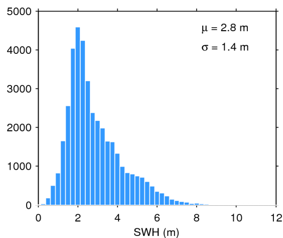
Figure 20. Histogram of science-valid SWH over oceans and lakes for 07/06/2017. The mean ( \mu ) and standard deviation ( \sigma ) are also shown. Note that values larger than 12 m are excluded from the histogram for the sake of readability but not from the computation of \mu and \sigma .
