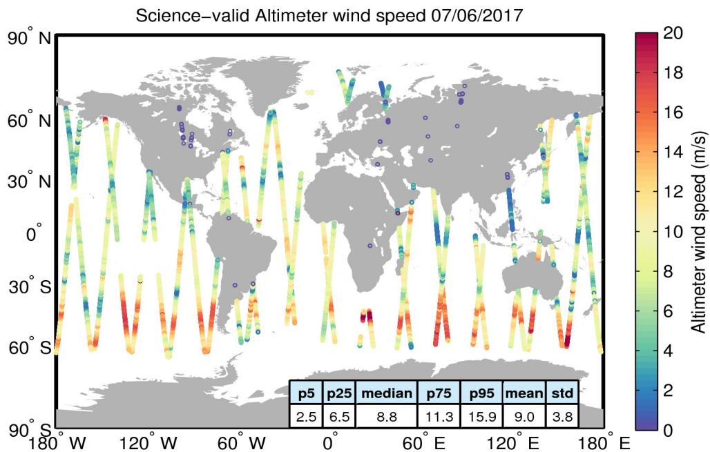
Figure 34. Geographical distribution of science-valid wind data over oceans and lakes for 07/06/2017. The statistical values shown in the table refer to the wind in m/s and are calculated over all measurements shown in the figure. Gray circles denote records that have been rejected based on the editing criteria described in Table 5.
