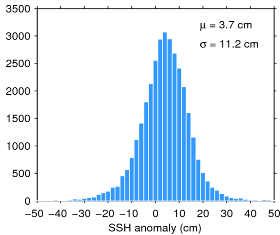
Figure 11. Histogram of science-valid SSH anomaly over oceans and lakes for 07/06/2017. The mean ( \mu ) and standard deviation ( \sigma ) are also shown. Note that values outside [-50 50] cm are excluded from the histogram for the sake of readability but not from the computation of \mu and \sigma .
