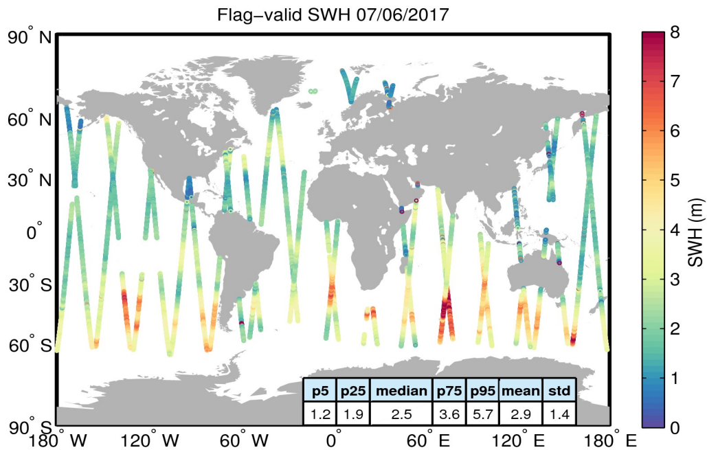
Figure 15. Geographical distribution of flag-valid SWH data over oceans and lakes for 07/06/2017. The statistical values shown in the table refer to the SWH in m and are calculated over all measurements shown in the figure.
