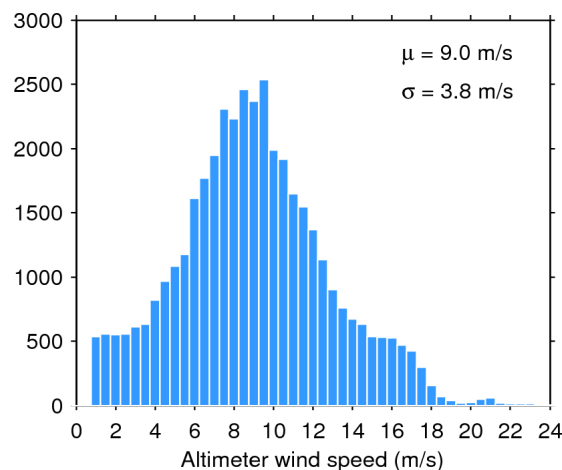
Figure 35. Histogram of science-valid wind over oceans and lakes for 07/06/2017. The mean ( \mu ) and standard deviation ( \sigma ) are also shown. Note that values larger than 24 m/s are excluded from the histogram for the sake of readability but not from the computation of \mu and \sigma .
