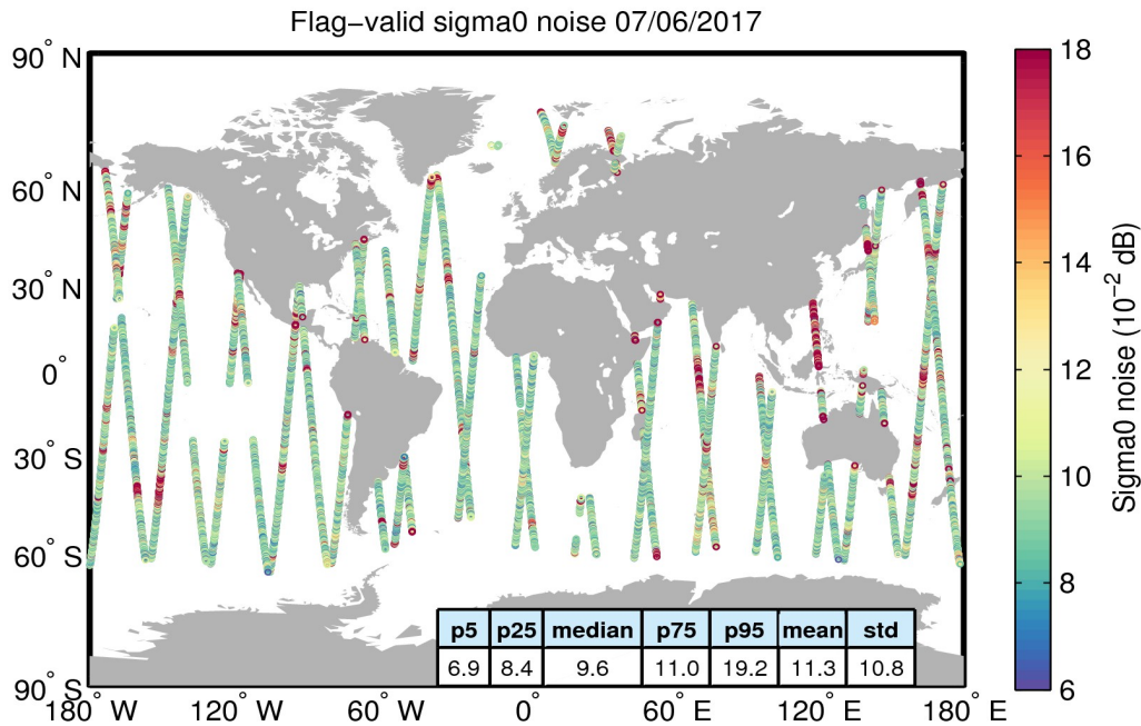
Figure 26. Geographical distribution of flag-valid 20-Hz sigma0 measurement noise over oceans and lakes for 07/06/2017. The statistical values shown in the table refer to the sigma0 noise and are calculated over all measurements shown in the figure.
