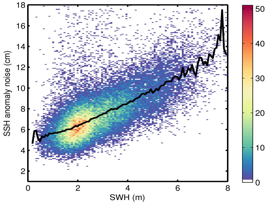
Figure 9. 2D histogram showing flag-valid SSH anomaly noise as a function of SWH for 07/06/2017. The black line denotes the median SSH anomaly noise as a function of SWH.
