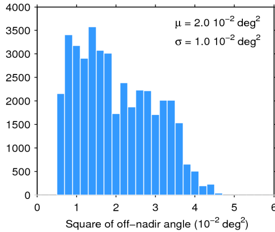
Figure 39. Histogram of flag-valid mispointing over oceans and lakes for 07/06/2017. The mean ( \mu ) and standard deviation ( \sigma ) are also shown. Note that values larger than 6 \cdot 10^{-2} \text{ deg}^2 are excluded from the histogram for the sake of readability but not from the computation of \mu and \sigma .
