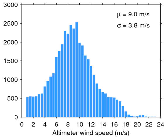
Figure 33. Histogram of flag-valid wind over oceans and lakes for 07/06/2017. The mean ( \mu ) and standard deviation ( \sigma ) are also shown. Note that values larger than 24 m/s are excluded from the histogram for the sake of readability but not from the computation of \mu and \sigma .
