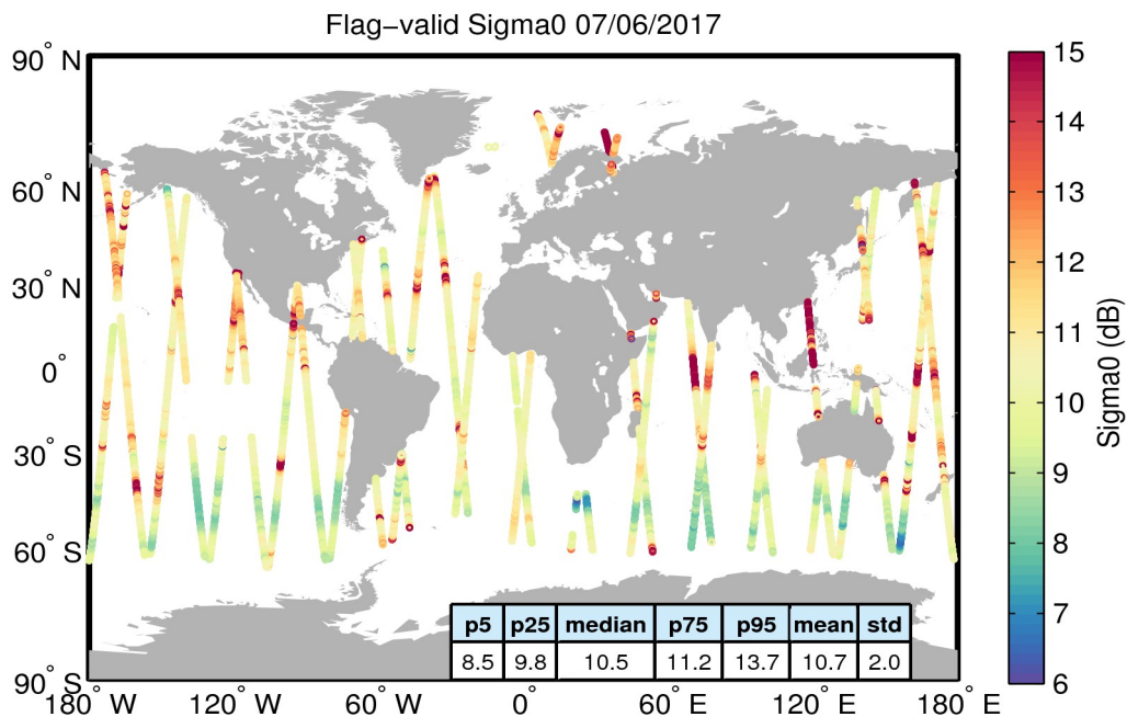
Figure 23. Geographical distribution of flag-valid sigma0 data over oceans and lakes for 07/06/2017. The statistical values shown in the table refer to the sigma0 in dB and are calculated over all measurements shown in the figure.
