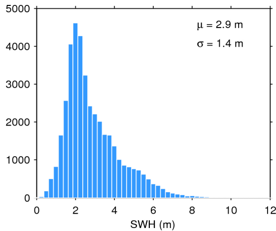
Figure 17. Histogram of flag-valid SWH over oceans and lakes for 07/06/2017. The mean ( \mu ) and standard deviation ( \sigma ) are also shown. Note that values larger than 12 m are excluded from the histogram for the sake of readability but not from the computation of \mu and \sigma .
