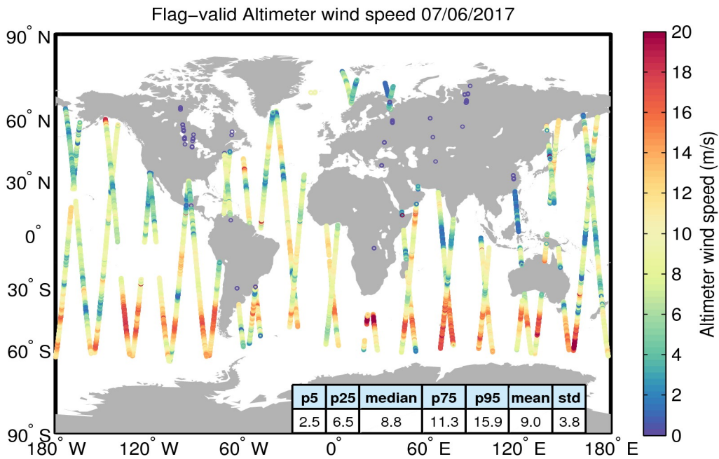
Figure 31. Geographical distribution of flag-valid wind data over oceans and lakes for 07/06/2017. The statistical values shown in the table refer to the wind in m/s and are calculated over all measurements shown in the figure.
