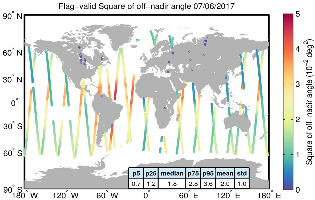
Figure 37. Geographical distribution of flag-valid mispointing data over oceans and lakes for 07/06/2017. The statistical values shown in the table refer to the mispointing in 10^{-2} deg 2 and are calculated over all measurements shown in the figure.
