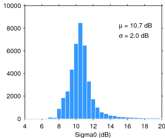
Figure 25. Histogram of flag-valid sigma0 over oceans and lakes for 07/06/2017. The mean ( \mu ) and standard deviation ( \sigma ) are also shown. Note that values outside [4 20] dB are excluded from the histogram for the sake of readability but not from the computation of \mu and \sigma .
