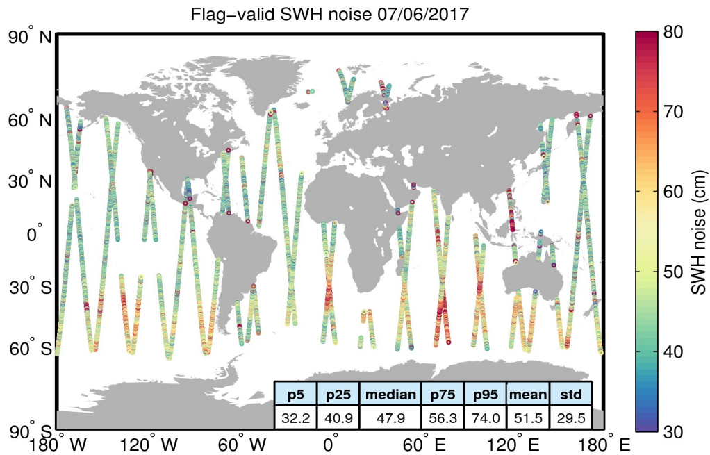
Figure 18. Geographical distribution of flag-valid 20-Hz SWH measurement noise over oceans and lakes for 07/06/2017. The statistical values shown in the table refer to the SWH noise and are calculated over all measurements shown in the figure.
