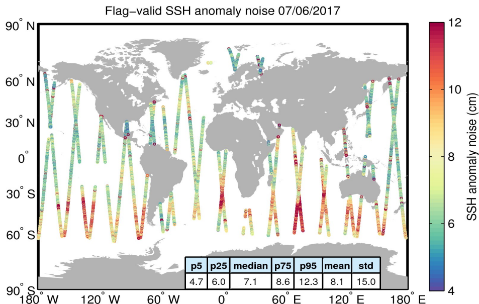
Figure 8. Geographical distribution of flag-valid 20-Hz SSH anomaly measurement noise over oceans and lakes for 07/06/2017. The statistical values shown in the table refer to the SSH anomaly noise and are calculated over all measurements shown in the figure.
