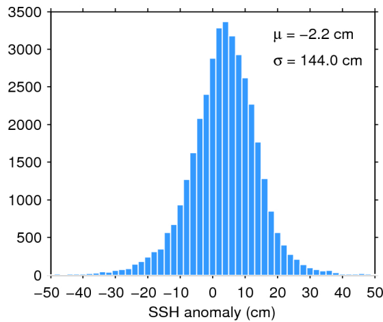
Figure 7. Histogram of flag-valid SSH anomaly over oceans and lakes for 07/06/2017. The mean ( \mu ) and standard deviation ( \sigma ) are also shown. Note that values outside [-50\ 50] cm are excluded from the histogram for the sake of readability but not from the computation of \mu and \sigma .
