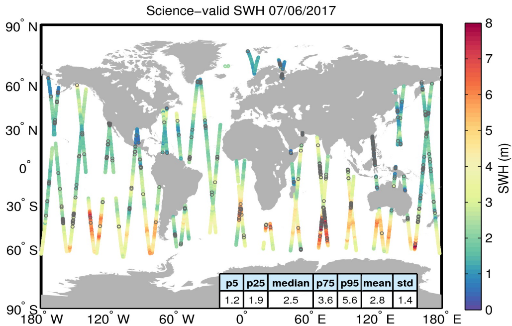
Figure 19. Geographical distribution of science-valid SWH data over oceans and lakes for 07/06/2017. The statistical values shown in the table refer to the SWH in m and are calculated over all measurements shown in the figure. Gray circles denote records that have been rejected based on the editing criteria described in Table 3.
