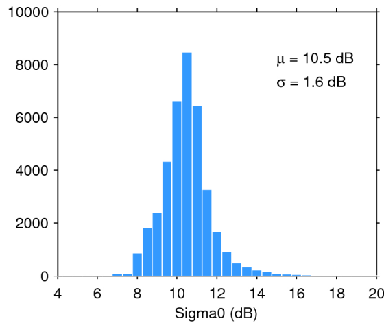
Figure 28. Histogram of science-valid sigma0 over oceans and lakes for 07/06/2017. The mean ( \mu ) and standard deviation ( \sigma ) are also shown. Note that values outside [4 20] dB are excluded from the histogram for the sake of readability but not from the computation of \mu and \sigma .
