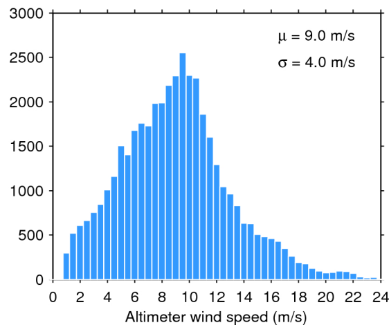
Figure 35. Histogram of science-valid wind over oceans and lakes for 06/06/2017. The mean ( \mu ) and standard deviation ( \sigma ) are also shown. Note that values larger than 24 m/s are excluded from the histogram for the sake of readability but not from the computation of \mu and \sigma .
