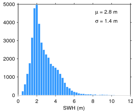
Figure 17. Histogram of flag-valid SWH over oceans and lakes for 06/06/2017. The mean ( \mu ) and standard deviation ( \sigma ) are also shown. Note that values larger than 12 m are excluded from the histogram for the sake of readability but not from the computation of \mu and \sigma .
