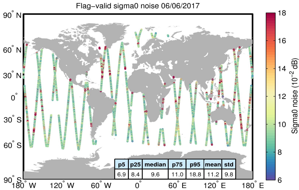
Figure 26. Geographical distribution of flag-valid 20-Hz sigma0 measurement noise over oceans and lakes for 06/06/2017. The statistical values shown in the table refer to the sigma0 noise and are calculated over all measurements shown in the figure.
