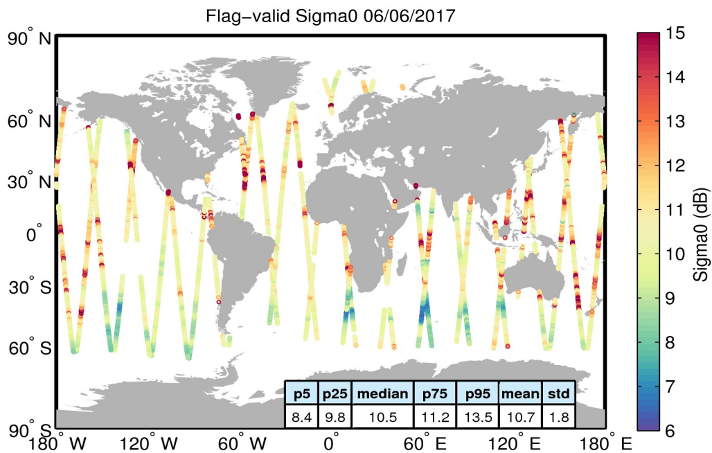
Figure 23. Geographical distribution of flag-valid sigma0 data over oceans and lakes for 06/06/2017. The statistical values shown in the table refer to the sigma0 in dB and are calculated over all measurements shown in the figure.
