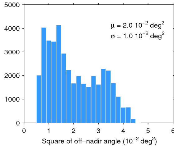
Figure 39. Histogram of flag-valid mispointing over oceans and lakes for 06/06/2017. The mean ( \mu ) and standard deviation ( \sigma ) are also shown. Note that values larger than 6 \cdot 10^{-2} \text{ deg}^2 are excluded from the histogram for the sake of readability but not from the computation of \mu and \sigma .
