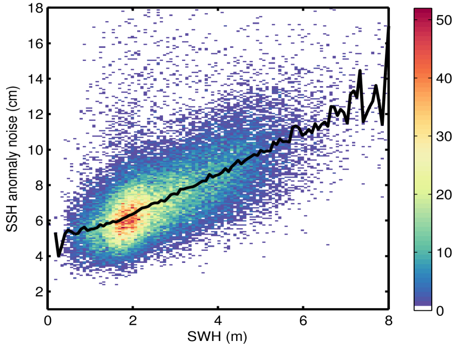
Figure 9. 2D histogram showing flag-valid SSH anomaly noise as a function of SWH for 06/06/2017. The black line denotes the median SSH anomaly noise as a function of SWH.
