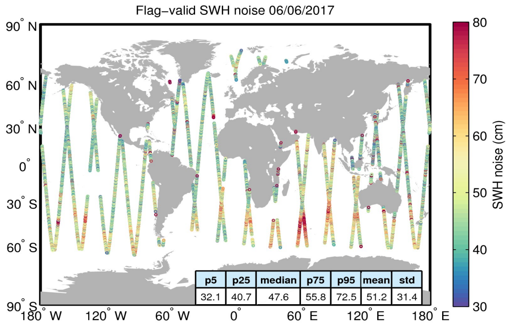
Figure 18. Geographical distribution of flag-valid 20-Hz SWH measurement noise over oceans and lakes for 06/06/2017. The statistical values shown in the table refer to the SWH noise and are calculated over all measurements shown in the figure.
