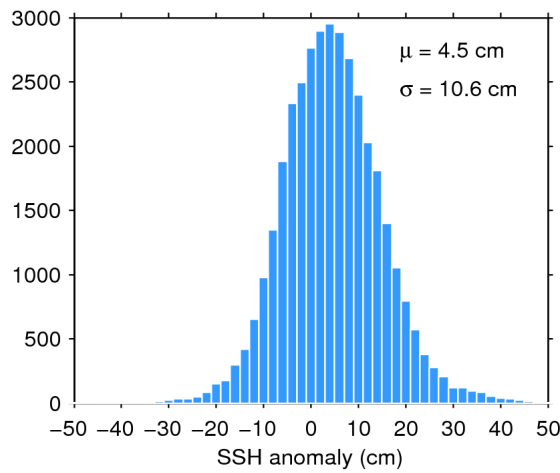
Figure 11. Histogram of science-valid SSH anomaly over oceans and lakes for 06/06/2017. The mean ( \mu ) and standard deviation ( \sigma ) are also shown. Note that values outside [-50 50] cm are excluded from the histogram for the sake of readability but not from the computation of \mu and \sigma .
