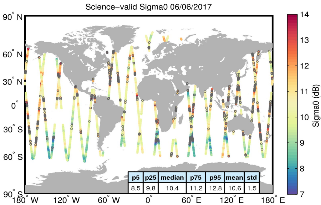
Figure 27. Geographical distribution of science-valid sigma0 data over oceans and lakes for 06/06/2017. The statistical values shown in the table refer to the sigma0 in dB and are calculated over all measurements shown in the figure. Gray circles denote records that have been rejected based on the editing criteria described in Table 4.
