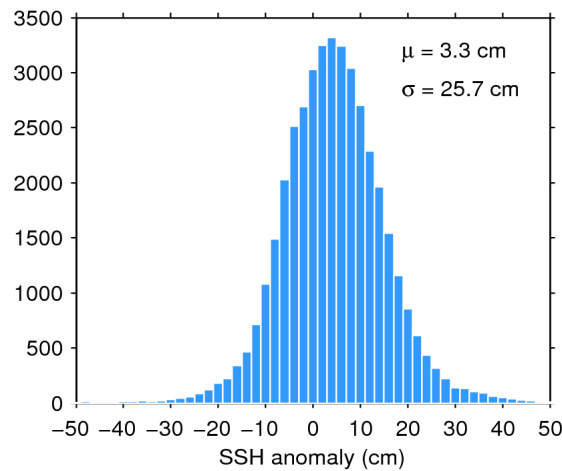
Figure 7. Histogram of flag-valid SSH anomaly over oceans and lakes for 06/06/2017. The mean ( \mu ) and standard deviation ( \sigma ) are also shown. Note that values outside [-50\ 50] cm are excluded from the histogram for the sake of readability but not from the computation of \mu and \sigma .
