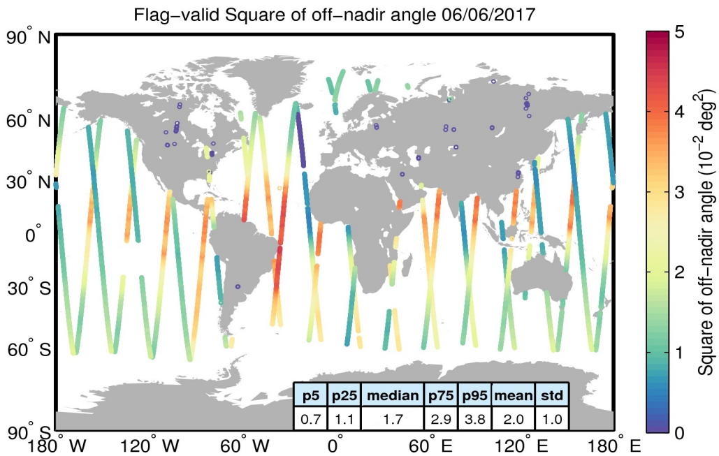
Figure 37. Geographical distribution of flag-valid mispointing data over oceans and lakes for 06/06/2017. The statistical values shown in the table refer to the mispointing in 10^{-2} deg 2 and are calculated over all measurements shown in the figure.
