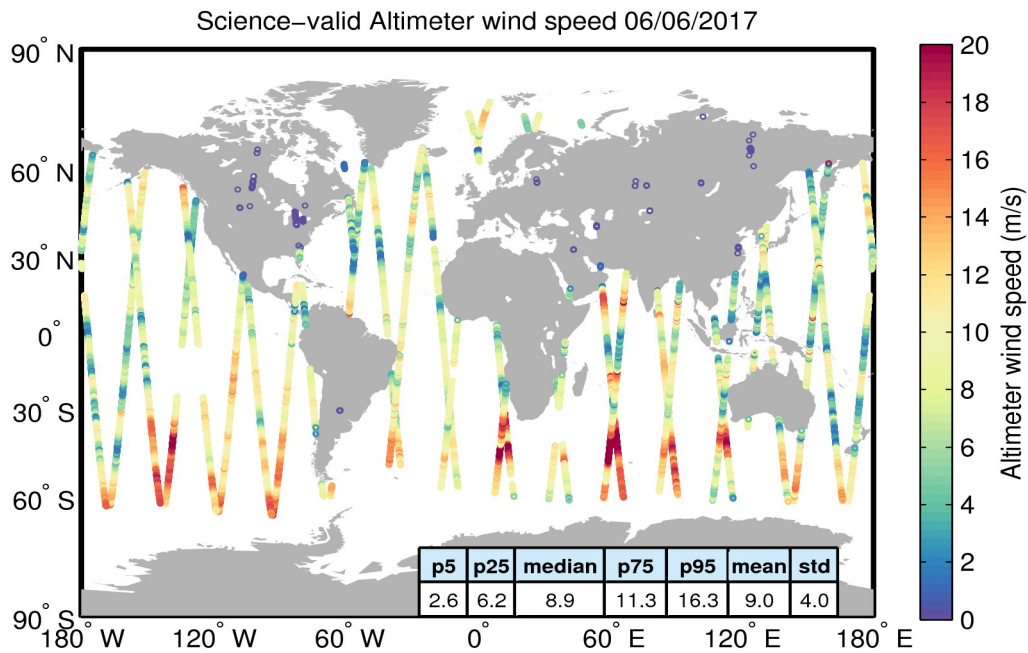
Figure 34. Geographical distribution of science-valid wind data over oceans and lakes for 06/06/2017. The statistical values shown in the table refer to the wind in m/s and are calculated over all measurements shown in the figure. Gray circles denote records that have been rejected based on the editing criteria described in Table 5.
