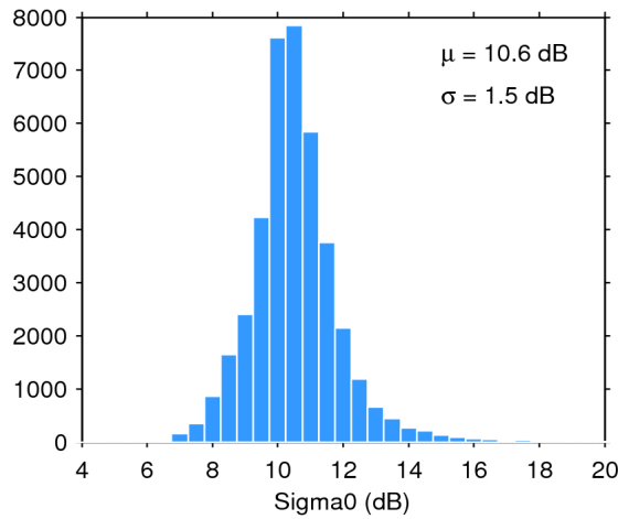
Figure 28. Histogram of science-valid sigma0 over oceans and lakes for 06/06/2017. The mean ( \mu ) and standard deviation ( \sigma ) are also shown. Note that values outside [4 20] dB are excluded from the histogram for the sake of readability but not from the computation of \mu and \sigma .
