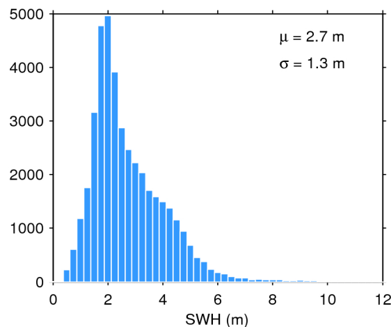
Figure 20. Histogram of science-valid SWH over oceans and lakes for 06/06/2017. The mean ( \mu ) and standard deviation ( \sigma ) are also shown. Note that values larger than 12 m are excluded from the histogram for the sake of readability but not from the computation of \mu and \sigma .
