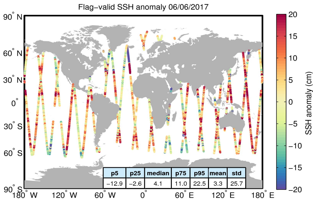
Figure 5. Geographical distribution of flag-valid 1-Hz SSH anomaly data over oceans and lakes for 06/06/2017. The statistical values shown in the table refer to the SSH anomaly in cm and are calculated over all measurements shown in the figure.
