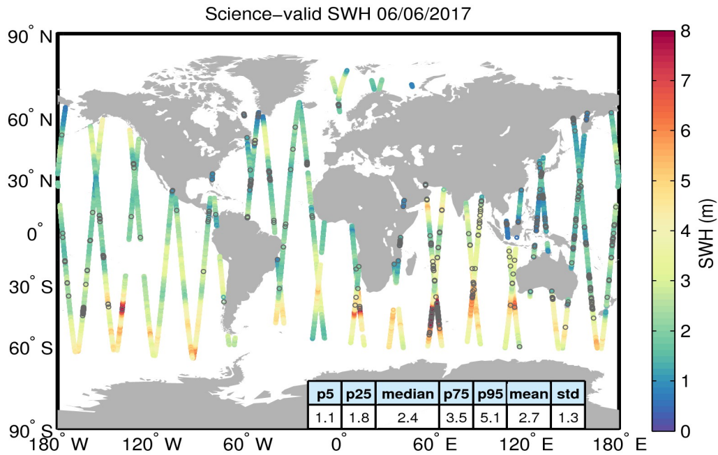
Figure 19. Geographical distribution of science-valid SWH data over oceans and lakes for 06/06/2017. The statistical values shown in the table refer to the SWH in m and are calculated over all measurements shown in the figure. Gray circles denote records that have been rejected based on the editing criteria described in Table 3.
