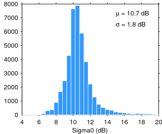
Figure 25. Histogram of flag-valid sigma0 over oceans and lakes for 06/06/2017. The mean ( \mu ) and standard deviation ( \sigma ) are also shown. Note that values outside [4 20] dB are excluded from the histogram for the sake of readability but not from the computation of \mu and \sigma .
