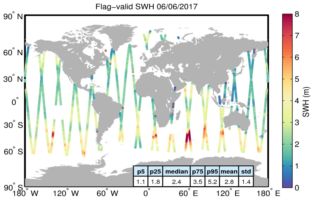
Figure 15. Geographical distribution of flag-valid SWH data over oceans and lakes for 06/06/2017. The statistical values shown in the table refer to the SWH in m and are calculated over all measurements shown in the figure.
