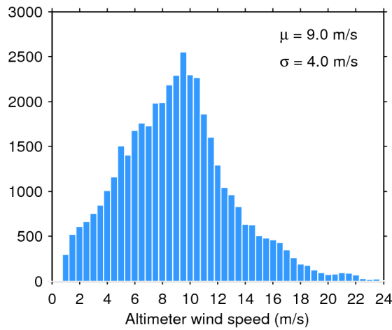
Figure 33. Histogram of flag-valid wind over oceans and lakes for 06/06/2017. The mean ( \mu ) and standard deviation ( \sigma ) are also shown. Note that values larger than 24 m/s are excluded from the histogram for the sake of readability but not from the computation of \mu and \sigma .
