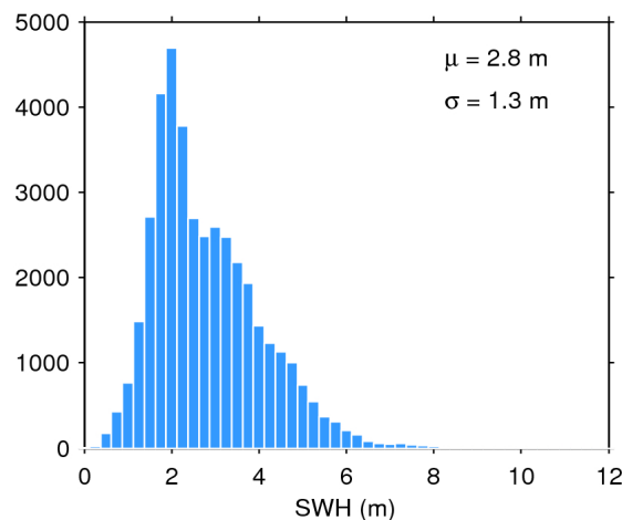
Figure 20. Histogram of science-valid SWH over oceans and lakes for 05/06/2017. The mean ( \mu ) and standard deviation ( \sigma ) are also shown. Note that values larger than 12 m are excluded from the histogram for the sake of readability but not from the computation of \mu and \sigma .
