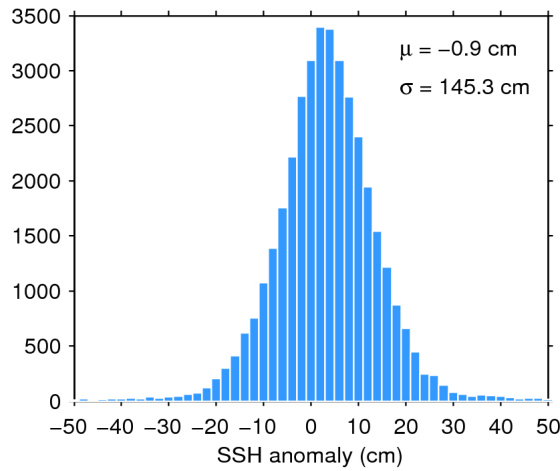
Figure 7. Histogram of flag-valid SSH anomaly over oceans and lakes for 05/06/2017. The mean ( \mu ) and standard deviation ( \sigma ) are also shown. Note that values outside [-50 50] cm are excluded from the histogram for the sake of readability but not from the computation of \mu and \sigma .
