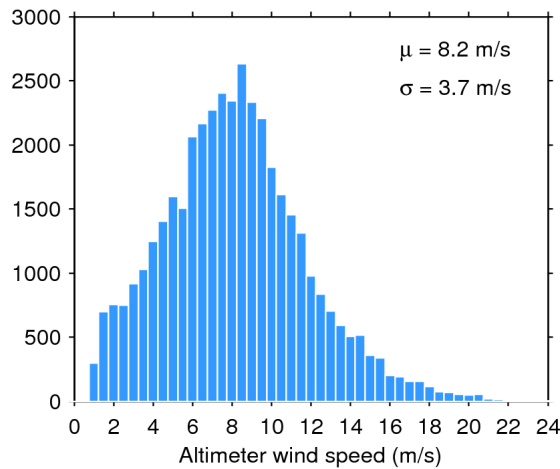
Figure 33. Histogram of flag-valid wind over oceans and lakes for 05/06/2017. The mean ( \mu ) and standard deviation ( \sigma ) are also shown. Note that values larger than 24 m/s are excluded from the histogram for the sake of readability but not from the computation of \mu and \sigma .
