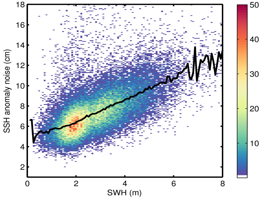
Figure 9. 2D histogram showing flag-valid SSH anomaly noise as a function of SWH for 05/06/2017. The black line denotes the median SSH anomaly noise as a function of SWH.
