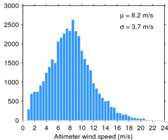
Figure 35. Histogram of science-valid wind over oceans and lakes for 05/06/2017. The mean ( \mu ) and standard deviation ( \sigma ) are also shown. Note that values larger than 24 m/s are excluded from the histogram for the sake of readability but not from the computation of \mu and \sigma .
