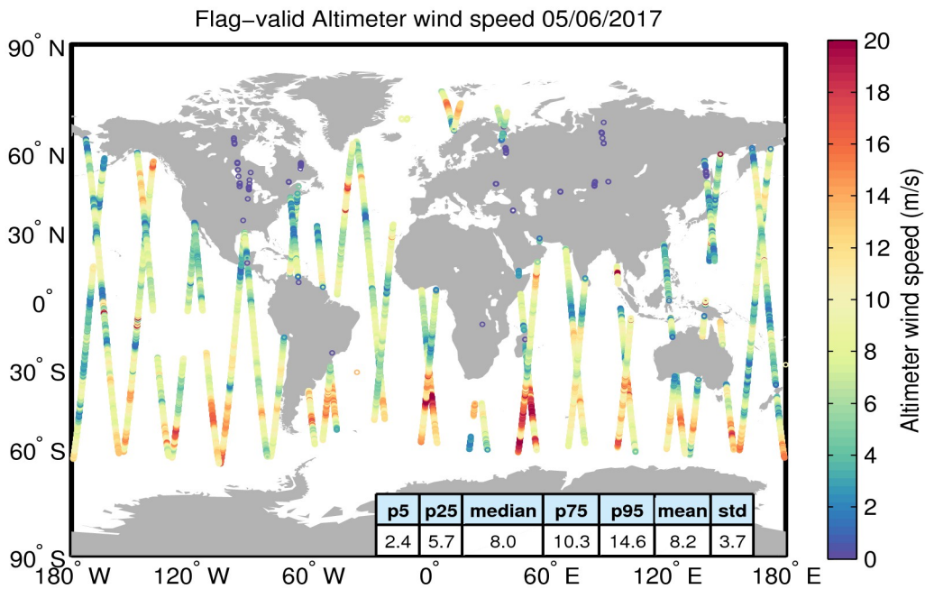
Figure 31. Geographical distribution of flag-valid wind data over oceans and lakes for 05/06/2017. The statistical values shown in the table refer to the wind in m/s and are calculated over all measurements shown in the figure.
