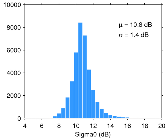
Figure 28. Histogram of science-valid sigma0 over oceans and lakes for 05/06/2017. The mean ( \mu ) and standard deviation ( \sigma ) are also shown. Note that values outside [4 20] dB are excluded from the histogram for the sake of readability but not from the computation of \mu and \sigma .
