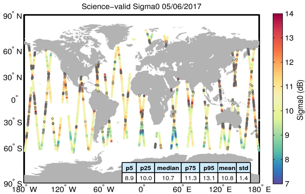
Figure 27. Geographical distribution of science-valid sigma0 data over oceans and lakes for 05/06/2017. The statistical values shown in the table refer to the sigma0 in dB and are calculated over all measurements shown in the figure. Gray circles denote records that have been rejected based on the editing criteria described in Table 4.
