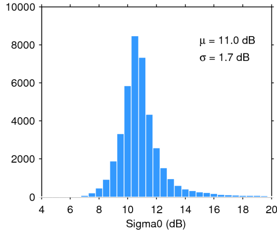
Figure 25. Histogram of flag-valid sigma0 over oceans and lakes for 05/06/2017. The mean ( \mu ) and standard deviation ( \sigma ) are also shown. Note that values outside [4 20] dB are excluded from the histogram for the sake of readability but not from the computation of \mu and \sigma .
