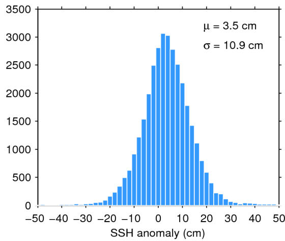
Figure 11. Histogram of science-valid SSH anomaly over oceans and lakes for 05/06/2017. The mean ( \mu ) and standard deviation ( \sigma ) are also shown. Note that values outside [-50 50] cm are excluded from the histogram for the sake of readability but not from the computation of \mu and \sigma .
