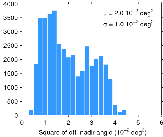
Figure 39. Histogram of flag-valid mispointing over oceans and lakes for 05/06/2017. The mean ( \mu ) and standard deviation ( \sigma ) are also shown. Note that values larger than 6 \cdot 10^{-2} \text{ deg}^2 are excluded from the histogram for the sake of readability but not from the computation of \mu and \sigma .
