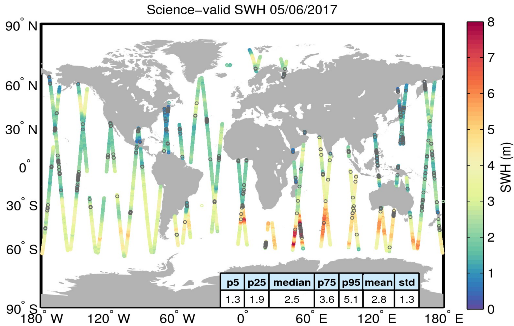
Figure 19. Geographical distribution of science-valid SWH data over oceans and lakes for 05/06/2017. The statistical values shown in the table refer to the SWH in m and are calculated over all measurements shown in the figure. Gray circles denote records that have been rejected based on the editing criteria described in Table 3.
