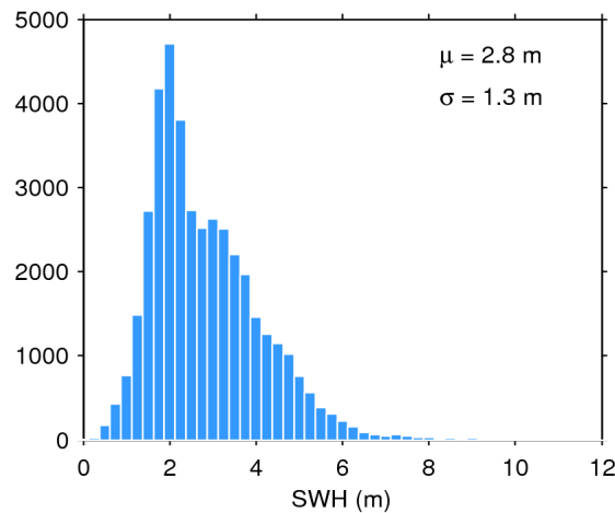
Figure 17. Histogram of flag-valid SWH over oceans and lakes for 05/06/2017. The mean ( \mu ) and standard deviation ( \sigma ) are also shown. Note that values larger than 12 m are excluded from the histogram for the sake of readability but not from the computation of \mu and \sigma .
