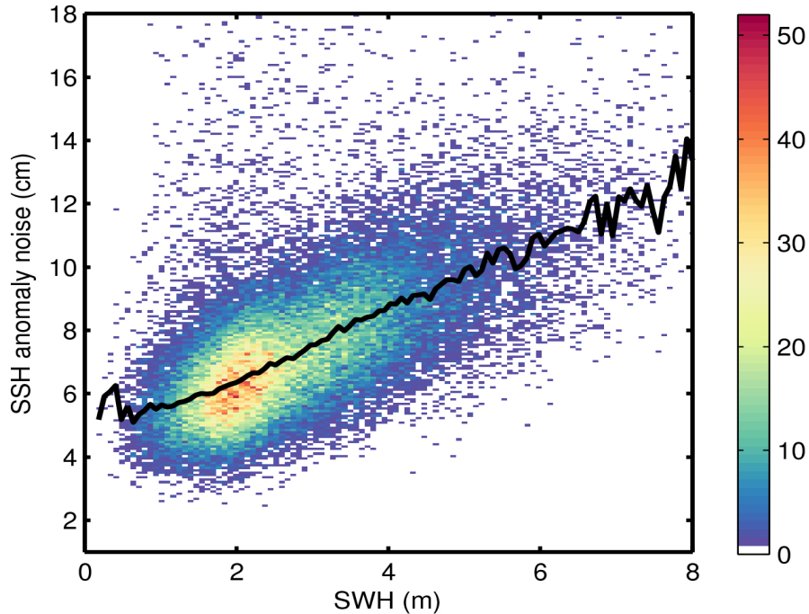
Figure 9. 2D histogram showing flag-valid SSH anomaly noise as a function of SWH for 04/06/2017. The black line denotes the median SSH anomaly noise as a function of SWH.
