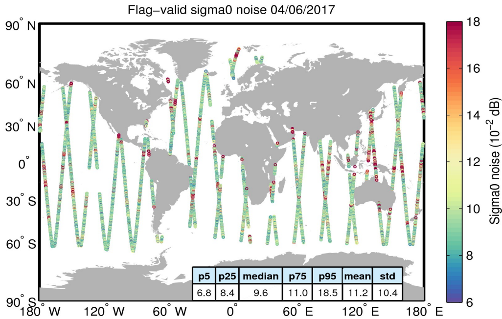
Figure 26. Geographical distribution of flag-valid 20-Hz sigma0 measurement noise over oceans and lakes for 04/06/2017. The statistical values shown in the table refer to the sigma0 noise and are calculated over all measurements shown in the figure.
