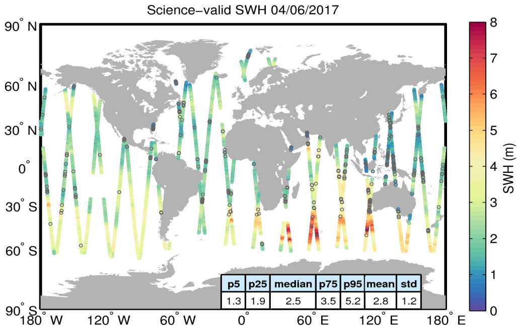
Figure 19. Geographical distribution of science-valid SWH data over oceans and lakes for 04/06/2017. The statistical values shown in the table refer to the SWH in m and are calculated over all measurements shown in the figure. Gray circles denote records that have been rejected based on the editing criteria described in Table 3.
