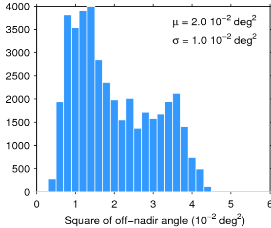
Figure 39. Histogram of flag-valid mispointing over oceans and lakes for 04/06/2017. The mean ( \mu ) and standard deviation ( \sigma ) are also shown. Note that values larger than 6 \cdot 10^{-2} \text{ deg}^2 are excluded from the histogram for the sake of readability but not from the computation of \mu and \sigma .
