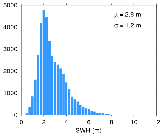
Figure 20. Histogram of science-valid SWH over oceans and lakes for 04/06/2017. The mean ( \mu ) and standard deviation ( \sigma ) are also shown. Note that values larger than 12 m are excluded from the histogram for the sake of readability but not from the computation of \mu and \sigma .
