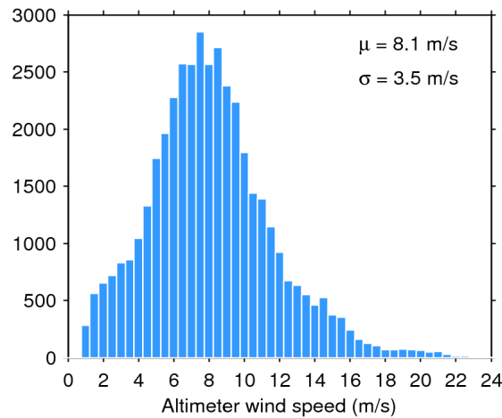
Figure 33. Histogram of flag-valid wind over oceans and lakes for 04/06/2017. The mean ( \mu ) and standard deviation ( \sigma ) are also shown. Note that values larger than 24 m/s are excluded from the histogram for the sake of readability but not from the computation of \mu and \sigma .
