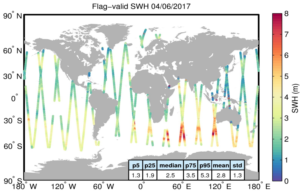
Figure 15. Geographical distribution of flag-valid SWH data over oceans and lakes for 04/06/2017. The statistical values shown in the table refer to the SWH in m and are calculated over all measurements shown in the figure.
