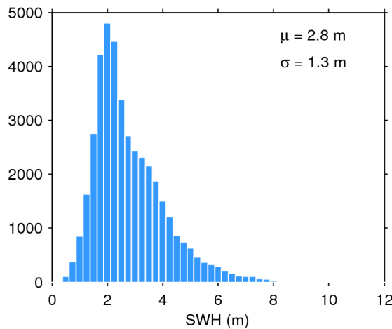
Figure 17. Histogram of flag-valid SWH over oceans and lakes for 04/06/2017. The mean ( \mu ) and standard deviation ( \sigma ) are also shown. Note that values larger than 12 m are excluded from the histogram for the sake of readability but not from the computation of \mu and \sigma .
