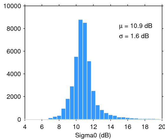
Figure 25. Histogram of flag-valid sigma0 over oceans and lakes for 04/06/2017. The mean ( \mu ) and standard deviation ( \sigma ) are also shown. Note that values outside [4 20] dB are excluded from the histogram for the sake of readability but not from the computation of \mu and \sigma .
