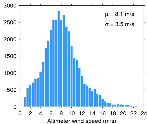
Figure 35. Histogram of science-valid wind over oceans and lakes for 04/06/2017. The mean ( \mu ) and standard deviation ( \sigma ) are also shown. Note that values larger than 24 m/s are excluded from the histogram for the sake of readability but not from the computation of \mu and \sigma .
