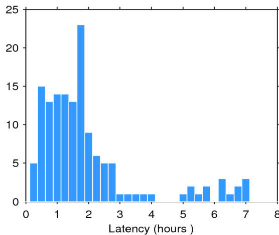
Figure 2. Histogram of the data latency for 04/06/2017. The y-axis denotes the number of files that are made available with a delay of x-hours with respect to the mean time of the records stored in the file.
