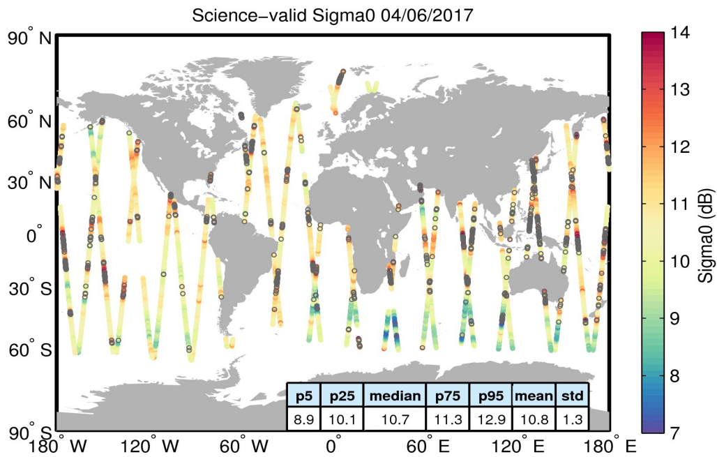
Figure 27. Geographical distribution of science-valid sigma0 data over oceans and lakes for 04/06/2017. The statistical values shown in the table refer to the sigma0 in dB and are calculated over all measurements shown in the figure. Gray circles denote records that have been rejected based on the editing criteria described in Table 4.
