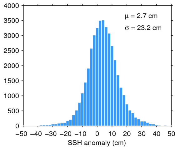
Figure 7. Histogram of flag-valid SSH anomaly over oceans and lakes for 04/06/2017. The mean ( \mu ) and standard deviation ( \sigma ) are also shown. Note that values outside [-50 50] cm are excluded from the histogram for the sake of readability but not from the computation of \mu and \sigma .
