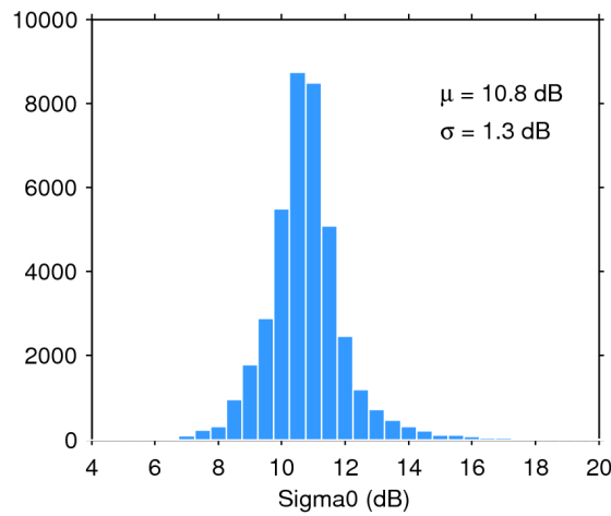
Figure 28. Histogram of science-valid sigma0 over oceans and lakes for 04/06/2017. The mean ( \mu ) and standard deviation ( \sigma ) are also shown. Note that values outside [4 20] dB are excluded from the histogram for the sake of readability but not from the computation of \mu and \sigma .
