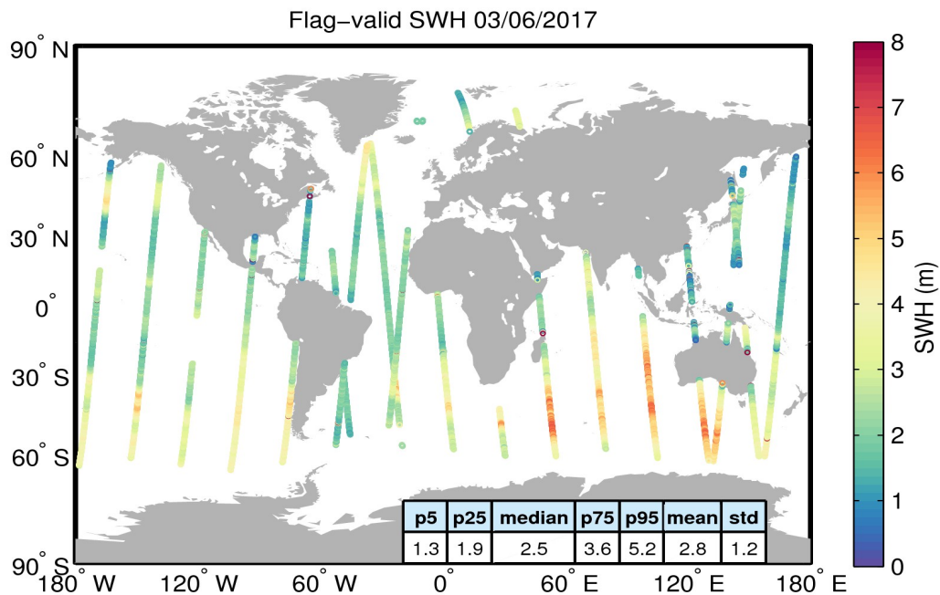
Figure 15. Geographical distribution of flag-valid SWH data over oceans and lakes for 03/06/2017. The statistical values shown in the table refer to the SWH in m and are calculated over all measurements shown in the figure.
