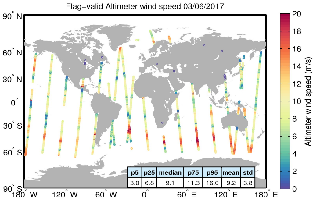
Figure 31. Geographical distribution of flag-valid wind data over oceans and lakes for 03/06/2017. The statistical values shown in the table refer to the wind in m/s and are calculated over all measurements shown in the figure.
