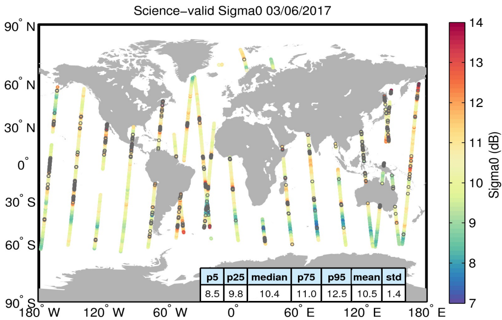
Figure 27. Geographical distribution of science-valid sigma0 data over oceans and lakes for 03/06/2017. The statistical values shown in the table refer to the sigma0 in dB and are calculated over all measurements shown in the figure. Gray circles denote records that have been rejected based on the editing criteria described in Table 4.
