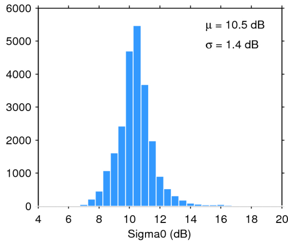
Figure 28. Histogram of science-valid sigma0 over oceans and lakes for 03/06/2017. The mean ( \mu ) and standard deviation ( \sigma ) are also shown. Note that values outside [4 20] dB are excluded from the histogram for the sake of readability but not from the computation of \mu and \sigma .
