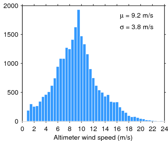
Figure 35. Histogram of science-valid wind over oceans and lakes for 03/06/2017. The mean ( \mu ) and standard deviation ( \sigma ) are also shown. Note that values larger than 24 m/s are excluded from the histogram for the sake of readability but not from the computation of \mu and \sigma .
