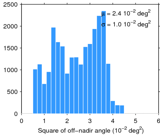
Figure 39. Histogram of flag-valid mispointing over oceans and lakes for 03/06/2017. The mean ( \mu ) and standard deviation ( \sigma ) are also shown. Note that values larger than 6 \cdot 10^{-2} \text{ deg}^2 are excluded from the histogram for the sake of readability but not from the computation of \mu and \sigma .
