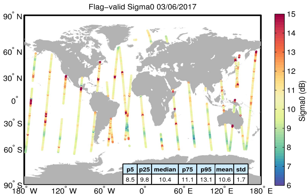
Figure 23. Geographical distribution of flag-valid sigma0 data over oceans and lakes for 03/06/2017. The statistical values shown in the table refer to the sigma0 in dB and are calculated over all measurements shown in the figure.
