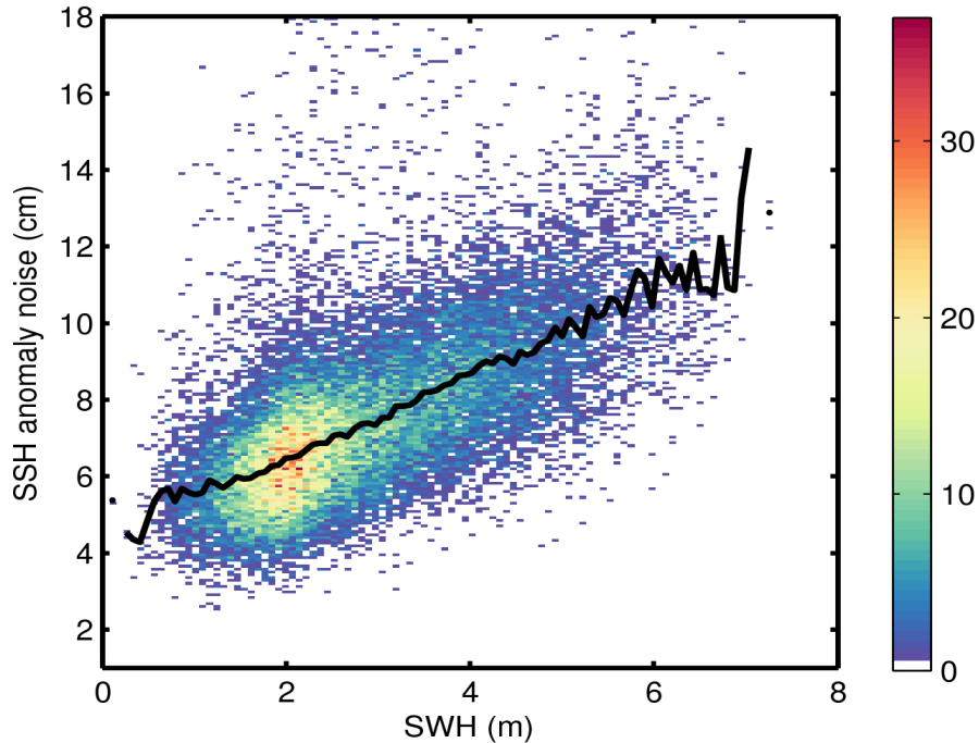
Figure 9. 2D histogram showing flag-valid SSH anomaly noise as a function of SWH for 03/06/2017. The black line denotes the median SSH anomaly noise as a function of SWH.
