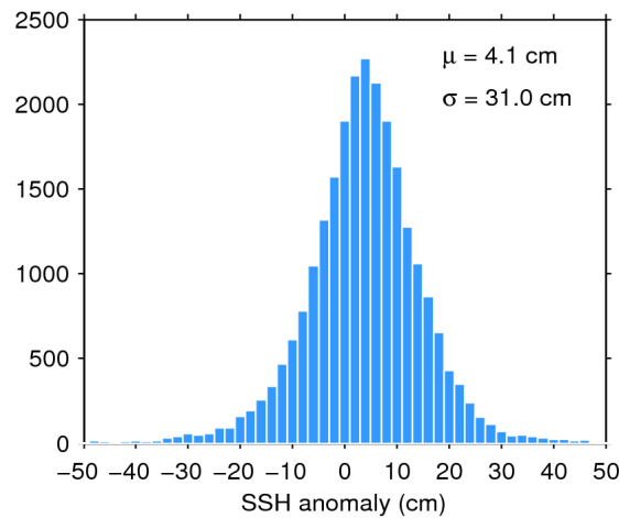
Figure 7. Histogram of flag-valid SSH anomaly over oceans and lakes for 03/06/2017. The mean ( \mu ) and standard deviation ( \sigma ) are also shown. Note that values outside [-50\ 50] cm are excluded from the histogram for the sake of readability but not from the computation of \mu and \sigma .
