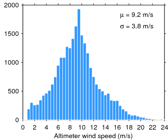
Figure 33. Histogram of flag-valid wind over oceans and lakes for 03/06/2017. The mean ( \mu ) and standard deviation ( \sigma ) are also shown. Note that values larger than 24 m/s are excluded from the histogram for the sake of readability but not from the computation of \mu and \sigma .
