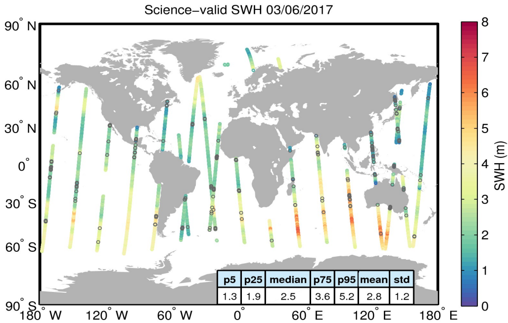
Figure 19. Geographical distribution of science-valid SWH data over oceans and lakes for 03/06/2017. The statistical values shown in the table refer to the SWH in m and are calculated over all measurements shown in the figure. Gray circles denote records that have been rejected based on the editing criteria described in Table 3.
