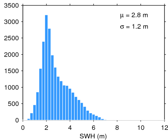
Figure 17. Histogram of flag-valid SWH over oceans and lakes for 03/06/2017. The mean ( \mu ) and standard deviation ( \sigma ) are also shown. Note that values larger than 12 m are excluded from the histogram for the sake of readability but not from the computation of \mu and \sigma .
