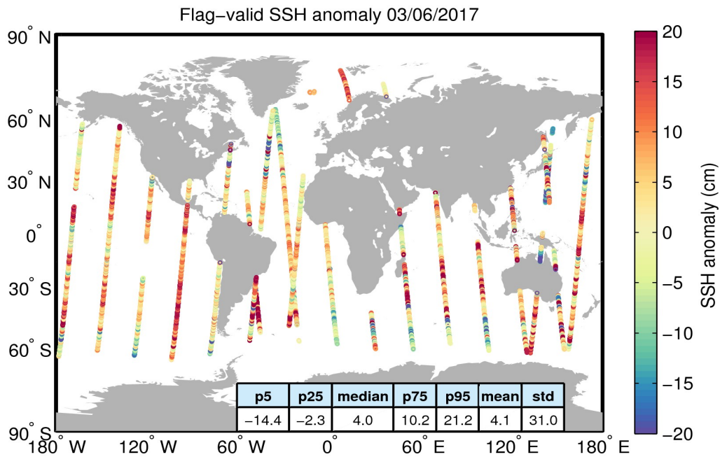
Figure 5. Geographical distribution of flag-valid 1-Hz SSH anomaly data over oceans and lakes for 03/06/2017. The statistical values shown in the table refer to the SSH anomaly in cm and are calculated over all measurements shown in the figure.
