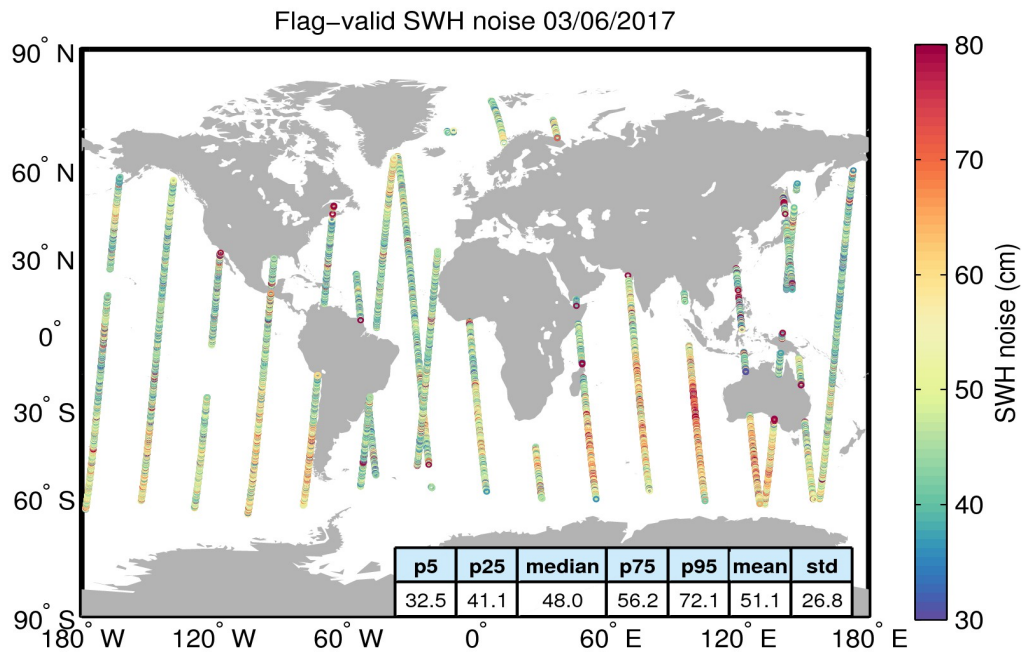
Figure 18. Geographical distribution of flag-valid 20-Hz SWH measurement noise over oceans and lakes for 03/06/2017. The statistical values shown in the table refer to the SWH noise and are calculated over all measurements shown in the figure.
