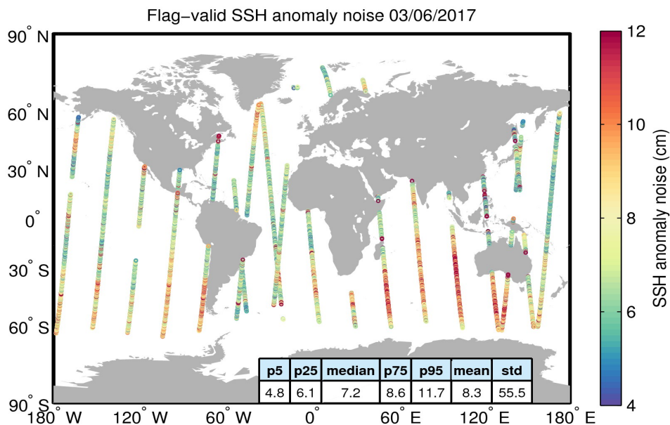
Figure 8. Geographical distribution of flag-valid 20-Hz SSH anomaly measurement noise over oceans and lakes for 03/06/2017. The statistical values shown in the table refer to the SSH anomaly noise and are calculated over all measurements shown in the figure.
