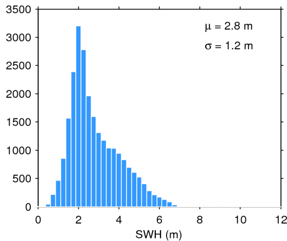
Figure 20. Histogram of science-valid SWH over oceans and lakes for 03/06/2017. The mean ( \mu ) and standard deviation ( \sigma ) are also shown. Note that values larger than 12 m are excluded from the histogram for the sake of readability but not from the computation of \mu and \sigma .
