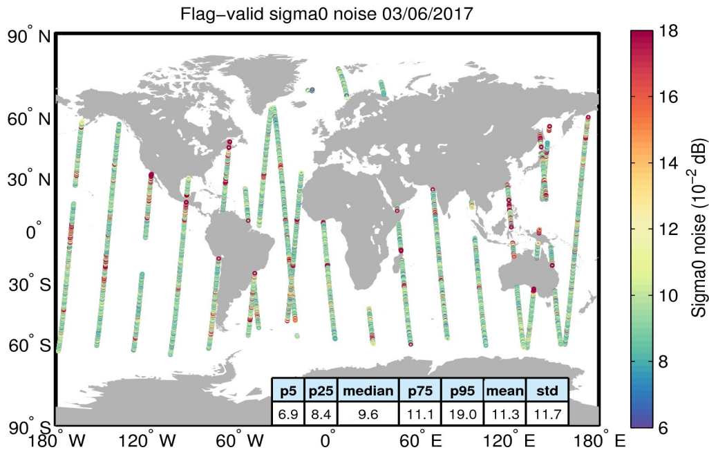
Figure 26. Geographical distribution of flag-valid 20-Hz sigma0 measurement noise over oceans and lakes for 03/06/2017. The statistical values shown in the table refer to the sigma0 noise and are calculated over all measurements shown in the figure.
