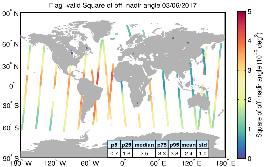
Figure 37. Geographical distribution of flag-valid mispointing data over oceans and lakes for 03/06/2017. The statistical values shown in the table refer to the mispointing in 10^{-2} deg 2 and are calculated over all measurements shown in the figure.
