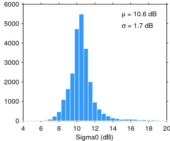
Figure 25. Histogram of flag-valid sigma0 over oceans and lakes for 03/06/2017. The mean ( \mu ) and standard deviation ( \sigma ) are also shown. Note that values outside [4 20] dB are excluded from the histogram for the sake of readability but not from the computation of \mu and \sigma .
