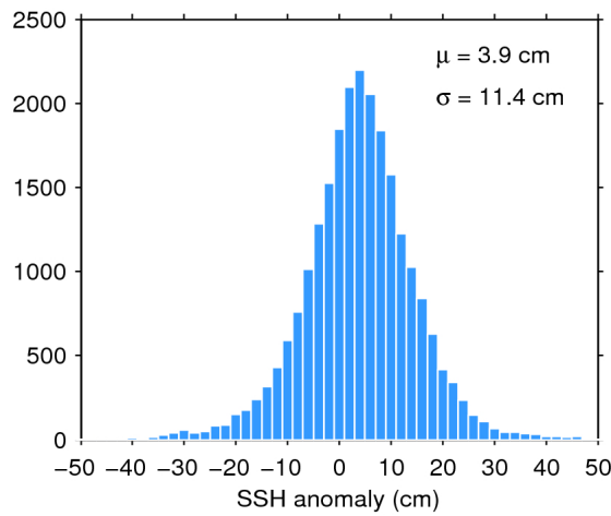
Figure 11. Histogram of science-valid SSH anomaly over oceans and lakes for 03/06/2017. The mean ( \mu ) and standard deviation ( \sigma ) are also shown. Note that values outside [-50 50] cm are excluded from the histogram for the sake of readability but not from the computation of \mu and \sigma .
