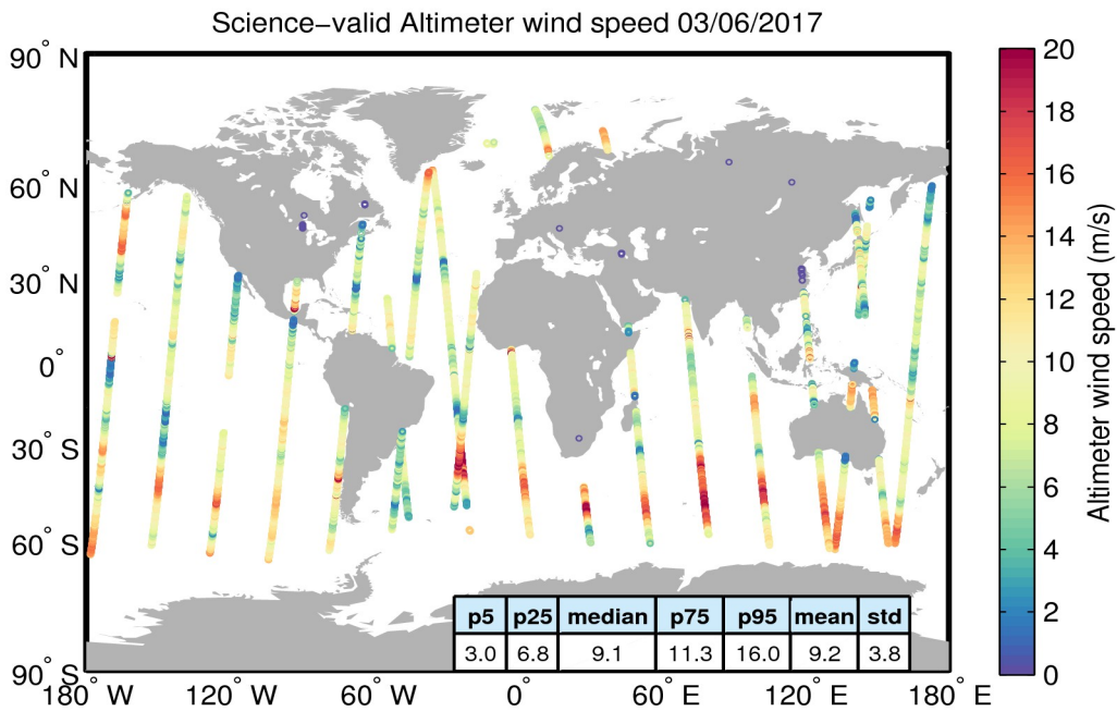
Figure 34. Geographical distribution of science-valid wind data over oceans and lakes for 03/06/2017. The statistical values shown in the table refer to the wind in m/s and are calculated over all measurements shown in the figure. Gray circles denote records that have been rejected based on the editing criteria described in Table 5.
