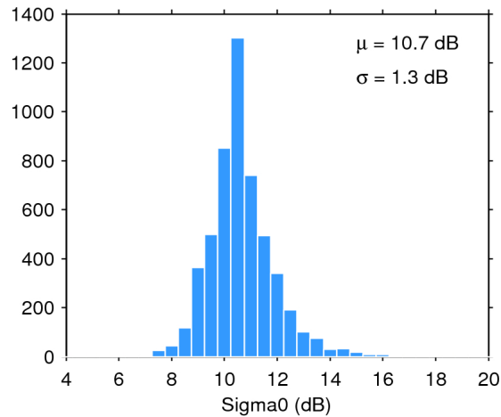
Figure 25. Histogram of flag-valid sigma0 over oceans and lakes for 02/06/2017. The mean ( \mu ) and standard deviation ( \sigma ) are also shown. Note that values outside [4 20] dB are excluded from the histogram for the sake of readability but not from the computation of \mu and \sigma .
