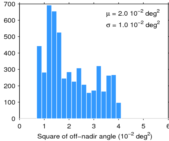
Figure 39. Histogram of flag-valid mispointing over oceans and lakes for 02/06/2017. The mean ( \mu ) and standard deviation ( \sigma ) are also shown. Note that values larger than 6 \cdot 10^{-2} \text{ deg}^2 are excluded from the histogram for the sake of readability but not from the computation of \mu and \sigma .
