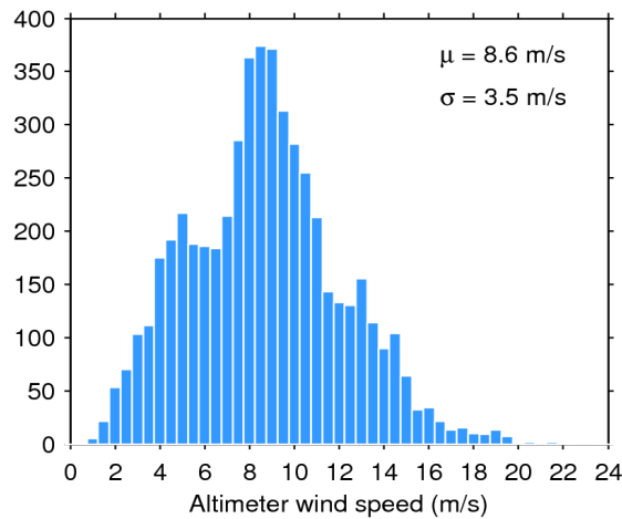
Figure 33. Histogram of flag-valid wind over oceans and lakes for 02/06/2017. The mean ( \mu ) and standard deviation ( \sigma ) are also shown. Note that values larger than 24 m/s are excluded from the histogram for the sake of readability but not from the computation of \mu and \sigma .
