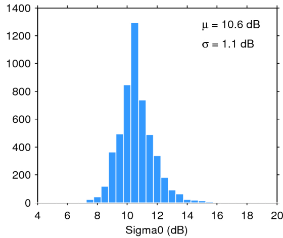
Figure 28. Histogram of science-valid sigma0 over oceans and lakes for 02/06/2017. The mean ( \mu ) and standard deviation ( \sigma ) are also shown. Note that values outside [4 20] dB are excluded from the histogram for the sake of readability but not from the computation of \mu and \sigma .
