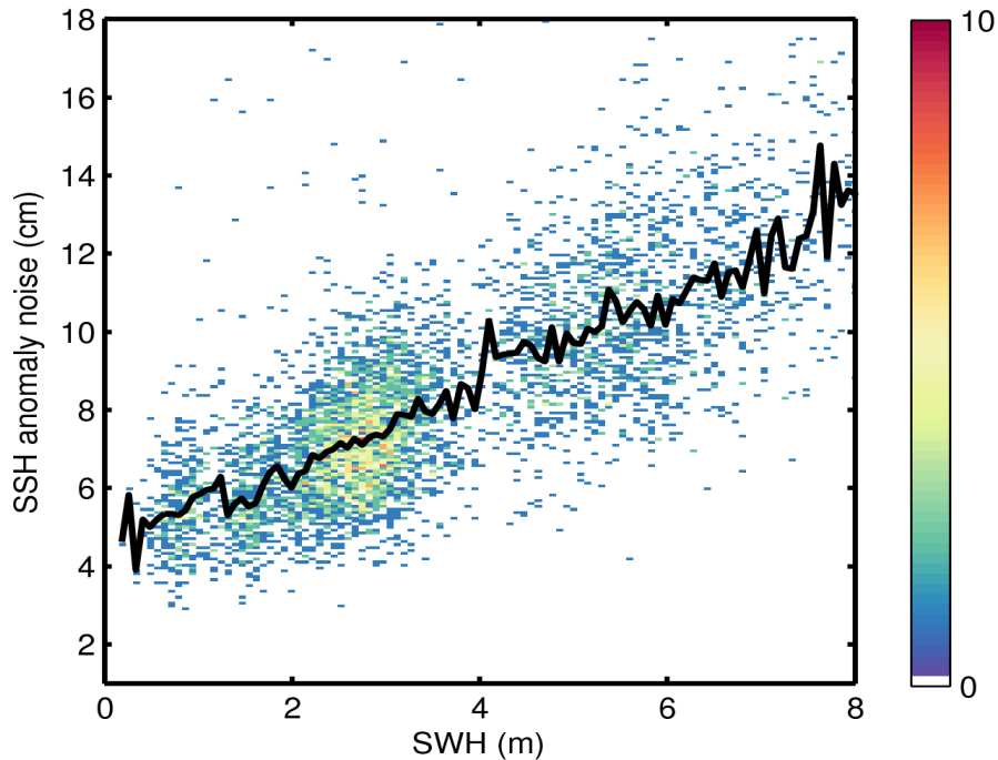
Figure 9. 2D histogram showing flag-valid SSH anomaly noise as a function of SWH for 02/06/2017. The black line denotes the median SSH anomaly noise as a function of SWH.
