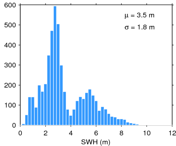
Figure 20. Histogram of science-valid SWH over oceans and lakes for 02/06/2017. The mean ( \mu ) and standard deviation ( \sigma ) are also shown. Note that values larger than 12 m are excluded from the histogram for the sake of readability but not from the computation of \mu and \sigma .
