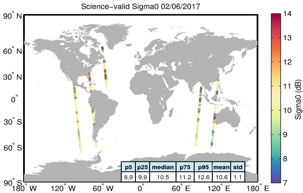
Figure 27. Geographical distribution of science-valid sigma0 data over oceans and lakes for 02/06/2017. The statistical values shown in the table refer to the sigma0 in dB and are calculated over all measurements shown in the figure. Gray circles denote records that have been rejected based on the editing criteria described in Table 4.
