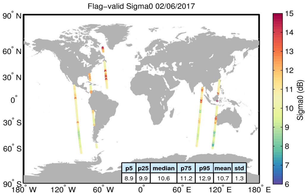
Figure 23. Geographical distribution of flag-valid sigma0 data over oceans and lakes for 02/06/2017. The statistical values shown in the table refer to the sigma0 in dB and are calculated over all measurements shown in the figure.
