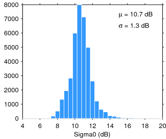
Figure 28. Histogram of science-valid sigma0 over oceans and lakes for 01/06/2017. The mean ( \mu ) and standard deviation ( \sigma ) are also shown. Note that values outside [4 20] dB are excluded from the histogram for the sake of readability but not from the computation of \mu and \sigma .
