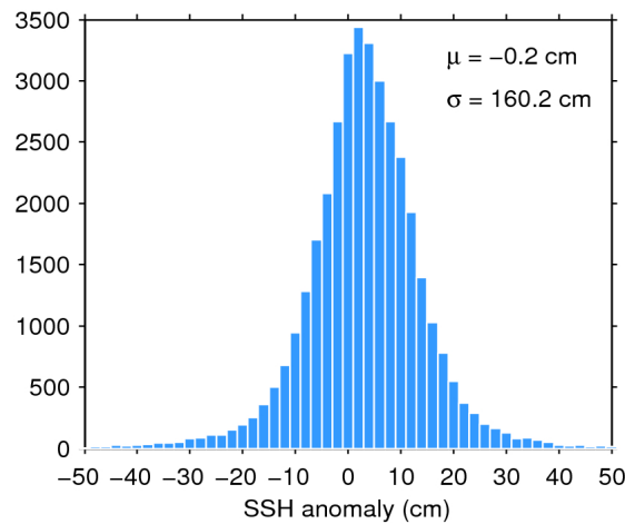
Figure 7. Histogram of flag-valid SSH anomaly over oceans and lakes for 01/06/2017. The mean ( \mu ) and standard deviation ( \sigma ) are also shown. Note that values outside [-50 50] cm are excluded from the histogram for the sake of readability but not from the computation of \mu and \sigma .
