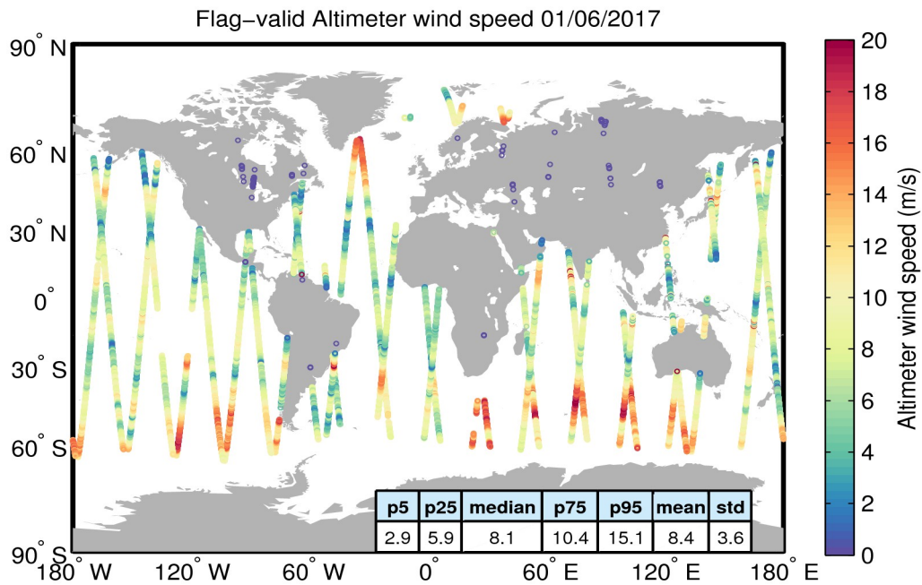
Figure 31. Geographical distribution of flag-valid wind data over oceans and lakes for 01/06/2017. The statistical values shown in the table refer to the wind in m/s and are calculated over all measurements shown in the figure.
