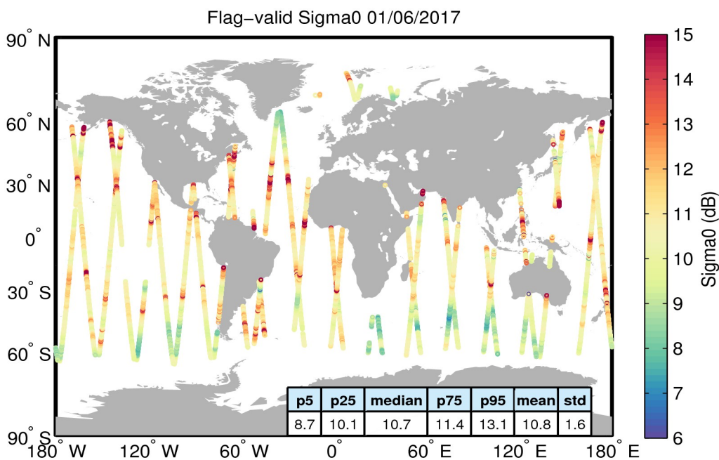
Figure 23. Geographical distribution of flag-valid sigma0 data over oceans and lakes for 01/06/2017. The statistical values shown in the table refer to the sigma0 in dB and are calculated over all measurements shown in the figure.
