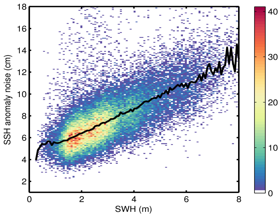
Figure 9. 2D histogram showing flag-valid SSH anomaly noise as a function of SWH for 01/06/2017. The black line denotes the median SSH anomaly noise as a function of SWH.
