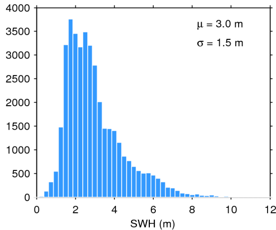
Figure 20. Histogram of science-valid SWH over oceans and lakes for 01/06/2017. The mean ( \mu ) and standard deviation ( \sigma ) are also shown. Note that values larger than 12 m are excluded from the histogram for the sake of readability but not from the computation of \mu and \sigma .
