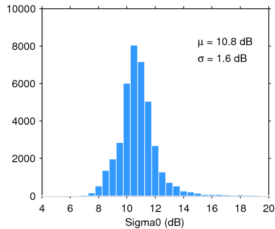
Figure 25. Histogram of flag-valid sigma0 over oceans and lakes for 01/06/2017. The mean ( \mu ) and standard deviation ( \sigma ) are also shown. Note that values outside [4 20] dB are excluded from the histogram for the sake of readability but not from the computation of \mu and \sigma .
