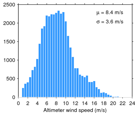
Figure 35. Histogram of science-valid wind over oceans and lakes for 01/06/2017. The mean ( \mu ) and standard deviation ( \sigma ) are also shown. Note that values larger than 24 m/s are excluded from the histogram for the sake of readability but not from the computation of \mu and \sigma .
