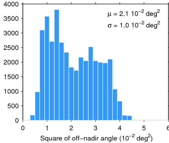
Figure 39. Histogram of flag-valid mispointing over oceans and lakes for 01/06/2017. The mean ( \mu ) and standard deviation ( \sigma ) are also shown. Note that values larger than 6 \cdot 10^{-2} \text{ deg}^2 are excluded from the histogram for the sake of readability but not from the computation of \mu and \sigma .
