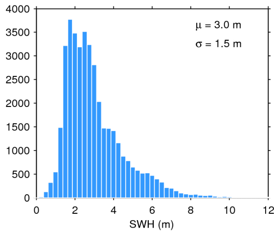
Figure 17. Histogram of flag-valid SWH over oceans and lakes for 01/06/2017. The mean ( \mu ) and standard deviation ( \sigma ) are also shown. Note that values larger than 12 m are excluded from the histogram for the sake of readability but not from the computation of \mu and \sigma .
