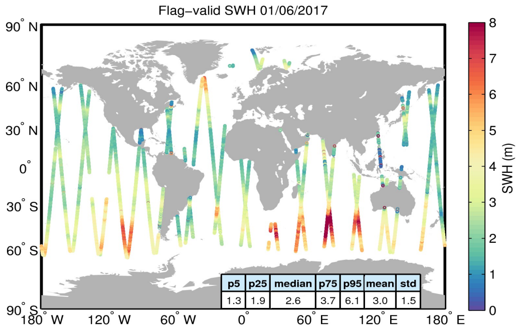
Figure 15. Geographical distribution of flag-valid SWH data over oceans and lakes for 01/06/2017. The statistical values shown in the table refer to the SWH in m and are calculated over all measurements shown in the figure.
