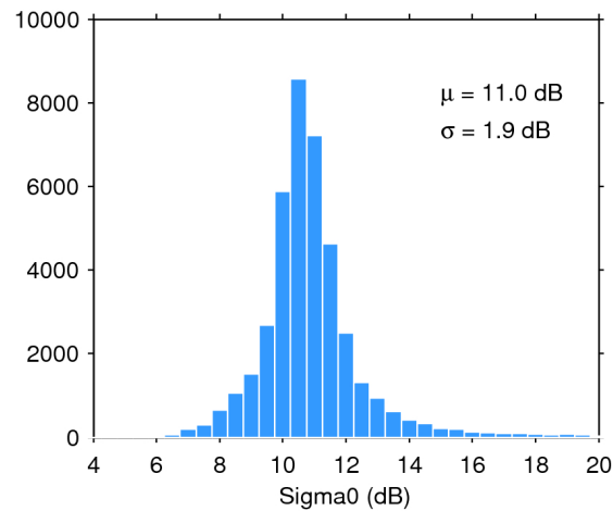
Figure 25. Histogram of flag-valid sigma0 over oceans and lakes for 31/05/2017. The mean ( \mu ) and standard deviation ( \sigma ) are also shown. Note that values outside [4 20] dB are excluded from the histogram for the sake of readability but not from the computation of \mu and \sigma .
