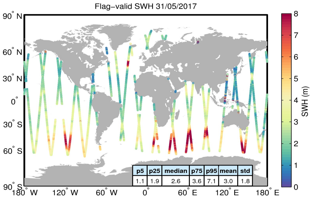
Figure 15. Geographical distribution of flag-valid SWH data over oceans and lakes for 31/05/2017. The statistical values shown in the table refer to the SWH in m and are calculated over all measurements shown in the figure.
