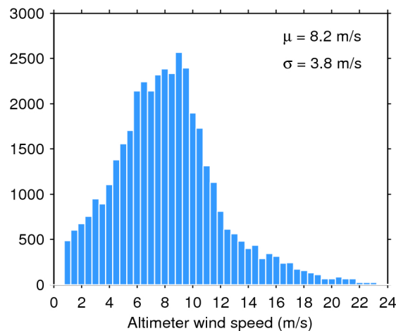
Figure 35. Histogram of science-valid wind over oceans and lakes for 31/05/2017. The mean ( \mu ) and standard deviation ( \sigma ) are also shown. Note that values larger than 24 m/s are excluded from the histogram for the sake of readability but not from the computation of \mu and \sigma .
