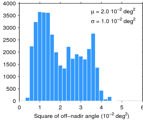
Figure 39. Histogram of flag-valid mispointing over oceans and lakes for 31/05/2017. The mean ( \mu ) and standard deviation ( \sigma ) are also shown. Note that values larger than 6 \cdot 10^{-2} \text{ deg}^2 are excluded from the histogram for the sake of readability but not from the computation of \mu and \sigma .
