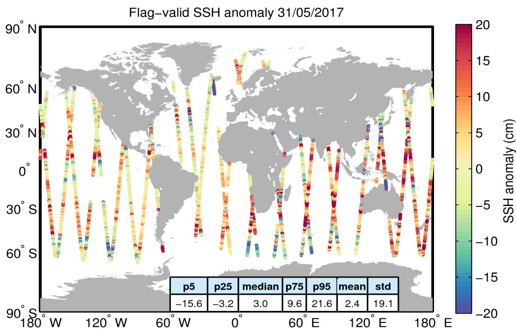
Figure 5. Geographical distribution of flag-valid 1-Hz SSH anomaly data over oceans and lakes for 31/05/2017. The statistical values shown in the table refer to the SSH anomaly in cm and are calculated over all measurements shown in the figure.
