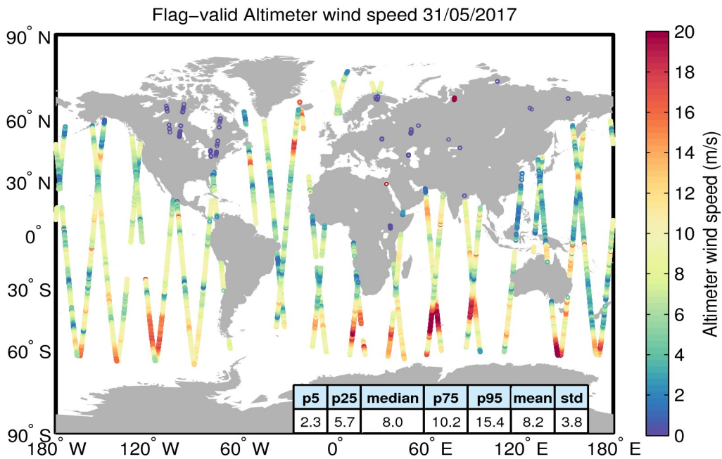
Figure 31. Geographical distribution of flag-valid wind data over oceans and lakes for 31/05/2017. The statistical values shown in the table refer to the wind in m/s and are calculated over all measurements shown in the figure.
