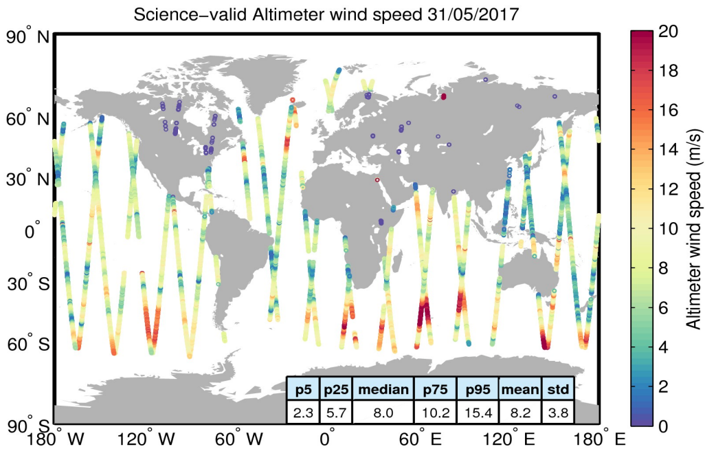
Figure 34. Geographical distribution of science-valid wind data over oceans and lakes for 31/05/2017. The statistical values shown in the table refer to the wind in m/s and are calculated over all measurements shown in the figure. Gray circles denote records that have been rejected based on the editing criteria described in Table 5.
