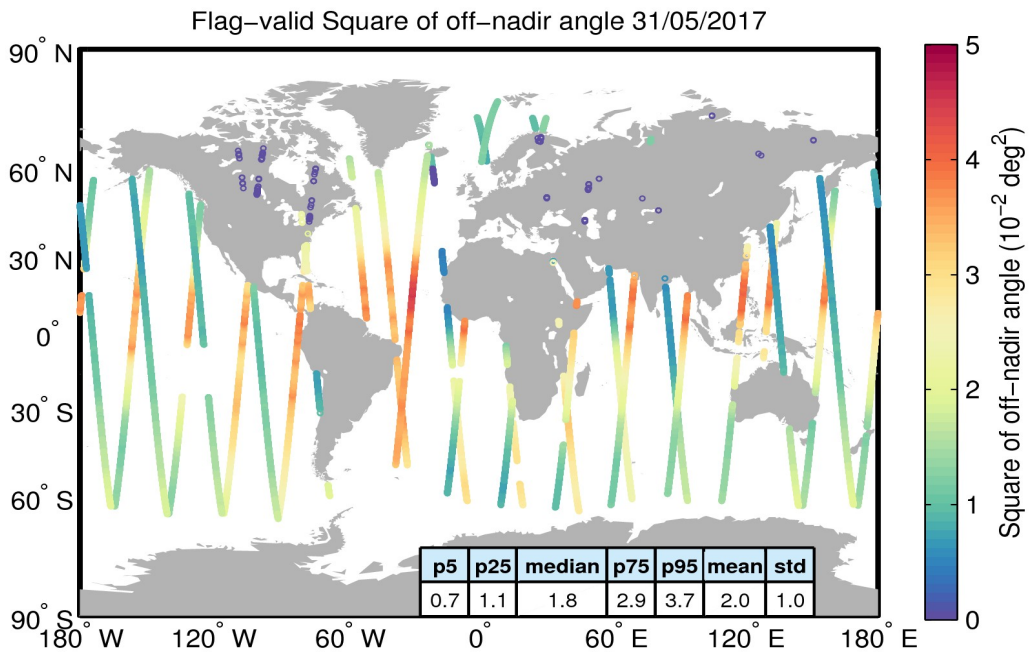
Figure 37. Geographical distribution of flag-valid mispointing data over oceans and lakes for 31/05/2017. The statistical values shown in the table refer to the mispointing in 10^{-2} deg 2 and are calculated over all measurements shown in the figure.
