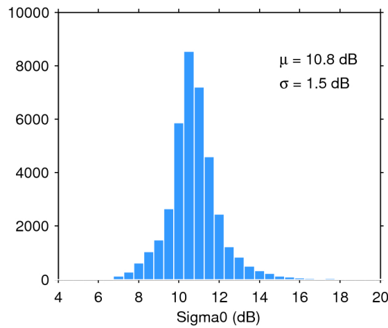
Figure 28. Histogram of science-valid sigma0 over oceans and lakes for 31/05/2017. The mean ( \mu ) and standard deviation ( \sigma ) are also shown. Note that values outside [4 20] dB are excluded from the histogram for the sake of readability but not from the computation of \mu and \sigma .
