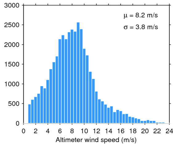
Figure 33. Histogram of flag-valid wind over oceans and lakes for 31/05/2017. The mean ( \mu ) and standard deviation ( \sigma ) are also shown. Note that values larger than 24 m/s are excluded from the histogram for the sake of readability but not from the computation of \mu and \sigma .
