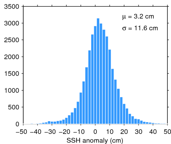
Figure 11. Histogram of science-valid SSH anomaly over oceans and lakes for 31/05/2017. The mean ( \mu ) and standard deviation ( \sigma ) are also shown. Note that values outside [-50 50] cm are excluded from the histogram for the sake of readability but not from the computation of \mu and \sigma .
