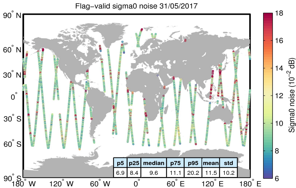
Figure 26. Geographical distribution of flag-valid 20-Hz sigma0 measurement noise over oceans and lakes for 31/05/2017. The statistical values shown in the table refer to the sigma0 noise and are calculated over all measurements shown in the figure.
