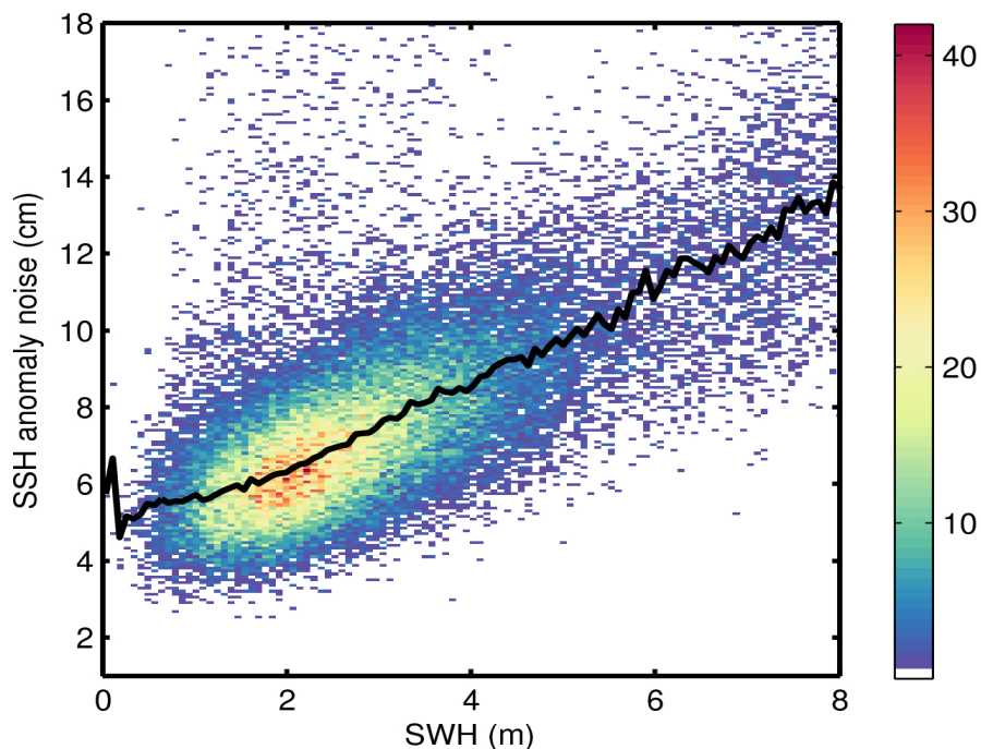
Figure 9. 2D histogram showing flag-valid SSH anomaly noise as a function of SWH for 31/05/2017. The black line denotes the median SSH anomaly noise as a function of SWH.
