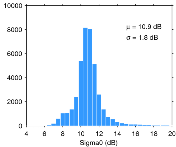
Figure 25. Histogram of flag-valid sigma0 over oceans and lakes for 30/05/2017. The mean ( \mu ) and standard deviation ( \sigma ) are also shown. Note that values outside [4 20] dB are excluded from the histogram for the sake of readability but not from the computation of \mu and \sigma .
