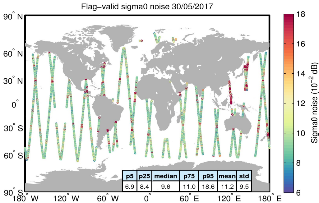
Figure 26. Geographical distribution of flag-valid 20-Hz sigma0 measurement noise over oceans and lakes for 30/05/2017. The statistical values shown in the table refer to the sigma0 noise and are calculated over all measurements shown in the figure.
