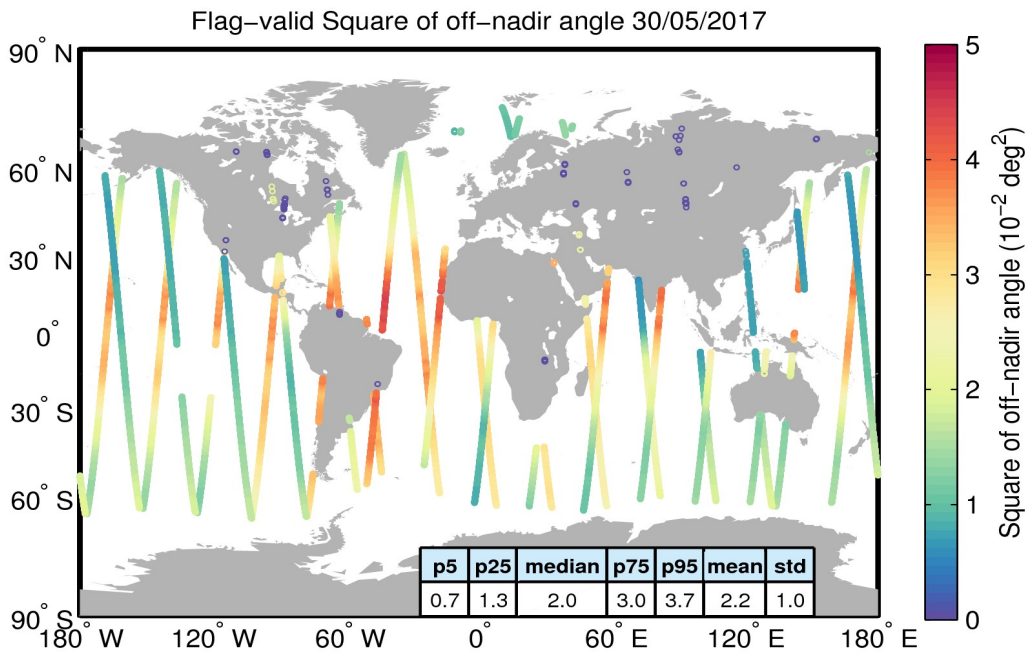
Figure 37. Geographical distribution of flag-valid mispointing data over oceans and lakes for 30/05/2017. The statistical values shown in the table refer to the mispointing in 10^{-2} deg 2 and are calculated over all measurements shown in the figure.
