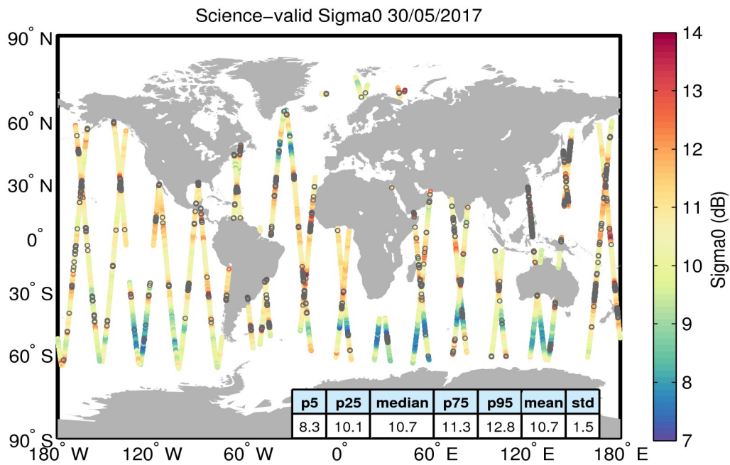
Figure 27. Geographical distribution of science-valid sigma0 data over oceans and lakes for 30/05/2017. The statistical values shown in the table refer to the sigma0 in dB and are calculated over all measurements shown in the figure. Gray circles denote records that have been rejected based on the editing criteria described in Table 4.
