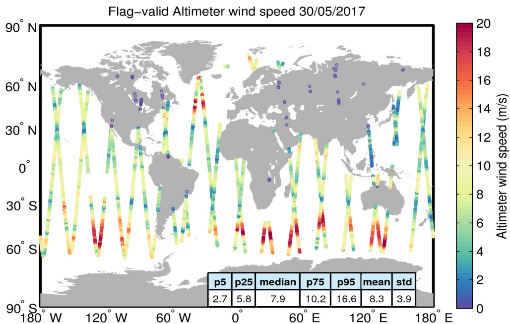
Figure 31. Geographical distribution of flag-valid wind data over oceans and lakes for 30/05/2017. The statistical values shown in the table refer to the wind in m/s and are calculated over all measurements shown in the figure.
