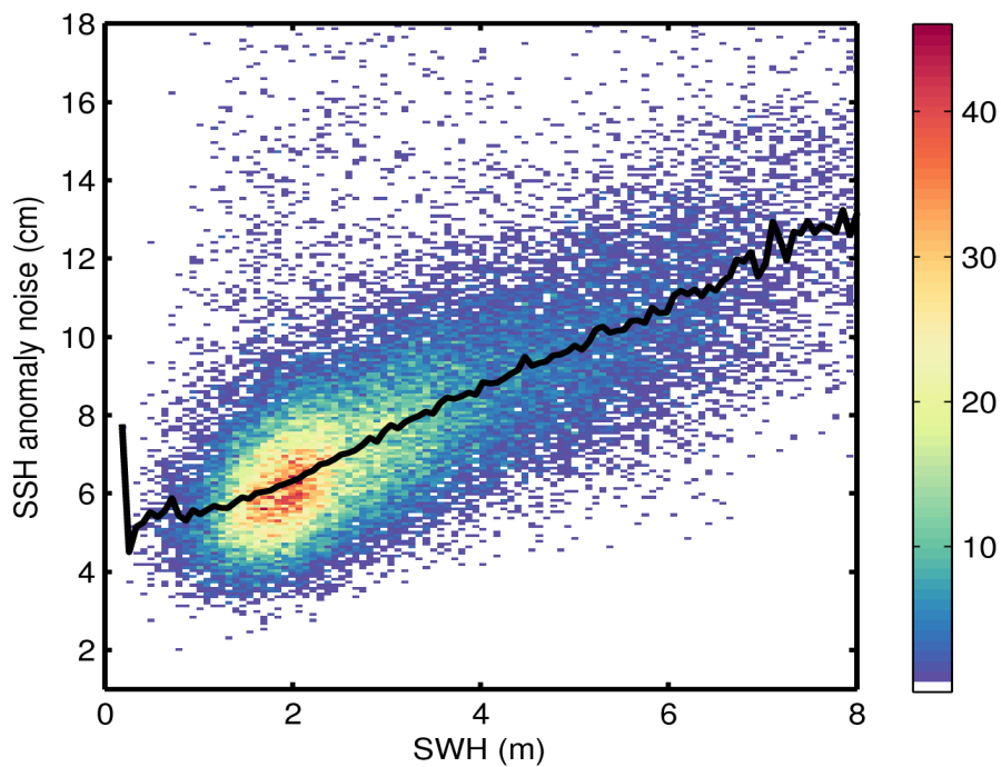
Figure 9. 2D histogram showing flag-valid SSH anomaly noise as a function of SWH for 30/05/2017. The black line denotes the median SSH anomaly noise as a function of SWH.
