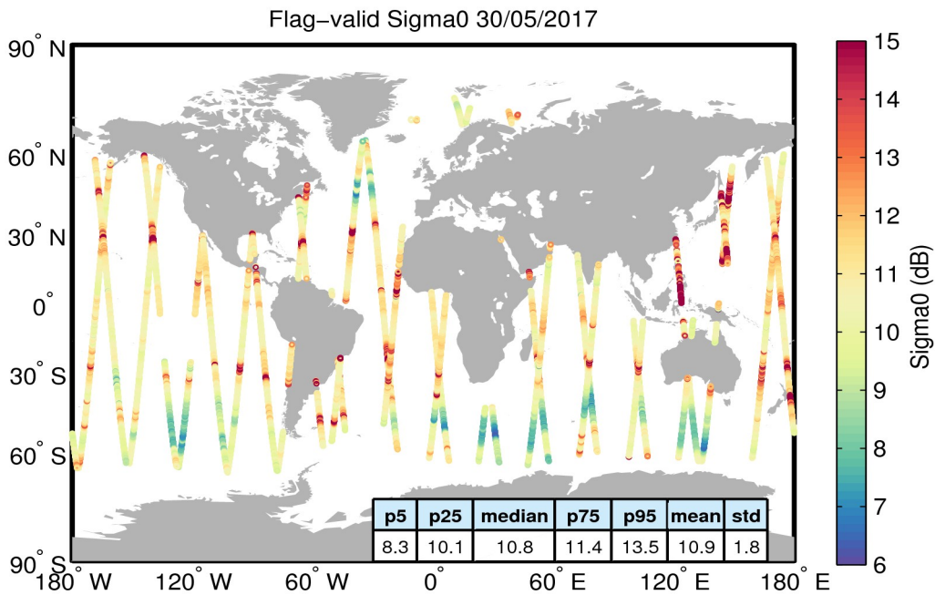
Figure 23. Geographical distribution of flag-valid sigma0 data over oceans and lakes for 30/05/2017. The statistical values shown in the table refer to the sigma0 in dB and are calculated over all measurements shown in the figure.
