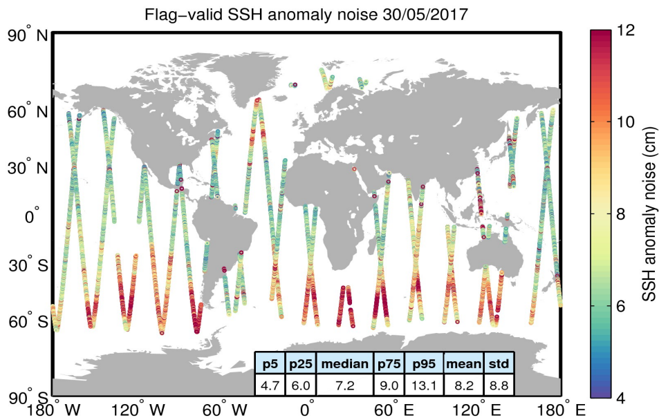
Figure 8. Geographical distribution of flag-valid 20-Hz SSH anomaly measurement noise over oceans and lakes for 30/05/2017. The statistical values shown in the table refer to the SSH anomaly noise and are calculated over all measurements shown in the figure.
