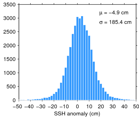
Figure 7. Histogram of flag-valid SSH anomaly over oceans and lakes for 30/05/2017. The mean ( \mu ) and standard deviation ( \sigma ) are also shown. Note that values outside [-50 50] cm are excluded from the histogram for the sake of readability but not from the computation of \mu and \sigma .
