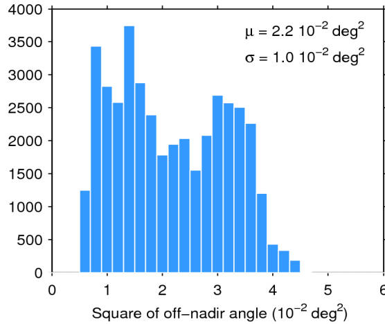
Figure 39. Histogram of flag-valid mispointing over oceans and lakes for 30/05/2017. The mean ( \mu ) and standard deviation ( \sigma ) are also shown. Note that values larger than 6 \cdot 10^{-2} \text{ deg}^2 are excluded from the histogram for the sake of readability but not from the computation of \mu and \sigma .
