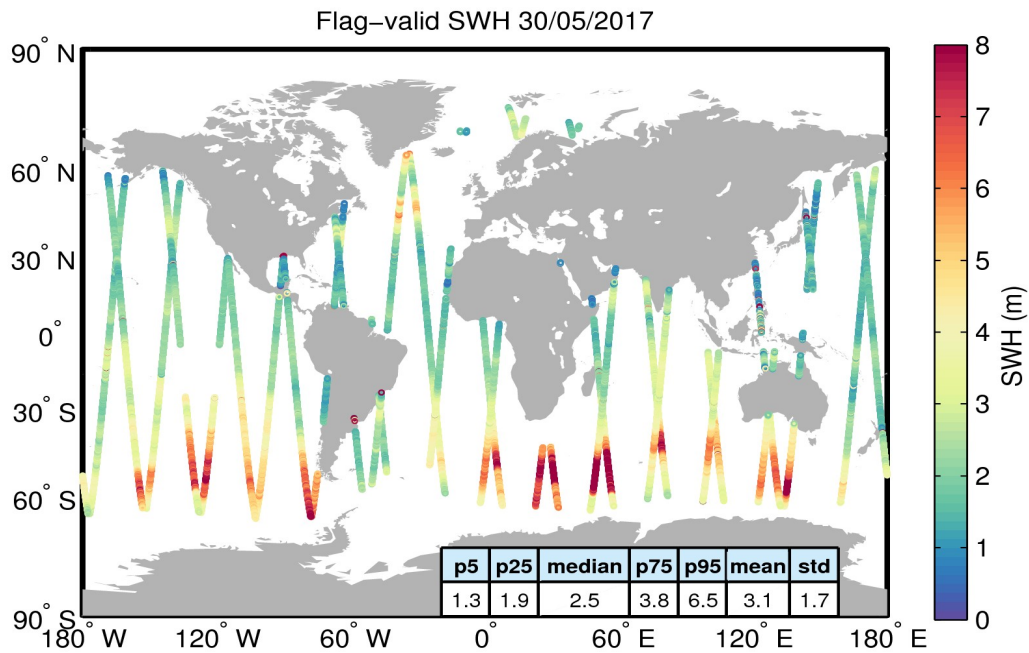
Figure 15. Geographical distribution of flag-valid SWH data over oceans and lakes for 30/05/2017. The statistical values shown in the table refer to the SWH in m and are calculated over all measurements shown in the figure.
