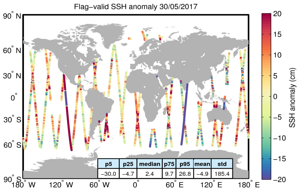
Figure 5. Geographical distribution of flag-valid 1-Hz SSH anomaly data over oceans and lakes for 30/05/2017. The statistical values shown in the table refer to the SSH anomaly in cm and are calculated over all measurements shown in the figure.
