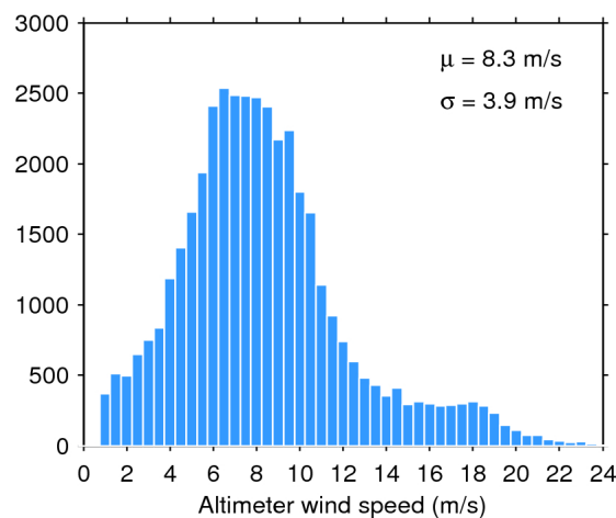
Figure 35. Histogram of science-valid wind over oceans and lakes for 30/05/2017. The mean ( \mu ) and standard deviation ( \sigma ) are also shown. Note that values larger than 24 m/s are excluded from the histogram for the sake of readability but not from the computation of \mu and \sigma .
