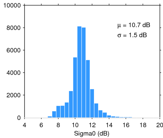
Figure 28. Histogram of science-valid sigma0 over oceans and lakes for 30/05/2017. The mean ( \mu ) and standard deviation ( \sigma ) are also shown. Note that values outside [4 20] dB are excluded from the histogram for the sake of readability but not from the computation of \mu and \sigma .
