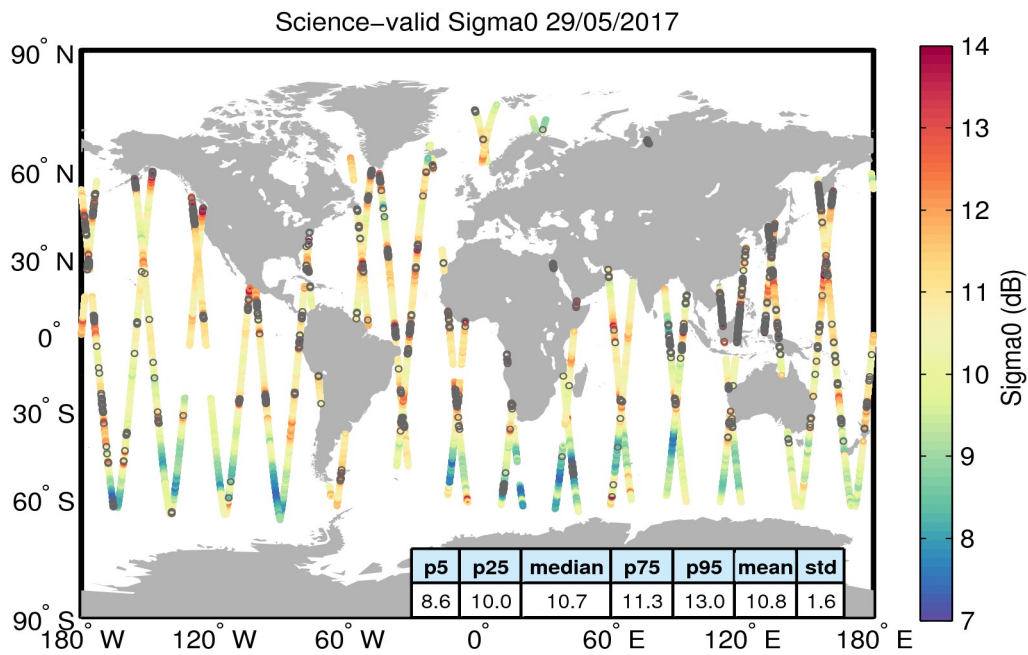
Figure 27. Geographical distribution of science-valid sigma0 data over oceans and lakes for 29/05/2017. The statistical values shown in the table refer to the sigma0 in dB and are calculated over all measurements shown in the figure. Gray circles denote records that have been rejected based on the editing criteria described in Table 4.
