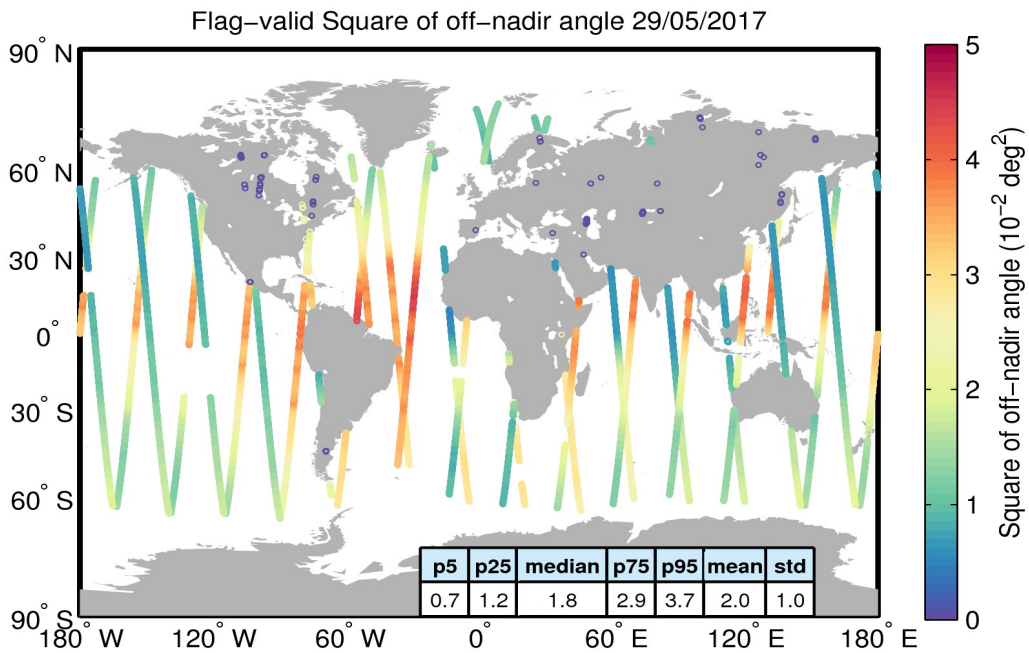
Figure 37. Geographical distribution of flag-valid mispointing data over oceans and lakes for 29/05/2017. The statistical values shown in the table refer to the mispointing in 10^{-2} deg 2 and are calculated over all measurements shown in the figure.
