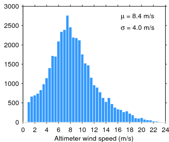
Figure 35. Histogram of science-valid wind over oceans and lakes for 29/05/2017. The mean ( \mu ) and standard deviation ( \sigma ) are also shown. Note that values larger than 24 m/s are excluded from the histogram for the sake of readability but not from the computation of \mu and \sigma .
