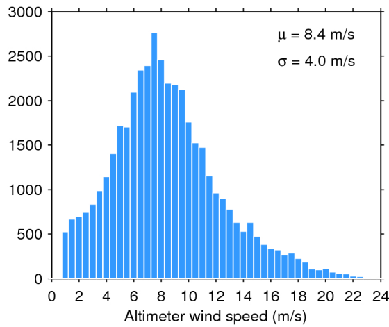
Figure 33. Histogram of flag-valid wind over oceans and lakes for 29/05/2017. The mean ( \mu ) and standard deviation ( \sigma ) are also shown. Note that values larger than 24 m/s are excluded from the histogram for the sake of readability but not from the computation of \mu and \sigma .
