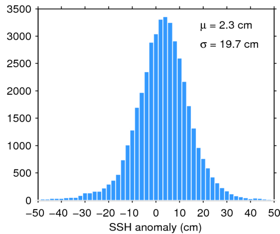
Figure 7. Histogram of flag-valid SSH anomaly over oceans and lakes for 29/05/2017. The mean ( \mu ) and standard deviation ( \sigma ) are also shown. Note that values outside [-50 50] cm are excluded from the histogram for the sake of readability but not from the computation of \mu and \sigma .
