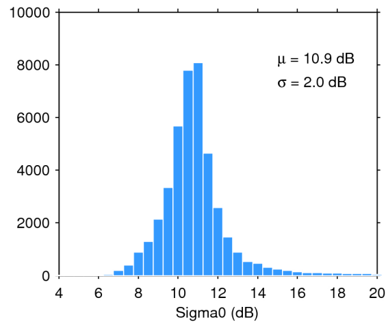
Figure 25. Histogram of flag-valid sigma0 over oceans and lakes for 29/05/2017. The mean ( \mu ) and standard deviation ( \sigma ) are also shown. Note that values outside [4 20] dB are excluded from the histogram for the sake of readability but not from the computation of \mu and \sigma .
