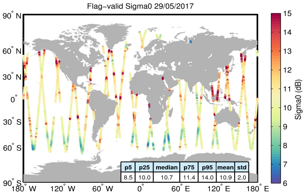
Figure 23. Geographical distribution of flag-valid sigma0 data over oceans and lakes for 29/05/2017. The statistical values shown in the table refer to the sigma0 in dB and are calculated over all measurements shown in the figure.
