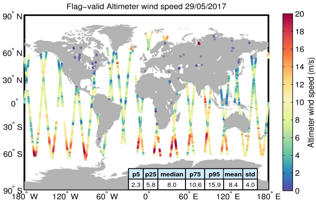
Figure 31. Geographical distribution of flag-valid wind data over oceans and lakes for 29/05/2017. The statistical values shown in the table refer to the wind in m/s and are calculated over all measurements shown in the figure.
