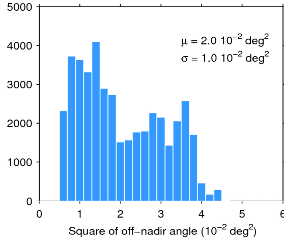
Figure 39. Histogram of flag-valid mispointing over oceans and lakes for 29/05/2017. The mean ( \mu ) and standard deviation ( \sigma ) are also shown. Note that values larger than 6 \cdot 10^{-2} \text{ deg}^2 are excluded from the histogram for the sake of readability but not from the computation of \mu and \sigma .
