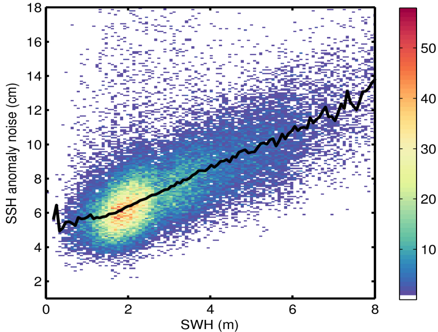
Figure 9. 2D histogram showing flag-valid SSH anomaly noise as a function of SWH for 29/05/2017. The black line denotes the median SSH anomaly noise as a function of SWH.
