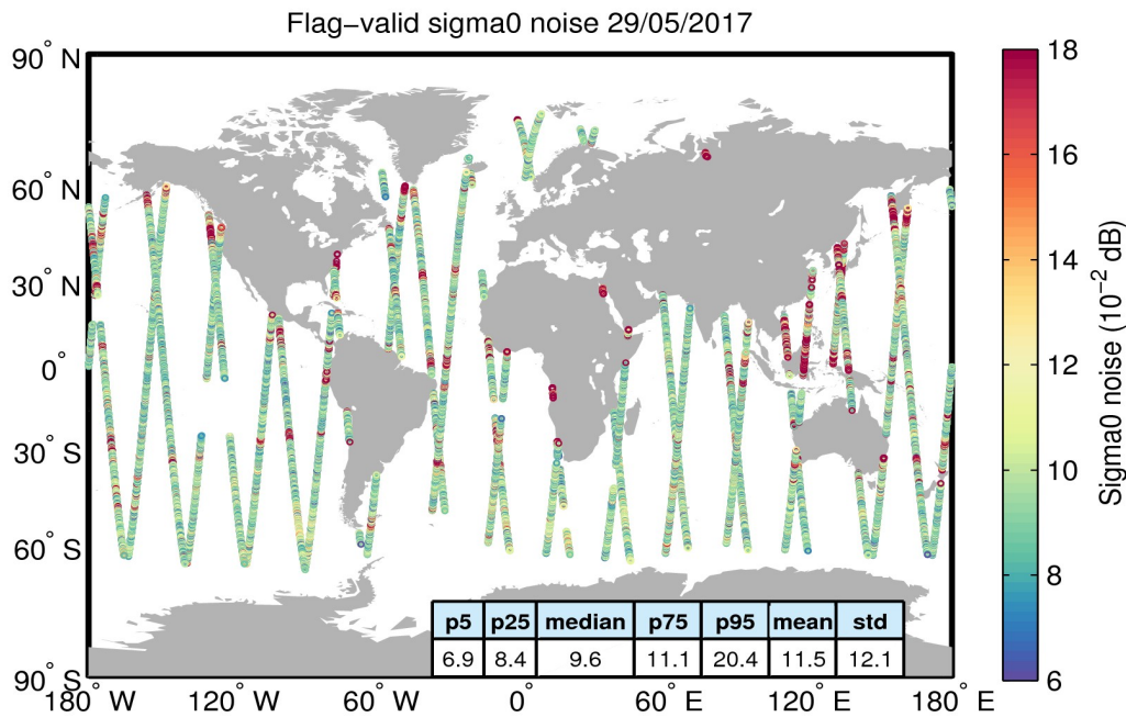
Figure 26. Geographical distribution of flag-valid 20-Hz sigma0 measurement noise over oceans and lakes for 29/05/2017. The statistical values shown in the table refer to the sigma0 noise and are calculated over all measurements shown in the figure.
