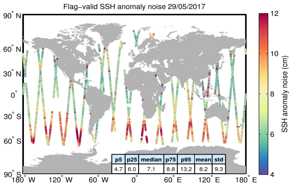
Figure 8. Geographical distribution of flag-valid 20-Hz SSH anomaly measurement noise over oceans and lakes for 29/05/2017. The statistical values shown in the table refer to the SSH anomaly noise and are calculated over all measurements shown in the figure.
