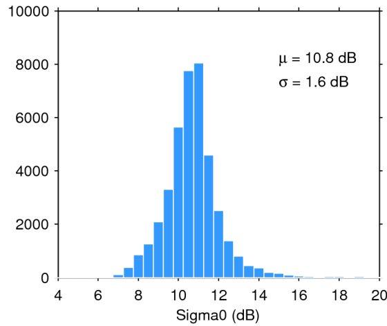
Figure 28. Histogram of science-valid sigma0 over oceans and lakes for 29/05/2017. The mean ( \mu ) and standard deviation ( \sigma ) are also shown. Note that values outside [4 20] dB are excluded from the histogram for the sake of readability but not from the computation of \mu and \sigma .
