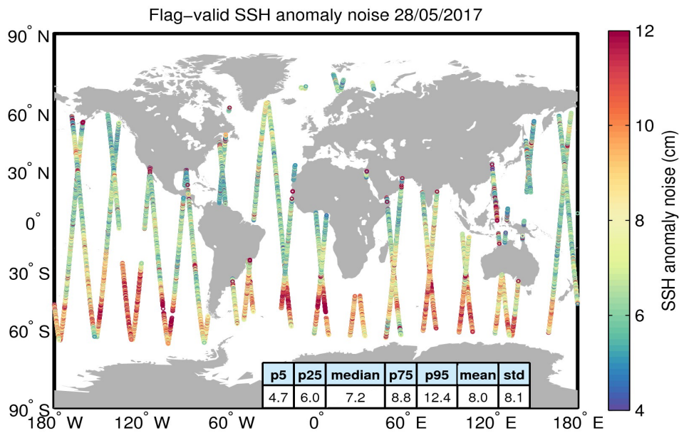
Figure 8. Geographical distribution of flag-valid 20-Hz SSH anomaly measurement noise over oceans and lakes for 28/05/2017. The statistical values shown in the table refer to the SSH anomaly noise and are calculated over all measurements shown in the figure.
