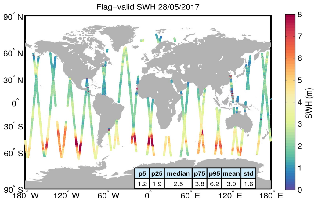
Figure 15. Geographical distribution of flag-valid SWH data over oceans and lakes for 28/05/2017. The statistical values shown in the table refer to the SWH in m and are calculated over all measurements shown in the figure.
