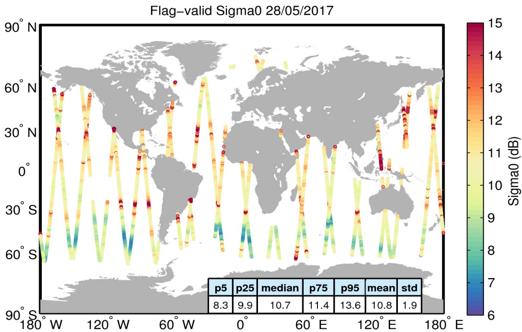
Figure 23. Geographical distribution of flag-valid sigma0 data over oceans and lakes for 28/05/2017. The statistical values shown in the table refer to the sigma0 in dB and are calculated over all measurements shown in the figure.
