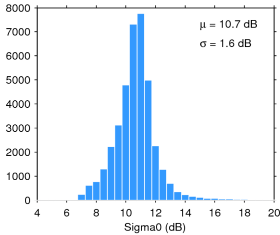
Figure 28. Histogram of science-valid sigma0 over oceans and lakes for 28/05/2017. The mean ( \mu ) and standard deviation ( \sigma ) are also shown. Note that values outside [4 20] dB are excluded from the histogram for the sake of readability but not from the computation of \mu and \sigma .
