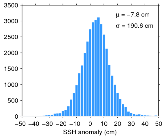
Figure 7. Histogram of flag-valid SSH anomaly over oceans and lakes for 28/05/2017. The mean ( \mu ) and standard deviation ( \sigma ) are also shown. Note that values outside [-50 50] cm are excluded from the histogram for the sake of readability but not from the computation of \mu and \sigma .
