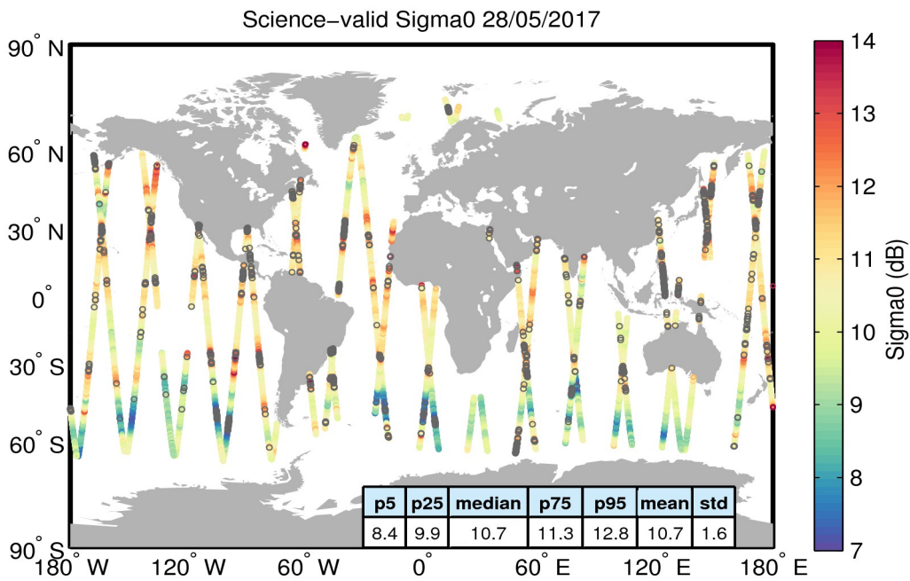
Figure 27. Geographical distribution of science-valid sigma0 data over oceans and lakes for 28/05/2017. The statistical values shown in the table refer to the sigma0 in dB and are calculated over all measurements shown in the figure. Gray circles denote records that have been rejected based on the editing criteria described in Table 4.
