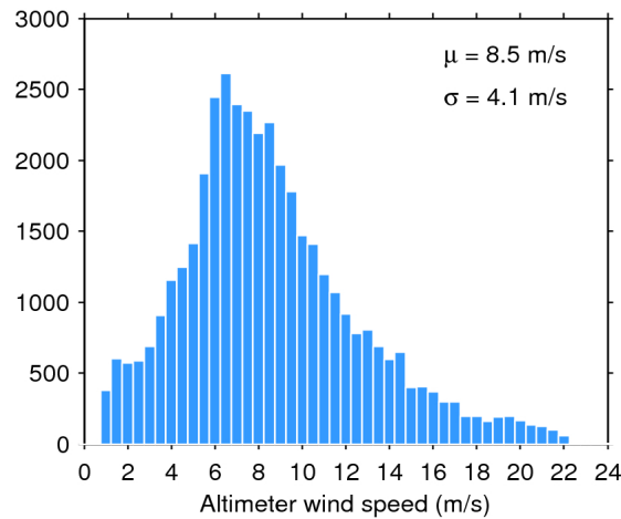
Figure 33. Histogram of flag-valid wind over oceans and lakes for 28/05/2017. The mean ( \mu ) and standard deviation ( \sigma ) are also shown. Note that values larger than 24 m/s are excluded from the histogram for the sake of readability but not from the computation of \mu and \sigma .
