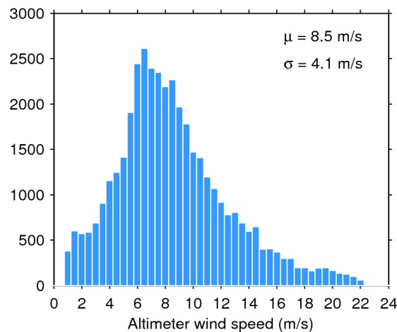
Figure 35. Histogram of science-valid wind over oceans and lakes for 28/05/2017. The mean ( \mu ) and standard deviation ( \sigma ) are also shown. Note that values larger than 24 m/s are excluded from the histogram for the sake of readability but not from the computation of \mu and \sigma .
