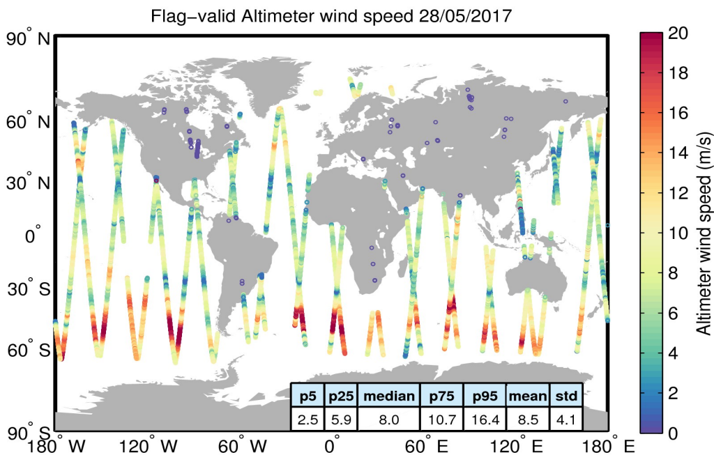
Figure 31. Geographical distribution of flag-valid wind data over oceans and lakes for 28/05/2017. The statistical values shown in the table refer to the wind in m/s and are calculated over all measurements shown in the figure.
