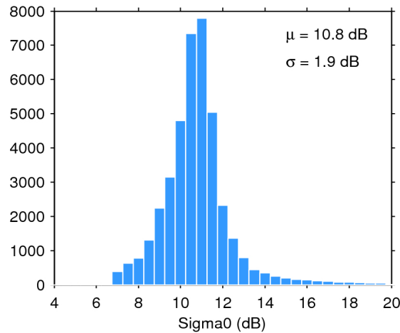
Figure 25. Histogram of flag-valid sigma0 over oceans and lakes for 28/05/2017. The mean ( \mu ) and standard deviation ( \sigma ) are also shown. Note that values outside [4 20] dB are excluded from the histogram for the sake of readability but not from the computation of \mu and \sigma .
