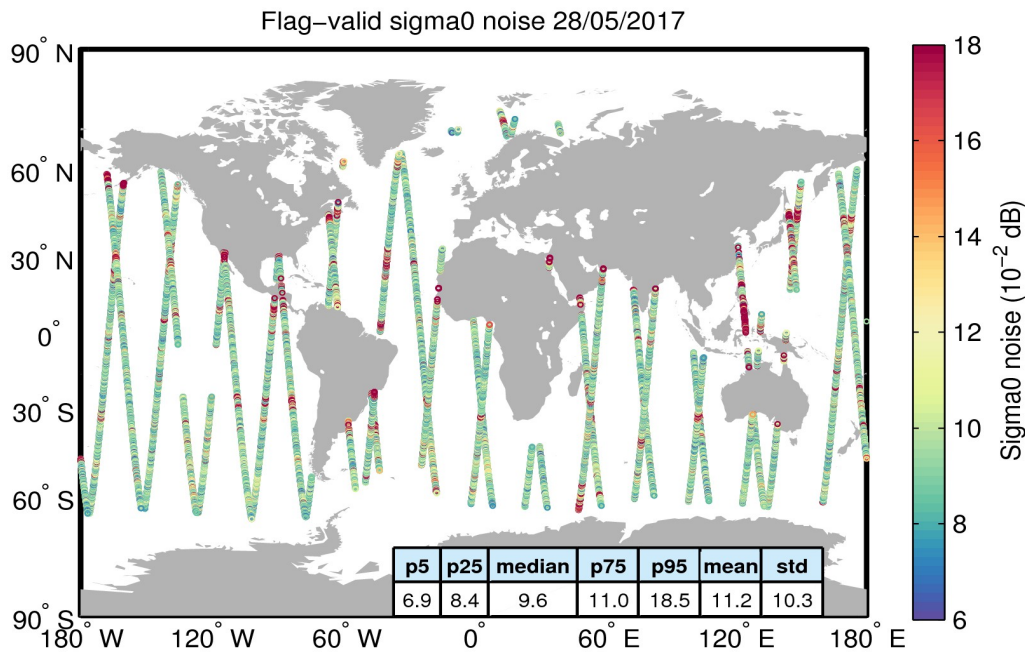
Figure 26. Geographical distribution of flag-valid 20-Hz sigma0 measurement noise over oceans and lakes for 28/05/2017. The statistical values shown in the table refer to the sigma0 noise and are calculated over all measurements shown in the figure.
