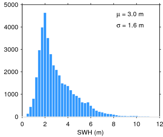
Figure 17. Histogram of flag-valid SWH over oceans and lakes for 28/05/2017. The mean ( \mu ) and standard deviation ( \sigma ) are also shown. Note that values larger than 12 m are excluded from the histogram for the sake of readability but not from the computation of \mu and \sigma .
