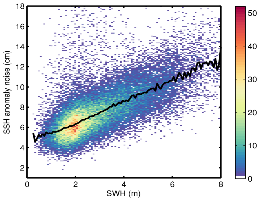
Figure 9. 2D histogram showing flag-valid SSH anomaly noise as a function of SWH for 28/05/2017. The black line denotes the median SSH anomaly noise as a function of SWH.
