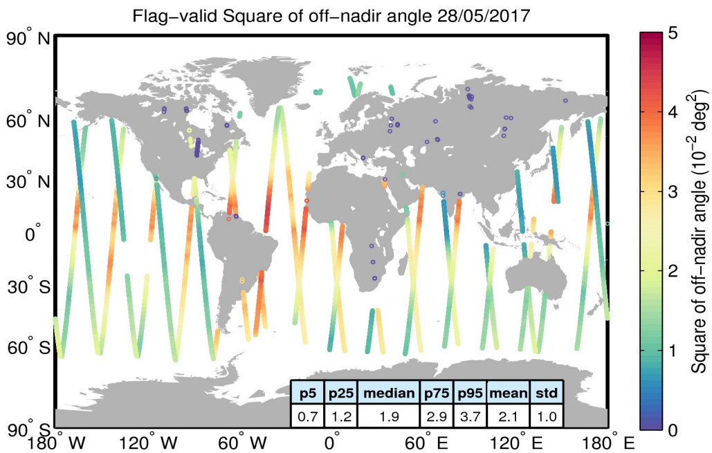
Figure 37. Geographical distribution of flag-valid mispointing data over oceans and lakes for 28/05/2017. The statistical values shown in the table refer to the mispointing in 10^{-2} deg 2 and are calculated over all measurements shown in the figure.
