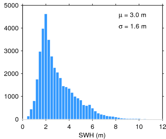
Figure 20. Histogram of science-valid SWH over oceans and lakes for 28/05/2017. The mean ( \mu ) and standard deviation ( \sigma ) are also shown. Note that values larger than 12 m are excluded from the histogram for the sake of readability but not from the computation of \mu and \sigma .
