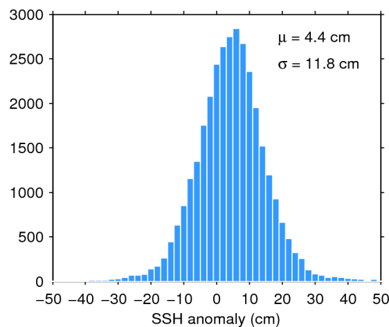
Figure 11. Histogram of science-valid SSH anomaly over oceans and lakes for 28/05/2017. The mean ( \mu ) and standard deviation ( \sigma ) are also shown. Note that values outside [-50 50] cm are excluded from the histogram for the sake of readability but not from the computation of \mu and \sigma .
