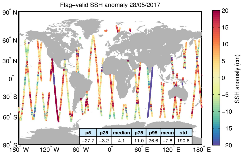
Figure 5. Geographical distribution of flag-valid 1-Hz SSH anomaly data over oceans and lakes for 28/05/2017. The statistical values shown in the table refer to the SSH anomaly in cm and are calculated over all measurements shown in the figure.
