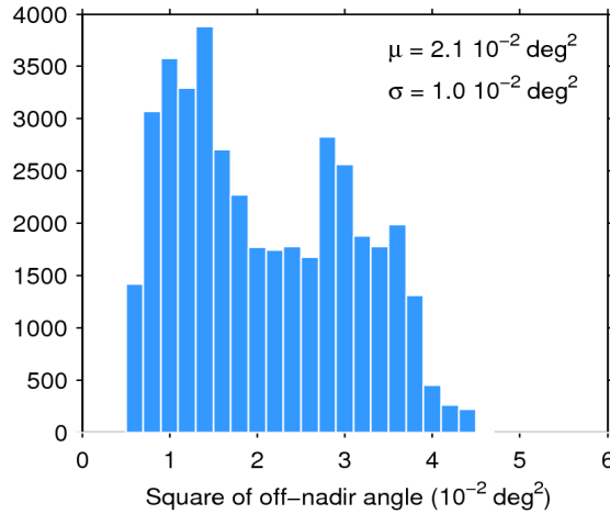
Figure 39. Histogram of flag-valid mispointing over oceans and lakes for 28/05/2017. The mean ( \mu ) and standard deviation ( \sigma ) are also shown. Note that values larger than 6 \cdot 10^{-2} \text{ deg}^2 are excluded from the histogram for the sake of readability but not from the computation of \mu and \sigma .
