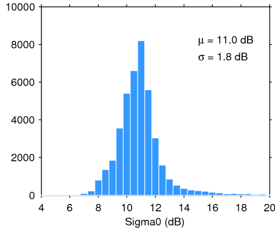
Figure 25. Histogram of flag-valid sigma0 over oceans and lakes for 27/05/2017. The mean ( \mu ) and standard deviation ( \sigma ) are also shown. Note that values outside [4 20] dB are excluded from the histogram for the sake of readability but not from the computation of \mu and \sigma .
