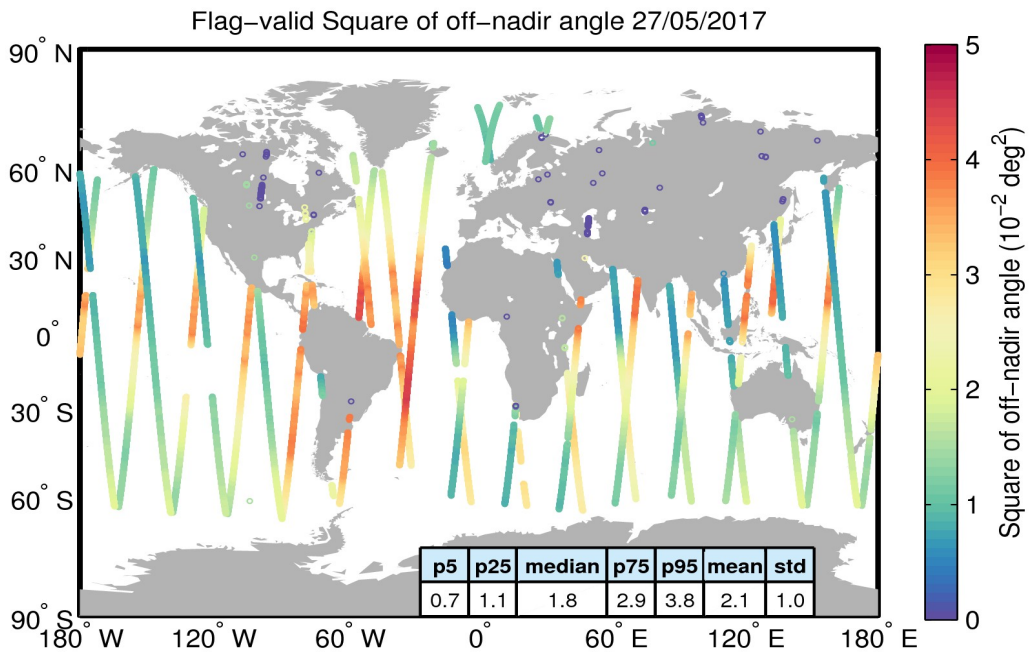
Figure 37. Geographical distribution of flag-valid mispointing data over oceans and lakes for 27/05/2017. The statistical values shown in the table refer to the mispointing in 10^{-2} deg 2 and are calculated over all measurements shown in the figure.
