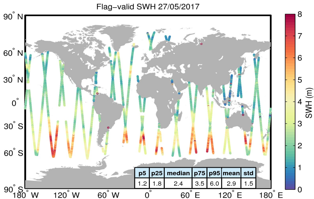
Figure 15. Geographical distribution of flag-valid SWH data over oceans and lakes for 27/05/2017. The statistical values shown in the table refer to the SWH in m and are calculated over all measurements shown in the figure.
