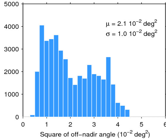
Figure 39. Histogram of flag-valid mispointing over oceans and lakes for 27/05/2017. The mean ( \mu ) and standard deviation ( \sigma ) are also shown. Note that values larger than 6 \cdot 10^{-2} \text{ deg}^2 are excluded from the histogram for the sake of readability but not from the computation of \mu and \sigma .
