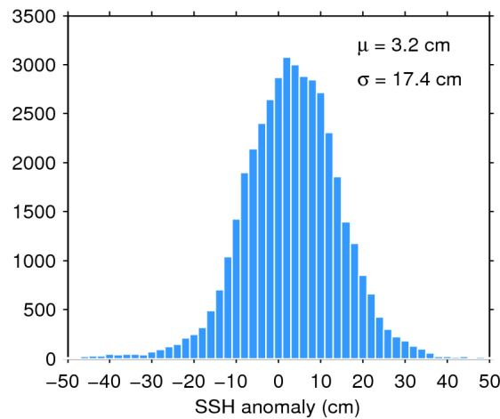
Figure 7. Histogram of flag-valid SSH anomaly over oceans and lakes for 27/05/2017. The mean ( \mu ) and standard deviation ( \sigma ) are also shown. Note that values outside [-50 50] cm are excluded from the histogram for the sake of readability but not from the computation of \mu and \sigma .
