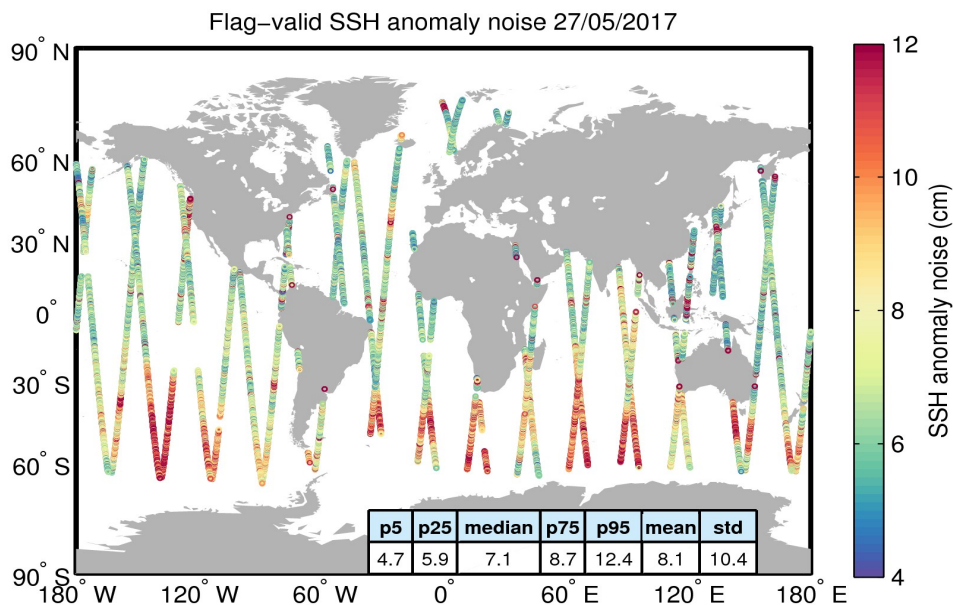
Figure 8. Geographical distribution of flag-valid 20-Hz SSH anomaly measurement noise over oceans and lakes for 27/05/2017. The statistical values shown in the table refer to the SSH anomaly noise and are calculated over all measurements shown in the figure.
