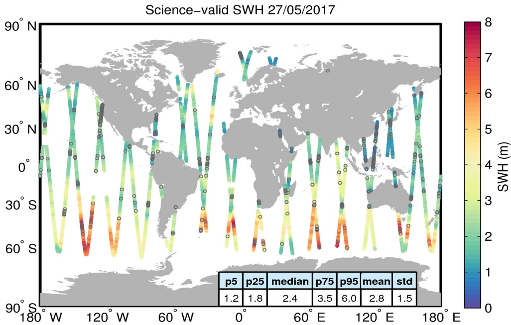
Figure 19. Geographical distribution of science-valid SWH data over oceans and lakes for 27/05/2017. The statistical values shown in the table refer to the SWH in m and are calculated over all measurements shown in the figure. Gray circles denote records that have been rejected based on the editing criteria described in Table 3.
