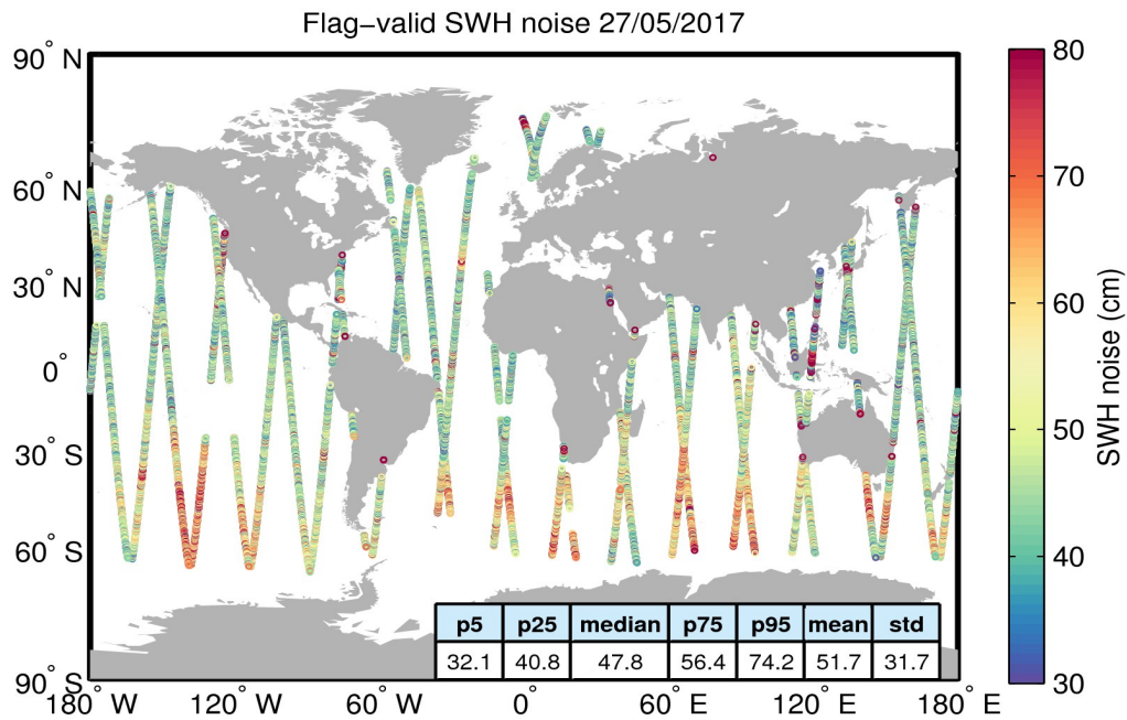
Figure 18. Geographical distribution of flag-valid 20-Hz SWH measurement noise over oceans and lakes for 27/05/2017. The statistical values shown in the table refer to the SWH noise and are calculated over all measurements shown in the figure.
