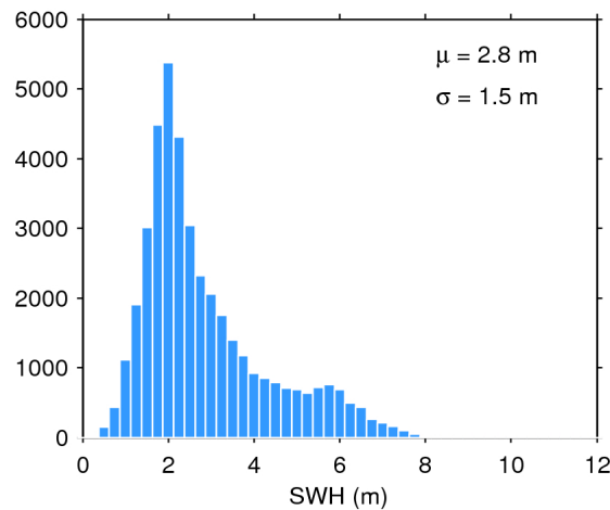
Figure 20. Histogram of science-valid SWH over oceans and lakes for 27/05/2017. The mean ( \mu ) and standard deviation ( \sigma ) are also shown. Note that values larger than 12 m are excluded from the histogram for the sake of readability but not from the computation of \mu and \sigma .
