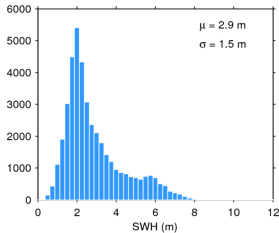
Figure 17. Histogram of flag-valid SWH over oceans and lakes for 27/05/2017. The mean ( \mu ) and standard deviation ( \sigma ) are also shown. Note that values larger than 12 m are excluded from the histogram for the sake of readability but not from the computation of \mu and \sigma .
