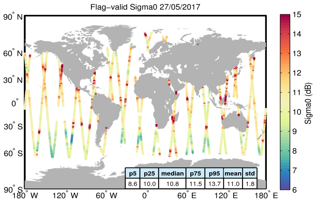
Figure 23. Geographical distribution of flag-valid sigma0 data over oceans and lakes for 27/05/2017. The statistical values shown in the table refer to the sigma0 in dB and are calculated over all measurements shown in the figure.
