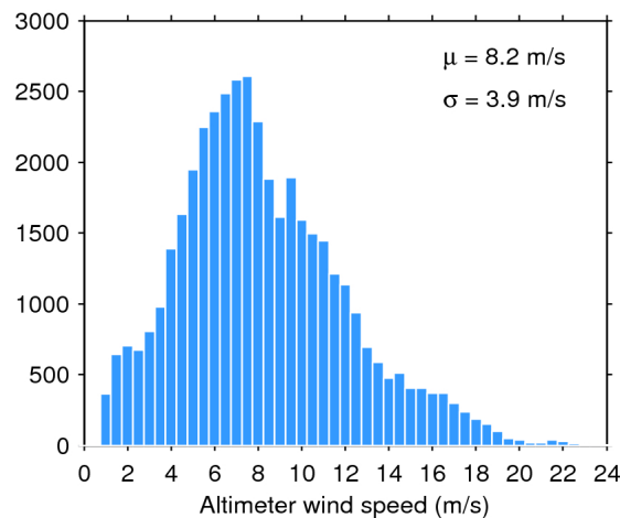
Figure 35. Histogram of science-valid wind over oceans and lakes for 27/05/2017. The mean ( \mu ) and standard deviation ( \sigma ) are also shown. Note that values larger than 24 m/s are excluded from the histogram for the sake of readability but not from the computation of \mu and \sigma .
