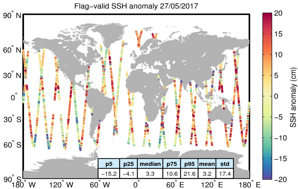
Figure 5. Geographical distribution of flag-valid 1-Hz SSH anomaly data over oceans and lakes for 27/05/2017. The statistical values shown in the table refer to the SSH anomaly in cm and are calculated over all measurements shown in the figure.
