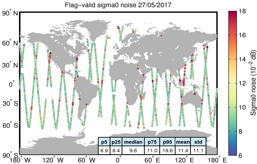
Figure 26. Geographical distribution of flag-valid 20-Hz sigma0 measurement noise over oceans and lakes for 27/05/2017. The statistical values shown in the table refer to the sigma0 noise and are calculated over all measurements shown in the figure.
