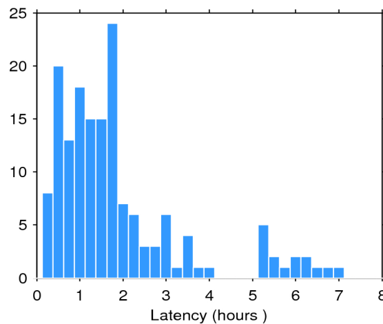
Figure 2. Histogram of the data latency for 27/05/2017. The y-axis denotes the number of files that are made available with a delay of x-hours with respect to the mean time of the records stored in the file.
