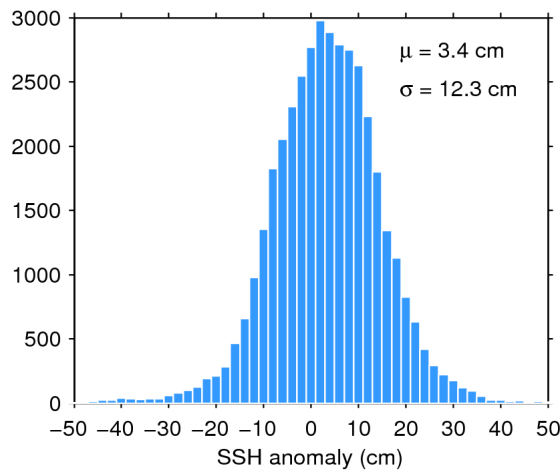
Figure 11. Histogram of science-valid SSH anomaly over oceans and lakes for 27/05/2017. The mean ( \mu ) and standard deviation ( \sigma ) are also shown. Note that values outside [-50 50] cm are excluded from the histogram for the sake of readability but not from the computation of \mu and \sigma .
