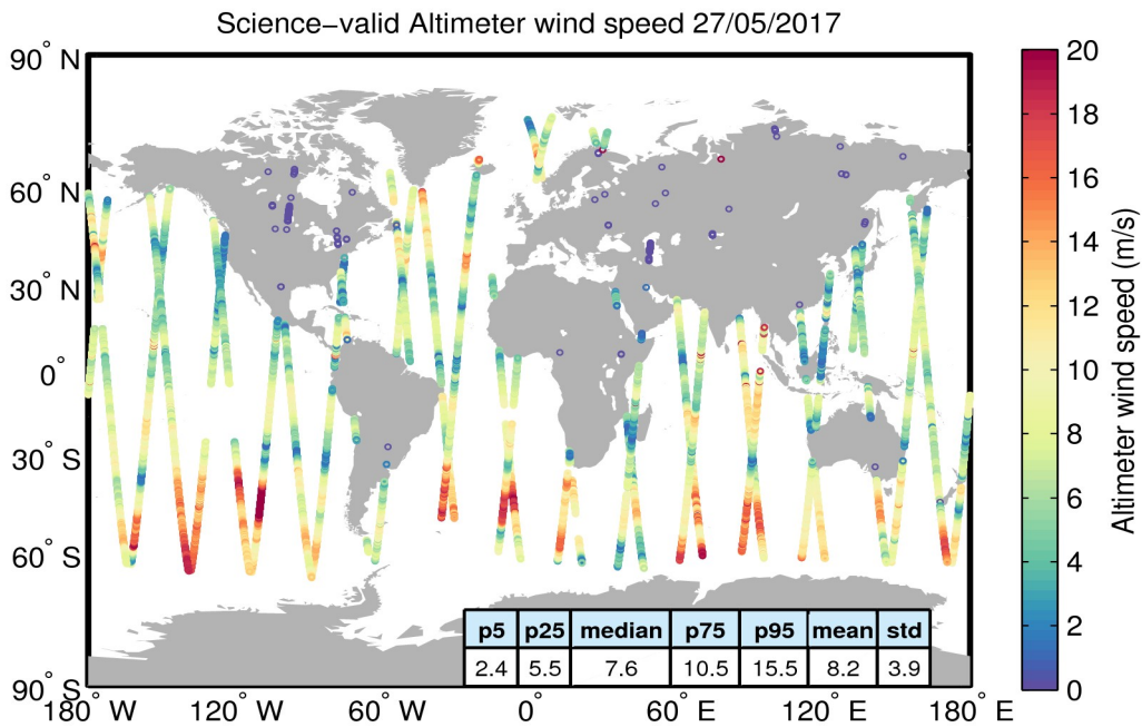
Figure 34. Geographical distribution of science-valid wind data over oceans and lakes for 27/05/2017. The statistical values shown in the table refer to the wind in m/s and are calculated over all measurements shown in the figure. Gray circles denote records that have been rejected based on the editing criteria described in Table 5.
