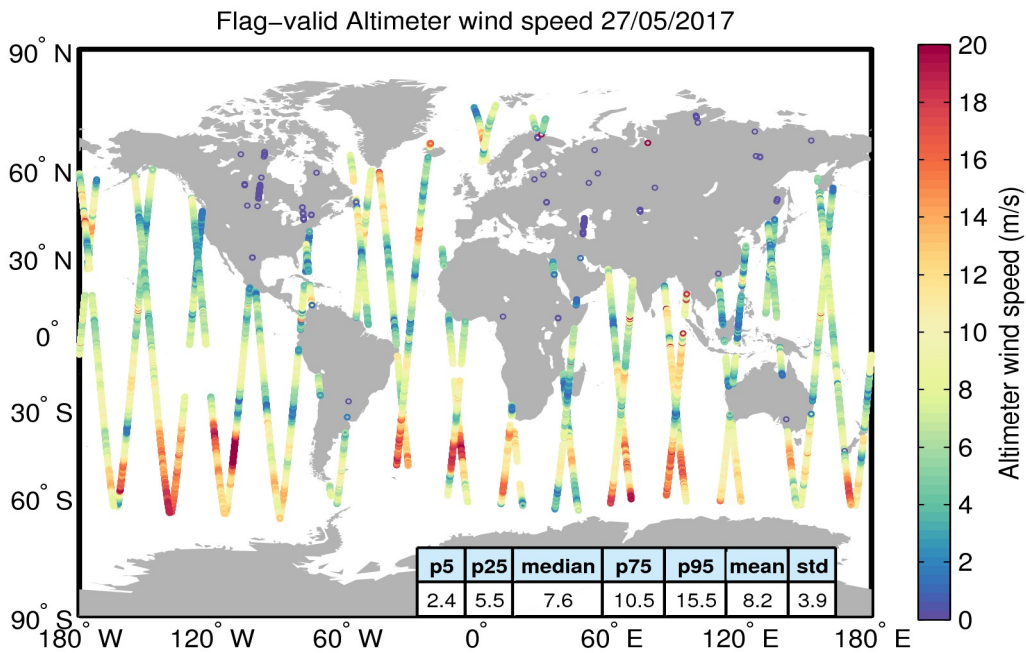
Figure 31. Geographical distribution of flag-valid wind data over oceans and lakes for 27/05/2017. The statistical values shown in the table refer to the wind in m/s and are calculated over all measurements shown in the figure.
