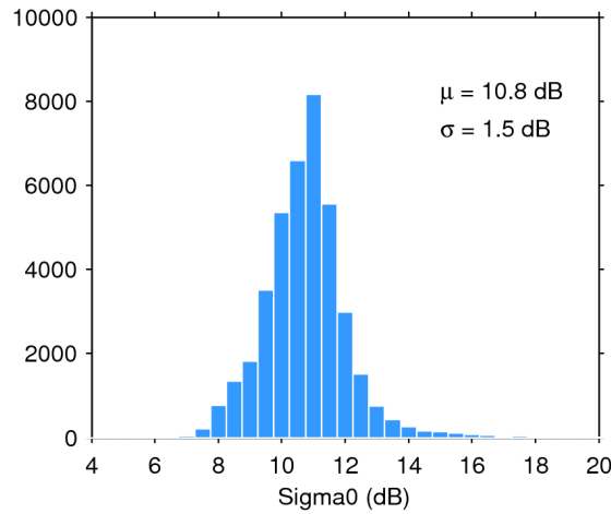
Figure 28. Histogram of science-valid sigma0 over oceans and lakes for 27/05/2017. The mean ( \mu ) and standard deviation ( \sigma ) are also shown. Note that values outside [4 20] dB are excluded from the histogram for the sake of readability but not from the computation of \mu and \sigma .
