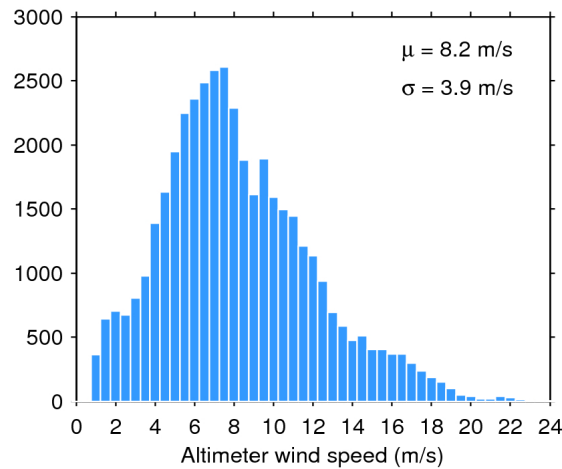
Figure 33. Histogram of flag-valid wind over oceans and lakes for 27/05/2017. The mean ( \mu ) and standard deviation ( \sigma ) are also shown. Note that values larger than 24 m/s are excluded from the histogram for the sake of readability but not from the computation of \mu and \sigma .
