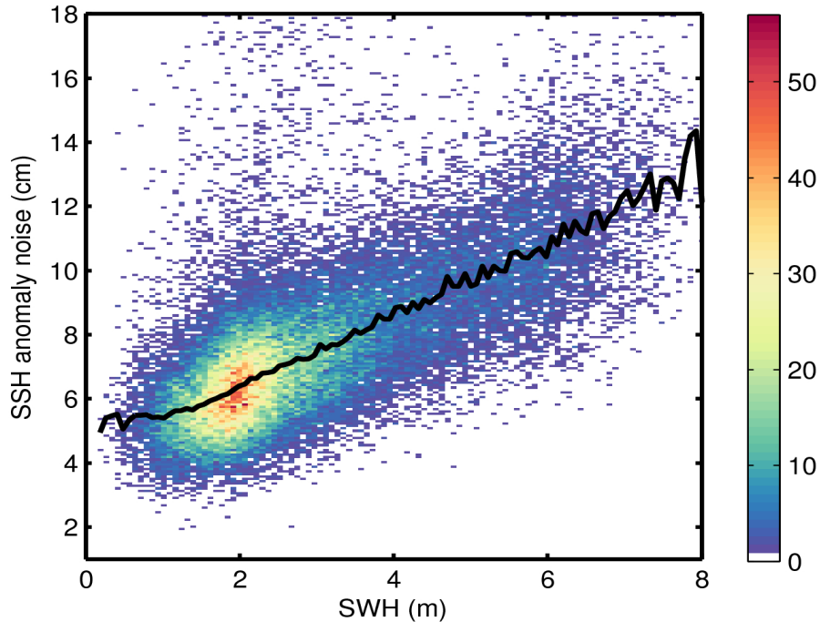
Figure 9. 2D histogram showing flag-valid SSH anomaly noise as a function of SWH for 27/05/2017. The black line denotes the median SSH anomaly noise as a function of SWH.
