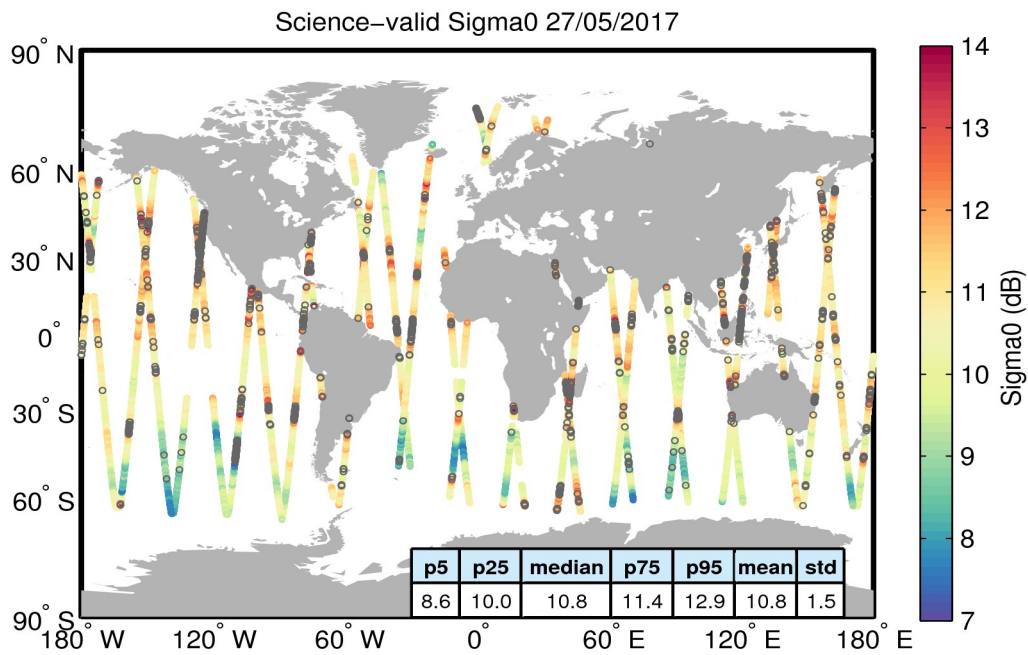
Figure 27. Geographical distribution of science-valid sigma0 data over oceans and lakes for 27/05/2017. The statistical values shown in the table refer to the sigma0 in dB and are calculated over all measurements shown in the figure. Gray circles denote records that have been rejected based on the editing criteria described in Table 4.
