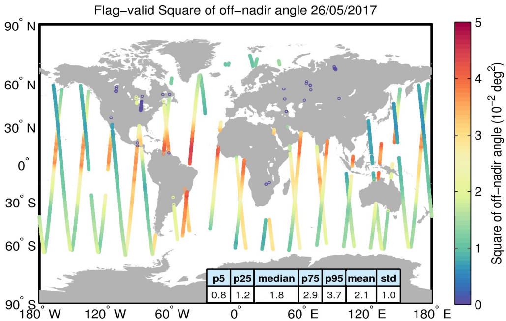
Figure 37. Geographical distribution of flag-valid mispointing data over oceans and lakes for 26/05/2017. The statistical values shown in the table refer to the mispointing in 10^{-2} deg 2 and are calculated over all measurements shown in the figure.
