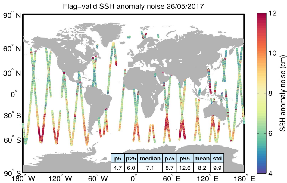
Figure 8. Geographical distribution of flag-valid 20-Hz SSH anomaly measurement noise over oceans and lakes for 26/05/2017. The statistical values shown in the table refer to the SSH anomaly noise and are calculated over all measurements shown in the figure.
