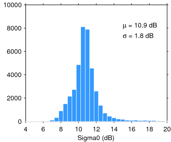
Figure 25. Histogram of flag-valid sigma0 over oceans and lakes for 26/05/2017. The mean ( \mu ) and standard deviation ( \sigma ) are also shown. Note that values outside [4 20] dB are excluded from the histogram for the sake of readability but not from the computation of \mu and \sigma .
