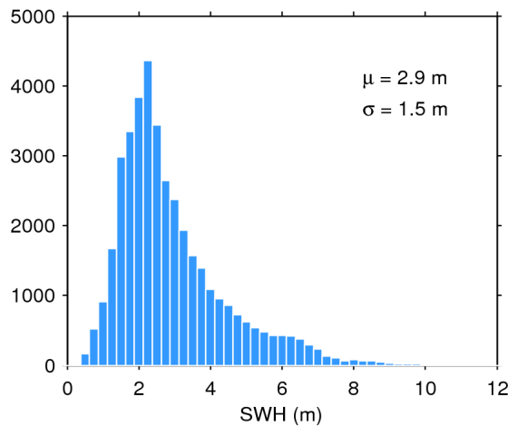
Figure 20. Histogram of science-valid SWH over oceans and lakes for 26/05/2017. The mean ( \mu ) and standard deviation ( \sigma ) are also shown. Note that values larger than 12 m are excluded from the histogram for the sake of readability but not from the computation of \mu and \sigma .
