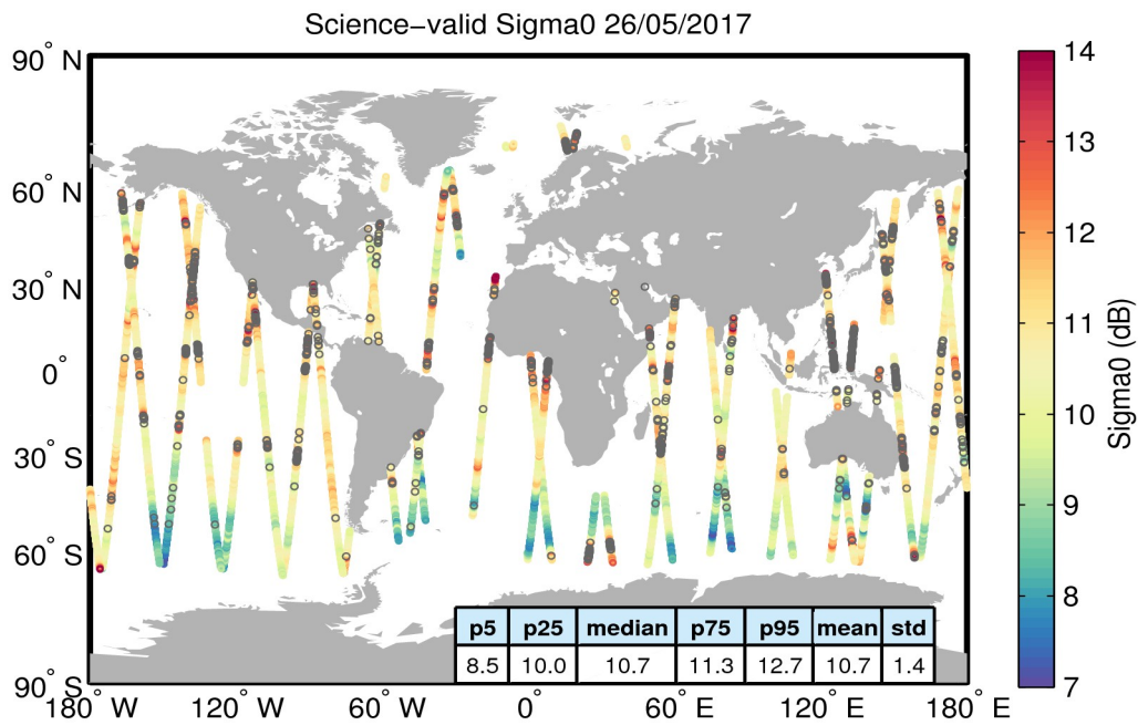
Figure 27. Geographical distribution of science-valid sigma0 data over oceans and lakes for 26/05/2017. The statistical values shown in the table refer to the sigma0 in dB and are calculated over all measurements shown in the figure. Gray circles denote records that have been rejected based on the editing criteria described in Table 4.
