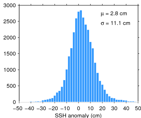
Figure 11. Histogram of science-valid SSH anomaly over oceans and lakes for 26/05/2017. The mean ( \mu ) and standard deviation ( \sigma ) are also shown. Note that values outside [-50 50] cm are excluded from the histogram for the sake of readability but not from the computation of \mu and \sigma .
