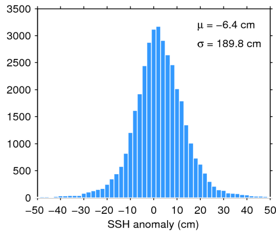
Figure 7. Histogram of flag-valid SSH anomaly over oceans and lakes for 26/05/2017. The mean ( \mu ) and standard deviation ( \sigma ) are also shown. Note that values outside [-50 50] cm are excluded from the histogram for the sake of readability but not from the computation of \mu and \sigma .
