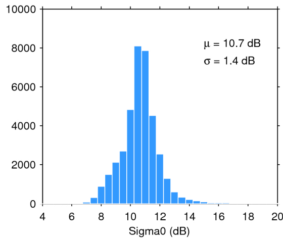
Figure 28. Histogram of science-valid sigma0 over oceans and lakes for 26/05/2017. The mean ( \mu ) and standard deviation ( \sigma ) are also shown. Note that values outside [4 20] dB are excluded from the histogram for the sake of readability but not from the computation of \mu and \sigma .
