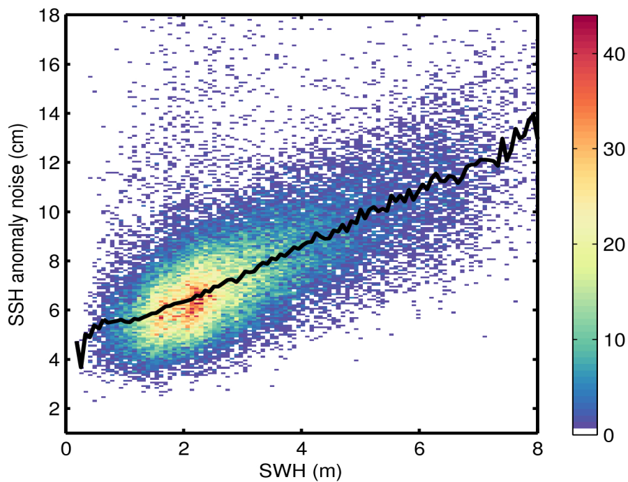
Figure 9. 2D histogram showing flag-valid SSH anomaly noise as a function of SWH for 26/05/2017. The black line denotes the median SSH anomaly noise as a function of SWH.
