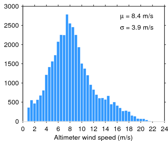
Figure 35. Histogram of science-valid wind over oceans and lakes for 26/05/2017. The mean ( \mu ) and standard deviation ( \sigma ) are also shown. Note that values larger than 24 m/s are excluded from the histogram for the sake of readability but not from the computation of \mu and \sigma .
