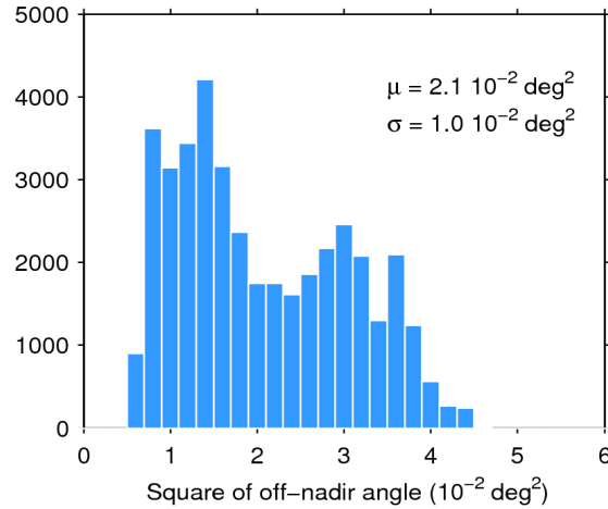
Figure 39. Histogram of flag-valid mispointing over oceans and lakes for 26/05/2017. The mean ( \mu ) and standard deviation ( \sigma ) are also shown. Note that values larger than 6 \cdot 10^{-2} \text{ deg}^2 are excluded from the histogram for the sake of readability but not from the computation of \mu and \sigma .
