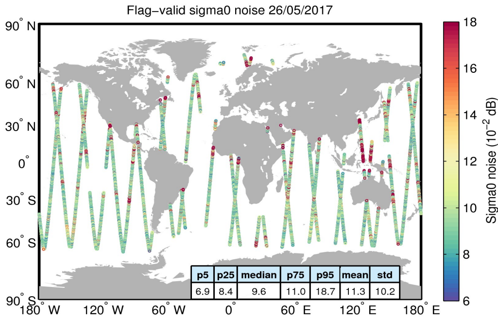
Figure 26. Geographical distribution of flag-valid 20-Hz sigma0 measurement noise over oceans and lakes for 26/05/2017. The statistical values shown in the table refer to the sigma0 noise and are calculated over all measurements shown in the figure.
