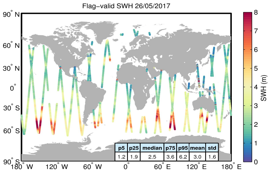
Figure 15. Geographical distribution of flag-valid SWH data over oceans and lakes for 26/05/2017. The statistical values shown in the table refer to the SWH in m and are calculated over all measurements shown in the figure.
