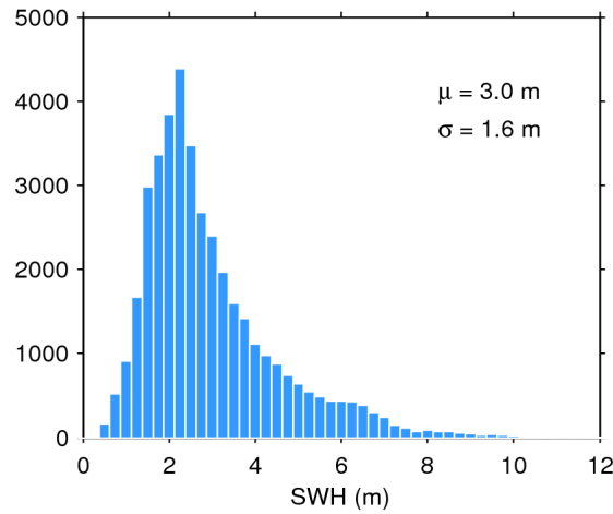
Figure 17. Histogram of flag-valid SWH over oceans and lakes for 26/05/2017. The mean ( \mu ) and standard deviation ( \sigma ) are also shown. Note that values larger than 12 m are excluded from the histogram for the sake of readability but not from the computation of \mu and \sigma .
