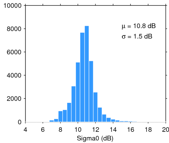
Figure 28. Histogram of science-valid sigma0 over oceans and lakes for 25/05/2017. The mean ( \mu ) and standard deviation ( \sigma ) are also shown. Note that values outside [4 20] dB are excluded from the histogram for the sake of readability but not from the computation of \mu and \sigma .
