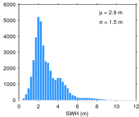
Figure 17. Histogram of flag-valid SWH over oceans and lakes for 25/05/2017. The mean ( \mu ) and standard deviation ( \sigma ) are also shown. Note that values larger than 12 m are excluded from the histogram for the sake of readability but not from the computation of \mu and \sigma .
