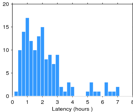
Figure 2. Histogram of the data latency for 25/05/2017. The y-axis denotes the number of files that are made available with a delay of x-hours with respect to the mean time of the records stored in the file.
