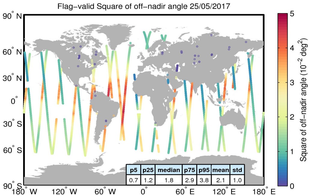
Figure 37. Geographical distribution of flag-valid mispointing data over oceans and lakes for 25/05/2017. The statistical values shown in the table refer to the mispointing in 10^{-2} deg 2 and are calculated over all measurements shown in the figure.
