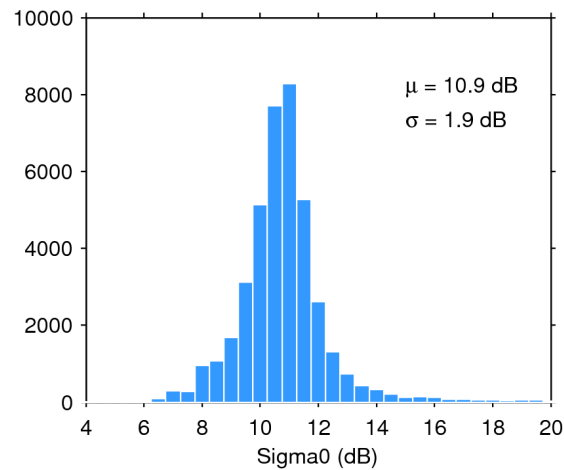
Figure 25. Histogram of flag-valid sigma0 over oceans and lakes for 25/05/2017. The mean ( \mu ) and standard deviation ( \sigma ) are also shown. Note that values outside [4 20] dB are excluded from the histogram for the sake of readability but not from the computation of \mu and \sigma .
