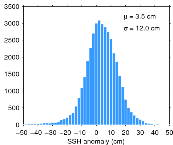
Figure 11. Histogram of science-valid SSH anomaly over oceans and lakes for 25/05/2017. The mean ( \mu ) and standard deviation ( \sigma ) are also shown. Note that values outside [-50 50] cm are excluded from the histogram for the sake of readability but not from the computation of \mu and \sigma .
