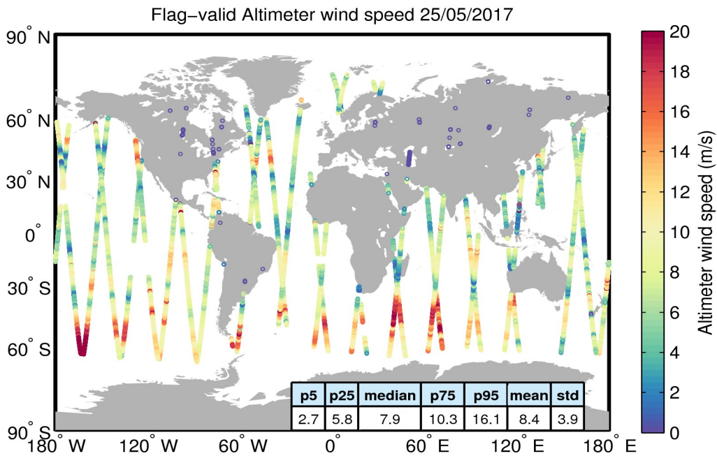
Figure 31. Geographical distribution of flag-valid wind data over oceans and lakes for 25/05/2017. The statistical values shown in the table refer to the wind in m/s and are calculated over all measurements shown in the figure.
