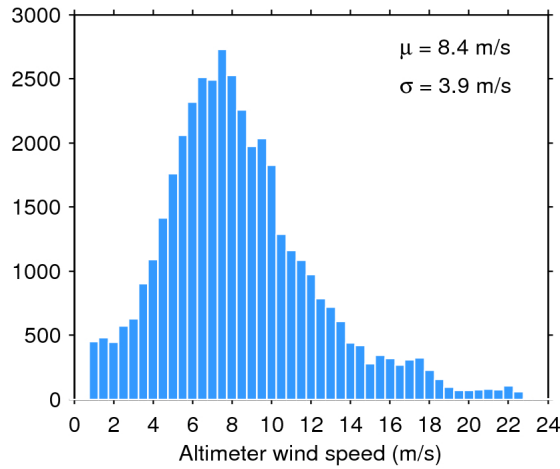
Figure 33. Histogram of flag-valid wind over oceans and lakes for 25/05/2017. The mean ( \mu ) and standard deviation ( \sigma ) are also shown. Note that values larger than 24 m/s are excluded from the histogram for the sake of readability but not from the computation of \mu and \sigma .
