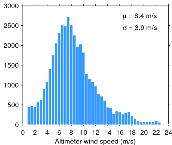
Figure 35. Histogram of science-valid wind over oceans and lakes for 25/05/2017. The mean ( \mu ) and standard deviation ( \sigma ) are also shown. Note that values larger than 24 m/s are excluded from the histogram for the sake of readability but not from the computation of \mu and \sigma .
