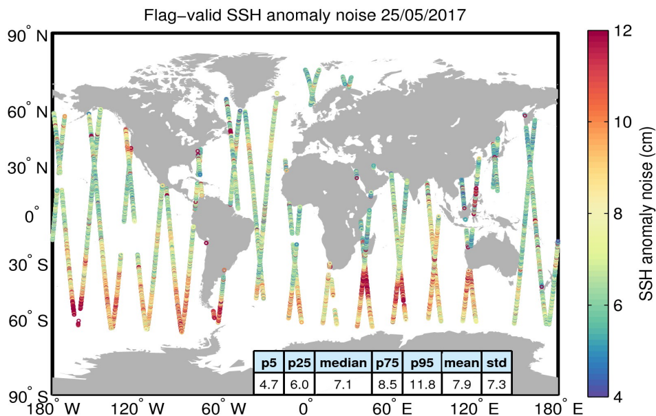
Figure 8. Geographical distribution of flag-valid 20-Hz SSH anomaly measurement noise over oceans and lakes for 25/05/2017. The statistical values shown in the table refer to the SSH anomaly noise and are calculated over all measurements shown in the figure.
