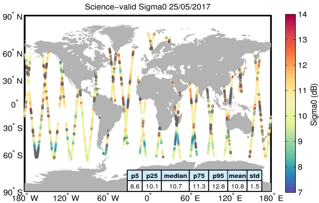
Figure 27. Geographical distribution of science-valid sigma0 data over oceans and lakes for 25/05/2017. The statistical values shown in the table refer to the sigma0 in dB and are calculated over all measurements shown in the figure. Gray circles denote records that have been rejected based on the editing criteria described in Table 4.
