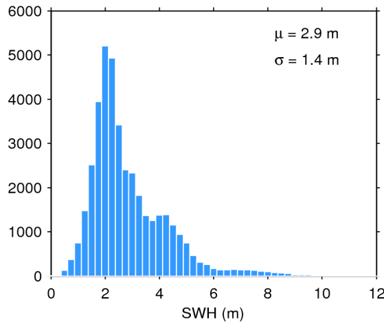
Figure 20. Histogram of science-valid SWH over oceans and lakes for 25/05/2017. The mean ( \mu ) and standard deviation ( \sigma ) are also shown. Note that values larger than 12 m are excluded from the histogram for the sake of readability but not from the computation of \mu and \sigma .
