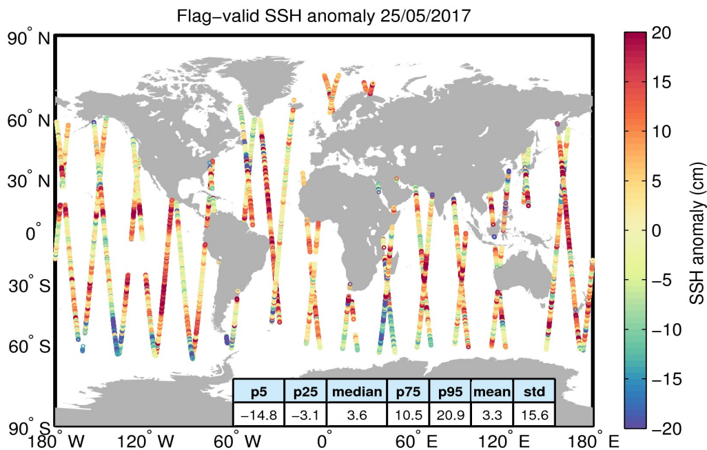
Figure 5. Geographical distribution of flag-valid 1-Hz SSH anomaly data over oceans and lakes for 25/05/2017. The statistical values shown in the table refer to the SSH anomaly in cm and are calculated over all measurements shown in the figure.
