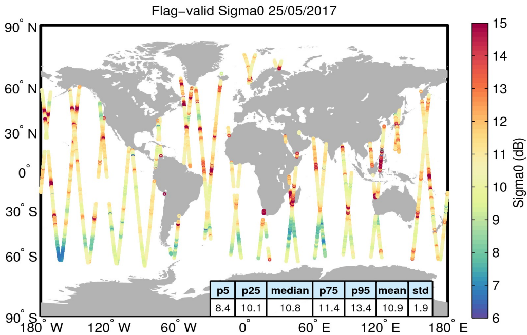
Figure 23. Geographical distribution of flag-valid sigma0 data over oceans and lakes for 25/05/2017. The statistical values shown in the table refer to the sigma0 in dB and are calculated over all measurements shown in the figure.
