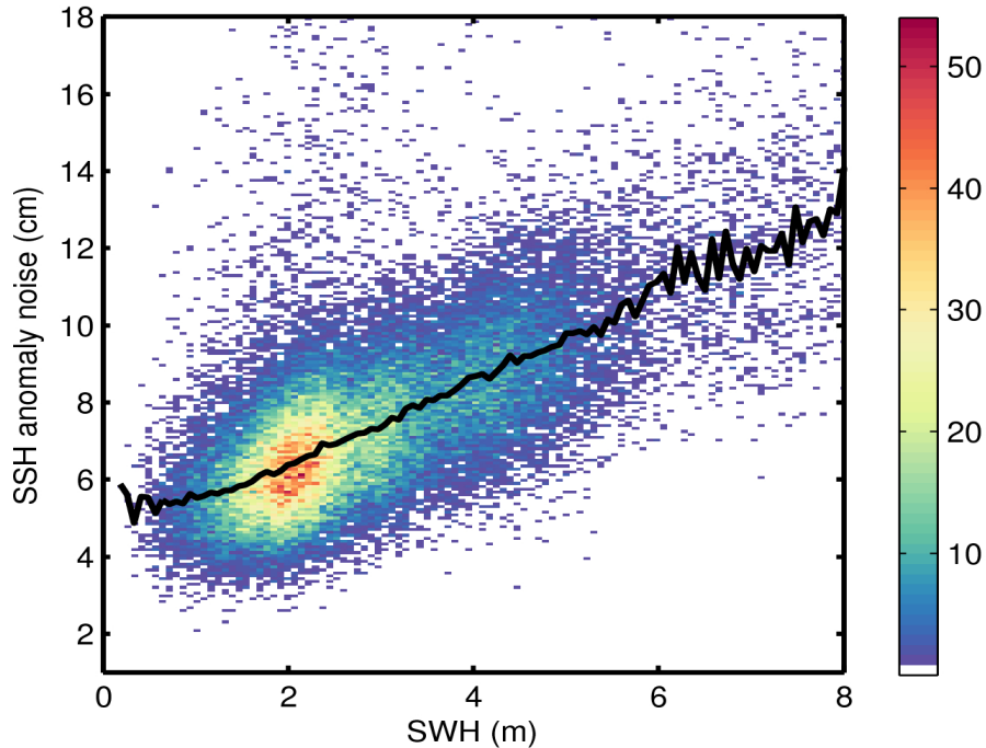
Figure 9. 2D histogram showing flag-valid SSH anomaly noise as a function of SWH for 25/05/2017. The black line denotes the median SSH anomaly noise as a function of SWH.
