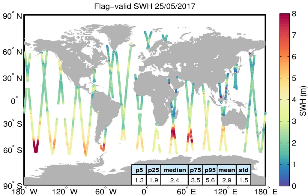
Figure 15. Geographical distribution of flag-valid SWH data over oceans and lakes for 25/05/2017. The statistical values shown in the table refer to the SWH in m and are calculated over all measurements shown in the figure.
