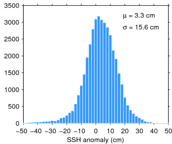
Figure 7. Histogram of flag-valid SSH anomaly over oceans and lakes for 25/05/2017. The mean ( \mu ) and standard deviation ( \sigma ) are also shown. Note that values outside [-50 50] cm are excluded from the histogram for the sake of readability but not from the computation of \mu and \sigma .
