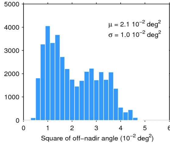
Figure 39. Histogram of flag-valid mispointing over oceans and lakes for 25/05/2017. The mean ( \mu ) and standard deviation ( \sigma ) are also shown. Note that values larger than 6 \cdot 10^{-2} \text{ deg}^2 are excluded from the histogram for the sake of readability but not from the computation of \mu and \sigma .
