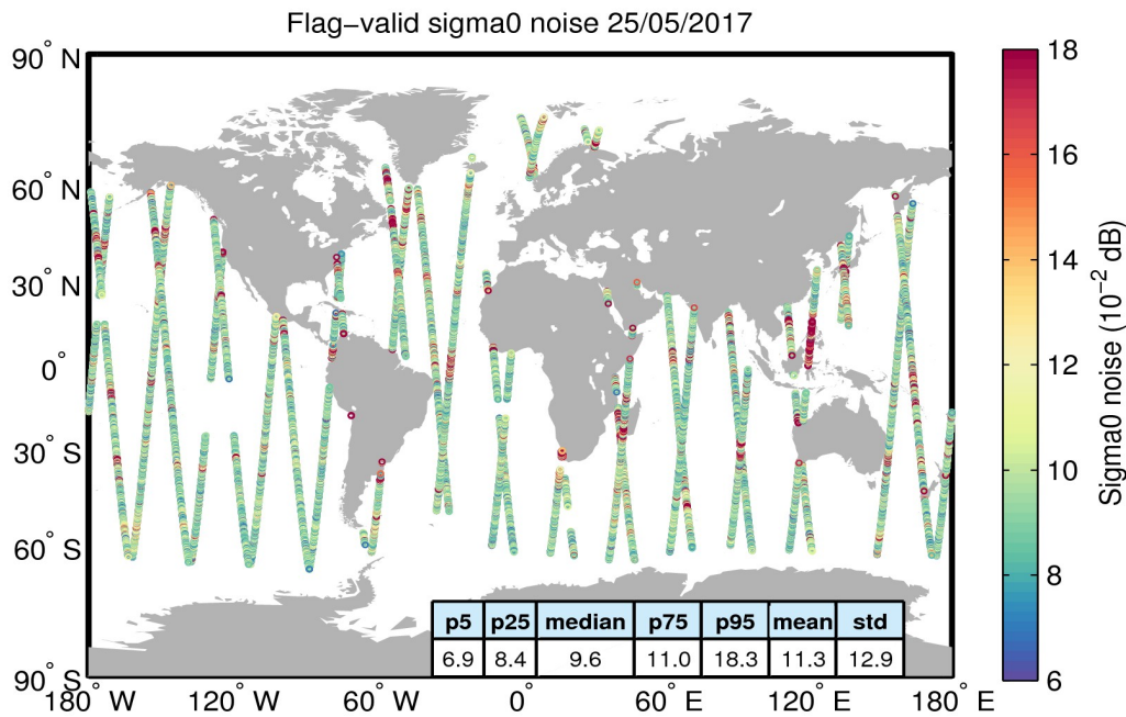
Figure 26. Geographical distribution of flag-valid 20-Hz sigma0 measurement noise over oceans and lakes for 25/05/2017. The statistical values shown in the table refer to the sigma0 noise and are calculated over all measurements shown in the figure.
