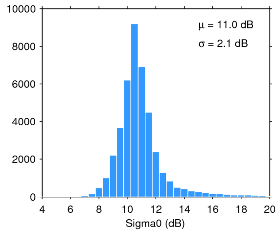
Figure 25. Histogram of flag-valid sigma0 over oceans and lakes for 24/05/2017. The mean ( \mu ) and standard deviation ( \sigma ) are also shown. Note that values outside [4 20] dB are excluded from the histogram for the sake of readability but not from the computation of \mu and \sigma .
