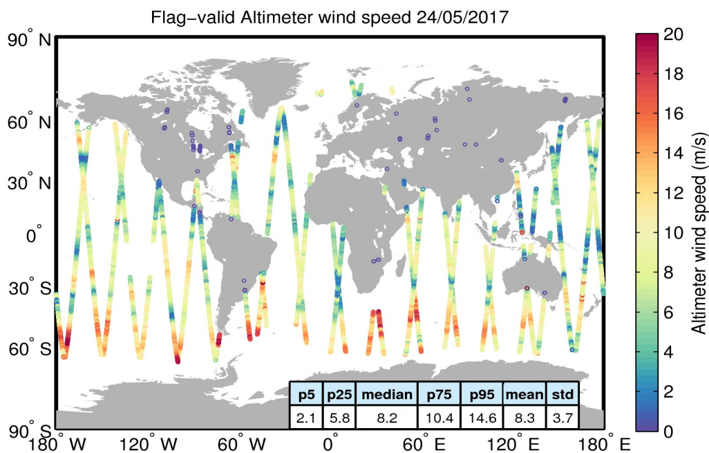
Figure 31. Geographical distribution of flag-valid wind data over oceans and lakes for 24/05/2017. The statistical values shown in the table refer to the wind in m/s and are calculated over all measurements shown in the figure.
