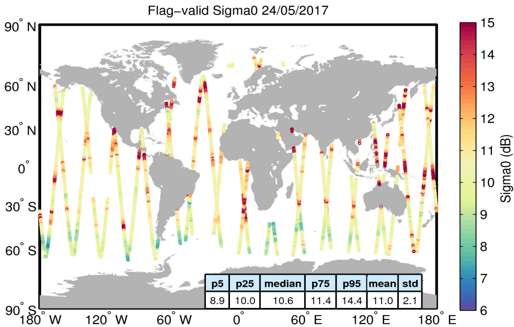
Figure 23. Geographical distribution of flag-valid sigma0 data over oceans and lakes for 24/05/2017. The statistical values shown in the table refer to the sigma0 in dB and are calculated over all measurements shown in the figure.
