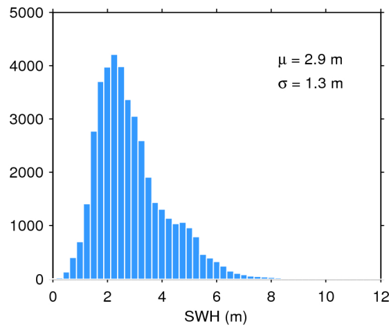
Figure 17. Histogram of flag-valid SWH over oceans and lakes for 24/05/2017. The mean ( \mu ) and standard deviation ( \sigma ) are also shown. Note that values larger than 12 m are excluded from the histogram for the sake of readability but not from the computation of \mu and \sigma .
