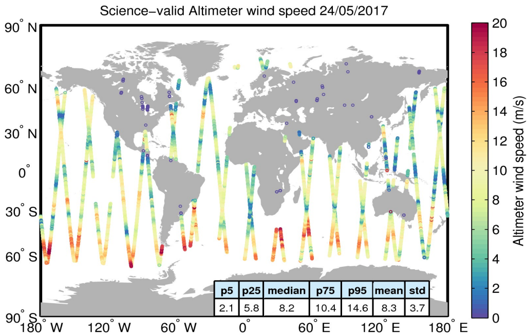
Figure 34. Geographical distribution of science-valid wind data over oceans and lakes for 24/05/2017. The statistical values shown in the table refer to the wind in m/s and are calculated over all measurements shown in the figure. Gray circles denote records that have been rejected based on the editing criteria described in Table 5.
