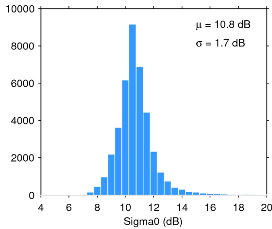
Figure 28. Histogram of science-valid sigma0 over oceans and lakes for 24/05/2017. The mean ( \mu ) and standard deviation ( \sigma ) are also shown. Note that values outside [4 20] dB are excluded from the histogram for the sake of readability but not from the computation of \mu and \sigma .
