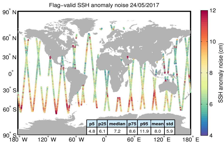
Figure 8. Geographical distribution of flag-valid 20-Hz SSH anomaly measurement noise over oceans and lakes for 24/05/2017. The statistical values shown in the table refer to the SSH anomaly noise and are calculated over all measurements shown in the figure.
