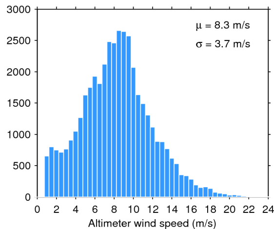
Figure 35. Histogram of science-valid wind over oceans and lakes for 24/05/2017. The mean ( \mu ) and standard deviation ( \sigma ) are also shown. Note that values larger than 24 m/s are excluded from the histogram for the sake of readability but not from the computation of \mu and \sigma .
