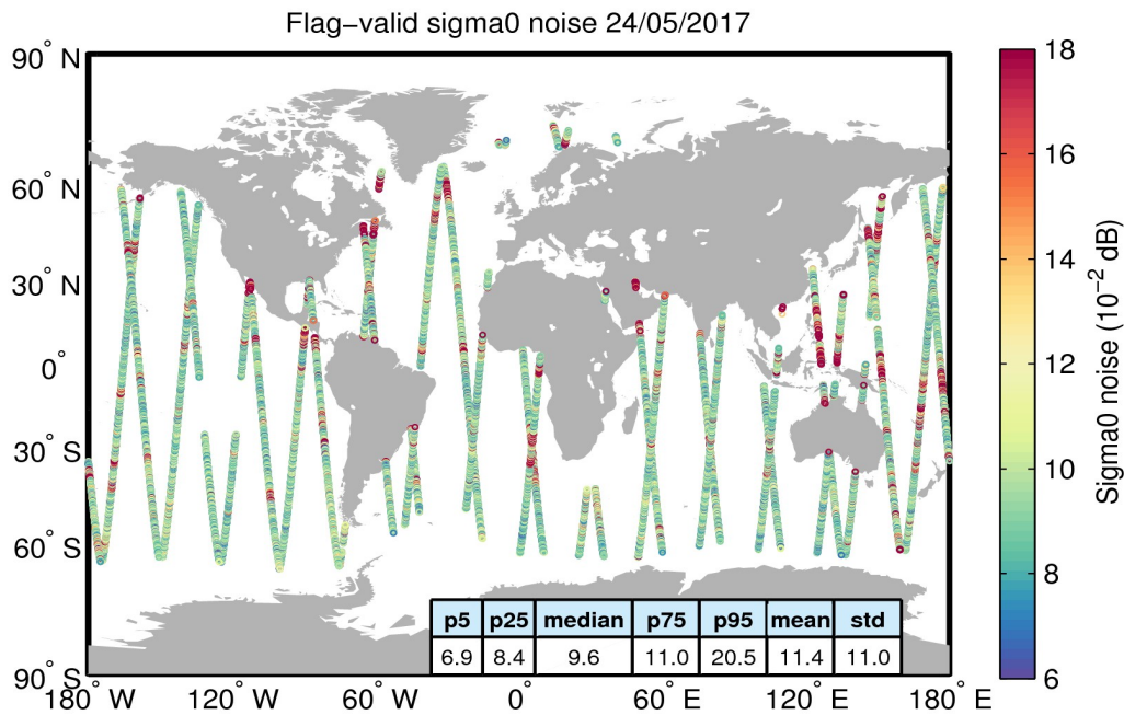
Figure 26. Geographical distribution of flag-valid 20-Hz sigma0 measurement noise over oceans and lakes for 24/05/2017. The statistical values shown in the table refer to the sigma0 noise and are calculated over all measurements shown in the figure.
