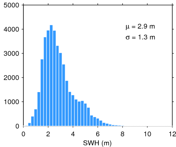
Figure 20. Histogram of science-valid SWH over oceans and lakes for 24/05/2017. The mean ( \mu ) and standard deviation ( \sigma ) are also shown. Note that values larger than 12 m are excluded from the histogram for the sake of readability but not from the computation of \mu and \sigma .
