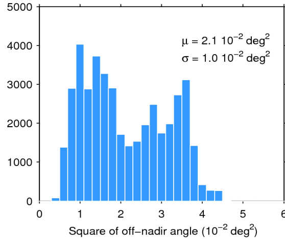
Figure 39. Histogram of flag-valid mispointing over oceans and lakes for 24/05/2017. The mean ( \mu ) and standard deviation ( \sigma ) are also shown. Note that values larger than 6 \cdot 10^{-2} \text{ deg}^2 are excluded from the histogram for the sake of readability but not from the computation of \mu and \sigma .
