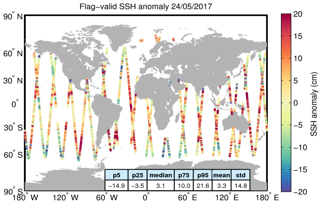
Figure 5. Geographical distribution of flag-valid 1-Hz SSH anomaly data over oceans and lakes for 24/05/2017. The statistical values shown in the table refer to the SSH anomaly in cm and are calculated over all measurements shown in the figure.
