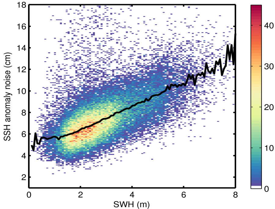
Figure 9. 2D histogram showing flag-valid SSH anomaly noise as a function of SWH for 24/05/2017. The black line denotes the median SSH anomaly noise as a function of SWH.
