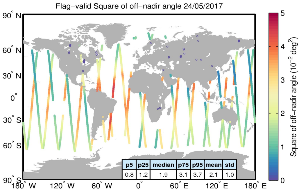
Figure 37. Geographical distribution of flag-valid mispointing data over oceans and lakes for 24/05/2017. The statistical values shown in the table refer to the mispointing in 10^{-2} deg 2 and are calculated over all measurements shown in the figure.
