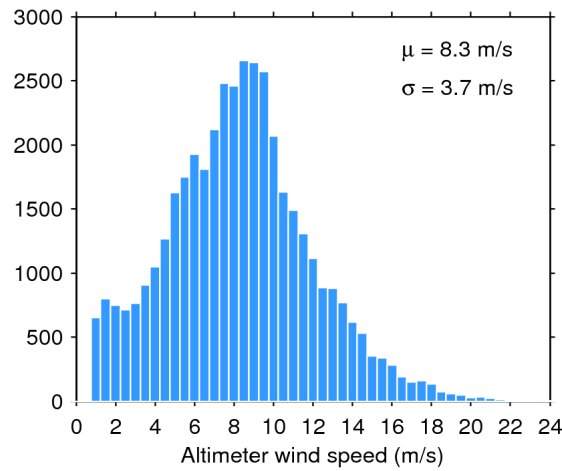
Figure 33. Histogram of flag-valid wind over oceans and lakes for 24/05/2017. The mean ( \mu ) and standard deviation ( \sigma ) are also shown. Note that values larger than 24 m/s are excluded from the histogram for the sake of readability but not from the computation of \mu and \sigma .
