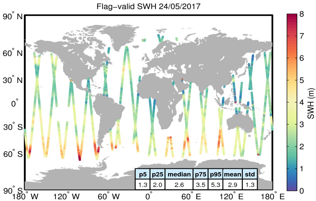
Figure 15. Geographical distribution of flag-valid SWH data over oceans and lakes for 24/05/2017. The statistical values shown in the table refer to the SWH in m and are calculated over all measurements shown in the figure.
