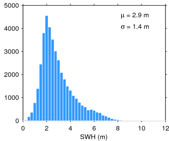
Figure 17. Histogram of flag-valid SWH over oceans and lakes for 23/05/2017. The mean ( \mu ) and standard deviation ( \sigma ) are also shown. Note that values larger than 12 m are excluded from the histogram for the sake of readability but not from the computation of \mu and \sigma .
