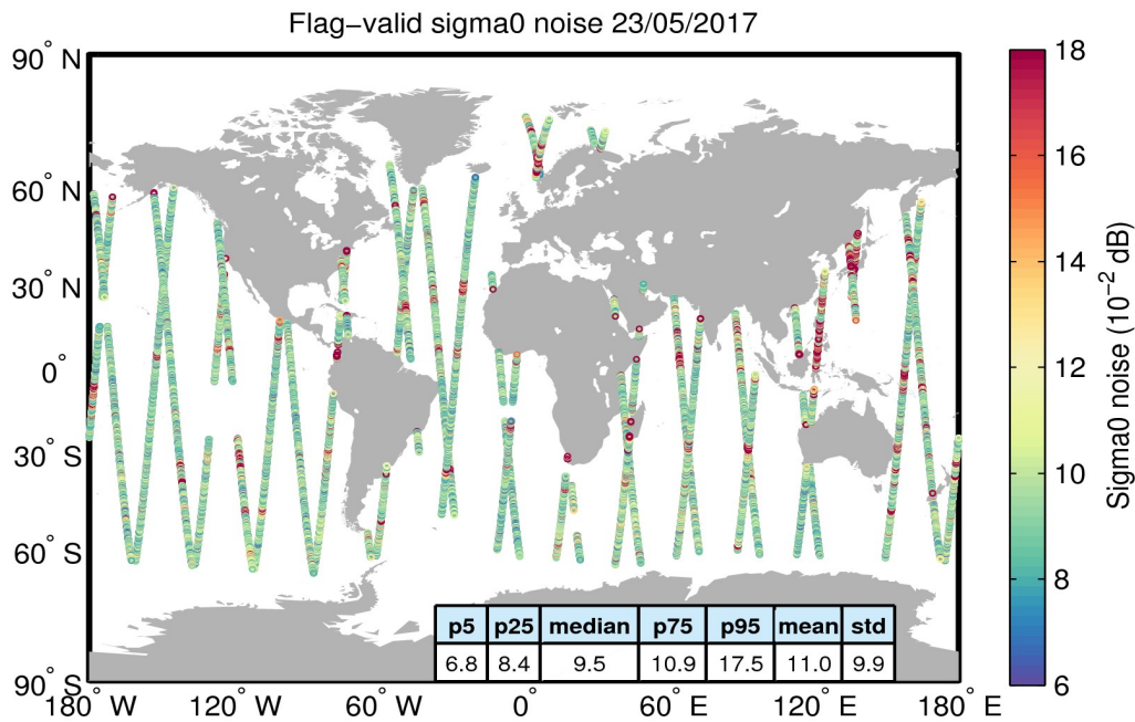
Figure 26. Geographical distribution of flag-valid 20-Hz sigma0 measurement noise over oceans and lakes for 23/05/2017. The statistical values shown in the table refer to the sigma0 noise and are calculated over all measurements shown in the figure.
