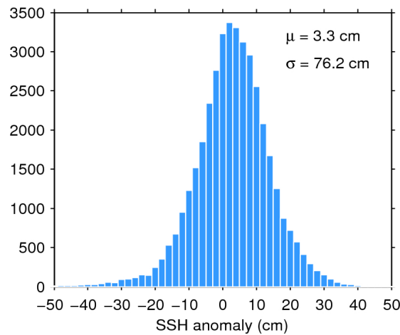
Figure 7. Histogram of flag-valid SSH anomaly over oceans and lakes for 23/05/2017. The mean ( \mu ) and standard deviation ( \sigma ) are also shown. Note that values outside [-50 50] cm are excluded from the histogram for the sake of readability but not from the computation of \mu and \sigma .
