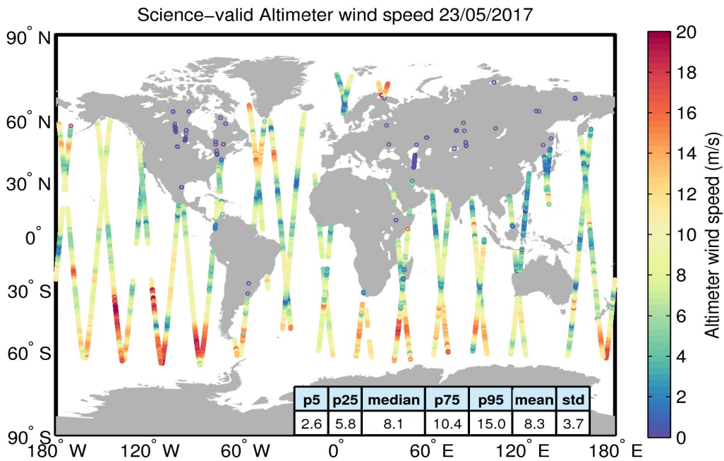
Figure 34. Geographical distribution of science-valid wind data over oceans and lakes for 23/05/2017. The statistical values shown in the table refer to the wind in m/s and are calculated over all measurements shown in the figure. Gray circles denote records that have been rejected based on the editing criteria described in Table 5.
