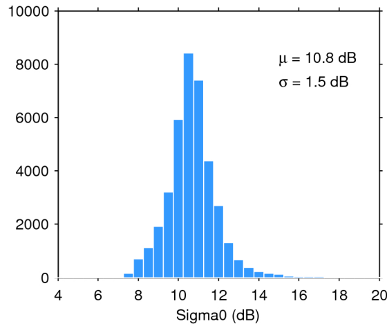
Figure 28. Histogram of science-valid sigma0 over oceans and lakes for 23/05/2017. The mean ( \mu ) and standard deviation ( \sigma ) are also shown. Note that values outside [4 20] dB are excluded from the histogram for the sake of readability but not from the computation of \mu and \sigma .
