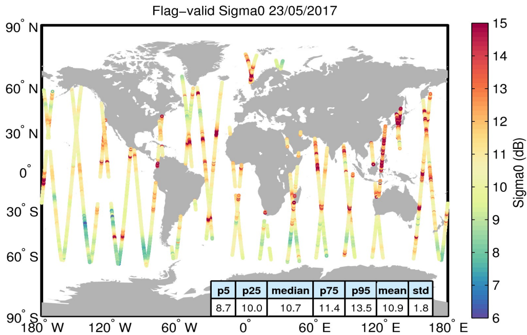
Figure 23. Geographical distribution of flag-valid sigma0 data over oceans and lakes for 23/05/2017. The statistical values shown in the table refer to the sigma0 in dB and are calculated over all measurements shown in the figure.
