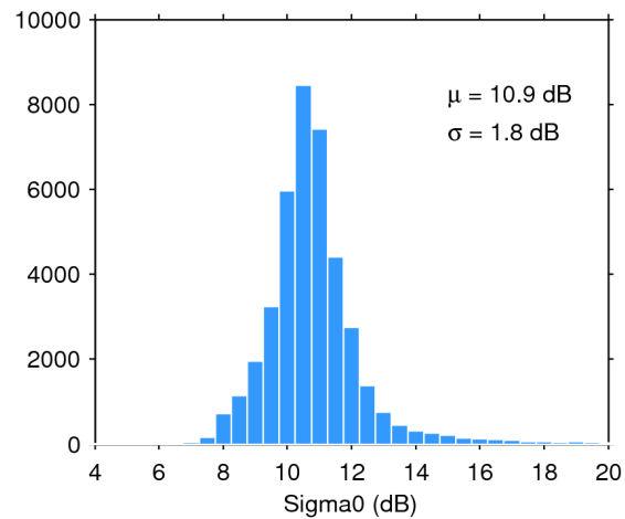
Figure 25. Histogram of flag-valid sigma0 over oceans and lakes for 23/05/2017. The mean ( \mu ) and standard deviation ( \sigma ) are also shown. Note that values outside [4 20] dB are excluded from the histogram for the sake of readability but not from the computation of \mu and \sigma .
