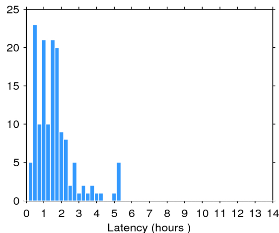
Figure 2. Histogram of the data latency for 23/05/2017. The y-axis denotes the number of files that are made available with a delay of x-hours with respect to the mean time of the records stored in the file.
