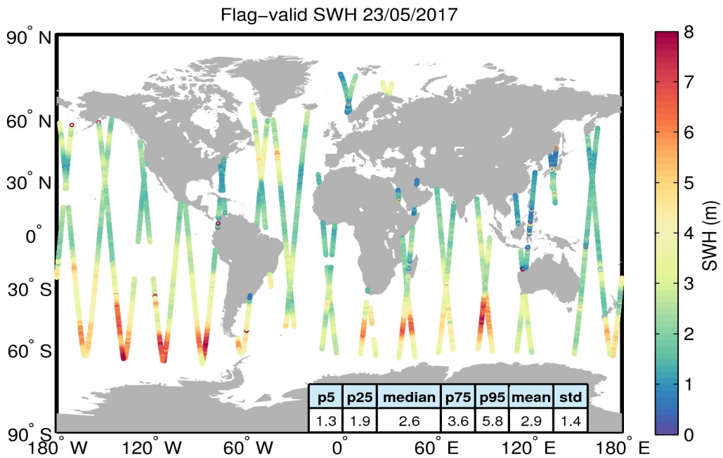
Figure 15. Geographical distribution of flag-valid SWH data over oceans and lakes for 23/05/2017. The statistical values shown in the table refer to the SWH in m and are calculated over all measurements shown in the figure.
