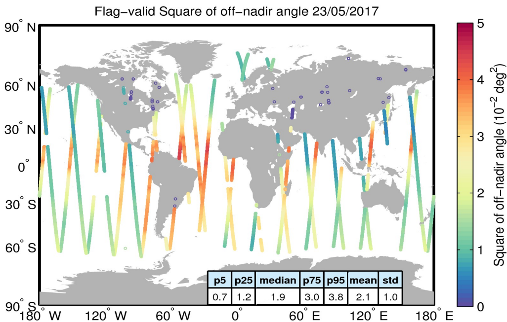
Figure 37. Geographical distribution of flag-valid mispointing data over oceans and lakes for 23/05/2017. The statistical values shown in the table refer to the mispointing in 10^{-2} deg 2 and are calculated over all measurements shown in the figure.
