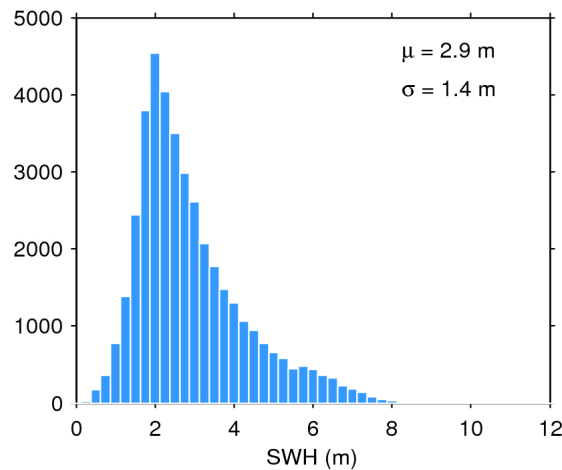
Figure 20. Histogram of science-valid SWH over oceans and lakes for 23/05/2017. The mean ( \mu ) and standard deviation ( \sigma ) are also shown. Note that values larger than 12 m are excluded from the histogram for the sake of readability but not from the computation of \mu and \sigma .
