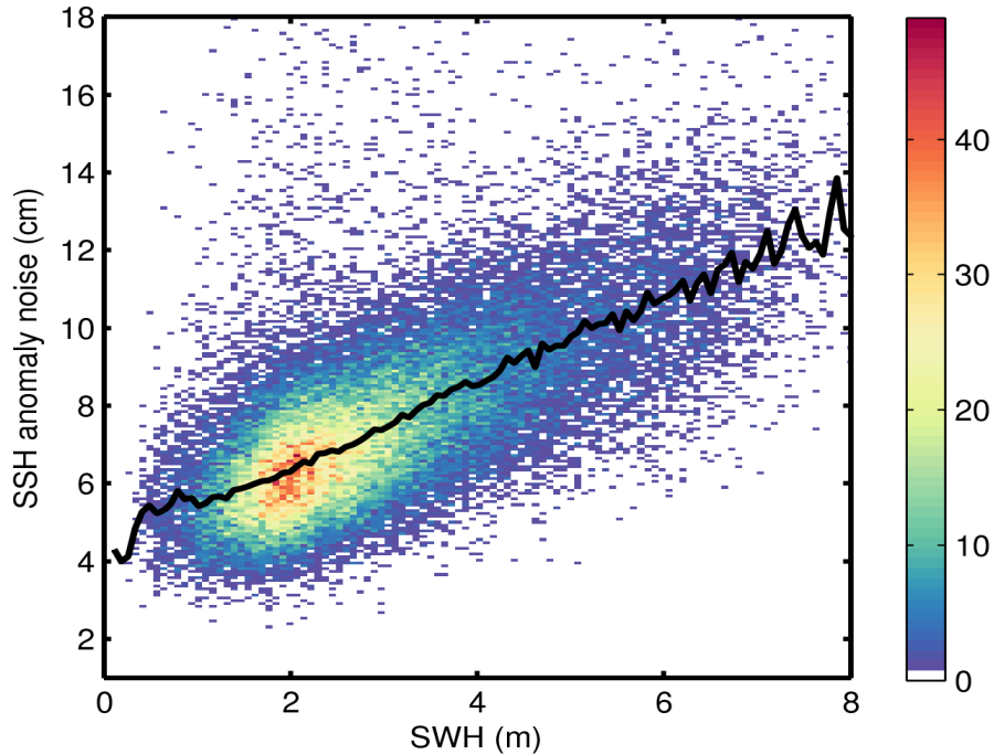
Figure 9. 2D histogram showing flag-valid SSH anomaly noise as a function of SWH for 23/05/2017. The black line denotes the median SSH anomaly noise as a function of SWH.
