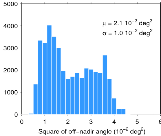
Figure 39. Histogram of flag-valid mispointing over oceans and lakes for 23/05/2017. The mean ( \mu ) and standard deviation ( \sigma ) are also shown. Note that values larger than 6 \cdot 10^{-2} \text{ deg}^2 are excluded from the histogram for the sake of readability but not from the computation of \mu and \sigma .
