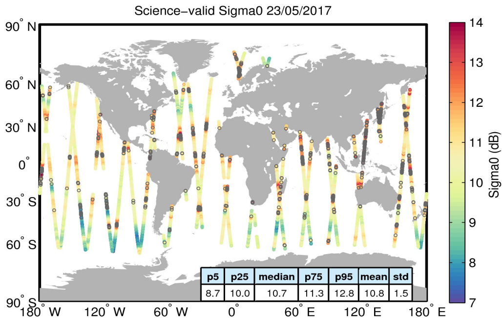
Figure 27. Geographical distribution of science-valid sigma0 data over oceans and lakes for 23/05/2017. The statistical values shown in the table refer to the sigma0 in dB and are calculated over all measurements shown in the figure. Gray circles denote records that have been rejected based on the editing criteria described in Table 4.
