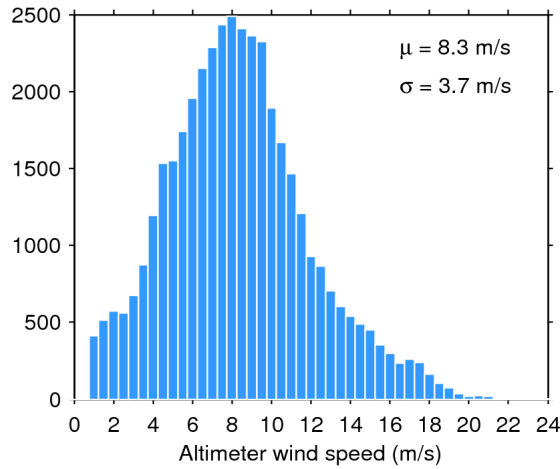
Figure 33. Histogram of flag-valid wind over oceans and lakes for 23/05/2017. The mean ( \mu ) and standard deviation ( \sigma ) are also shown. Note that values larger than 24 m/s are excluded from the histogram for the sake of readability but not from the computation of \mu and \sigma .
