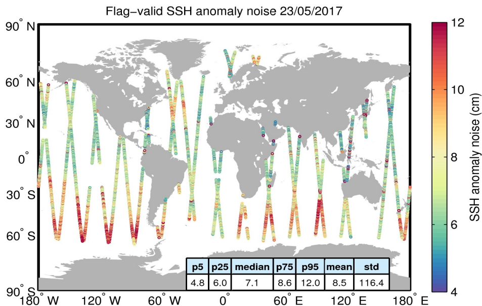
Figure 8. Geographical distribution of flag-valid 20-Hz SSH anomaly measurement noise over oceans and lakes for 23/05/2017. The statistical values shown in the table refer to the SSH anomaly noise and are calculated over all measurements shown in the figure.
