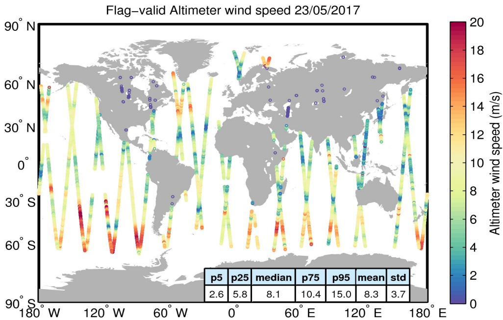
Figure 31. Geographical distribution of flag-valid wind data over oceans and lakes for 23/05/2017. The statistical values shown in the table refer to the wind in m/s and are calculated over all measurements shown in the figure.
