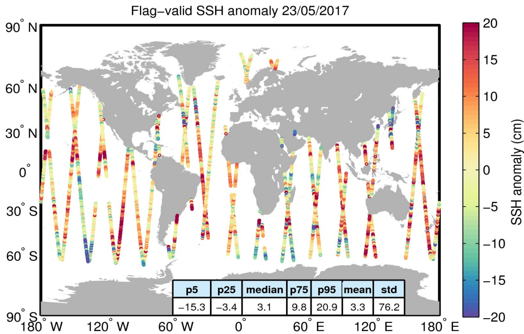
Figure 5. Geographical distribution of flag-valid 1-Hz SSH anomaly data over oceans and lakes for 23/05/2017. The statistical values shown in the table refer to the SSH anomaly in cm and are calculated over all measurements shown in the figure.
