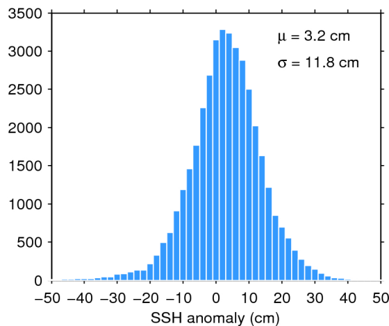
Figure 11. Histogram of science-valid SSH anomaly over oceans and lakes for 23/05/2017. The mean ( \mu ) and standard deviation ( \sigma ) are also shown. Note that values outside [-50 50] cm are excluded from the histogram for the sake of readability but not from the computation of \mu and \sigma .
