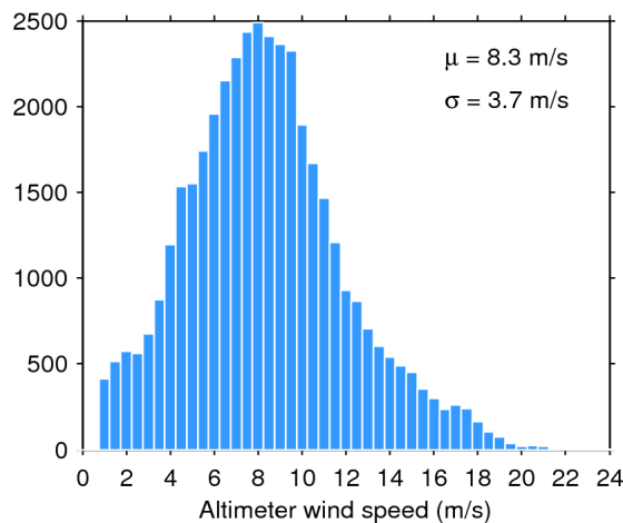
Figure 35. Histogram of science-valid wind over oceans and lakes for 23/05/2017. The mean ( \mu ) and standard deviation ( \sigma ) are also shown. Note that values larger than 24 m/s are excluded from the histogram for the sake of readability but not from the computation of \mu and \sigma .
