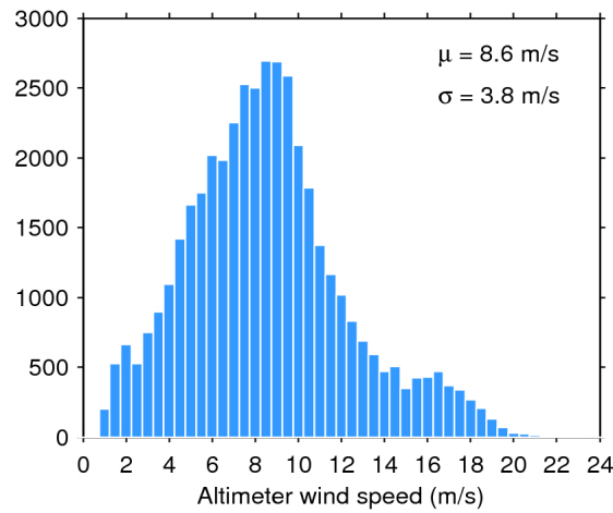
Figure 33. Histogram of flag-valid wind over oceans and lakes for 22/05/2017. The mean ( \mu ) and standard deviation ( \sigma ) are also shown. Note that values larger than 24 m/s are excluded from the histogram for the sake of readability but not from the computation of \mu and \sigma .
