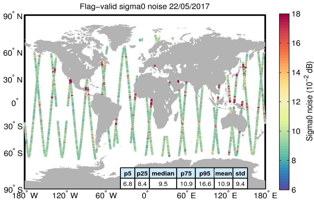
Figure 26. Geographical distribution of flag-valid 20-Hz sigma0 measurement noise over oceans and lakes for 22/05/2017. The statistical values shown in the table refer to the sigma0 noise and are calculated over all measurements shown in the figure.
