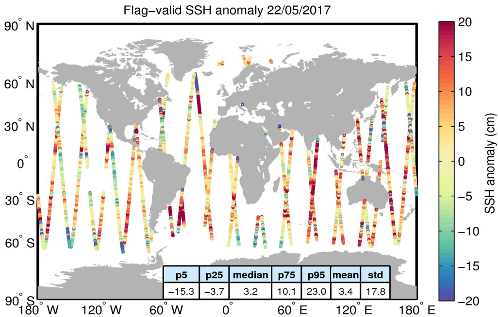
Figure 5. Geographical distribution of flag-valid 1-Hz SSH anomaly data over oceans and lakes for 22/05/2017. The statistical values shown in the table refer to the SSH anomaly in cm and are calculated over all measurements shown in the figure.
