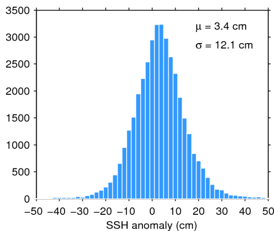
Figure 11. Histogram of science-valid SSH anomaly over oceans and lakes for 22/05/2017. The mean ( \mu ) and standard deviation ( \sigma ) are also shown. Note that values outside [-50 50] cm are excluded from the histogram for the sake of readability but not from the computation of \mu and \sigma .
