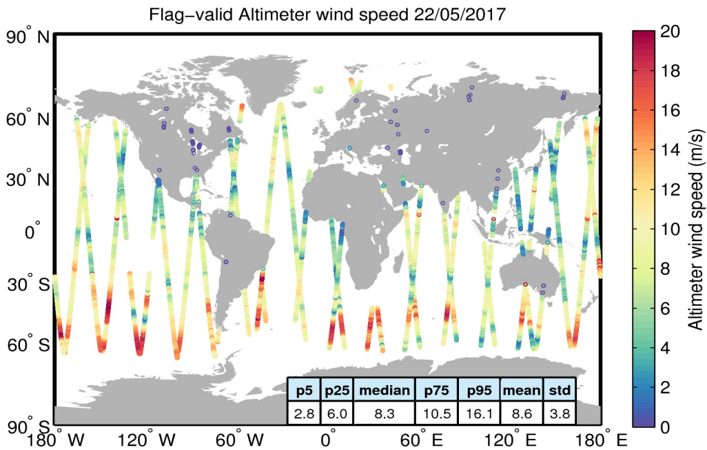
Figure 31. Geographical distribution of flag-valid wind data over oceans and lakes for 22/05/2017. The statistical values shown in the table refer to the wind in m/s and are calculated over all measurements shown in the figure.
