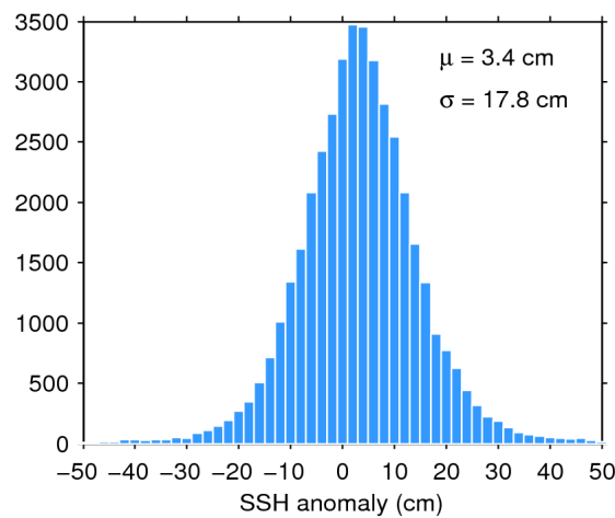
Figure 7. Histogram of flag-valid SSH anomaly over oceans and lakes for 22/05/2017. The mean ( \mu ) and standard deviation ( \sigma ) are also shown. Note that values outside [-50 50] cm are excluded from the histogram for the sake of readability but not from the computation of \mu and \sigma .
