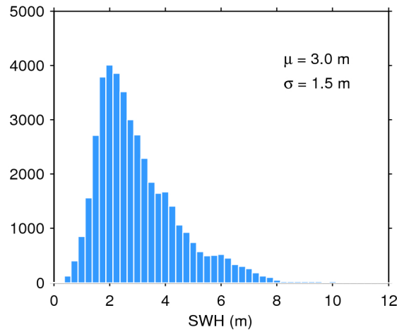
Figure 17. Histogram of flag-valid SWH over oceans and lakes for 22/05/2017. The mean ( \mu ) and standard deviation ( \sigma ) are also shown. Note that values larger than 12 m are excluded from the histogram for the sake of readability but not from the computation of \mu and \sigma .
