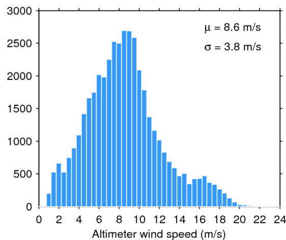
Figure 35. Histogram of science-valid wind over oceans and lakes for 22/05/2017. The mean ( \mu ) and standard deviation ( \sigma ) are also shown. Note that values larger than 24 m/s are excluded from the histogram for the sake of readability but not from the computation of \mu and \sigma .
