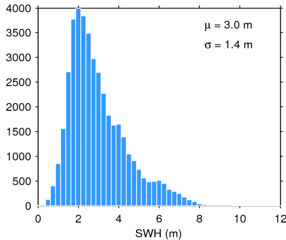
Figure 20. Histogram of science-valid SWH over oceans and lakes for 22/05/2017. The mean ( \mu ) and standard deviation ( \sigma ) are also shown. Note that values larger than 12 m are excluded from the histogram for the sake of readability but not from the computation of \mu and \sigma .
