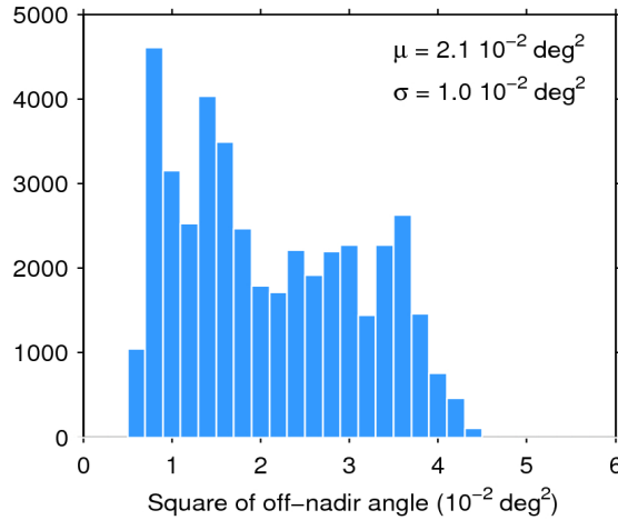
Figure 39. Histogram of flag-valid mispointing over oceans and lakes for 22/05/2017. The mean ( \mu ) and standard deviation ( \sigma ) are also shown. Note that values larger than 6 \cdot 10^{-2} \text{ deg}^2 are excluded from the histogram for the sake of readability but not from the computation of \mu and \sigma .
