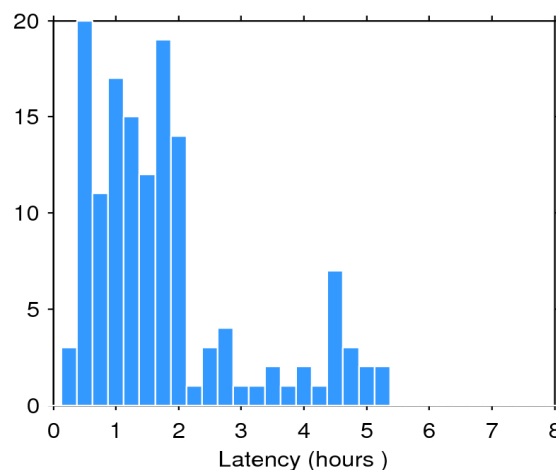
Figure 2. Histogram of the data latency for 22/05/2017. The y-axis denotes the number of files that are made available with a delay of x-hours with respect to the mean time of the records stored in the file.
