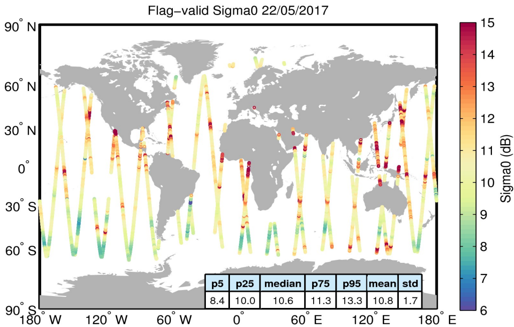
Figure 23. Geographical distribution of flag-valid sigma0 data over oceans and lakes for 22/05/2017. The statistical values shown in the table refer to the sigma0 in dB and are calculated over all measurements shown in the figure.
