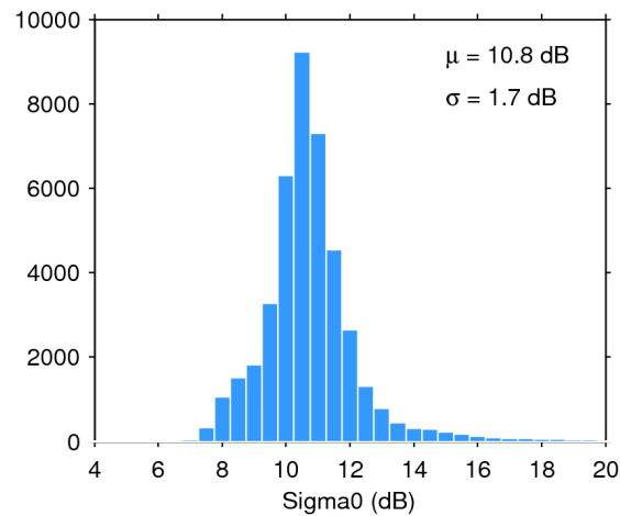
Figure 25. Histogram of flag-valid sigma0 over oceans and lakes for 22/05/2017. The mean ( \mu ) and standard deviation ( \sigma ) are also shown. Note that values outside [4 20] dB are excluded from the histogram for the sake of readability but not from the computation of \mu and \sigma .
