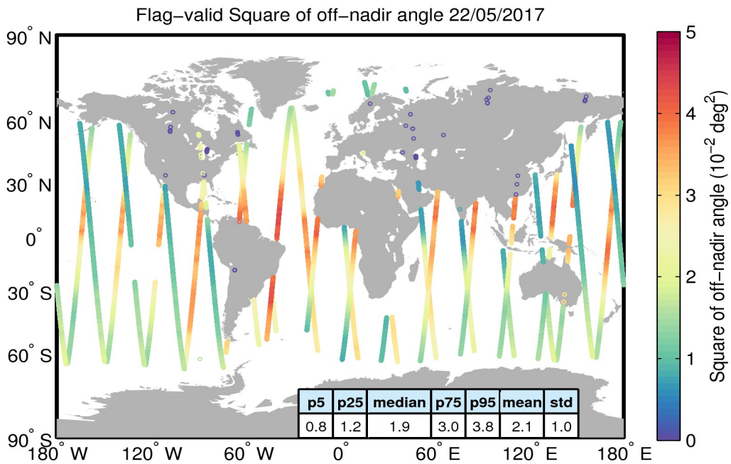
Figure 37. Geographical distribution of flag-valid mispointing data over oceans and lakes for 22/05/2017. The statistical values shown in the table refer to the mispointing in 10^{-2} deg 2 and are calculated over all measurements shown in the figure.
