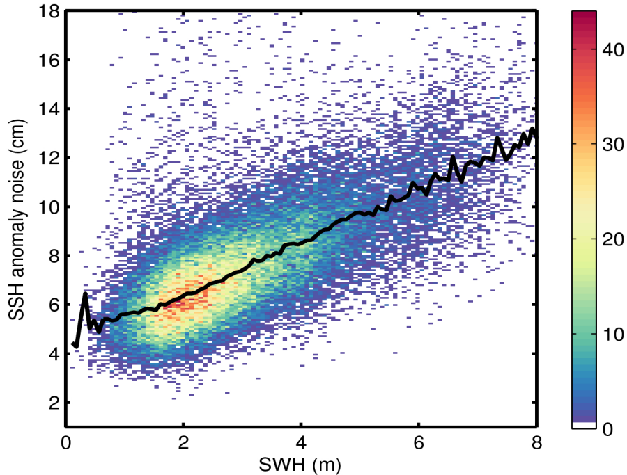
Figure 9. 2D histogram showing flag-valid SSH anomaly noise as a function of SWH for 22/05/2017. The black line denotes the median SSH anomaly noise as a function of SWH.
