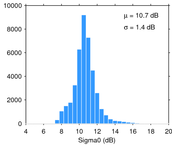
Figure 28. Histogram of science-valid sigma0 over oceans and lakes for 22/05/2017. The mean ( \mu ) and standard deviation ( \sigma ) are also shown. Note that values outside [4 20] dB are excluded from the histogram for the sake of readability but not from the computation of \mu and \sigma .
