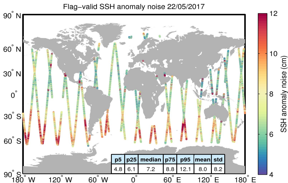
Figure 8. Geographical distribution of flag-valid 20-Hz SSH anomaly measurement noise over oceans and lakes for 22/05/2017. The statistical values shown in the table refer to the SSH anomaly noise and are calculated over all measurements shown in the figure.
