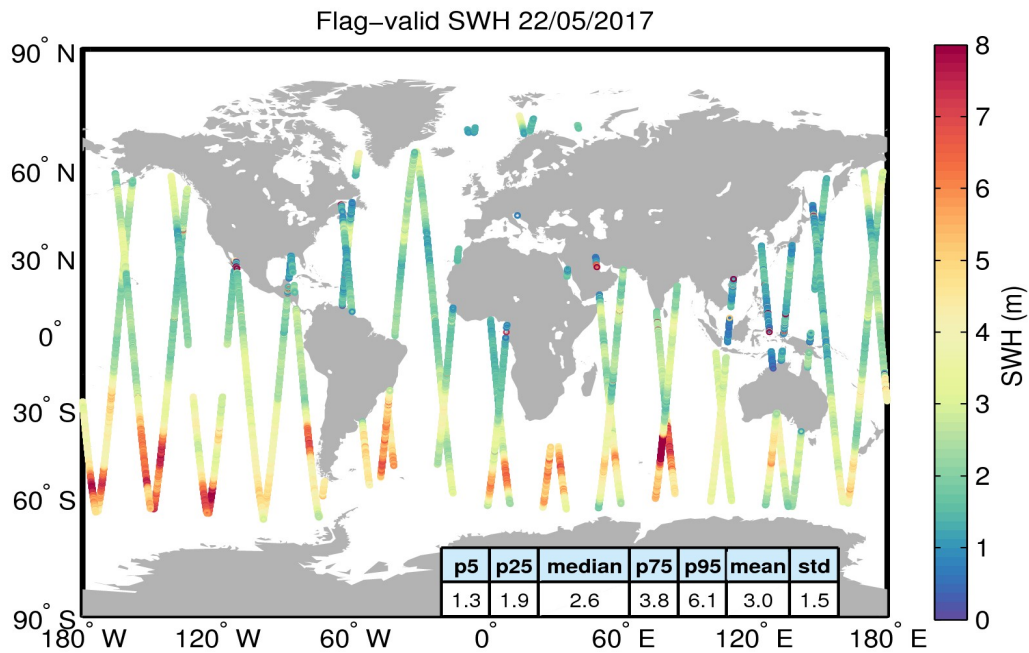
Figure 15. Geographical distribution of flag-valid SWH data over oceans and lakes for 22/05/2017. The statistical values shown in the table refer to the SWH in m and are calculated over all measurements shown in the figure.
