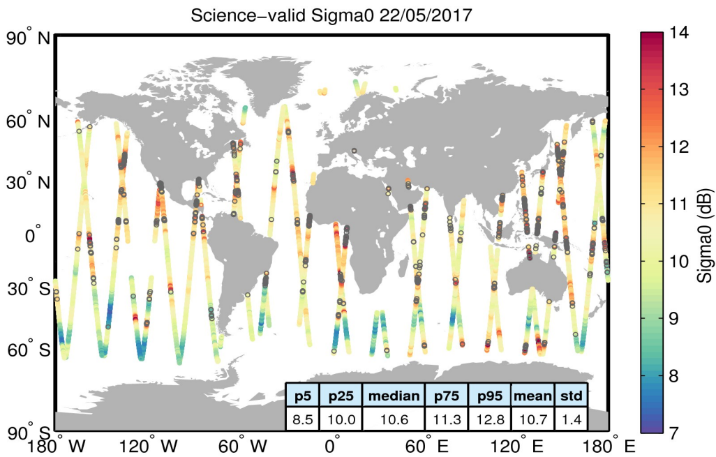
Figure 27. Geographical distribution of science-valid sigma0 data over oceans and lakes for 22/05/2017. The statistical values shown in the table refer to the sigma0 in dB and are calculated over all measurements shown in the figure. Gray circles denote records that have been rejected based on the editing criteria described in Table 4.
