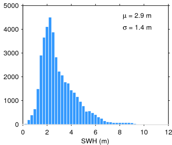
Figure 20. Histogram of science-valid SWH over oceans and lakes for 20/05/2017. The mean ( \mu ) and standard deviation ( \sigma ) are also shown. Note that values larger than 12 m are excluded from the histogram for the sake of readability but not from the computation of \mu and \sigma .
