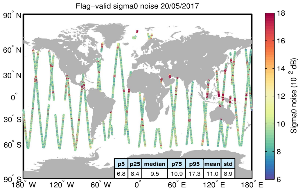
Figure 26. Geographical distribution of flag-valid 20-Hz sigma0 measurement noise over oceans and lakes for 20/05/2017. The statistical values shown in the table refer to the sigma0 noise and are calculated over all measurements shown in the figure.
