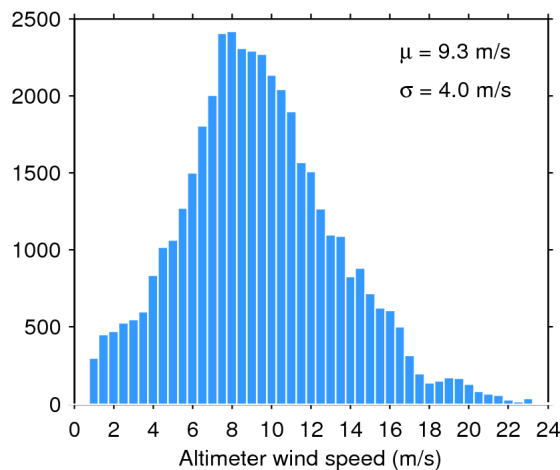
Figure 35. Histogram of science-valid wind over oceans and lakes for 20/05/2017. The mean ( \mu ) and standard deviation ( \sigma ) are also shown. Note that values larger than 24 m/s are excluded from the histogram for the sake of readability but not from the computation of \mu and \sigma .
