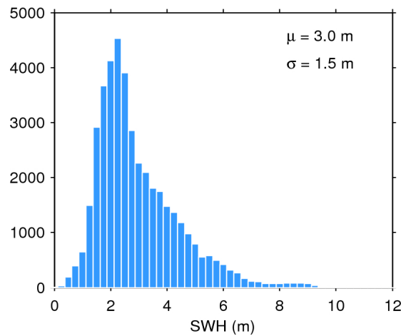
Figure 17. Histogram of flag-valid SWH over oceans and lakes for 20/05/2017. The mean ( \mu ) and standard deviation ( \sigma ) are also shown. Note that values larger than 12 m are excluded from the histogram for the sake of readability but not from the computation of \mu and \sigma .
