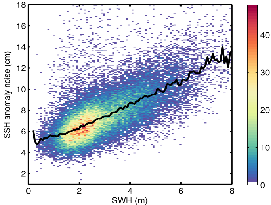
Figure 9. 2D histogram showing flag-valid SSH anomaly noise as a function of SWH for 20/05/2017. The black line denotes the median SSH anomaly noise as a function of SWH.
