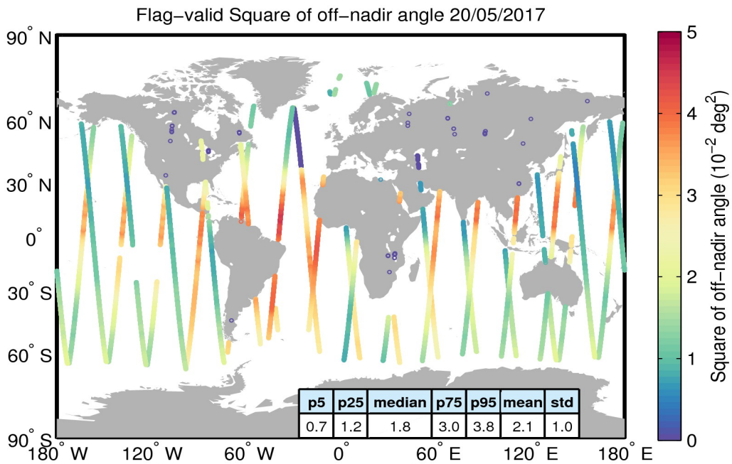
Figure 37. Geographical distribution of flag-valid mispointing data over oceans and lakes for 20/05/2017. The statistical values shown in the table refer to the mispointing in 10^{-2} deg 2 and are calculated over all measurements shown in the figure.
