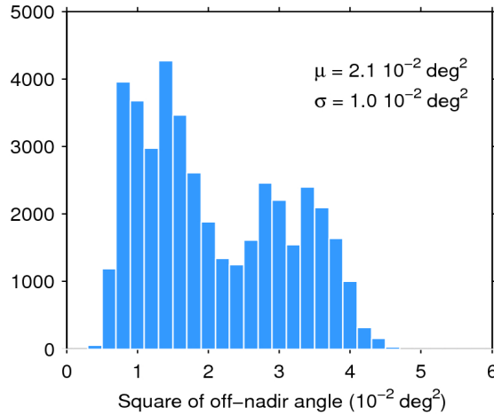
Figure 39. Histogram of flag-valid mispointing over oceans and lakes for 20/05/2017. The mean ( \mu ) and standard deviation ( \sigma ) are also shown. Note that values larger than 6 \cdot 10^{-2} \text{ deg}^2 are excluded from the histogram for the sake of readability but not from the computation of \mu and \sigma .
