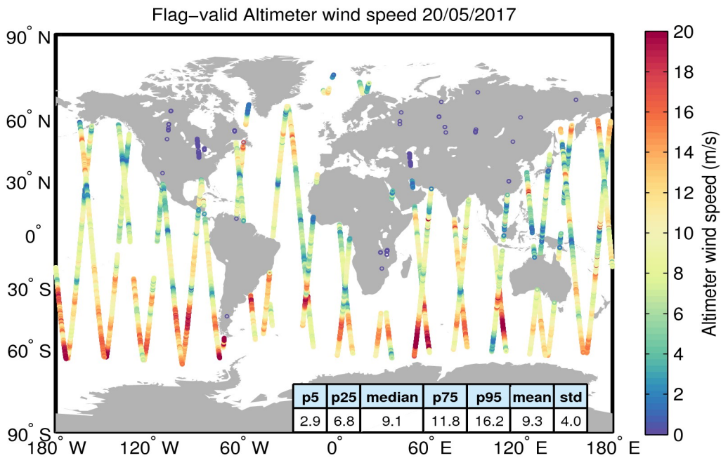
Figure 31. Geographical distribution of flag-valid wind data over oceans and lakes for 20/05/2017. The statistical values shown in the table refer to the wind in m/s and are calculated over all measurements shown in the figure.
