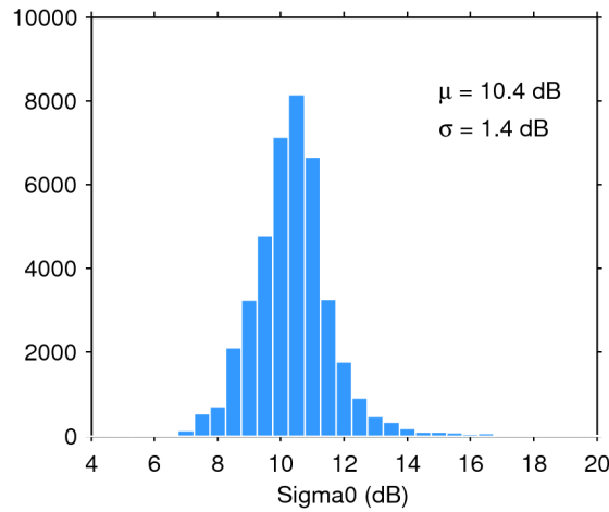
Figure 28. Histogram of science-valid sigma0 over oceans and lakes for 20/05/2017. The mean ( \mu ) and standard deviation ( \sigma ) are also shown. Note that values outside [4 20] dB are excluded from the histogram for the sake of readability but not from the computation of \mu and \sigma .
