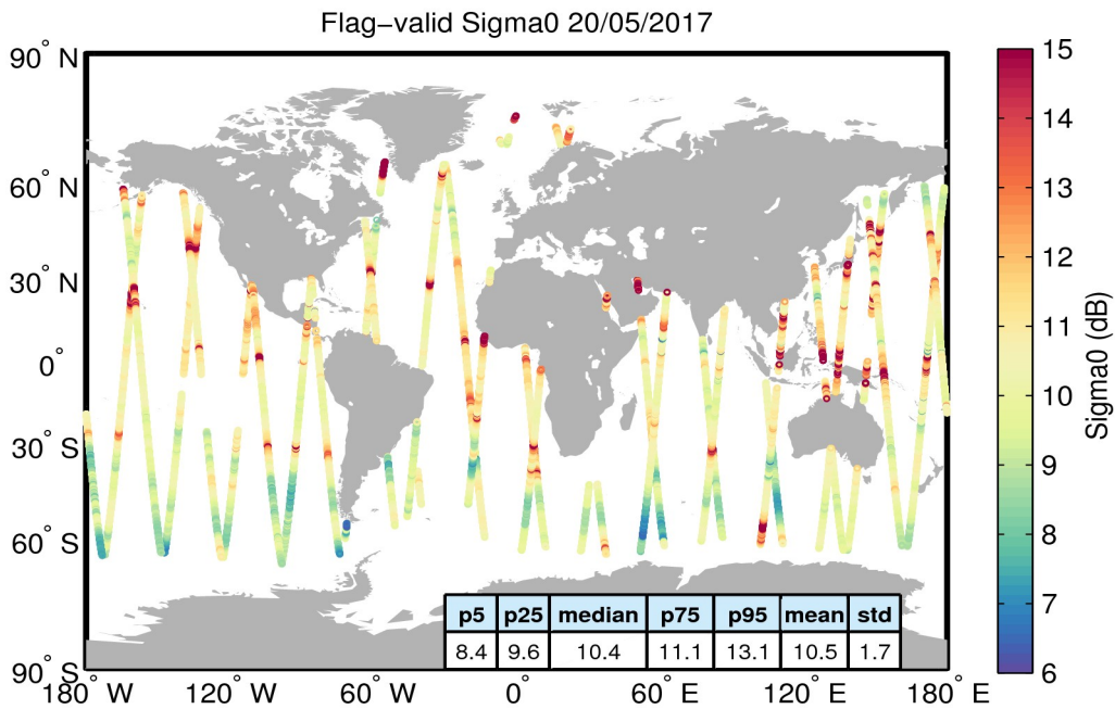
Figure 23. Geographical distribution of flag-valid sigma0 data over oceans and lakes for 20/05/2017. The statistical values shown in the table refer to the sigma0 in dB and are calculated over all measurements shown in the figure.
