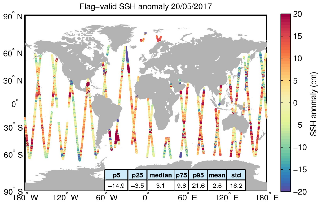
Figure 5. Geographical distribution of flag-valid 1-Hz SSH anomaly data over oceans and lakes for 20/05/2017. The statistical values shown in the table refer to the SSH anomaly in cm and are calculated over all measurements shown in the figure.
