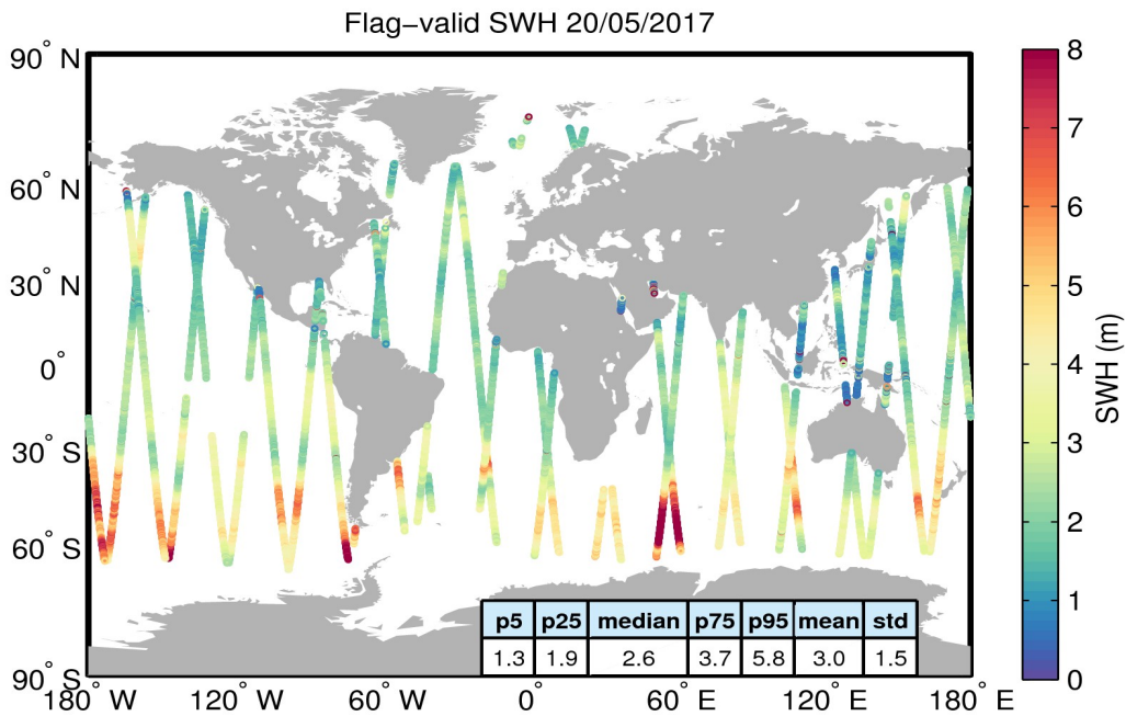
Figure 15. Geographical distribution of flag-valid SWH data over oceans and lakes for 20/05/2017. The statistical values shown in the table refer to the SWH in m and are calculated over all measurements shown in the figure.
