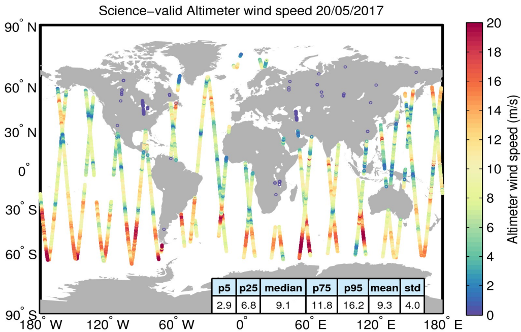
Figure 34. Geographical distribution of science-valid wind data over oceans and lakes for 20/05/2017. The statistical values shown in the table refer to the wind in m/s and are calculated over all measurements shown in the figure. Gray circles denote records that have been rejected based on the editing criteria described in Table 5.
