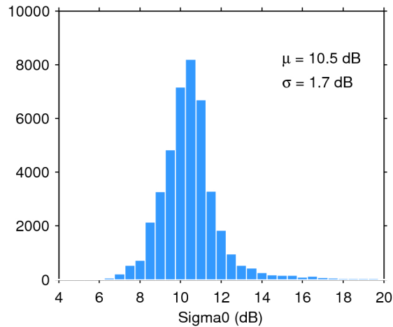
Figure 25. Histogram of flag-valid sigma0 over oceans and lakes for 20/05/2017. The mean ( \mu ) and standard deviation ( \sigma ) are also shown. Note that values outside [4 20] dB are excluded from the histogram for the sake of readability but not from the computation of \mu and \sigma .
