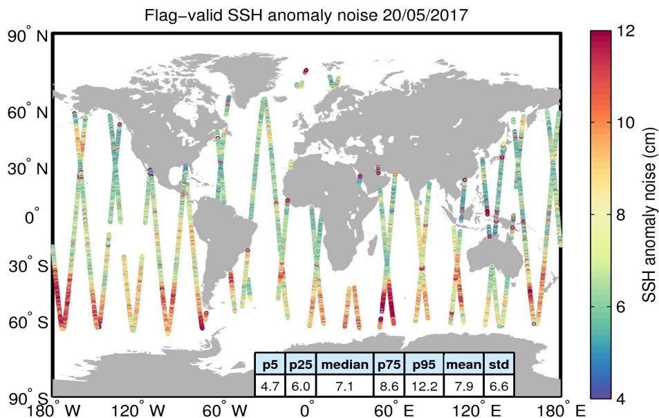
Figure 8. Geographical distribution of flag-valid 20-Hz SSH anomaly measurement noise over oceans and lakes for 20/05/2017. The statistical values shown in the table refer to the SSH anomaly noise and are calculated over all measurements shown in the figure.
