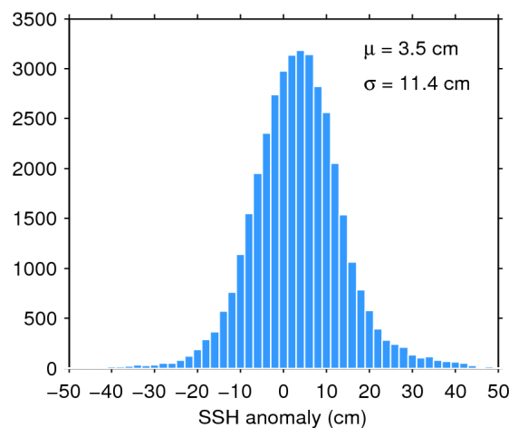
Figure 11. Histogram of science-valid SSH anomaly over oceans and lakes for 20/05/2017. The mean ( \mu ) and standard deviation ( \sigma ) are also shown. Note that values outside [-50 50] cm are excluded from the histogram for the sake of readability but not from the computation of \mu and \sigma .
