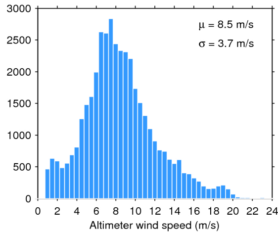
Figure 33. Histogram of flag-valid wind over oceans and lakes for 19/05/2017. The mean ( \mu ) and standard deviation ( \sigma ) are also shown. Note that values larger than 24 m/s are excluded from the histogram for the sake of readability but not from the computation of \mu and \sigma .
