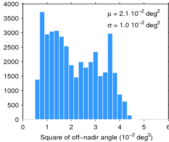
Figure 39. Histogram of flag-valid mispointing over oceans and lakes for 19/05/2017. The mean ( \mu ) and standard deviation ( \sigma ) are also shown. Note that values larger than 6 \cdot 10^{-2} \text{ deg}^2 are excluded from the histogram for the sake of readability but not from the computation of \mu and \sigma .
