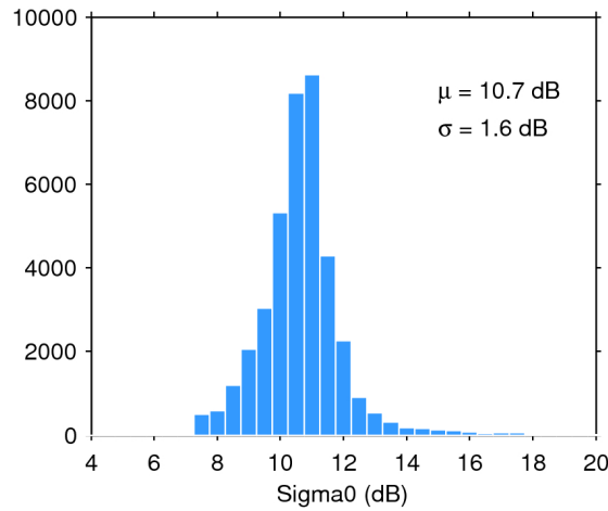
Figure 28. Histogram of science-valid sigma0 over oceans and lakes for 19/05/2017. The mean ( \mu ) and standard deviation ( \sigma ) are also shown. Note that values outside [4 20] dB are excluded from the histogram for the sake of readability but not from the computation of \mu and \sigma .
