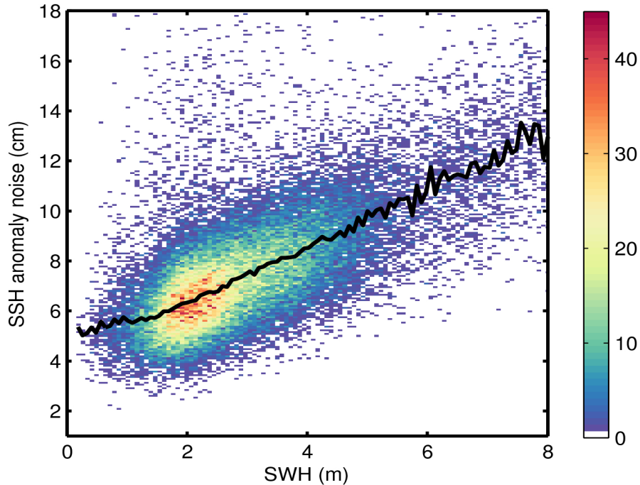
Figure 9. 2D histogram showing flag-valid SSH anomaly noise as a function of SWH for 19/05/2017. The black line denotes the median SSH anomaly noise as a function of SWH.
