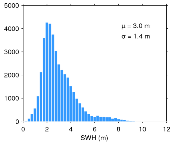
Figure 17. Histogram of flag-valid SWH over oceans and lakes for 19/05/2017. The mean ( \mu ) and standard deviation ( \sigma ) are also shown. Note that values larger than 12 m are excluded from the histogram for the sake of readability but not from the computation of \mu and \sigma .
