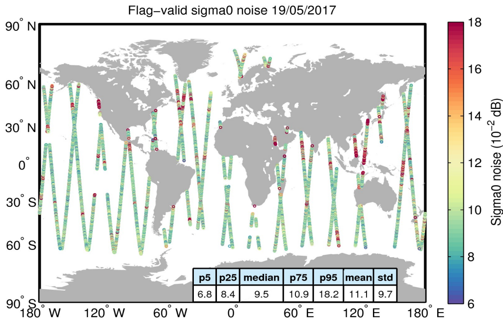
Figure 26. Geographical distribution of flag-valid 20-Hz sigma0 measurement noise over oceans and lakes for 19/05/2017. The statistical values shown in the table refer to the sigma0 noise and are calculated over all measurements shown in the figure.
