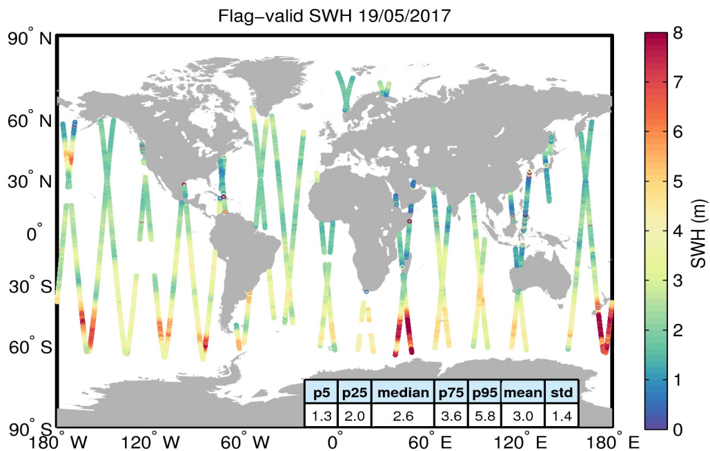
Figure 15. Geographical distribution of flag-valid SWH data over oceans and lakes for 19/05/2017. The statistical values shown in the table refer to the SWH in m and are calculated over all measurements shown in the figure.
