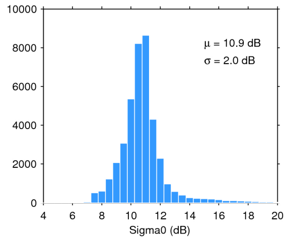
Figure 25. Histogram of flag-valid sigma0 over oceans and lakes for 19/05/2017. The mean ( \mu ) and standard deviation ( \sigma ) are also shown. Note that values outside [4 20] dB are excluded from the histogram for the sake of readability but not from the computation of \mu and \sigma .
