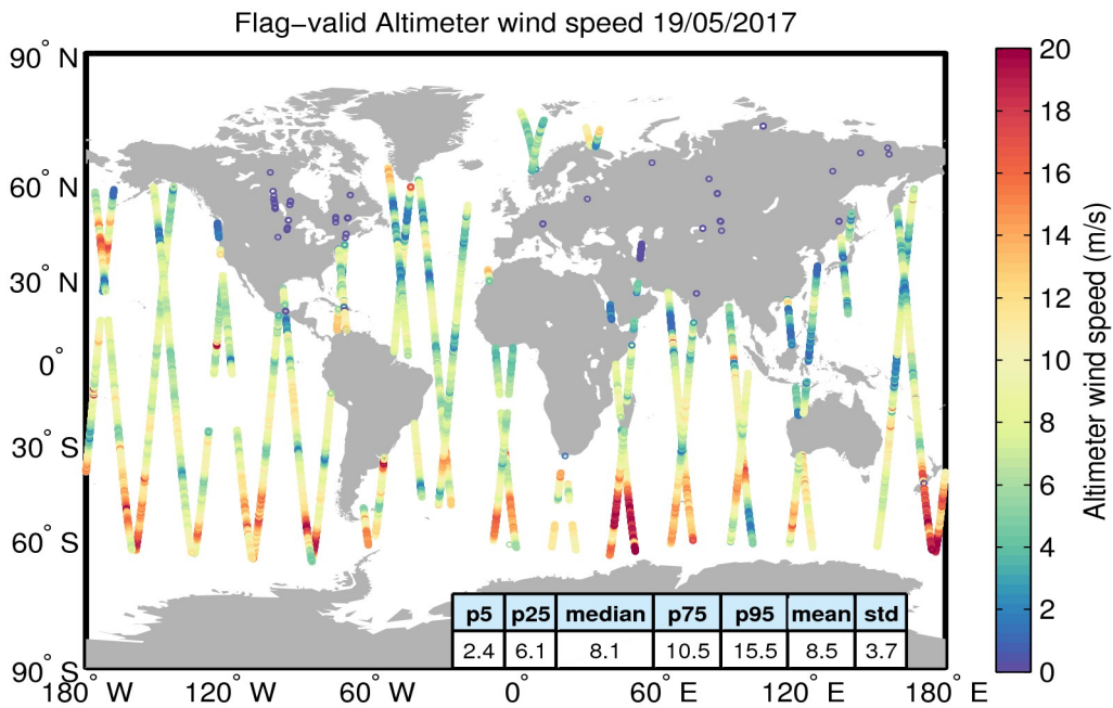
Figure 31. Geographical distribution of flag-valid wind data over oceans and lakes for 19/05/2017. The statistical values shown in the table refer to the wind in m/s and are calculated over all measurements shown in the figure.
