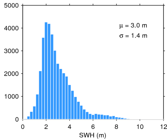
Figure 20. Histogram of science-valid SWH over oceans and lakes for 19/05/2017. The mean ( \mu ) and standard deviation ( \sigma ) are also shown. Note that values larger than 12 m are excluded from the histogram for the sake of readability but not from the computation of \mu and \sigma .
