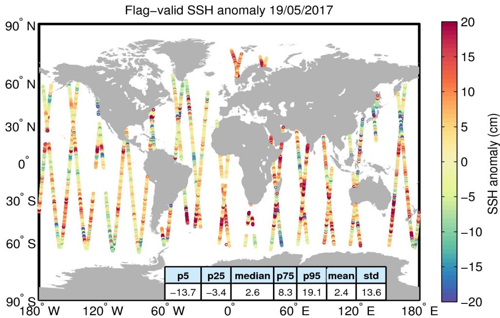
Figure 5. Geographical distribution of flag-valid 1-Hz SSH anomaly data over oceans and lakes for 19/05/2017. The statistical values shown in the table refer to the SSH anomaly in cm and are calculated over all measurements shown in the figure.
