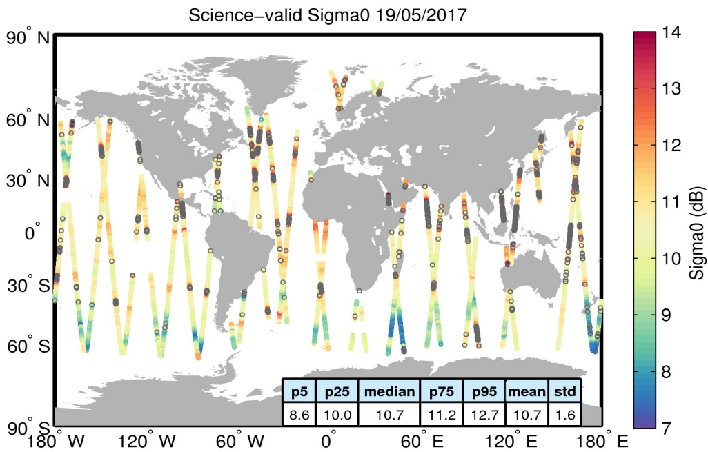
Figure 27. Geographical distribution of science-valid sigma0 data over oceans and lakes for 19/05/2017. The statistical values shown in the table refer to the sigma0 in dB and are calculated over all measurements shown in the figure. Gray circles denote records that have been rejected based on the editing criteria described in Table 4.
