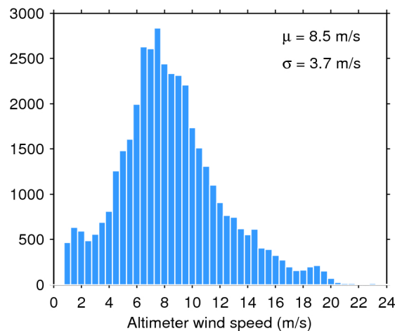
Figure 35. Histogram of science-valid wind over oceans and lakes for 19/05/2017. The mean ( \mu ) and standard deviation ( \sigma ) are also shown. Note that values larger than 24 m/s are excluded from the histogram for the sake of readability but not from the computation of \mu and \sigma .
