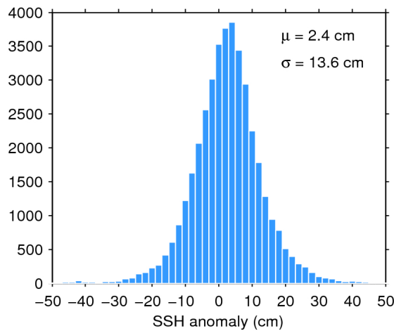
Figure 7. Histogram of flag-valid SSH anomaly over oceans and lakes for 19/05/2017. The mean ( \mu ) and standard deviation ( \sigma ) are also shown. Note that values outside [-50 50] cm are excluded from the histogram for the sake of readability but not from the computation of \mu and \sigma .
