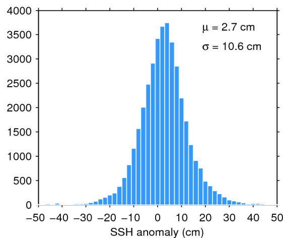
Figure 11. Histogram of science-valid SSH anomaly over oceans and lakes for 19/05/2017. The mean ( \mu ) and standard deviation ( \sigma ) are also shown. Note that values outside [-50 50] cm are excluded from the histogram for the sake of readability but not from the computation of \mu and \sigma .
