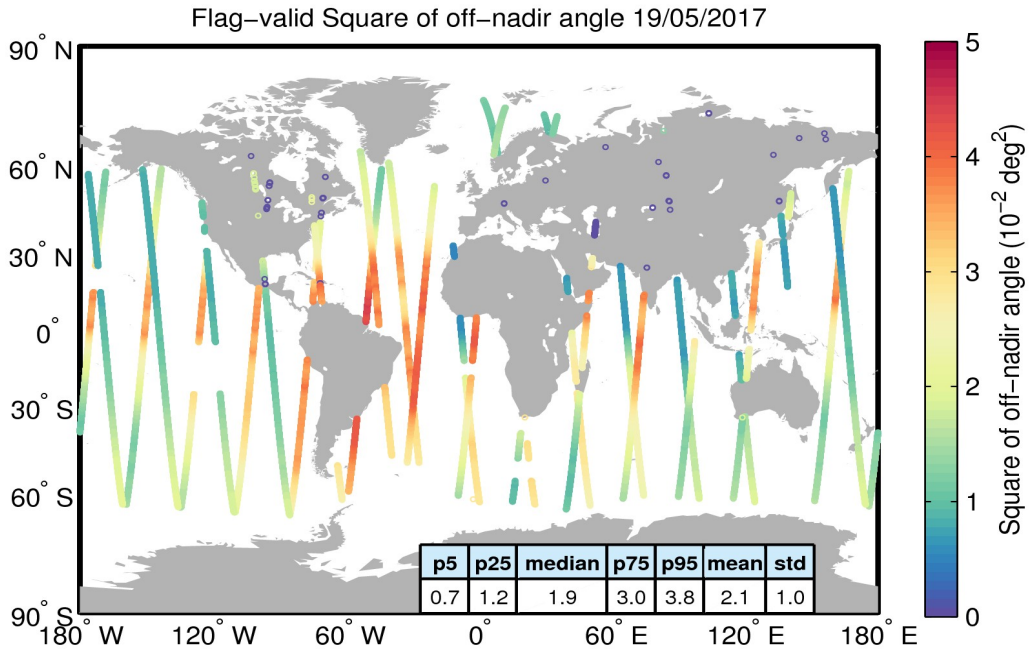
Figure 37. Geographical distribution of flag-valid mispointing data over oceans and lakes for 19/05/2017. The statistical values shown in the table refer to the mispointing in 10^{-2} deg 2 and are calculated over all measurements shown in the figure.
