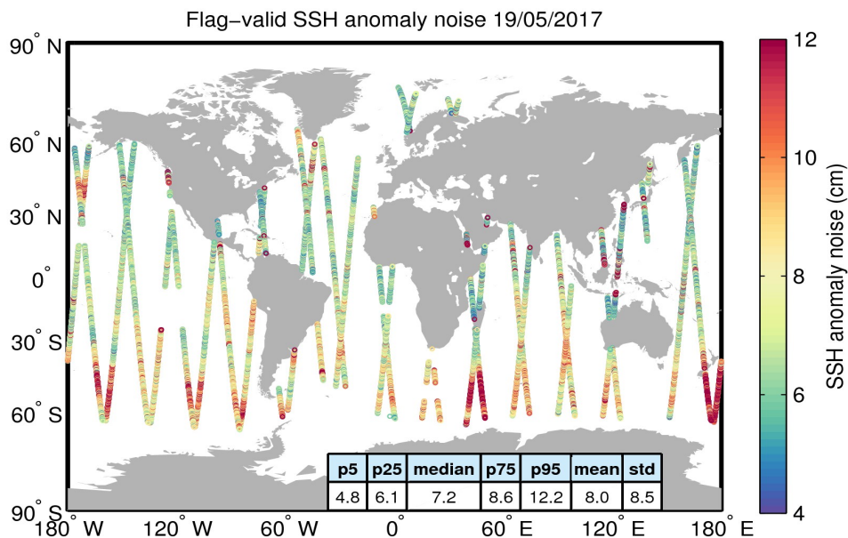
Figure 8. Geographical distribution of flag-valid 20-Hz SSH anomaly measurement noise over oceans and lakes for 19/05/2017. The statistical values shown in the table refer to the SSH anomaly noise and are calculated over all measurements shown in the figure.
