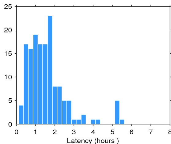
Figure 2. Histogram of the data latency for 19/05/2017. The y-axis denotes the number of files that are made available with a delay of x-hours with respect to the mean time of the records stored in the file.
