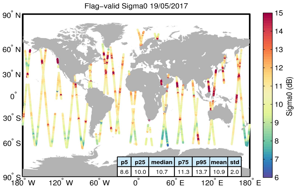
Figure 23. Geographical distribution of flag-valid sigma0 data over oceans and lakes for 19/05/2017. The statistical values shown in the table refer to the sigma0 in dB and are calculated over all measurements shown in the figure.
