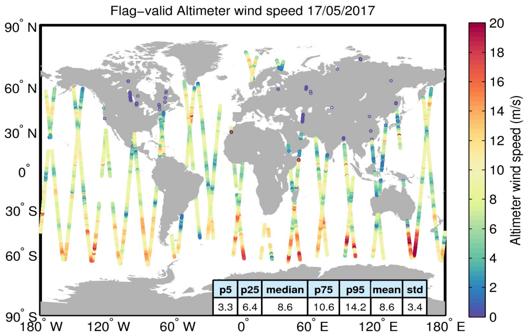
Figure 31. Geographical distribution of flag-valid wind data over oceans and lakes for 17/05/2017. The statistical values shown in the table refer to the wind in m/s and are calculated over all measurements shown in the figure.
