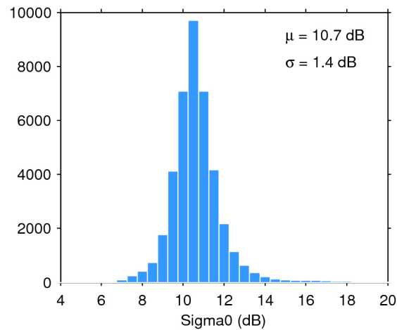
Figure 25. Histogram of flag-valid sigma0 over oceans and lakes for 17/05/2017. The mean ( \mu ) and standard deviation ( \sigma ) are also shown. Note that values outside [4 20] dB are excluded from the histogram for the sake of readability but not from the computation of \mu and \sigma .
