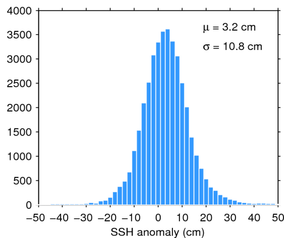
Figure 11. Histogram of science-valid SSH anomaly over oceans and lakes for 17/05/2017. The mean ( \mu ) and standard deviation ( \sigma ) are also shown. Note that values outside [-50 50] cm are excluded from the histogram for the sake of readability but not from the computation of \mu and \sigma .
