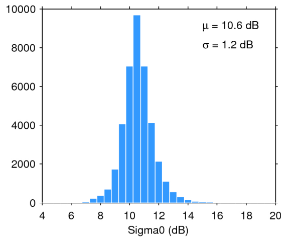
Figure 28. Histogram of science-valid sigma0 over oceans and lakes for 17/05/2017. The mean ( \mu ) and standard deviation ( \sigma ) are also shown. Note that values outside [4 20] dB are excluded from the histogram for the sake of readability but not from the computation of \mu and \sigma .
