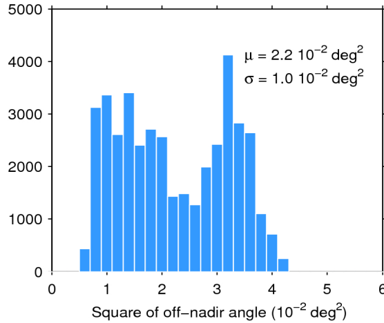
Figure 39. Histogram of flag-valid mispointing over oceans and lakes for 17/05/2017. The mean ( \mu ) and standard deviation ( \sigma ) are also shown. Note that values larger than 6 \cdot 10^{-2} \text{ deg}^2 are excluded from the histogram for the sake of readability but not from the computation of \mu and \sigma .
