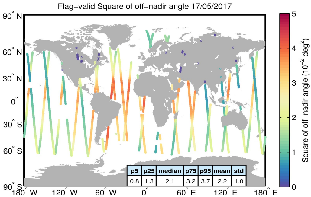
Figure 37. Geographical distribution of flag-valid mispointing data over oceans and lakes for 17/05/2017. The statistical values shown in the table refer to the mispointing in 10^{-2} deg 2 and are calculated over all measurements shown in the figure.
