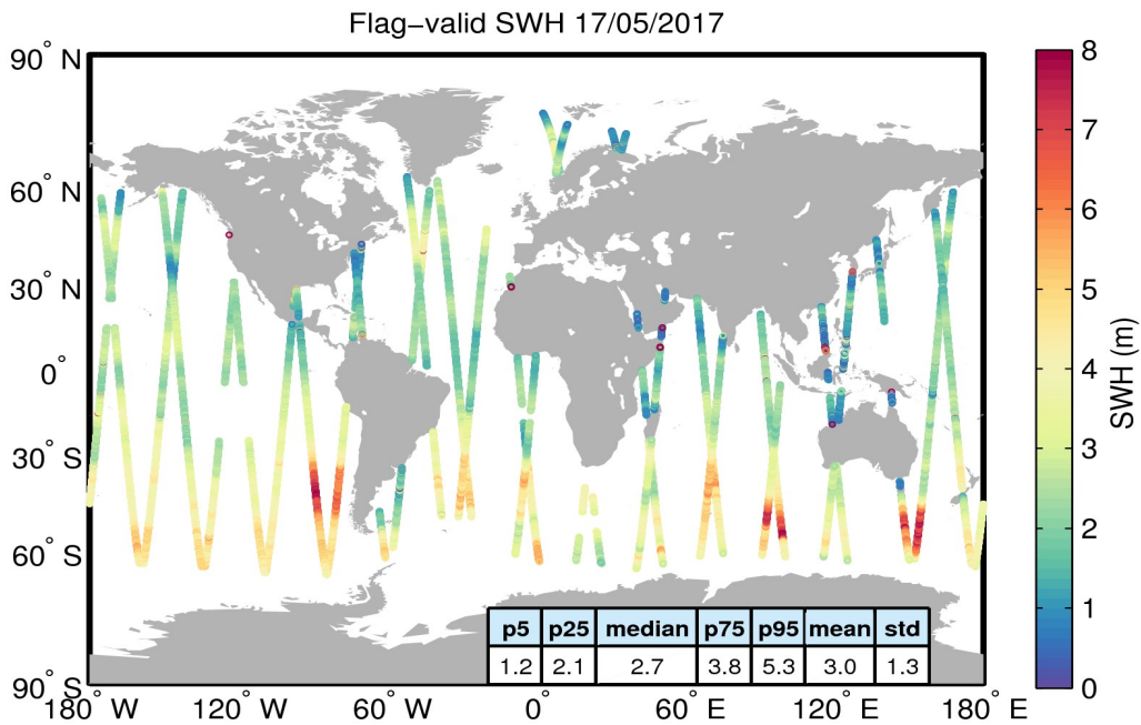
Figure 15. Geographical distribution of flag-valid SWH data over oceans and lakes for 17/05/2017. The statistical values shown in the table refer to the SWH in m and are calculated over all measurements shown in the figure.
