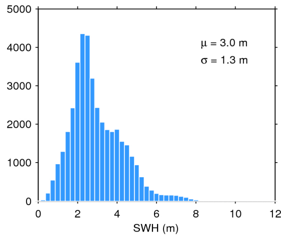
Figure 17. Histogram of flag-valid SWH over oceans and lakes for 17/05/2017. The mean ( \mu ) and standard deviation ( \sigma ) are also shown. Note that values larger than 12 m are excluded from the histogram for the sake of readability but not from the computation of \mu and \sigma .
