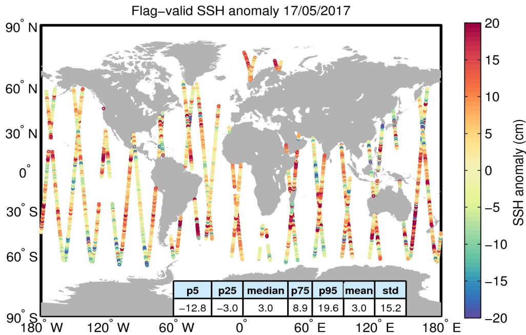
Figure 5. Geographical distribution of flag-valid 1-Hz SSH anomaly data over oceans and lakes for 17/05/2017. The statistical values shown in the table refer to the SSH anomaly in cm and are calculated over all measurements shown in the figure.
