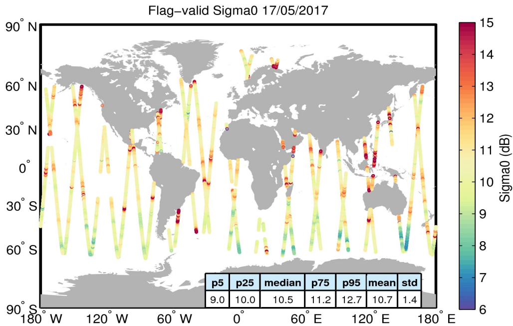
Figure 23. Geographical distribution of flag-valid sigma0 data over oceans and lakes for 17/05/2017. The statistical values shown in the table refer to the sigma0 in dB and are calculated over all measurements shown in the figure.
