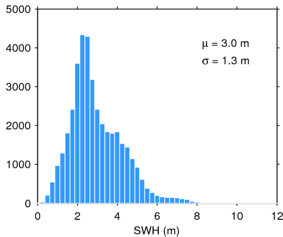
Figure 20. Histogram of science-valid SWH over oceans and lakes for 17/05/2017. The mean ( \mu ) and standard deviation ( \sigma ) are also shown. Note that values larger than 12 m are excluded from the histogram for the sake of readability but not from the computation of \mu and \sigma .
