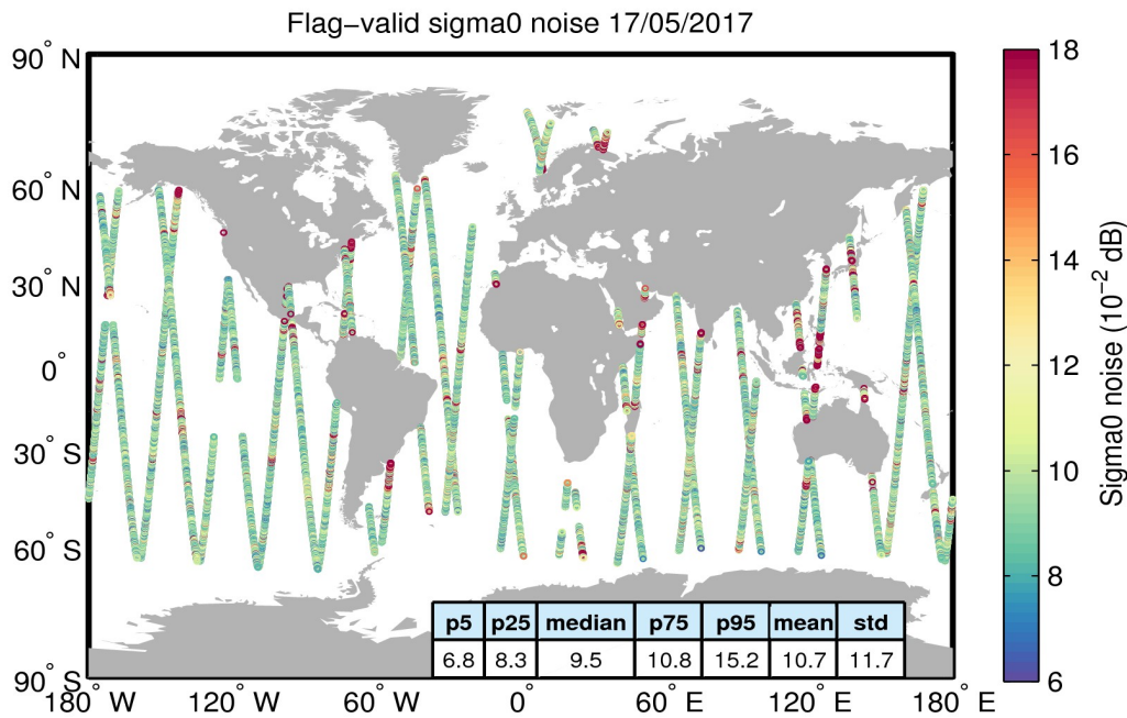
Figure 26. Geographical distribution of flag-valid 20-Hz sigma0 measurement noise over oceans and lakes for 17/05/2017. The statistical values shown in the table refer to the sigma0 noise and are calculated over all measurements shown in the figure.
