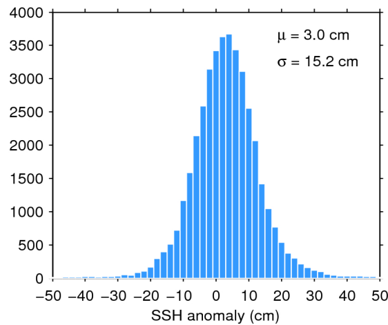
Figure 7. Histogram of flag-valid SSH anomaly over oceans and lakes for 17/05/2017. The mean ( \mu ) and standard deviation ( \sigma ) are also shown. Note that values outside [-50 50] cm are excluded from the histogram for the sake of readability but not from the computation of \mu and \sigma .
