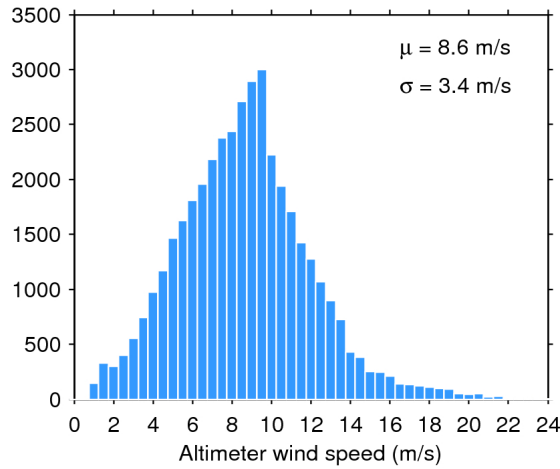
Figure 33. Histogram of flag-valid wind over oceans and lakes for 17/05/2017. The mean ( \mu ) and standard deviation ( \sigma ) are also shown. Note that values larger than 24 m/s are excluded from the histogram for the sake of readability but not from the computation of \mu and \sigma .
