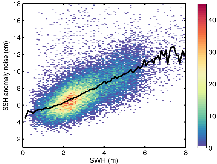
Figure 9. 2D histogram showing flag-valid SSH anomaly noise as a function of SWH for 16/05/2017. The black line denotes the median SSH anomaly noise as a function of SWH.
