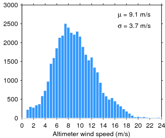
Figure 33. Histogram of flag-valid wind over oceans and lakes for 16/05/2017. The mean ( \mu ) and standard deviation ( \sigma ) are also shown. Note that values larger than 24 m/s are excluded from the histogram for the sake of readability but not from the computation of \mu and \sigma .
