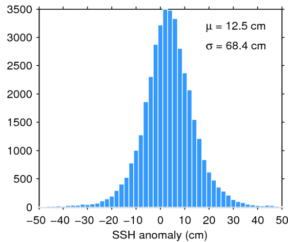
Figure 7. Histogram of flag-valid SSH anomaly over oceans and lakes for 16/05/2017. The mean ( \mu ) and standard deviation ( \sigma ) are also shown. Note that values outside [-50 50] cm are excluded from the histogram for the sake of readability but not from the computation of \mu and \sigma .
