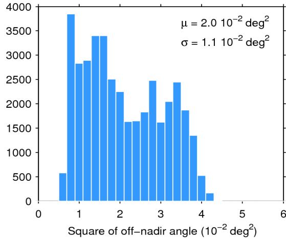
Figure 39. Histogram of flag-valid mispointing over oceans and lakes for 16/05/2017. The mean ( \mu ) and standard deviation ( \sigma ) are also shown. Note that values larger than 6 \cdot 10^{-2} \text{ deg}^2 are excluded from the histogram for the sake of readability but not from the computation of \mu and \sigma .
