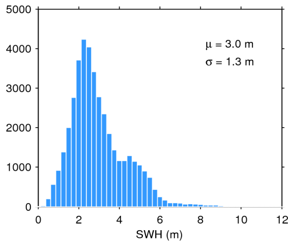
Figure 20. Histogram of science-valid SWH over oceans and lakes for 16/05/2017. The mean ( \mu ) and standard deviation ( \sigma ) are also shown. Note that values larger than 12 m are excluded from the histogram for the sake of readability but not from the computation of \mu and \sigma .
