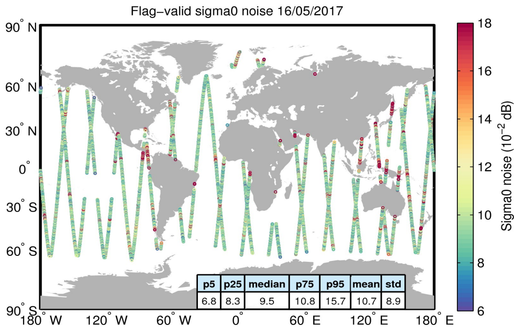
Figure 26. Geographical distribution of flag-valid 20-Hz sigma0 measurement noise over oceans and lakes for 16/05/2017. The statistical values shown in the table refer to the sigma0 noise and are calculated over all measurements shown in the figure.
