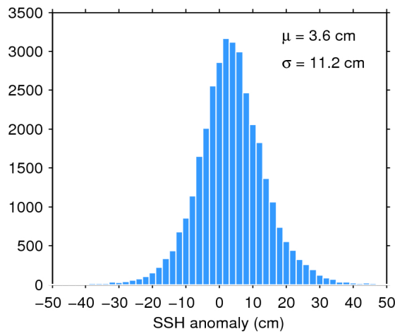
Figure 11. Histogram of science-valid SSH anomaly over oceans and lakes for 16/05/2017. The mean ( \mu ) and standard deviation ( \sigma ) are also shown. Note that values outside [-50 50] cm are excluded from the histogram for the sake of readability but not from the computation of \mu and \sigma .
