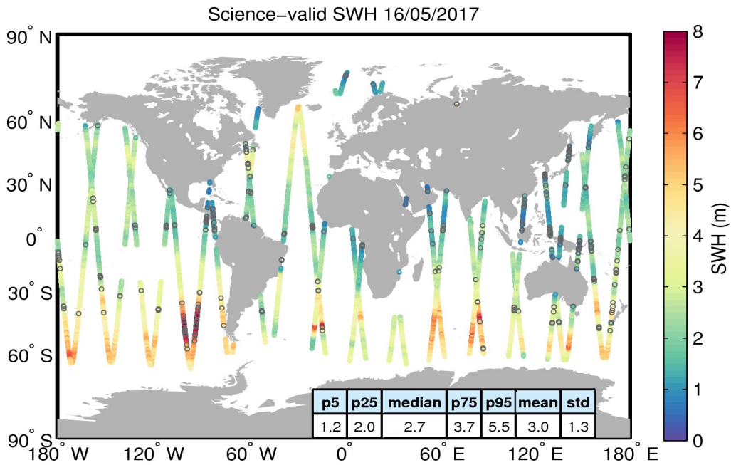
Figure 19. Geographical distribution of science-valid SWH data over oceans and lakes for 16/05/2017. The statistical values shown in the table refer to the SWH in m and are calculated over all measurements shown in the figure. Gray circles denote records that have been rejected based on the editing criteria described in Table 3.
