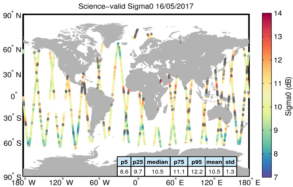
Figure 27. Geographical distribution of science-valid sigma0 data over oceans and lakes for 16/05/2017. The statistical values shown in the table refer to the sigma0 in dB and are calculated over all measurements shown in the figure. Gray circles denote records that have been rejected based on the editing criteria described in Table 4.
