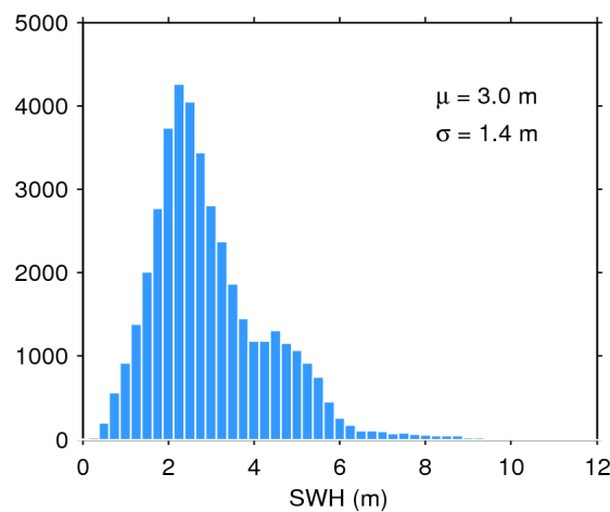
Figure 17. Histogram of flag-valid SWH over oceans and lakes for 16/05/2017. The mean ( \mu ) and standard deviation ( \sigma ) are also shown. Note that values larger than 12 m are excluded from the histogram for the sake of readability but not from the computation of \mu and \sigma .
