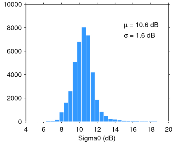
Figure 25. Histogram of flag-valid sigma0 over oceans and lakes for 16/05/2017. The mean ( \mu ) and standard deviation ( \sigma ) are also shown. Note that values outside [4 20] dB are excluded from the histogram for the sake of readability but not from the computation of \mu and \sigma .
