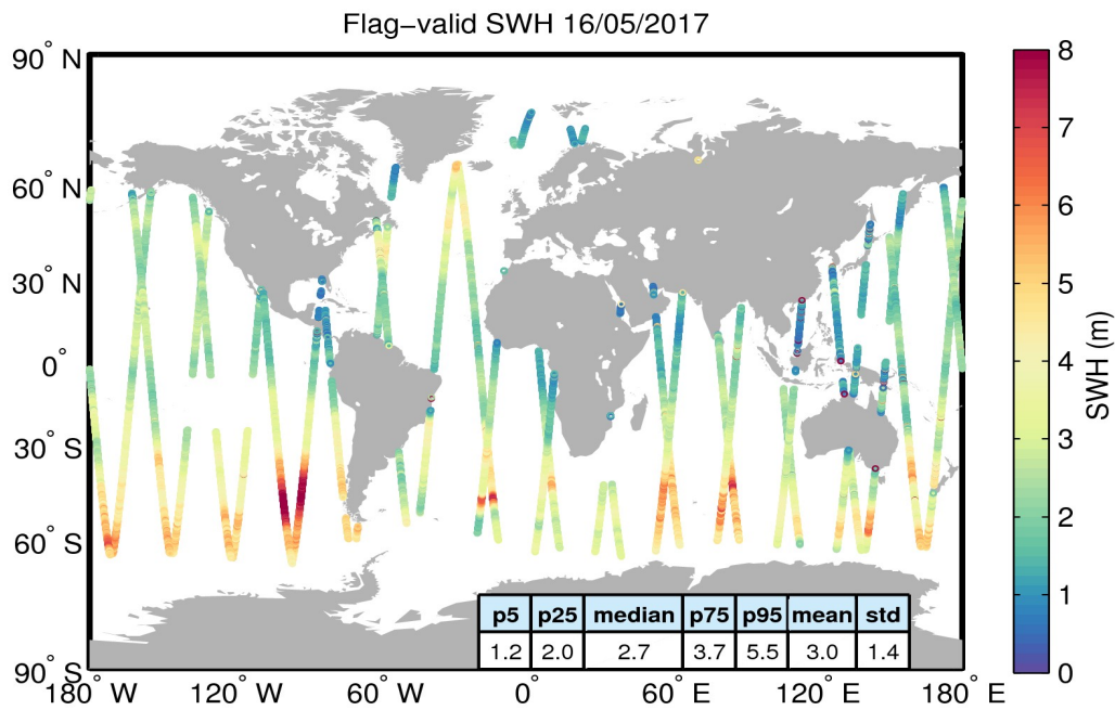
Figure 15. Geographical distribution of flag-valid SWH data over oceans and lakes for 16/05/2017. The statistical values shown in the table refer to the SWH in m and are calculated over all measurements shown in the figure.
