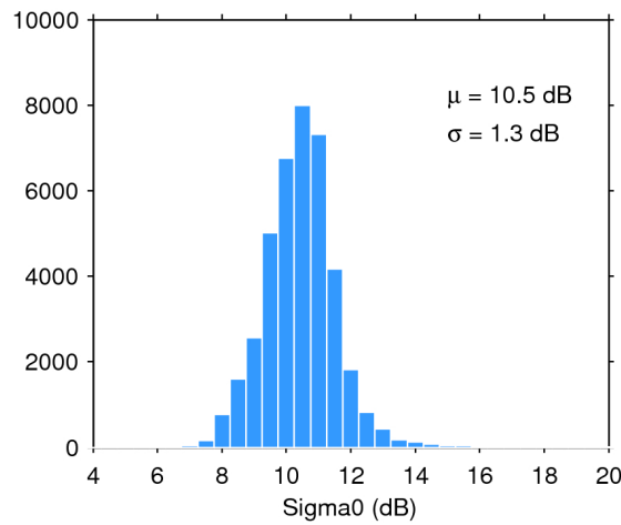
Figure 28. Histogram of science-valid sigma0 over oceans and lakes for 16/05/2017. The mean ( \mu ) and standard deviation ( \sigma ) are also shown. Note that values outside [4 20] dB are excluded from the histogram for the sake of readability but not from the computation of \mu and \sigma .
