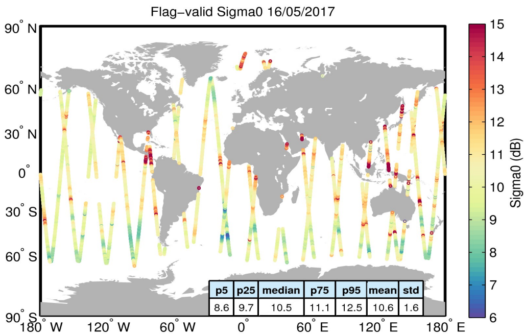
Figure 23. Geographical distribution of flag-valid sigma0 data over oceans and lakes for 16/05/2017. The statistical values shown in the table refer to the sigma0 in dB and are calculated over all measurements shown in the figure.
