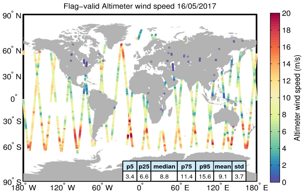
Figure 31. Geographical distribution of flag-valid wind data over oceans and lakes for 16/05/2017. The statistical values shown in the table refer to the wind in m/s and are calculated over all measurements shown in the figure.
