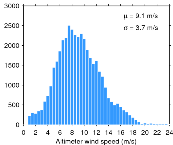
Figure 35. Histogram of science-valid wind over oceans and lakes for 16/05/2017. The mean ( \mu ) and standard deviation ( \sigma ) are also shown. Note that values larger than 24 m/s are excluded from the histogram for the sake of readability but not from the computation of \mu and \sigma .
