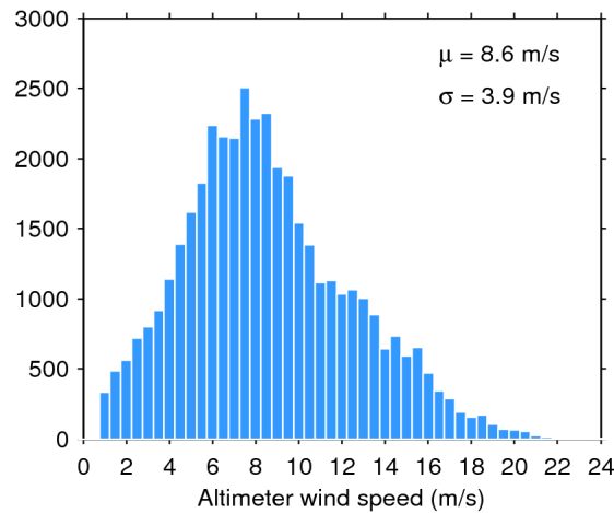
Figure 33. Histogram of flag-valid wind over oceans and lakes for 15/05/2017. The mean ( \mu ) and standard deviation ( \sigma ) are also shown. Note that values larger than 24 m/s are excluded from the histogram for the sake of readability but not from the computation of \mu and \sigma .
