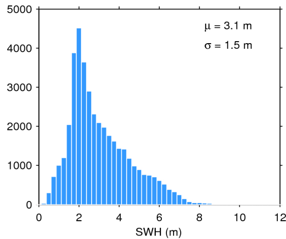
Figure 17. Histogram of flag-valid SWH over oceans and lakes for 15/05/2017. The mean ( \mu ) and standard deviation ( \sigma ) are also shown. Note that values larger than 12 m are excluded from the histogram for the sake of readability but not from the computation of \mu and \sigma .
