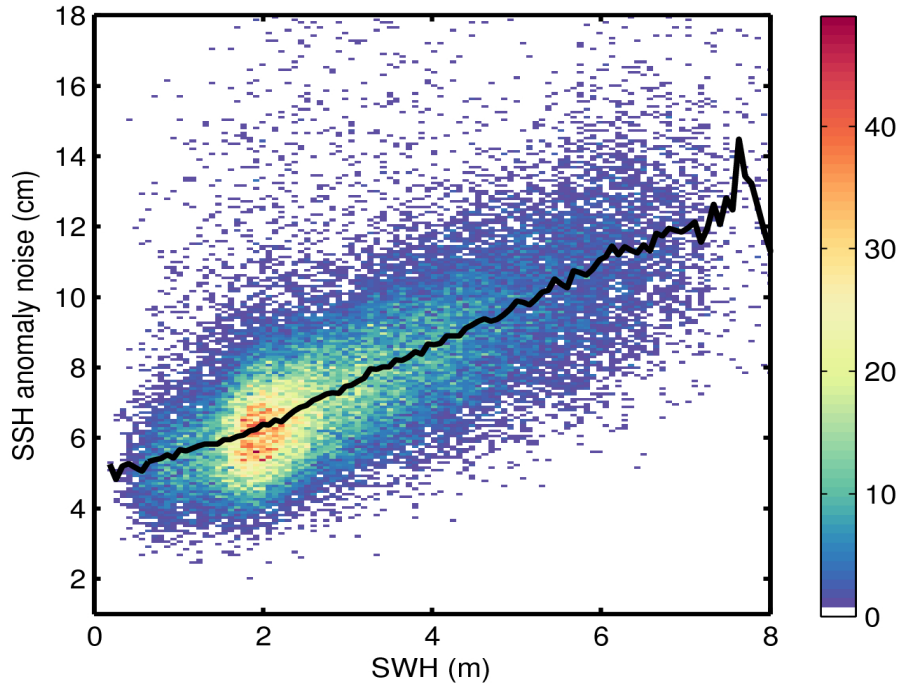
Figure 9. 2D histogram showing flag-valid SSH anomaly noise as a function of SWH for 15/05/2017. The black line denotes the median SSH anomaly noise as a function of SWH.
