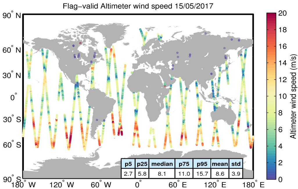
Figure 31. Geographical distribution of flag-valid wind data over oceans and lakes for 15/05/2017. The statistical values shown in the table refer to the wind in m/s and are calculated over all measurements shown in the figure.
