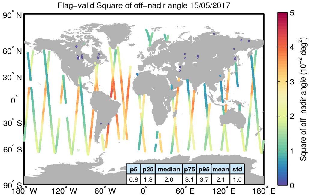
Figure 37. Geographical distribution of flag-valid mispointing data over oceans and lakes for 15/05/2017. The statistical values shown in the table refer to the mispointing in 10^{-2} deg 2 and are calculated over all measurements shown in the figure.
