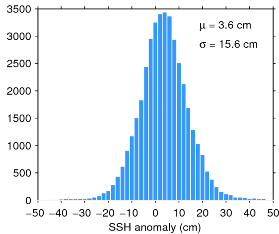
Figure 7. Histogram of flag-valid SSH anomaly over oceans and lakes for 15/05/2017. The mean ( \mu ) and standard deviation ( \sigma ) are also shown. Note that values outside [-50 50] cm are excluded from the histogram for the sake of readability but not from the computation of \mu and \sigma .
