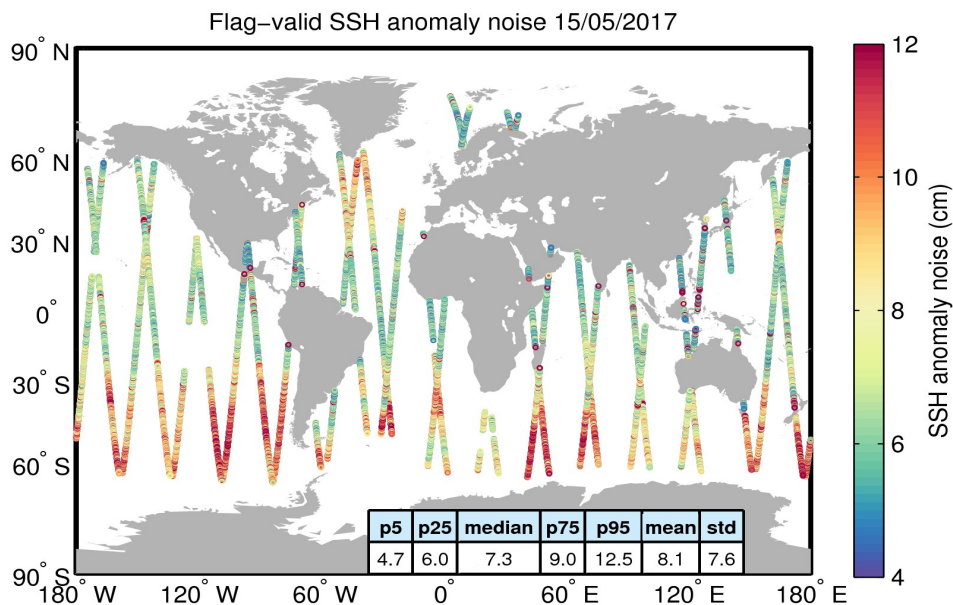
Figure 8. Geographical distribution of flag-valid 20-Hz SSH anomaly measurement noise over oceans and lakes for 15/05/2017. The statistical values shown in the table refer to the SSH anomaly noise and are calculated over all measurements shown in the figure.
