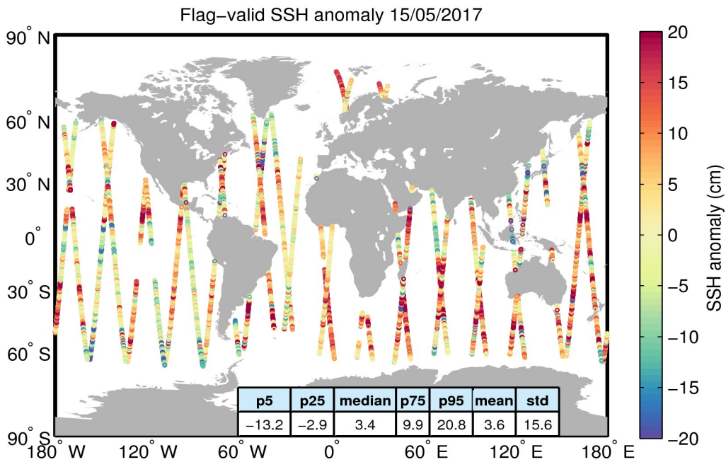
Figure 5. Geographical distribution of flag-valid 1-Hz SSH anomaly data over oceans and lakes for 15/05/2017. The statistical values shown in the table refer to the SSH anomaly in cm and are calculated over all measurements shown in the figure.
