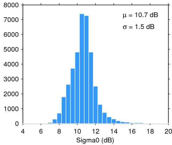
Figure 28. Histogram of science-valid sigma0 over oceans and lakes for 15/05/2017. The mean ( \mu ) and standard deviation ( \sigma ) are also shown. Note that values outside [4 20] dB are excluded from the histogram for the sake of readability but not from the computation of \mu and \sigma .
