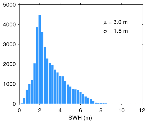
Figure 20. Histogram of science-valid SWH over oceans and lakes for 15/05/2017. The mean ( \mu ) and standard deviation ( \sigma ) are also shown. Note that values larger than 12 m are excluded from the histogram for the sake of readability but not from the computation of \mu and \sigma .
