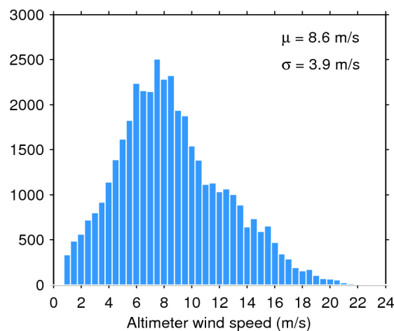
Figure 35. Histogram of science-valid wind over oceans and lakes for 15/05/2017. The mean ( \mu ) and standard deviation ( \sigma ) are also shown. Note that values larger than 24 m/s are excluded from the histogram for the sake of readability but not from the computation of \mu and \sigma .
