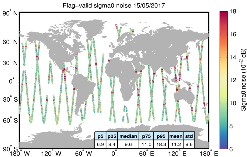
Figure 26. Geographical distribution of flag-valid 20-Hz sigma0 measurement noise over oceans and lakes for 15/05/2017. The statistical values shown in the table refer to the sigma0 noise and are calculated over all measurements shown in the figure.
