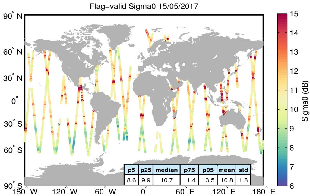
Figure 23. Geographical distribution of flag-valid sigma0 data over oceans and lakes for 15/05/2017. The statistical values shown in the table refer to the sigma0 in dB and are calculated over all measurements shown in the figure.
