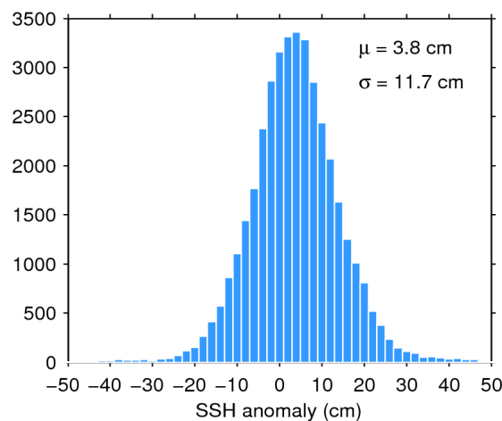
Figure 11. Histogram of science-valid SSH anomaly over oceans and lakes for 15/05/2017. The mean ( \mu ) and standard deviation ( \sigma ) are also shown. Note that values outside [-50 50] cm are excluded from the histogram for the sake of readability but not from the computation of \mu and \sigma .
