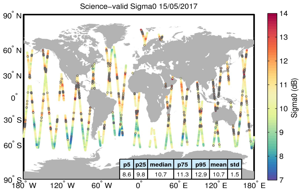
Figure 27. Geographical distribution of science-valid sigma0 data over oceans and lakes for 15/05/2017. The statistical values shown in the table refer to the sigma0 in dB and are calculated over all measurements shown in the figure. Gray circles denote records that have been rejected based on the editing criteria described in Table 4.
