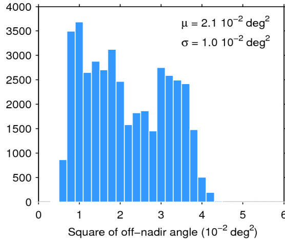
Figure 39. Histogram of flag-valid mispointing over oceans and lakes for 15/05/2017. The mean ( \mu ) and standard deviation ( \sigma ) are also shown. Note that values larger than 6 \cdot 10^{-2} \text{ deg}^2 are excluded from the histogram for the sake of readability but not from the computation of \mu and \sigma .
