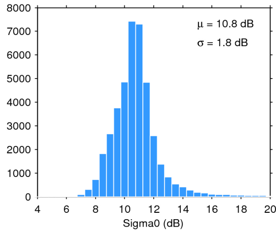
Figure 25. Histogram of flag-valid sigma0 over oceans and lakes for 15/05/2017. The mean ( \mu ) and standard deviation ( \sigma ) are also shown. Note that values outside [4 20] dB are excluded from the histogram for the sake of readability but not from the computation of \mu and \sigma .
