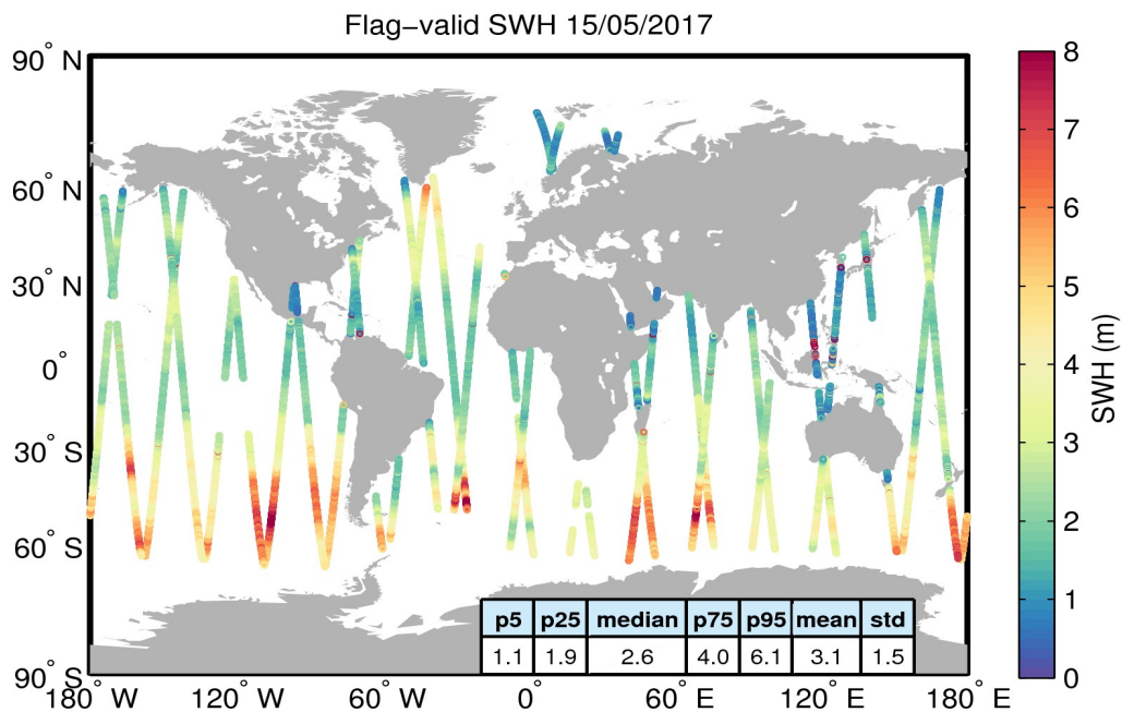
Figure 15. Geographical distribution of flag-valid SWH data over oceans and lakes for 15/05/2017. The statistical values shown in the table refer to the SWH in m and are calculated over all measurements shown in the figure.
