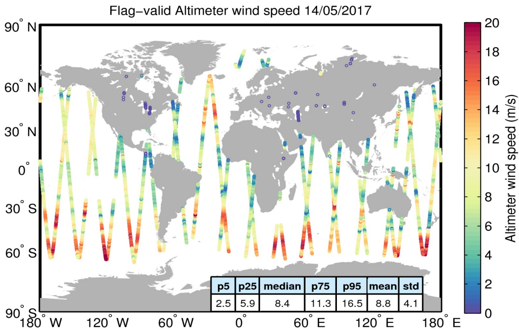
Figure 31. Geographical distribution of flag-valid wind data over oceans and lakes for 14/05/2017. The statistical values shown in the table refer to the wind in m/s and are calculated over all measurements shown in the figure.
