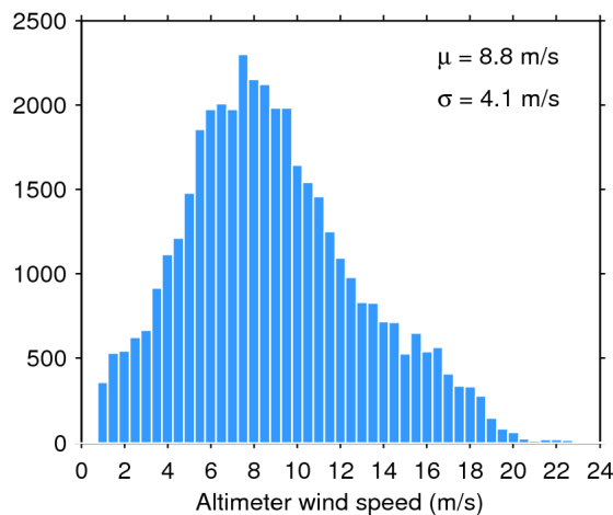
Figure 35. Histogram of science-valid wind over oceans and lakes for 14/05/2017. The mean ( \mu ) and standard deviation ( \sigma ) are also shown. Note that values larger than 24 m/s are excluded from the histogram for the sake of readability but not from the computation of \mu and \sigma .
