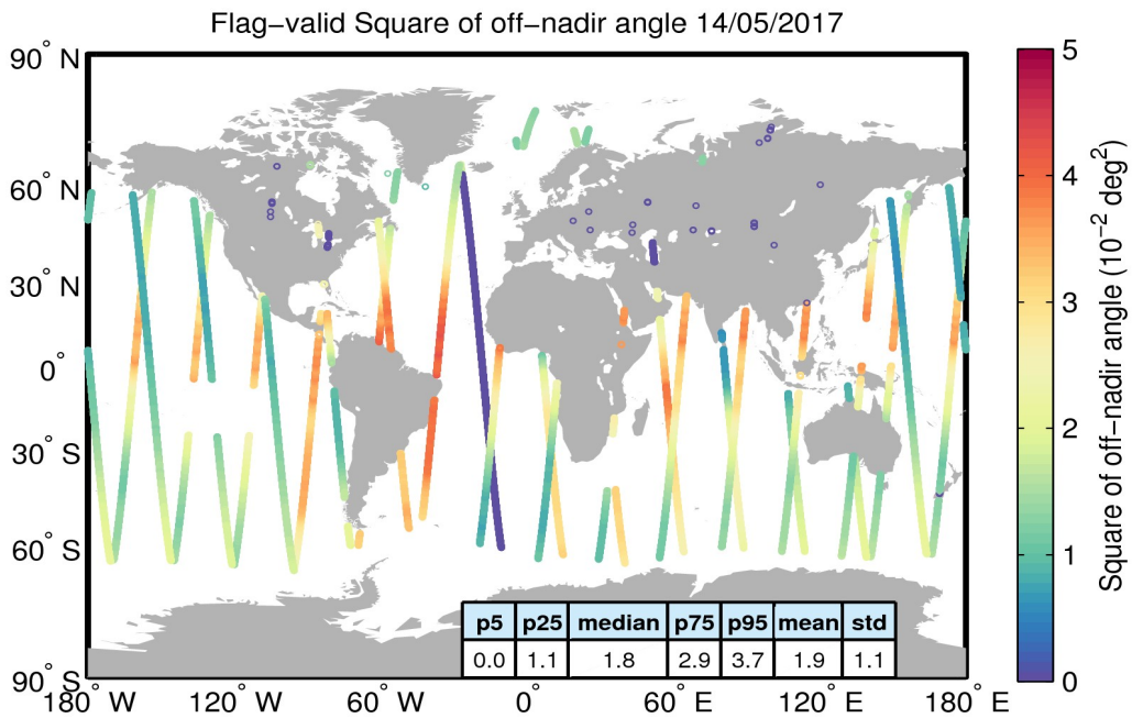
Figure 37. Geographical distribution of flag-valid mispointing data over oceans and lakes for 14/05/2017. The statistical values shown in the table refer to the mispointing in 10^{-2} deg 2 and are calculated over all measurements shown in the figure.
