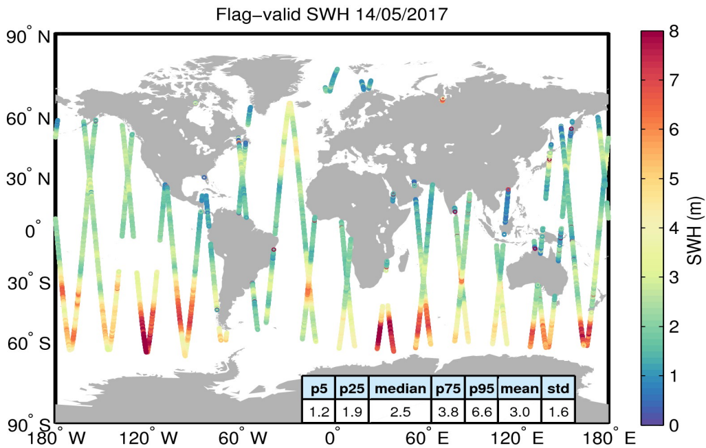
Figure 15. Geographical distribution of flag-valid SWH data over oceans and lakes for 14/05/2017. The statistical values shown in the table refer to the SWH in m and are calculated over all measurements shown in the figure.
