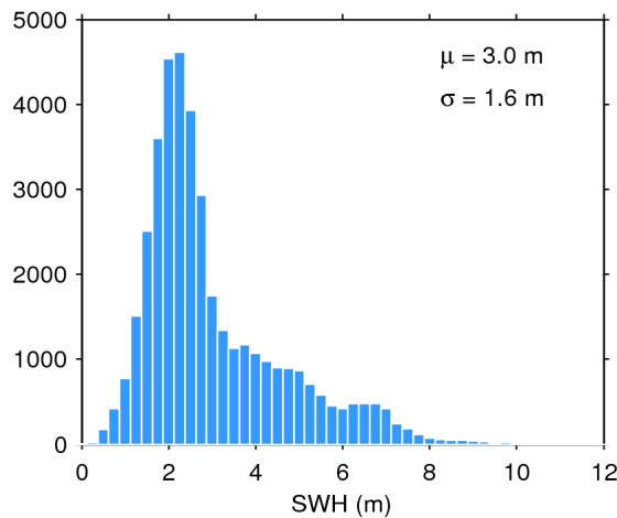
Figure 20. Histogram of science-valid SWH over oceans and lakes for 14/05/2017. The mean ( \mu ) and standard deviation ( \sigma ) are also shown. Note that values larger than 12 m are excluded from the histogram for the sake of readability but not from the computation of \mu and \sigma .
