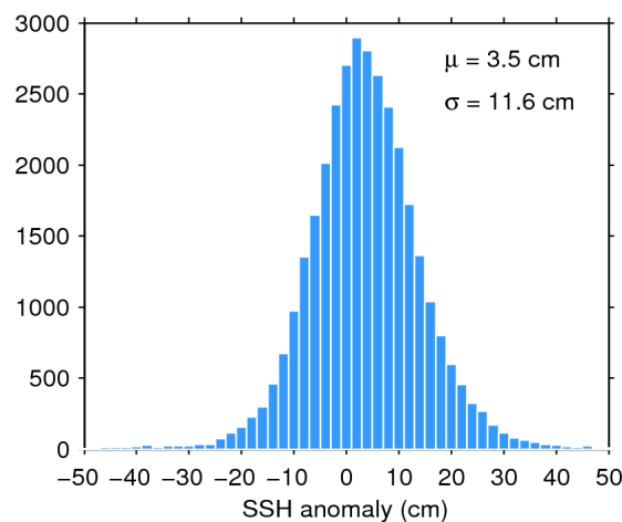
Figure 11. Histogram of science-valid SSH anomaly over oceans and lakes for 14/05/2017. The mean ( \mu ) and standard deviation ( \sigma ) are also shown. Note that values outside [-50 50] cm are excluded from the histogram for the sake of readability but not from the computation of \mu and \sigma .
