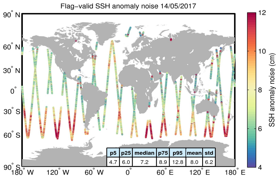
Figure 8. Geographical distribution of flag-valid 20-Hz SSH anomaly measurement noise over oceans and lakes for 14/05/2017. The statistical values shown in the table refer to the SSH anomaly noise and are calculated over all measurements shown in the figure.
