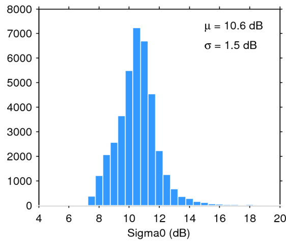
Figure 28. Histogram of science-valid sigma0 over oceans and lakes for 14/05/2017. The mean ( \mu ) and standard deviation ( \sigma ) are also shown. Note that values outside [4 20] dB are excluded from the histogram for the sake of readability but not from the computation of \mu and \sigma .
