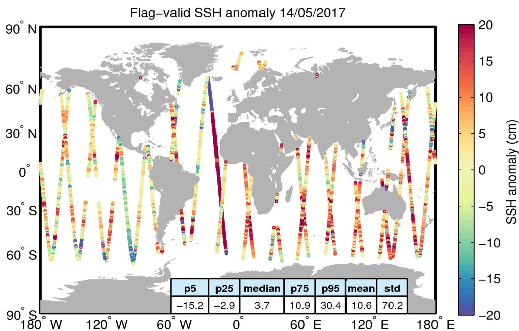
Figure 5. Geographical distribution of flag-valid 1-Hz SSH anomaly data over oceans and lakes for 14/05/2017. The statistical values shown in the table refer to the SSH anomaly in cm and are calculated over all measurements shown in the figure.
