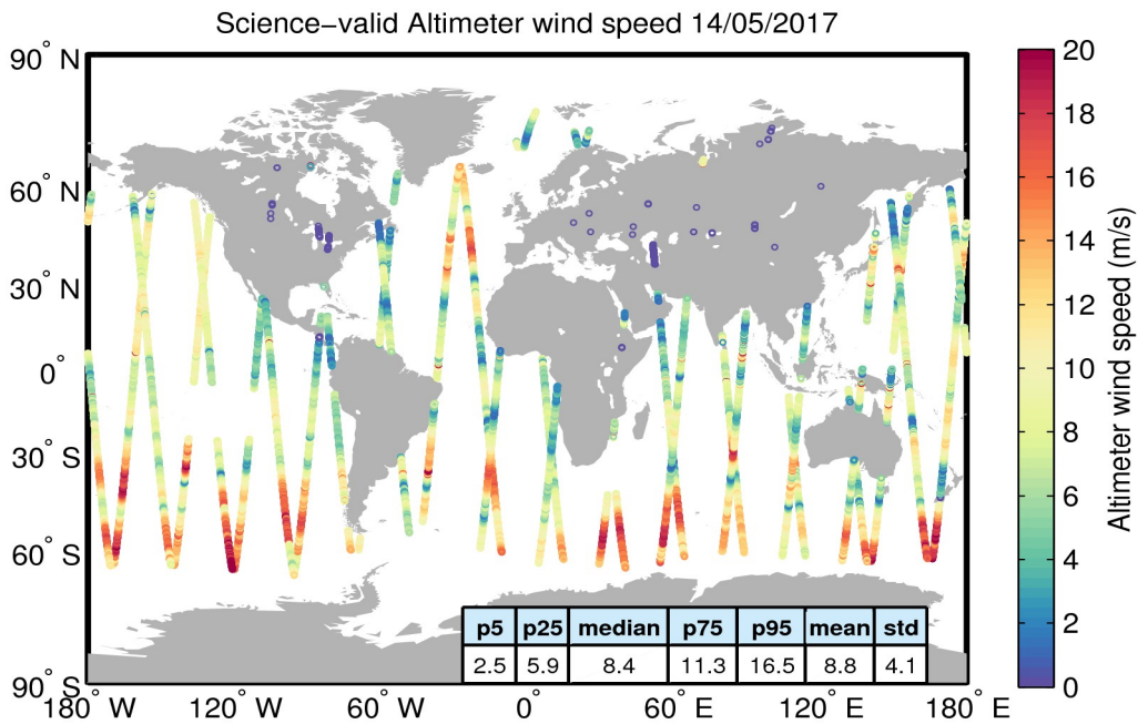
Figure 34. Geographical distribution of science-valid wind data over oceans and lakes for 14/05/2017. The statistical values shown in the table refer to the wind in m/s and are calculated over all measurements shown in the figure. Gray circles denote records that have been rejected based on the editing criteria described in Table 5.
