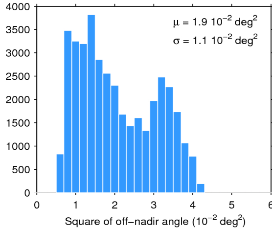
Figure 39. Histogram of flag-valid mispointing over oceans and lakes for 14/05/2017. The mean ( \mu ) and standard deviation ( \sigma ) are also shown. Note that values larger than 6 \cdot 10^{-2} \text{ deg}^2 are excluded from the histogram for the sake of readability but not from the computation of \mu and \sigma .
