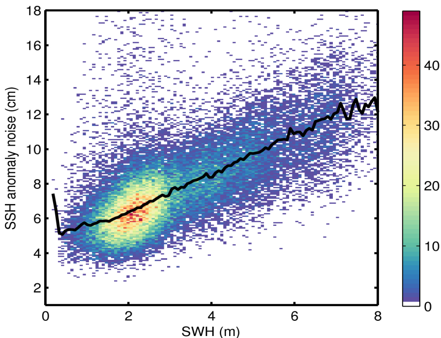
Figure 9. 2D histogram showing flag-valid SSH anomaly noise as a function of SWH for 14/05/2017. The black line denotes the median SSH anomaly noise as a function of SWH.
