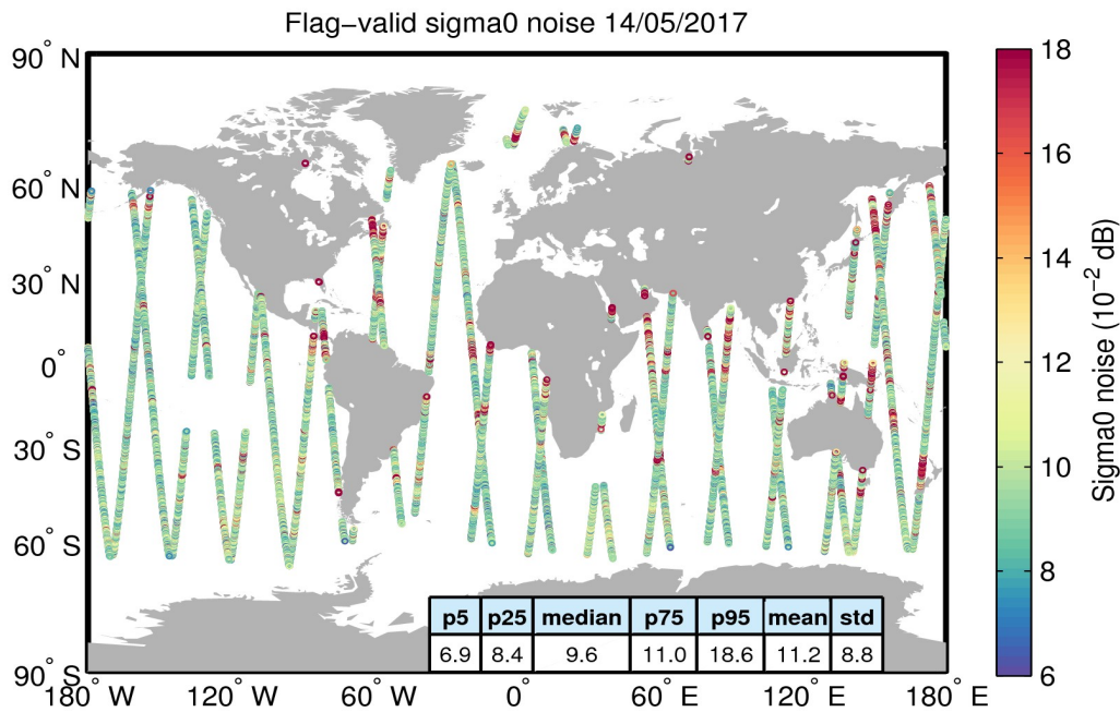
Figure 26. Geographical distribution of flag-valid 20-Hz sigma0 measurement noise over oceans and lakes for 14/05/2017. The statistical values shown in the table refer to the sigma0 noise and are calculated over all measurements shown in the figure.
