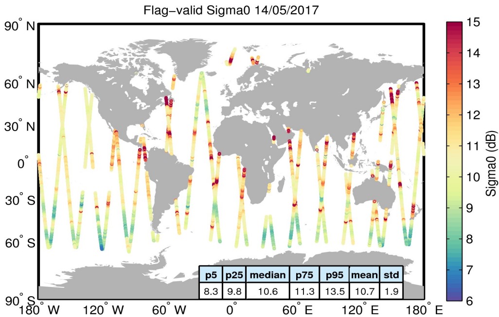
Figure 23. Geographical distribution of flag-valid sigma0 data over oceans and lakes for 14/05/2017. The statistical values shown in the table refer to the sigma0 in dB and are calculated over all measurements shown in the figure.
