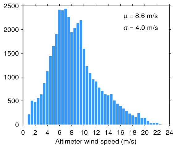
Figure 35. Histogram of science-valid wind over oceans and lakes for 13/05/2017. The mean ( \mu ) and standard deviation ( \sigma ) are also shown. Note that values larger than 24 m/s are excluded from the histogram for the sake of readability but not from the computation of \mu and \sigma .
