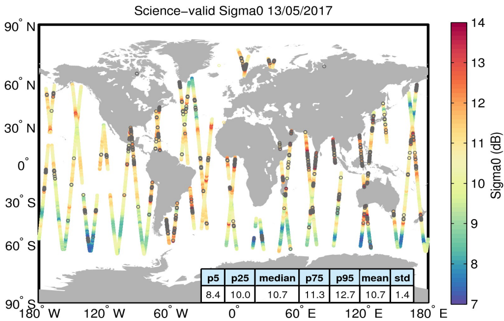
Figure 27. Geographical distribution of science-valid sigma0 data over oceans and lakes for 13/05/2017. The statistical values shown in the table refer to the sigma0 in dB and are calculated over all measurements shown in the figure. Gray circles denote records that have been rejected based on the editing criteria described in Table 4.
