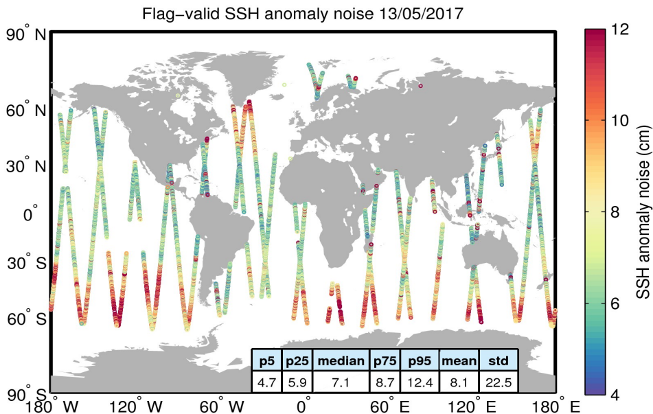
Figure 8. Geographical distribution of flag-valid 20-Hz SSH anomaly measurement noise over oceans and lakes for 13/05/2017. The statistical values shown in the table refer to the SSH anomaly noise and are calculated over all measurements shown in the figure.
