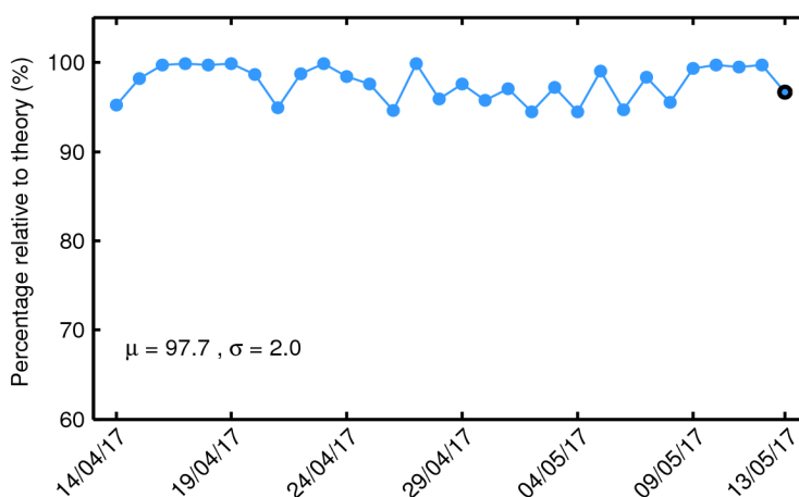
Figure 38. Percentage of flag-valid 1-Hz mispointing records over ocean and lakes relative to theory for each day in last 30-day window. The mean ( \mu ) and standard deviation ( \sigma ) are also shown.
