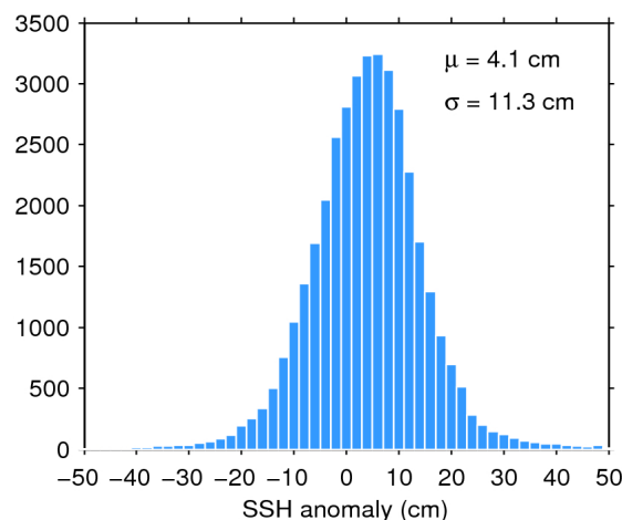
Figure 11. Histogram of science-valid SSH anomaly over oceans and lakes for 13/05/2017. The mean ( \mu ) and standard deviation ( \sigma ) are also shown. Note that values outside [-50 50] cm are excluded from the histogram for the sake of readability but not from the computation of \mu and \sigma .
