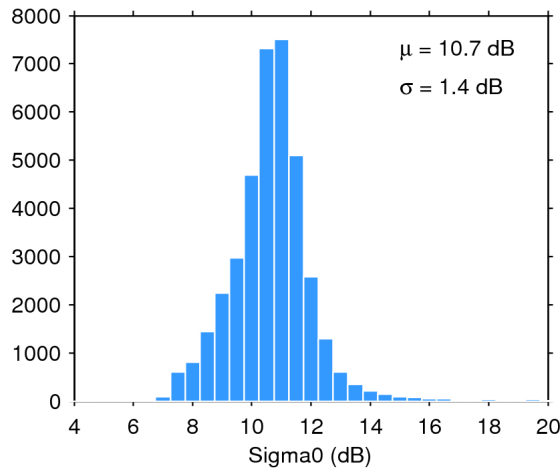
Figure 28. Histogram of science-valid sigma0 over oceans and lakes for 13/05/2017. The mean ( \mu ) and standard deviation ( \sigma ) are also shown. Note that values outside [4 20] dB are excluded from the histogram for the sake of readability but not from the computation of \mu and \sigma .
