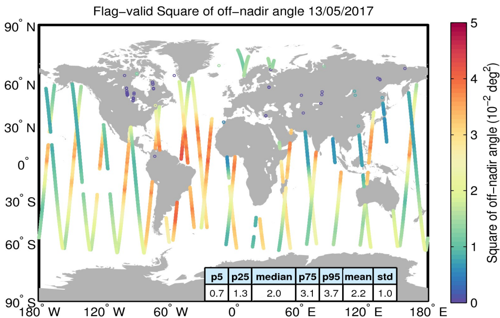
Figure 37. Geographical distribution of flag-valid mispointing data over oceans and lakes for 13/05/2017. The statistical values shown in the table refer to the mispointing in 10^{-2} deg 2 and are calculated over all measurements shown in the figure.
