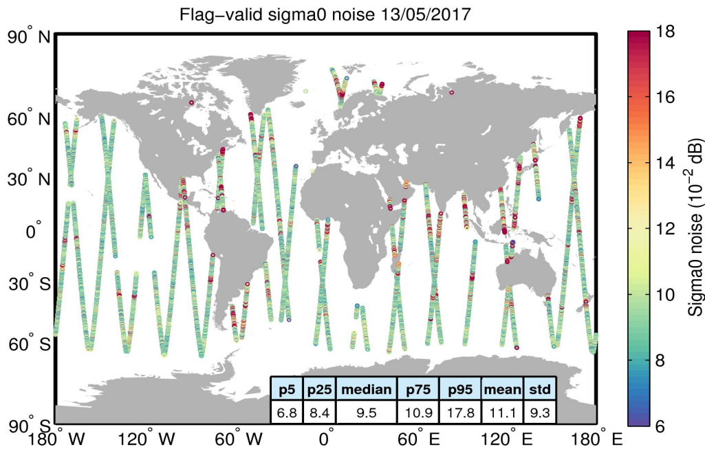
Figure 26. Geographical distribution of flag-valid 20-Hz sigma0 measurement noise over oceans and lakes for 13/05/2017. The statistical values shown in the table refer to the sigma0 noise and are calculated over all measurements shown in the figure.
