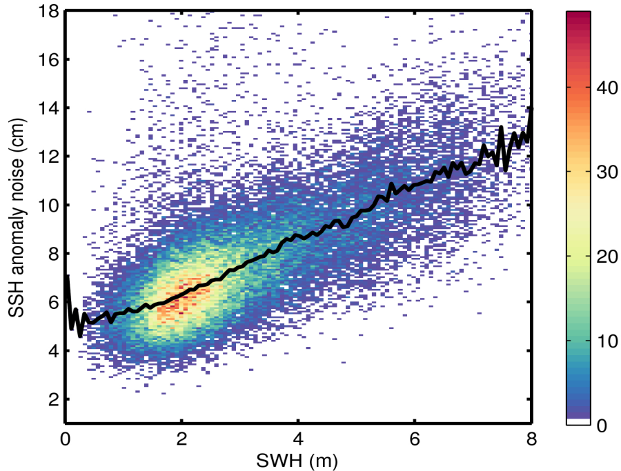
Figure 9. 2D histogram showing flag-valid SSH anomaly noise as a function of SWH for 13/05/2017. The black line denotes the median SSH anomaly noise as a function of SWH.
