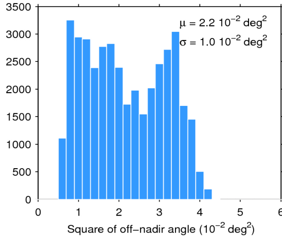
Figure 39. Histogram of flag-valid mispointing over oceans and lakes for 13/05/2017. The mean ( \mu ) and standard deviation ( \sigma ) are also shown. Note that values larger than 6 \cdot 10^{-2} \text{ deg}^2 are excluded from the histogram for the sake of readability but not from the computation of \mu and \sigma .
