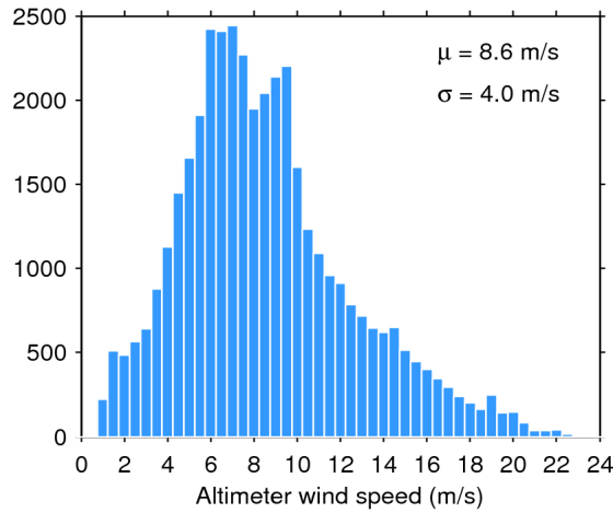
Figure 33. Histogram of flag-valid wind over oceans and lakes for 13/05/2017. The mean ( \mu ) and standard deviation ( \sigma ) are also shown. Note that values larger than 24 m/s are excluded from the histogram for the sake of readability but not from the computation of \mu and \sigma .
