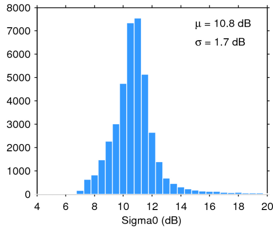
Figure 25. Histogram of flag-valid sigma0 over oceans and lakes for 13/05/2017. The mean ( \mu ) and standard deviation ( \sigma ) are also shown. Note that values outside [4 20] dB are excluded from the histogram for the sake of readability but not from the computation of \mu and \sigma .
