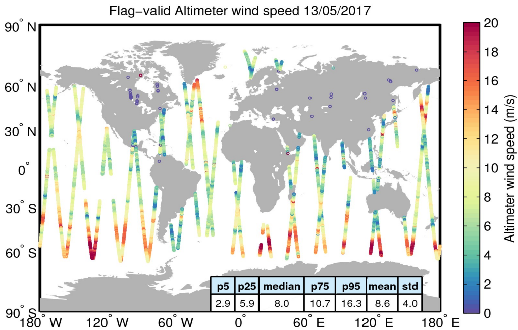
Figure 31. Geographical distribution of flag-valid wind data over oceans and lakes for 13/05/2017. The statistical values shown in the table refer to the wind in m/s and are calculated over all measurements shown in the figure.
