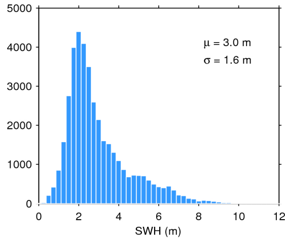
Figure 17. Histogram of flag-valid SWH over oceans and lakes for 13/05/2017. The mean ( \mu ) and standard deviation ( \sigma ) are also shown. Note that values larger than 12 m are excluded from the histogram for the sake of readability but not from the computation of \mu and \sigma .
