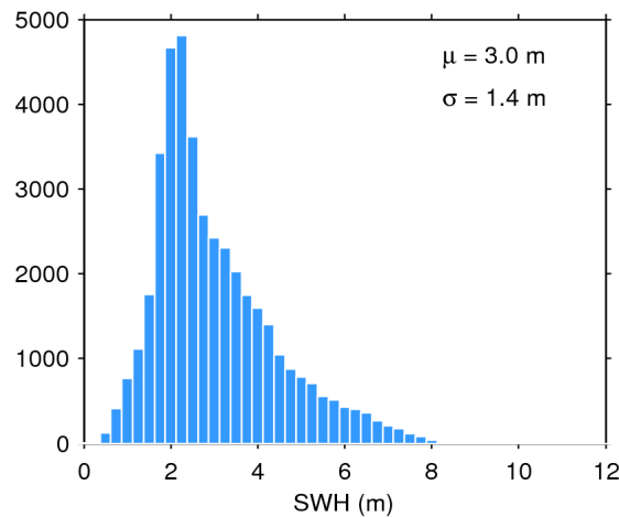
Figure 17. Histogram of flag-valid SWH over oceans and lakes for 12/05/2017. The mean ( \mu ) and standard deviation ( \sigma ) are also shown. Note that values larger than 12 m are excluded from the histogram for the sake of readability but not from the computation of \mu and \sigma .
