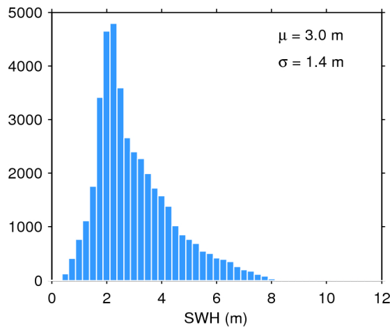
Figure 20. Histogram of science-valid SWH over oceans and lakes for 12/05/2017. The mean ( \mu ) and standard deviation ( \sigma ) are also shown. Note that values larger than 12 m are excluded from the histogram for the sake of readability but not from the computation of \mu and \sigma .
