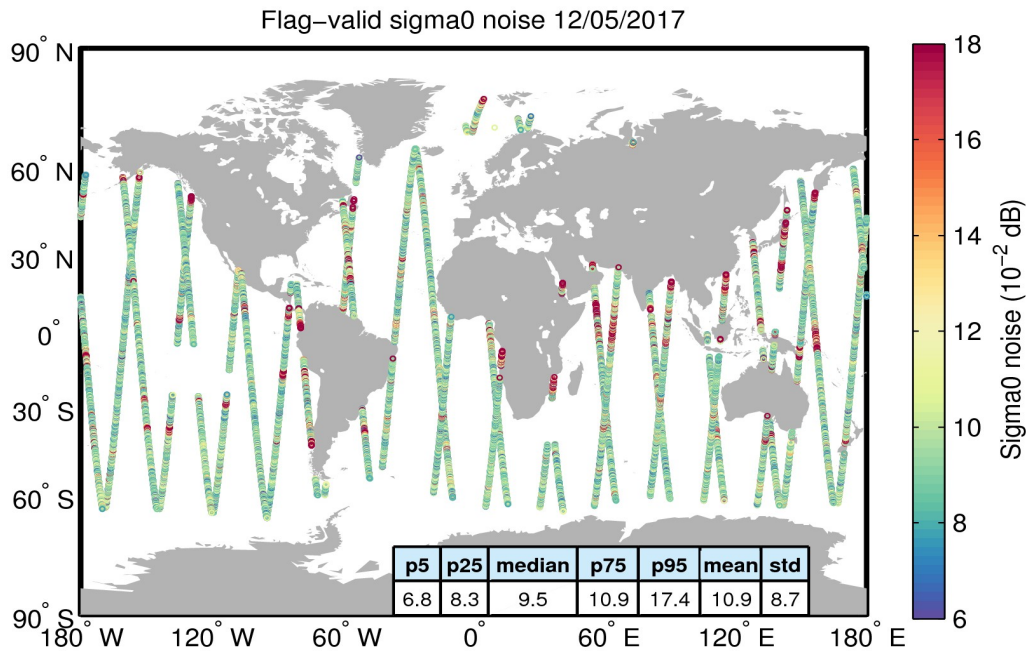
Figure 26. Geographical distribution of flag-valid 20-Hz sigma0 measurement noise over oceans and lakes for 12/05/2017. The statistical values shown in the table refer to the sigma0 noise and are calculated over all measurements shown in the figure.
