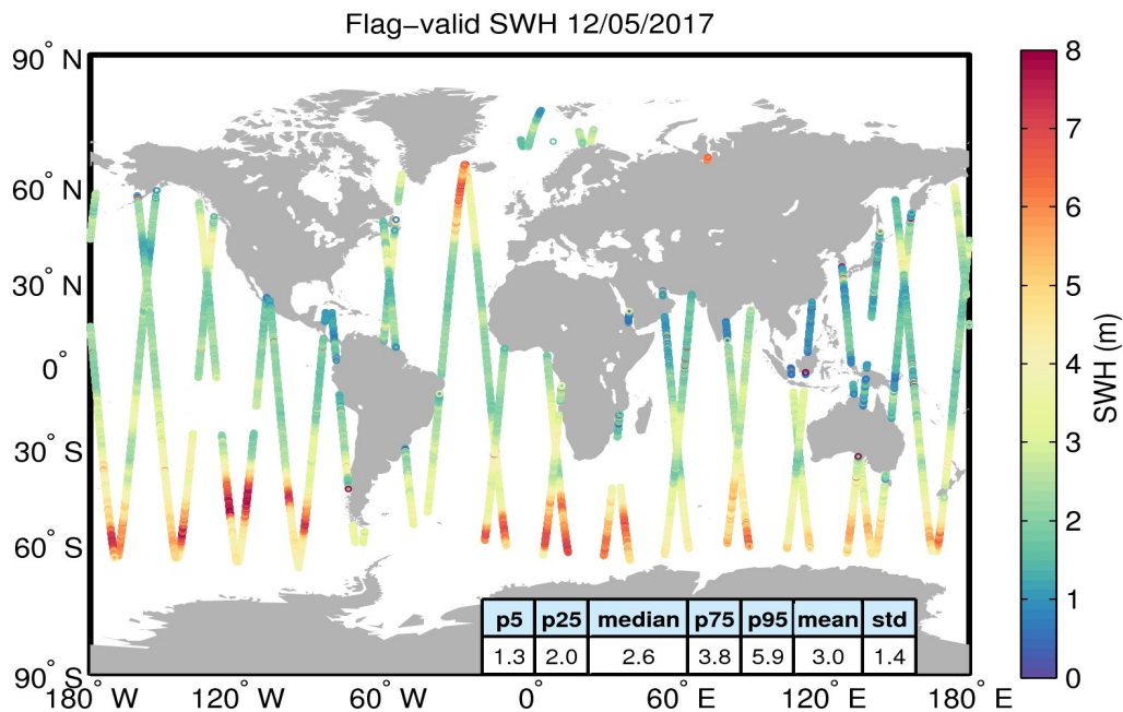
Figure 15. Geographical distribution of flag-valid SWH data over oceans and lakes for 12/05/2017. The statistical values shown in the table refer to the SWH in m and are calculated over all measurements shown in the figure.
