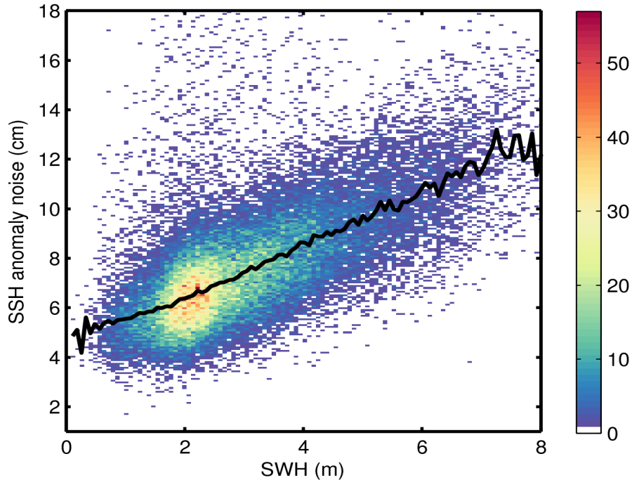
Figure 9. 2D histogram showing flag-valid SSH anomaly noise as a function of SWH for 12/05/2017. The black line denotes the median SSH anomaly noise as a function of SWH.
