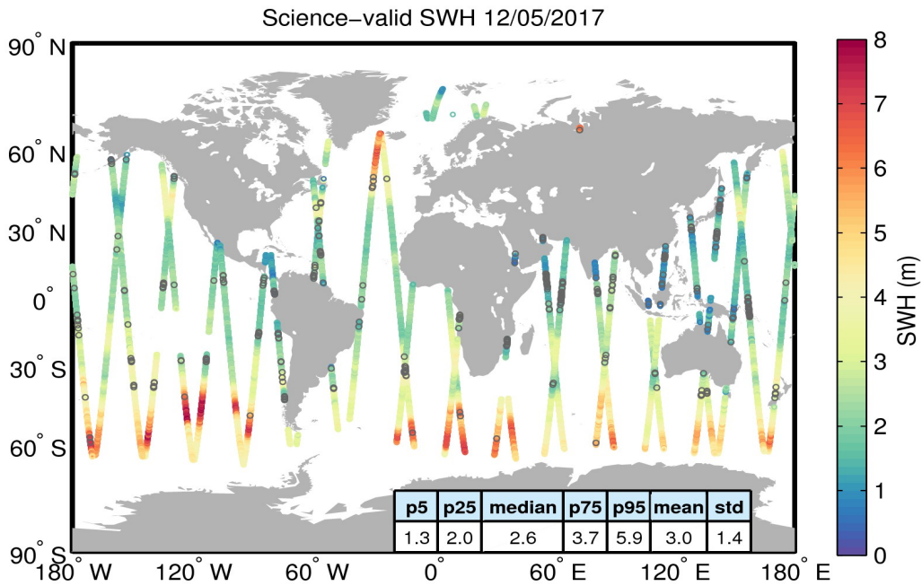
Figure 19. Geographical distribution of science-valid SWH data over oceans and lakes for 12/05/2017. The statistical values shown in the table refer to the SWH in m and are calculated over all measurements shown in the figure. Gray circles denote records that have been rejected based on the editing criteria described in Table 3.
