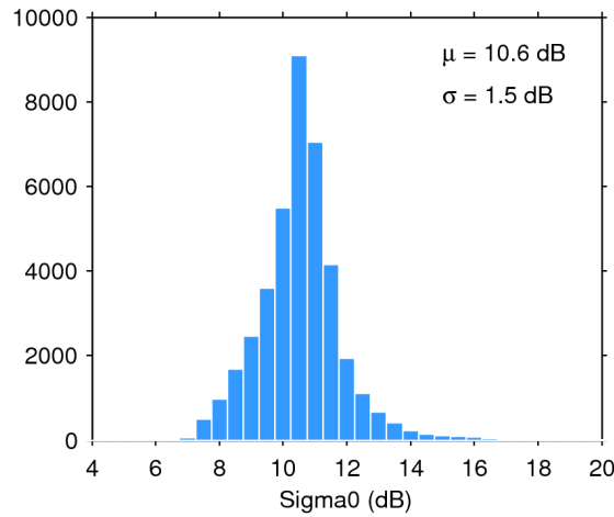
Figure 28. Histogram of science-valid sigma0 over oceans and lakes for 12/05/2017. The mean ( \mu ) and standard deviation ( \sigma ) are also shown. Note that values outside [4 20] dB are excluded from the histogram for the sake of readability but not from the computation of \mu and \sigma .
