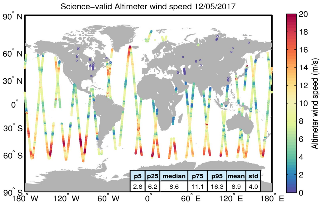
Figure 34. Geographical distribution of science-valid wind data over oceans and lakes for 12/05/2017. The statistical values shown in the table refer to the wind in m/s and are calculated over all measurements shown in the figure. Gray circles denote records that have been rejected based on the editing criteria described in Table 5.
