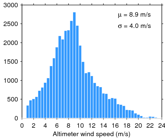
Figure 33. Histogram of flag-valid wind over oceans and lakes for 12/05/2017. The mean ( \mu ) and standard deviation ( \sigma ) are also shown. Note that values larger than 24 m/s are excluded from the histogram for the sake of readability but not from the computation of \mu and \sigma .
