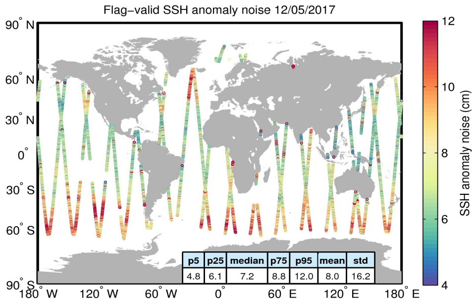
Figure 8. Geographical distribution of flag-valid 20-Hz SSH anomaly measurement noise over oceans and lakes for 12/05/2017. The statistical values shown in the table refer to the SSH anomaly noise and are calculated over all measurements shown in the figure.
