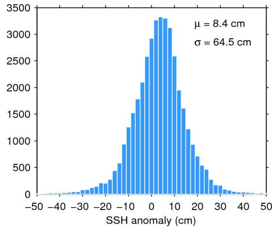
Figure 7. Histogram of flag-valid SSH anomaly over oceans and lakes for 12/05/2017. The mean ( \mu ) and standard deviation ( \sigma ) are also shown. Note that values outside [-50\ 50] cm are excluded from the histogram for the sake of readability but not from the computation of \mu and \sigma .
