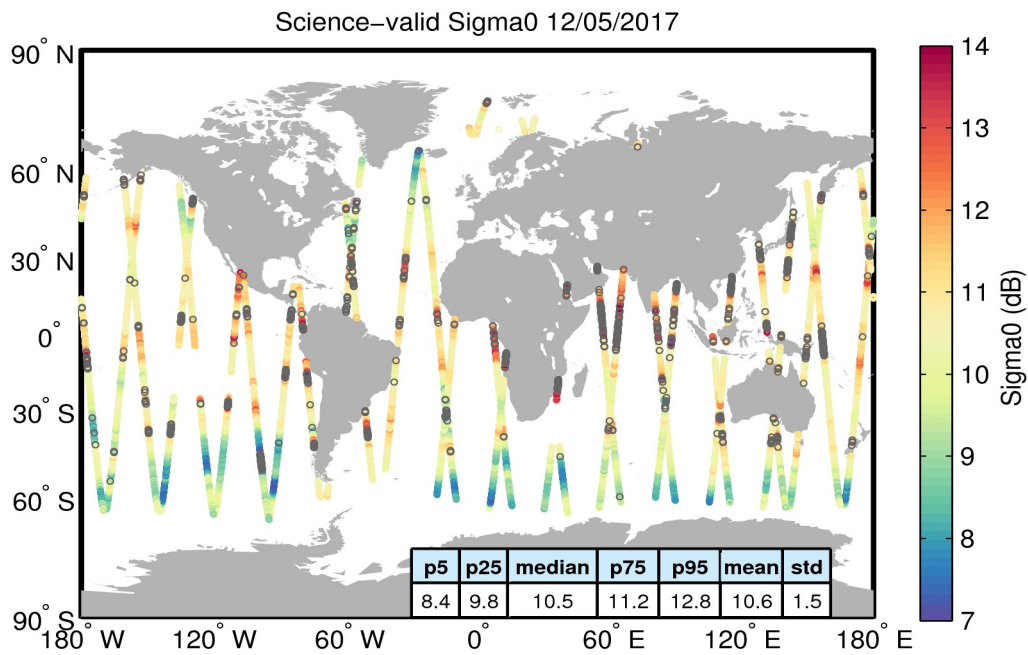
Figure 27. Geographical distribution of science-valid sigma0 data over oceans and lakes for 12/05/2017. The statistical values shown in the table refer to the sigma0 in dB and are calculated over all measurements shown in the figure. Gray circles denote records that have been rejected based on the editing criteria described in Table 4.
