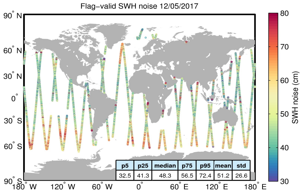
Figure 18. Geographical distribution of flag-valid 20-Hz SWH measurement noise over oceans and lakes for 12/05/2017. The statistical values shown in the table refer to the SWH noise and are calculated over all measurements shown in the figure.
