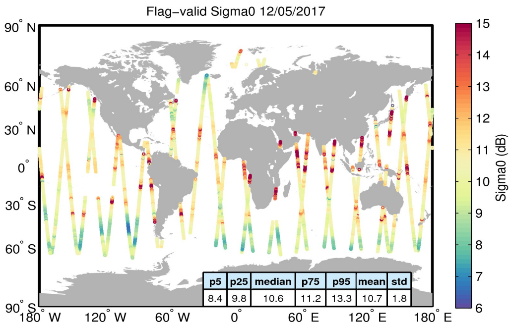
Figure 23. Geographical distribution of flag-valid sigma0 data over oceans and lakes for 12/05/2017. The statistical values shown in the table refer to the sigma0 in dB and are calculated over all measurements shown in the figure.
