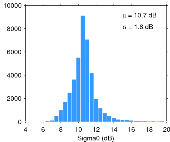
Figure 25. Histogram of flag-valid sigma0 over oceans and lakes for 12/05/2017. The mean ( \mu ) and standard deviation ( \sigma ) are also shown. Note that values outside [4 20] dB are excluded from the histogram for the sake of readability but not from the computation of \mu and \sigma .
