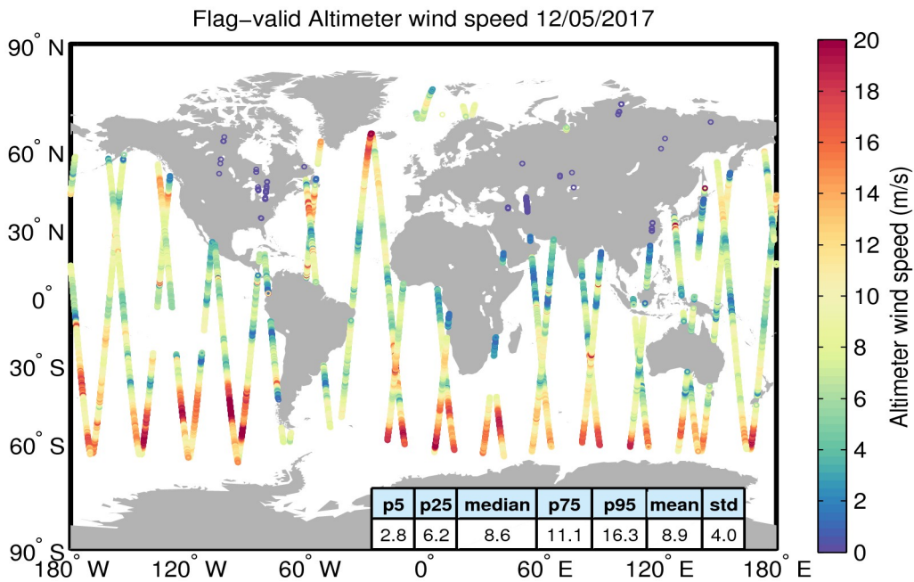
Figure 31. Geographical distribution of flag-valid wind data over oceans and lakes for 12/05/2017. The statistical values shown in the table refer to the wind in m/s and are calculated over all measurements shown in the figure.
