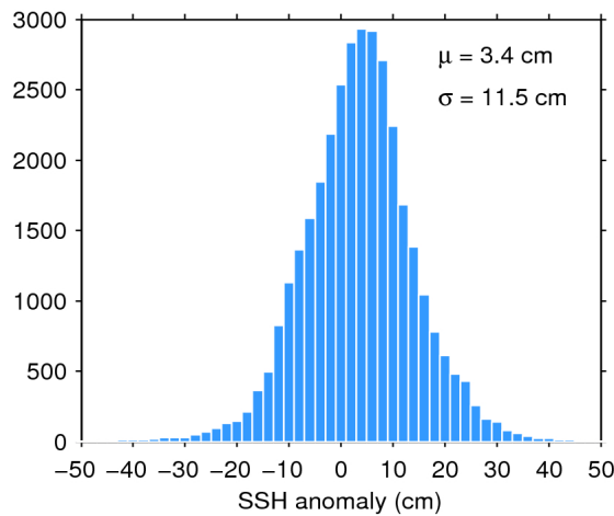
Figure 11. Histogram of science-valid SSH anomaly over oceans and lakes for 12/05/2017. The mean ( \mu ) and standard deviation ( \sigma ) are also shown. Note that values outside [-50 50] cm are excluded from the histogram for the sake of readability but not from the computation of \mu and \sigma .
