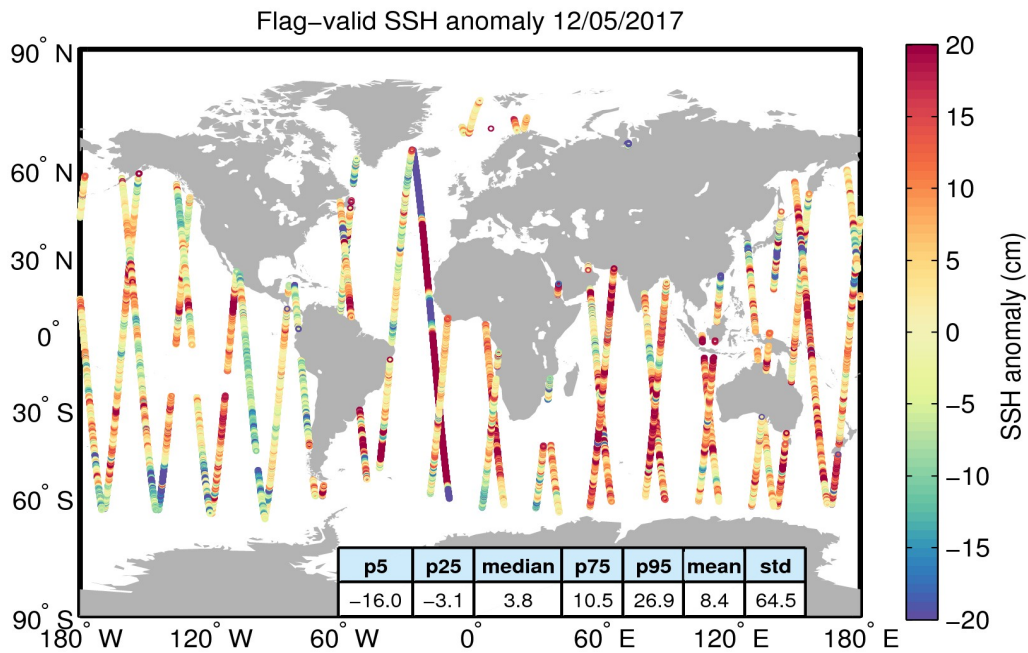
Figure 5. Geographical distribution of flag-valid 1-Hz SSH anomaly data over oceans and lakes for 12/05/2017. The statistical values shown in the table refer to the SSH anomaly in cm and are calculated over all measurements shown in the figure.
