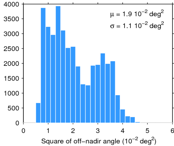
Figure 39. Histogram of flag-valid mispointing over oceans and lakes for 12/05/2017. The mean ( \mu ) and standard deviation ( \sigma ) are also shown. Note that values larger than 6 \cdot 10^{-2} \text{ deg}^2 are excluded from the histogram for the sake of readability but not from the computation of \mu and \sigma .
