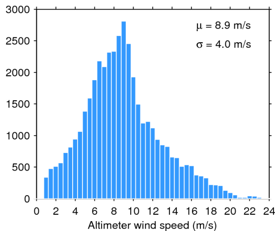
Figure 35. Histogram of science-valid wind over oceans and lakes for 12/05/2017. The mean ( \mu ) and standard deviation ( \sigma ) are also shown. Note that values larger than 24 m/s are excluded from the histogram for the sake of readability but not from the computation of \mu and \sigma .
