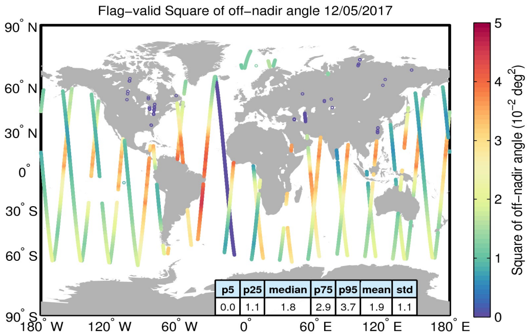
Figure 37. Geographical distribution of flag-valid mispointing data over oceans and lakes for 12/05/2017. The statistical values shown in the table refer to the mispointing in 10^{-2} deg 2 and are calculated over all measurements shown in the figure.
