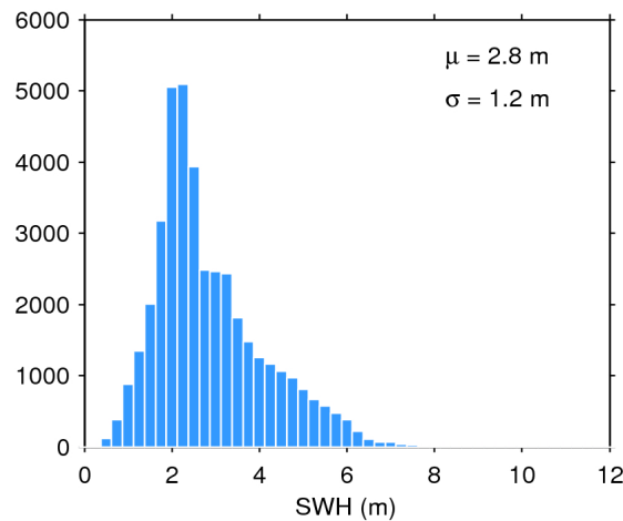
Figure 20. Histogram of science-valid SWH over oceans and lakes for 11/05/2017. The mean ( \mu ) and standard deviation ( \sigma ) are also shown. Note that values larger than 12 m are excluded from the histogram for the sake of readability but not from the computation of \mu and \sigma .
