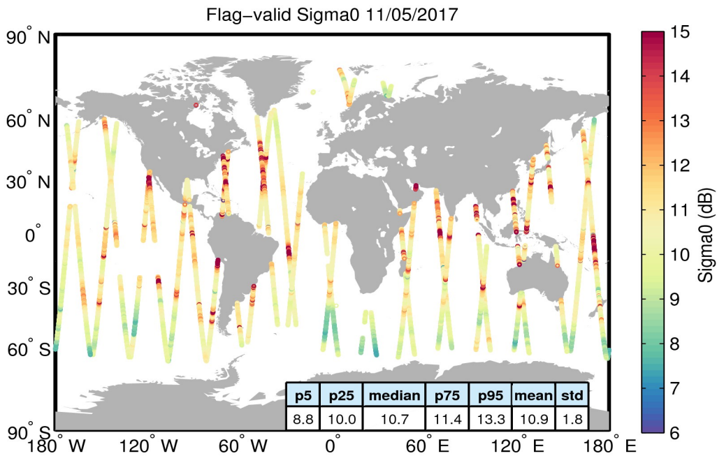
Figure 23. Geographical distribution of flag-valid sigma0 data over oceans and lakes for 11/05/2017. The statistical values shown in the table refer to the sigma0 in dB and are calculated over all measurements shown in the figure.
