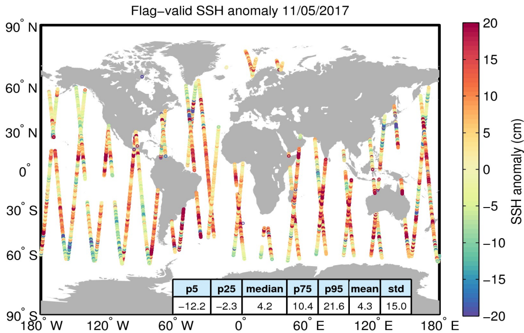
Figure 5. Geographical distribution of flag-valid 1-Hz SSH anomaly data over oceans and lakes for 11/05/2017. The statistical values shown in the table refer to the SSH anomaly in cm and are calculated over all measurements shown in the figure.
