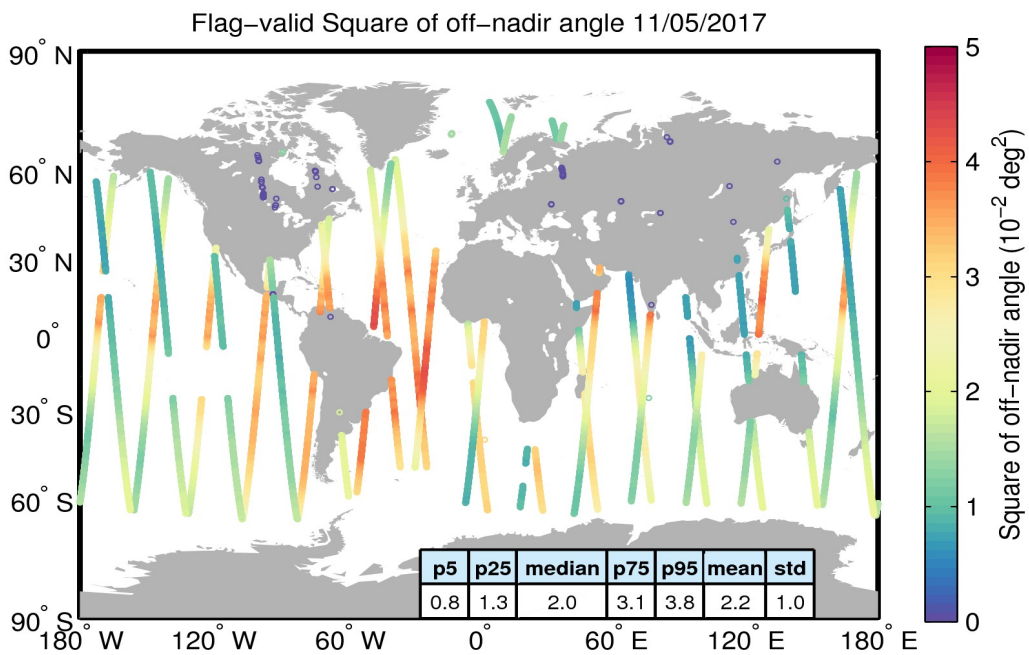
Figure 37. Geographical distribution of flag-valid mispointing data over oceans and lakes for 11/05/2017. The statistical values shown in the table refer to the mispointing in 10^{-2} deg 2 and are calculated over all measurements shown in the figure.
