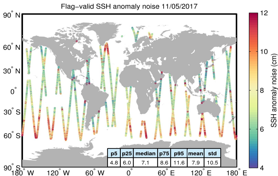
Figure 8. Geographical distribution of flag-valid 20-Hz SSH anomaly measurement noise over oceans and lakes for 11/05/2017. The statistical values shown in the table refer to the SSH anomaly noise and are calculated over all measurements shown in the figure.
