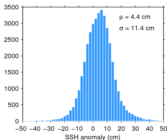
Figure 11. Histogram of science-valid SSH anomaly over oceans and lakes for 11/05/2017. The mean ( \mu ) and standard deviation ( \sigma ) are also shown. Note that values outside [-50 50] cm are excluded from the histogram for the sake of readability but not from the computation of \mu and \sigma .
