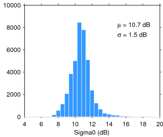
Figure 28. Histogram of science-valid sigma0 over oceans and lakes for 11/05/2017. The mean ( \mu ) and standard deviation ( \sigma ) are also shown. Note that values outside [4 20] dB are excluded from the histogram for the sake of readability but not from the computation of \mu and \sigma .
