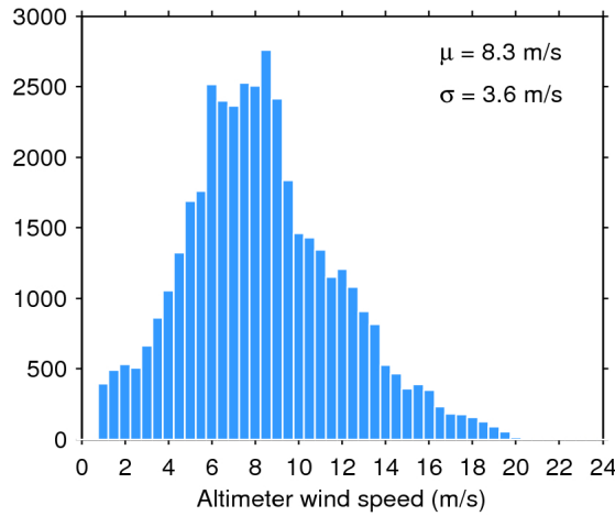
Figure 33. Histogram of flag-valid wind over oceans and lakes for 11/05/2017. The mean ( \mu ) and standard deviation ( \sigma ) are also shown. Note that values larger than 24 m/s are excluded from the histogram for the sake of readability but not from the computation of \mu and \sigma .
