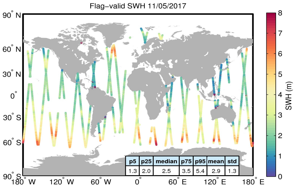
Figure 15. Geographical distribution of flag-valid SWH data over oceans and lakes for 11/05/2017. The statistical values shown in the table refer to the SWH in m and are calculated over all measurements shown in the figure.
