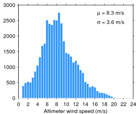
Figure 35. Histogram of science-valid wind over oceans and lakes for 11/05/2017. The mean ( \mu ) and standard deviation ( \sigma ) are also shown. Note that values larger than 24 m/s are excluded from the histogram for the sake of readability but not from the computation of \mu and \sigma .
