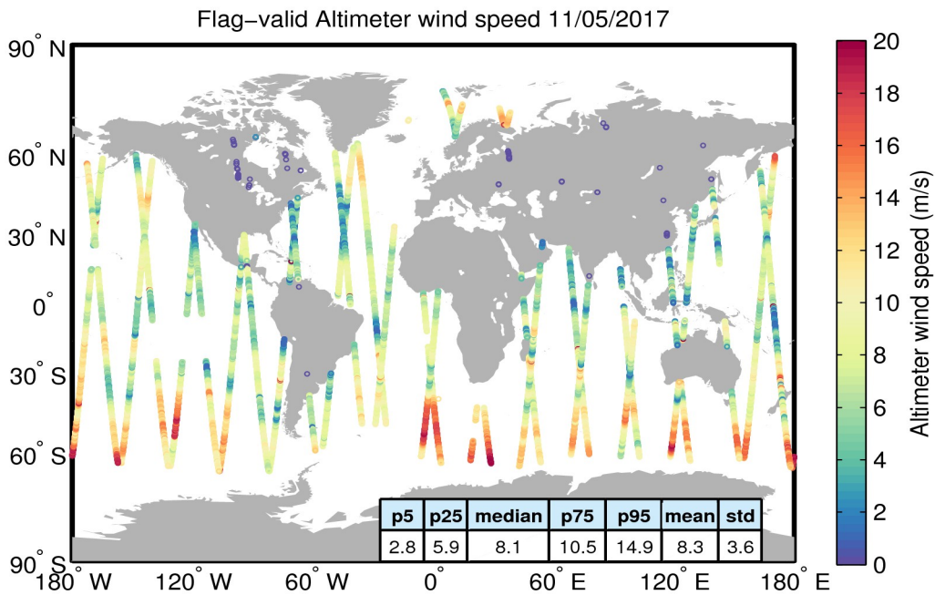
Figure 31. Geographical distribution of flag-valid wind data over oceans and lakes for 11/05/2017. The statistical values shown in the table refer to the wind in m/s and are calculated over all measurements shown in the figure.
