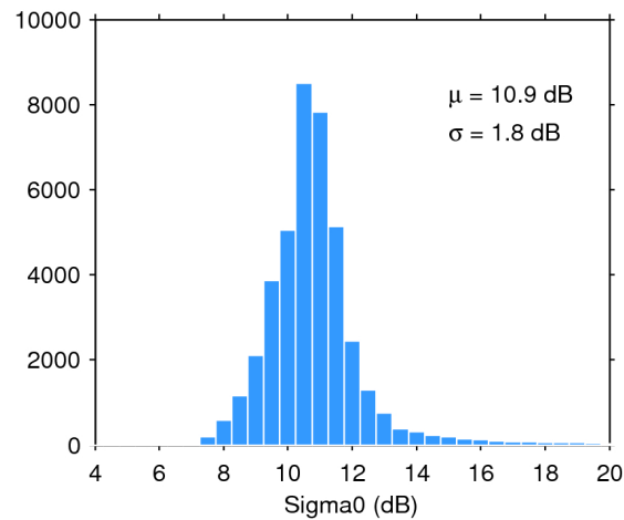
Figure 25. Histogram of flag-valid sigma0 over oceans and lakes for 11/05/2017. The mean ( \mu ) and standard deviation ( \sigma ) are also shown. Note that values outside [4 20] dB are excluded from the histogram for the sake of readability but not from the computation of \mu and \sigma .
