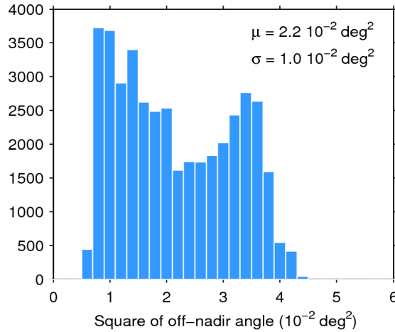
Figure 39. Histogram of flag-valid mispointing over oceans and lakes for 11/05/2017. The mean ( \mu ) and standard deviation ( \sigma ) are also shown. Note that values larger than 6 \cdot 10^{-2} \text{ deg}^2 are excluded from the histogram for the sake of readability but not from the computation of \mu and \sigma .
