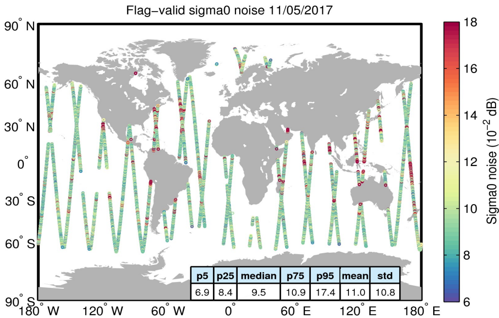
Figure 26. Geographical distribution of flag-valid 20-Hz sigma0 measurement noise over oceans and lakes for 11/05/2017. The statistical values shown in the table refer to the sigma0 noise and are calculated over all measurements shown in the figure.
