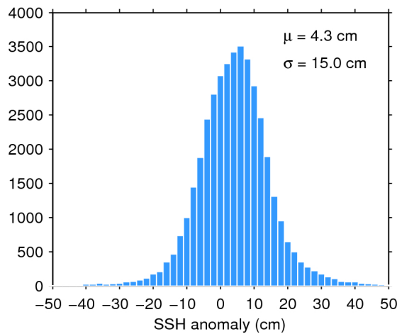
Figure 7. Histogram of flag-valid SSH anomaly over oceans and lakes for 11/05/2017. The mean ( \mu ) and standard deviation ( \sigma ) are also shown. Note that values outside [-50 50] cm are excluded from the histogram for the sake of readability but not from the computation of \mu and \sigma .
