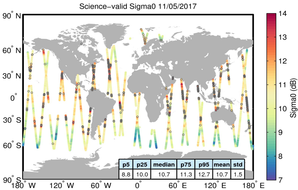
Figure 27. Geographical distribution of science-valid sigma0 data over oceans and lakes for 11/05/2017. The statistical values shown in the table refer to the sigma0 in dB and are calculated over all measurements shown in the figure. Gray circles denote records that have been rejected based on the editing criteria described in Table 4.
