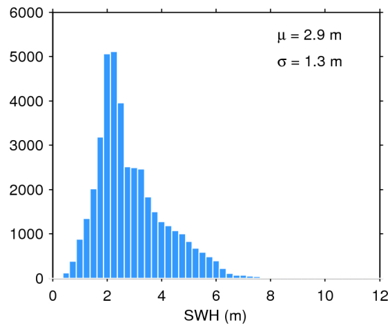
Figure 17. Histogram of flag-valid SWH over oceans and lakes for 11/05/2017. The mean ( \mu ) and standard deviation ( \sigma ) are also shown. Note that values larger than 12 m are excluded from the histogram for the sake of readability but not from the computation of \mu and \sigma .
