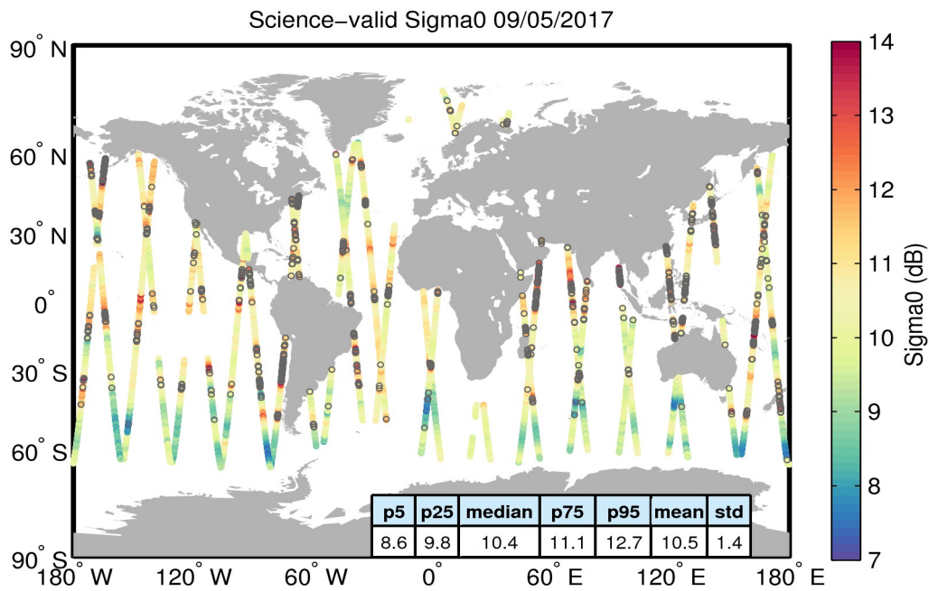
Figure 27. Geographical distribution of science-valid sigma0 data over oceans and lakes for 09/05/2017. The statistical values shown in the table refer to the sigma0 in dB and are calculated over all measurements shown in the figure. Gray circles denote records that have been rejected based on the editing criteria described in Table 4.
