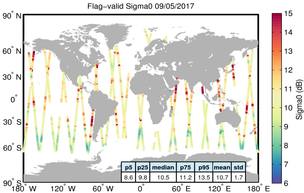
Figure 23. Geographical distribution of flag-valid sigma0 data over oceans and lakes for 09/05/2017. The statistical values shown in the table refer to the sigma0 in dB and are calculated over all measurements shown in the figure.
