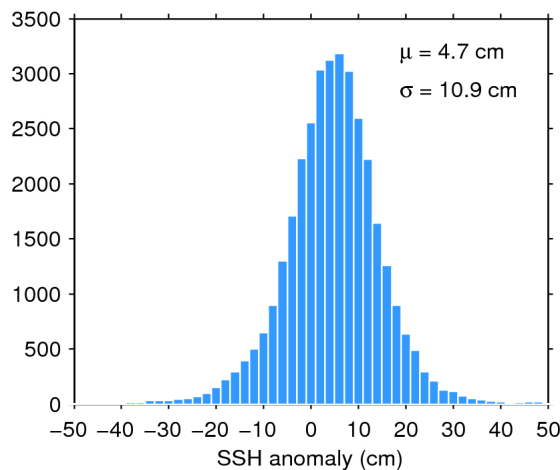
Figure 11. Histogram of science-valid SSH anomaly over oceans and lakes for 09/05/2017. The mean ( \mu ) and standard deviation ( \sigma ) are also shown. Note that values outside [-50 50] cm are excluded from the histogram for the sake of readability but not from the computation of \mu and \sigma .
