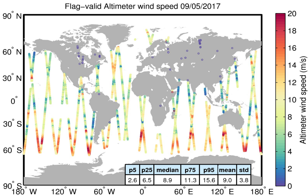
Figure 31. Geographical distribution of flag-valid wind data over oceans and lakes for 09/05/2017. The statistical values shown in the table refer to the wind in m/s and are calculated over all measurements shown in the figure.
