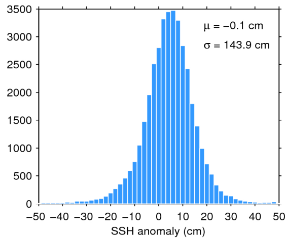
Figure 7. Histogram of flag-valid SSH anomaly over oceans and lakes for 09/05/2017. The mean ( \mu ) and standard deviation ( \sigma ) are also shown. Note that values outside [-50 50] cm are excluded from the histogram for the sake of readability but not from the computation of \mu and \sigma .
