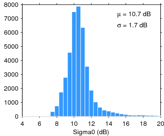
Figure 25. Histogram of flag-valid sigma0 over oceans and lakes for 09/05/2017. The mean ( \mu ) and standard deviation ( \sigma ) are also shown. Note that values outside [4 20] dB are excluded from the histogram for the sake of readability but not from the computation of \mu and \sigma .
