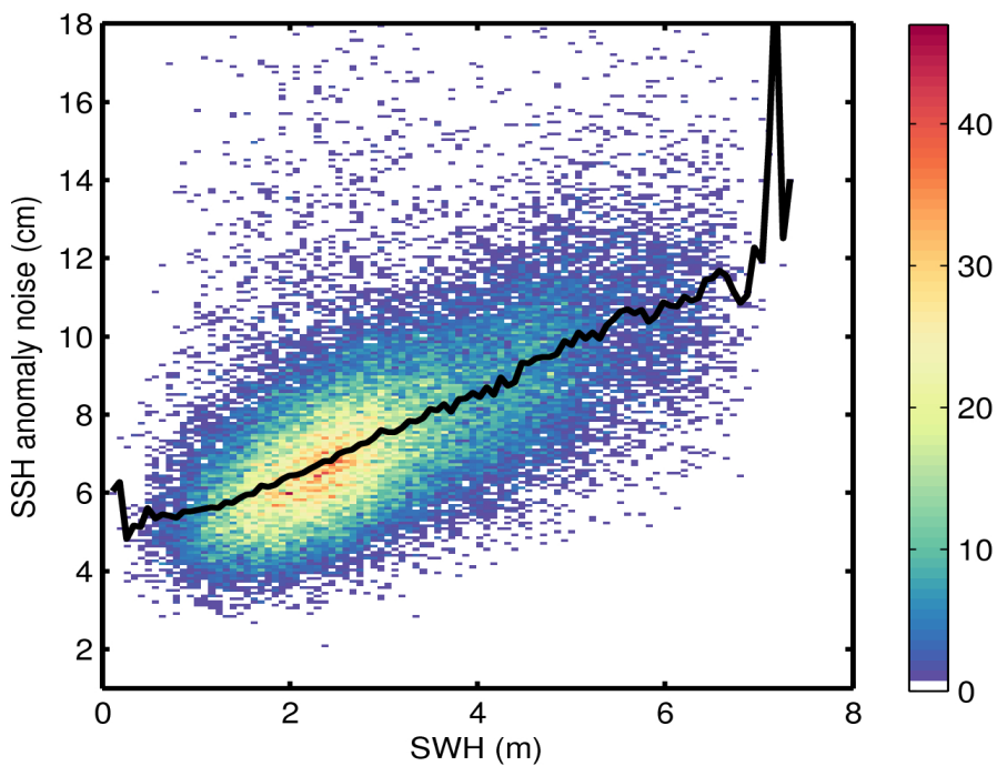
Figure 9. 2D histogram showing flag-valid SSH anomaly noise as a function of SWH for 09/05/2017. The black line denotes the median SSH anomaly noise as a function of SWH.
