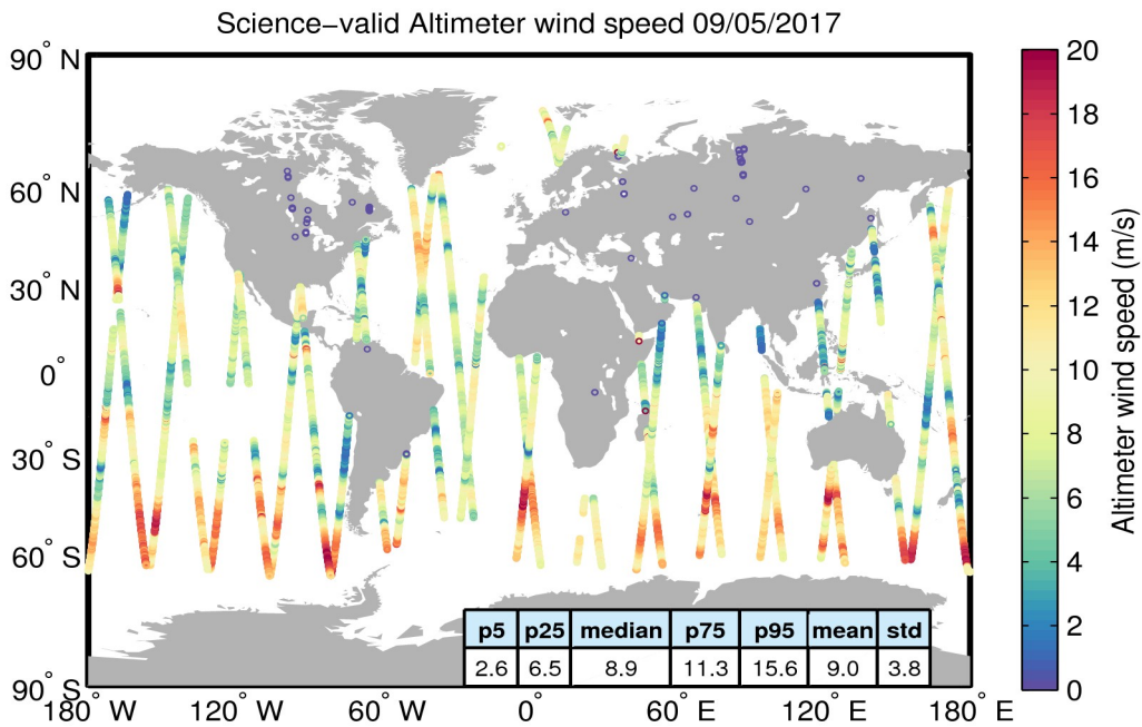
Figure 34. Geographical distribution of science-valid wind data over oceans and lakes for 09/05/2017. The statistical values shown in the table refer to the wind in m/s and are calculated over all measurements shown in the figure. Gray circles denote records that have been rejected based on the editing criteria described in Table 5.
