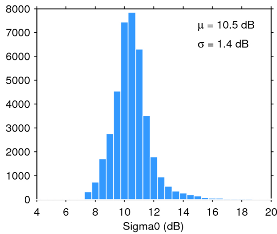
Figure 28. Histogram of science-valid sigma0 over oceans and lakes for 09/05/2017. The mean ( \mu ) and standard deviation ( \sigma ) are also shown. Note that values outside [4 20] dB are excluded from the histogram for the sake of readability but not from the computation of \mu and \sigma .
