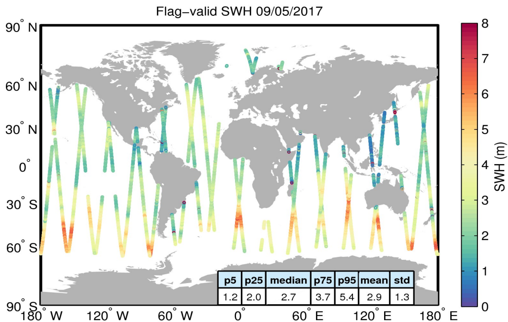
Figure 15. Geographical distribution of flag-valid SWH data over oceans and lakes for 09/05/2017. The statistical values shown in the table refer to the SWH in m and are calculated over all measurements shown in the figure.
