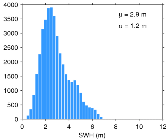
Figure 20. Histogram of science-valid SWH over oceans and lakes for 09/05/2017. The mean ( \mu ) and standard deviation ( \sigma ) are also shown. Note that values larger than 12 m are excluded from the histogram for the sake of readability but not from the computation of \mu and \sigma .
