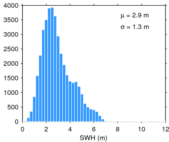
Figure 17. Histogram of flag-valid SWH over oceans and lakes for 09/05/2017. The mean ( \mu ) and standard deviation ( \sigma ) are also shown. Note that values larger than 12 m are excluded from the histogram for the sake of readability but not from the computation of \mu and \sigma .
