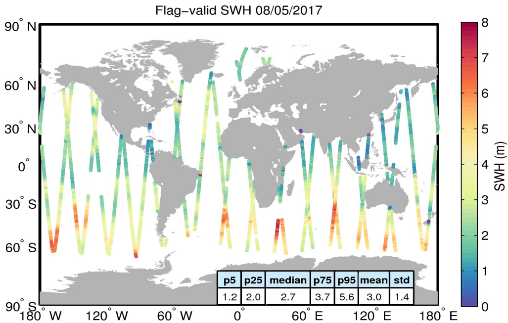
Figure 15. Geographical distribution of flag-valid SWH data over oceans and lakes for 08/05/2017. The statistical values shown in the table refer to the SWH in m and are calculated over all measurements shown in the figure.
