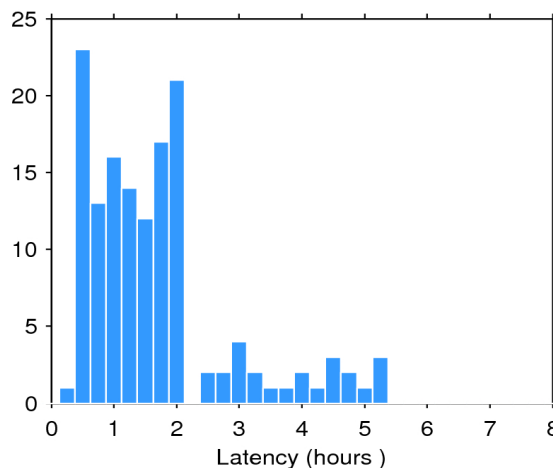
Figure 2. Histogram of the data latency for 08/05/2017. The y-axis denotes the number of files that are made available with a delay of x-hours with respect to the mean time of the records stored in the file.
