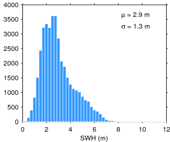
Figure 20. Histogram of science-valid SWH over oceans and lakes for 08/05/2017. The mean ( \mu ) and standard deviation ( \sigma ) are also shown. Note that values larger than 12 m are excluded from the histogram for the sake of readability but not from the computation of \mu and \sigma .
