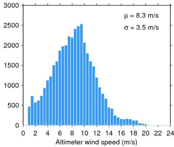
Figure 33. Histogram of flag-valid wind over oceans and lakes for 08/05/2017. The mean ( \mu ) and standard deviation ( \sigma ) are also shown. Note that values larger than 24 m/s are excluded from the histogram for the sake of readability but not from the computation of \mu and \sigma .
