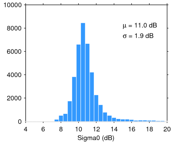
Figure 25. Histogram of flag-valid sigma0 over oceans and lakes for 08/05/2017. The mean ( \mu ) and standard deviation ( \sigma ) are also shown. Note that values outside [4 20] dB are excluded from the histogram for the sake of readability but not from the computation of \mu and \sigma .
