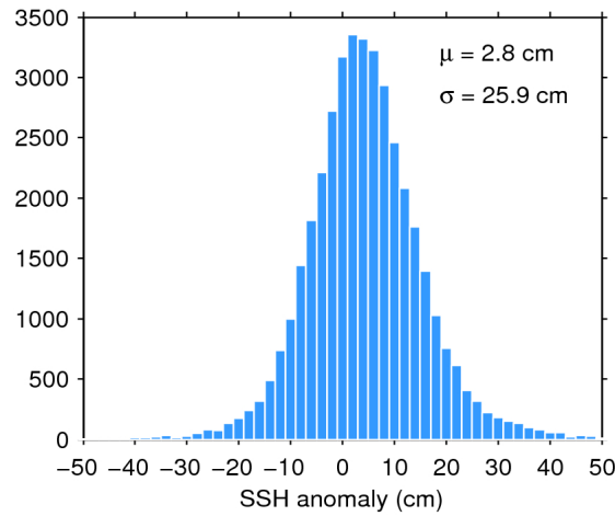
Figure 7. Histogram of flag-valid SSH anomaly over oceans and lakes for 08/05/2017. The mean ( \mu ) and standard deviation ( \sigma ) are also shown. Note that values outside [-50\ 50] cm are excluded from the histogram for the sake of readability but not from the computation of \mu and \sigma .
