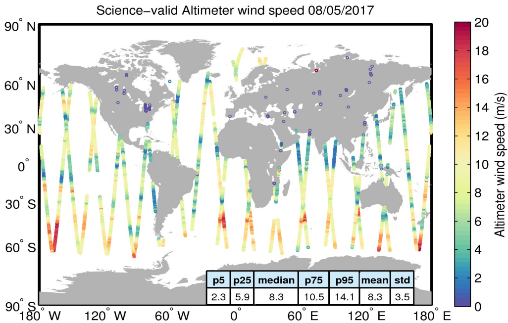
Figure 34. Geographical distribution of science-valid wind data over oceans and lakes for 08/05/2017. The statistical values shown in the table refer to the wind in m/s and are calculated over all measurements shown in the figure. Gray circles denote records that have been rejected based on the editing criteria described in Table 5.
