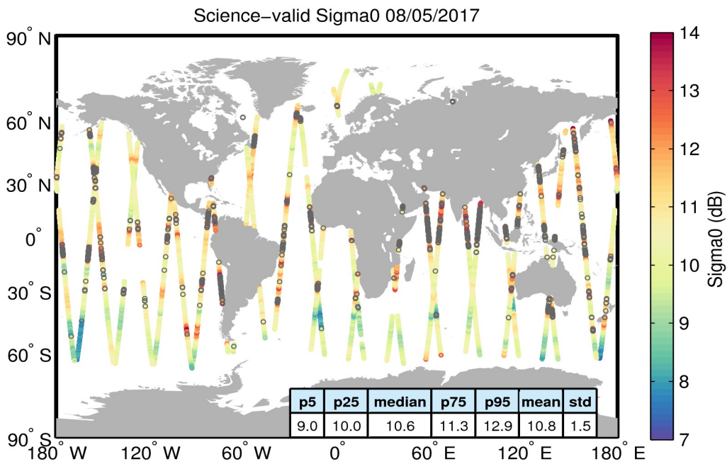
Figure 27. Geographical distribution of science-valid sigma0 data over oceans and lakes for 08/05/2017. The statistical values shown in the table refer to the sigma0 in dB and are calculated over all measurements shown in the figure. Gray circles denote records that have been rejected based on the editing criteria described in Table 4.
