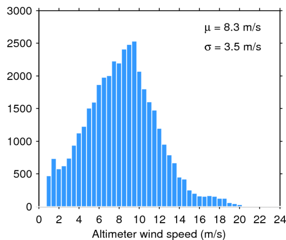
Figure 35. Histogram of science-valid wind over oceans and lakes for 08/05/2017. The mean ( \mu ) and standard deviation ( \sigma ) are also shown. Note that values larger than 24 m/s are excluded from the histogram for the sake of readability but not from the computation of \mu and \sigma .
