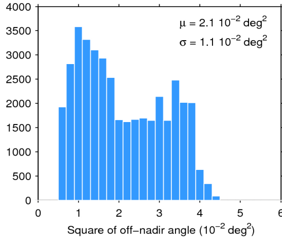
Figure 39. Histogram of flag-valid mispointing over oceans and lakes for 08/05/2017. The mean ( \mu ) and standard deviation ( \sigma ) are also shown. Note that values larger than 6 \cdot 10^{-2} \text{ deg}^2 are excluded from the histogram for the sake of readability but not from the computation of \mu and \sigma .
