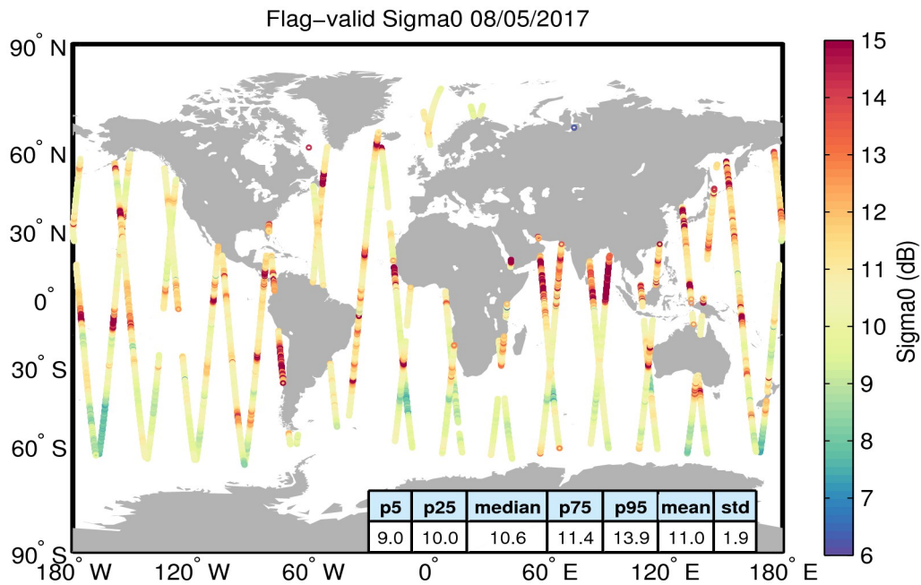
Figure 23. Geographical distribution of flag-valid sigma0 data over oceans and lakes for 08/05/2017. The statistical values shown in the table refer to the sigma0 in dB and are calculated over all measurements shown in the figure.
