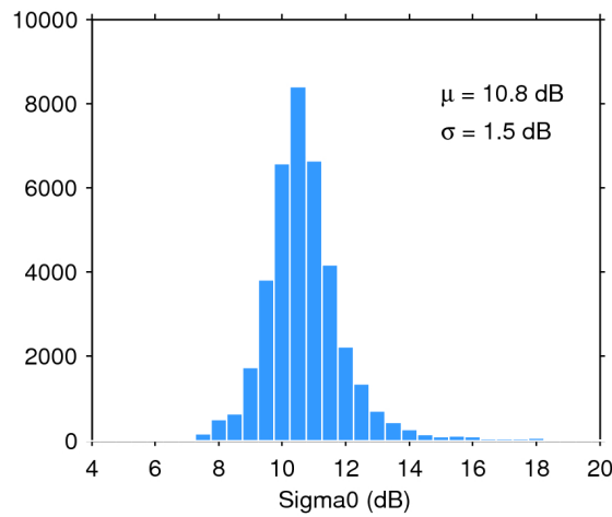
Figure 28. Histogram of science-valid sigma0 over oceans and lakes for 08/05/2017. The mean ( \mu ) and standard deviation ( \sigma ) are also shown. Note that values outside [4 20] dB are excluded from the histogram for the sake of readability but not from the computation of \mu and \sigma .
