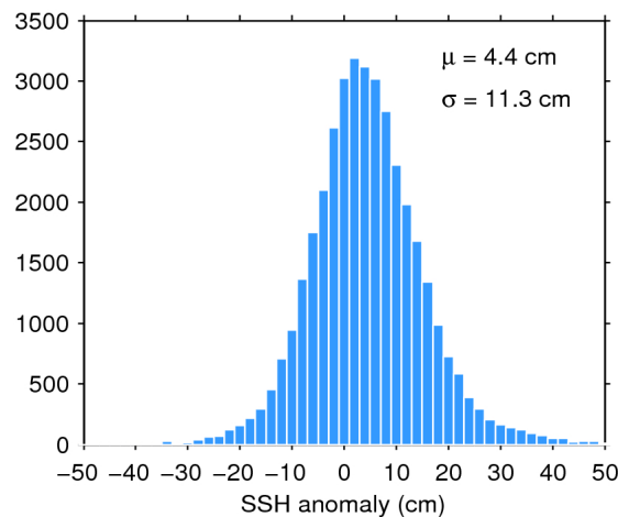
Figure 11. Histogram of science-valid SSH anomaly over oceans and lakes for 08/05/2017. The mean ( \mu ) and standard deviation ( \sigma ) are also shown. Note that values outside [-50 50] cm are excluded from the histogram for the sake of readability but not from the computation of \mu and \sigma .
