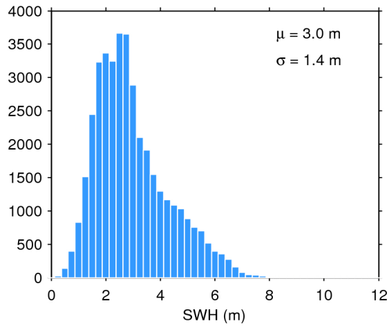
Figure 17. Histogram of flag-valid SWH over oceans and lakes for 08/05/2017. The mean ( \mu ) and standard deviation ( \sigma ) are also shown. Note that values larger than 12 m are excluded from the histogram for the sake of readability but not from the computation of \mu and \sigma .
