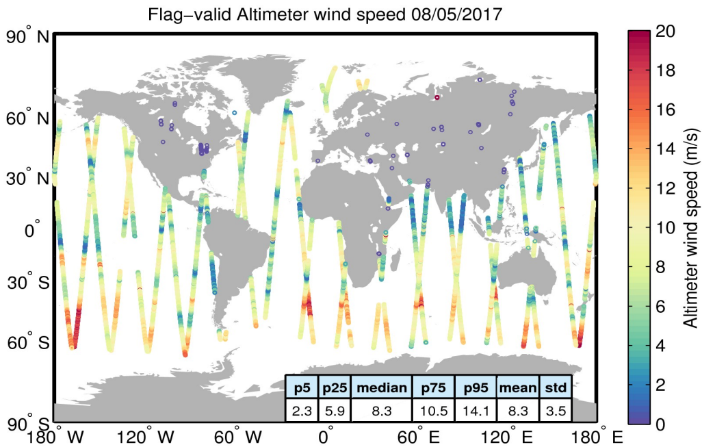
Figure 31. Geographical distribution of flag-valid wind data over oceans and lakes for 08/05/2017. The statistical values shown in the table refer to the wind in m/s and are calculated over all measurements shown in the figure.
