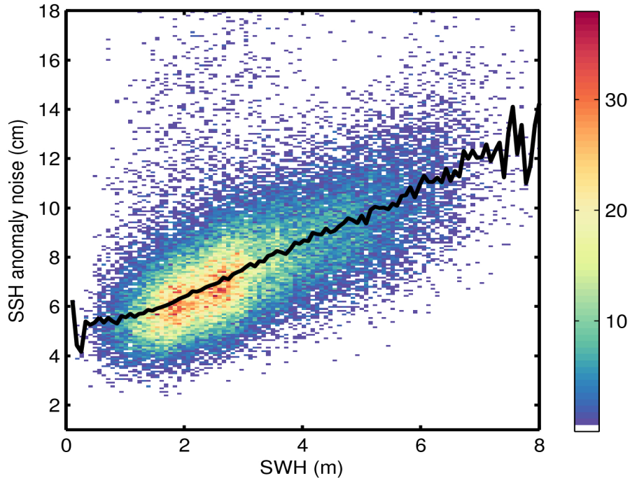
Figure 9. 2D histogram showing flag-valid SSH anomaly noise as a function of SWH for 08/05/2017. The black line denotes the median SSH anomaly noise as a function of SWH.
